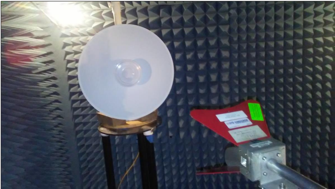
Photograph 2. Radiated Emissions Above 1GHz, 27dBi antenna – Setup photo
