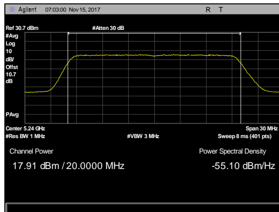
Plot 51. Conducted Transmitter Output Power, BW 20M, CF 5240M, 27dBi, c0
