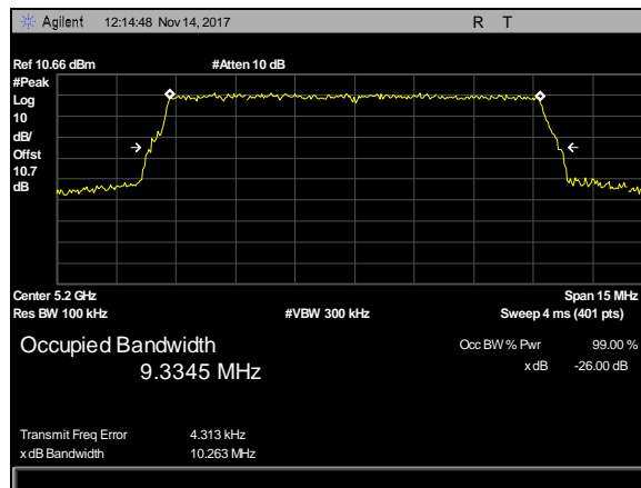
Plot 2. 26 dB - 99% Occupied Bandwidth, BW 10M, CF 5200M
