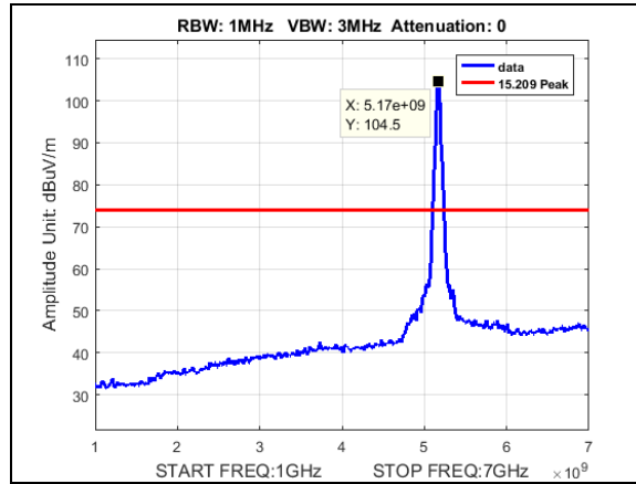
Plot 223. Undesirable Emissions, Peak radiated spurious BW 40M, CF 5170M, 27dBi, 1-7GHz
