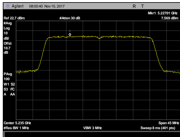
Plot 84. Power Spectral Density, BW 30M, CF 5235M, 19dBi, c0
