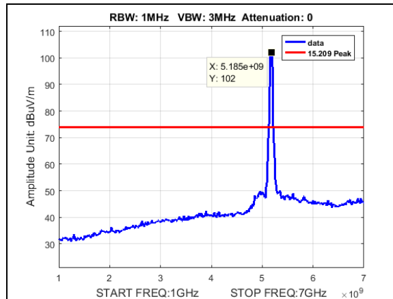
Plot 194. Undesirable Emissions, Peak radiated spurious BW 50M, CF 5175M, 19dBi, 1-7GHz
