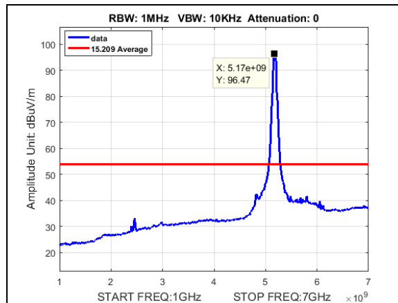
Plot 210. Undesirable Emissions, Average radiated spurious BW 50M, CF 5175M, 27dBi, 1-7GHz
