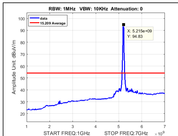
Plot 176. Undesirable Emissions, Average radiated spurious BW 40M, CF 5200M, 19dBi, 1-7GHz
