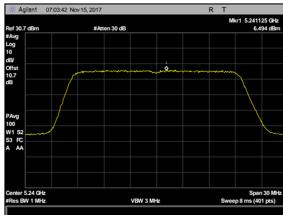
Plot 66. Power Spectral Density, BW 20M, CF 5240M, 27dBm, c0
