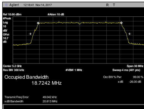
Plot 5. 26 dB - 99% Occupied Bandwidth, BW 20M, CF 5200M
