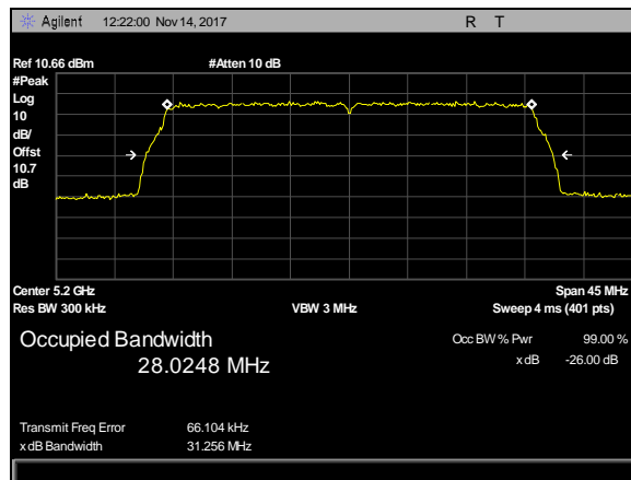
Plot 8. 26 dB - 99% Occupied Bandwidth, BW 30M, CF 5200M
