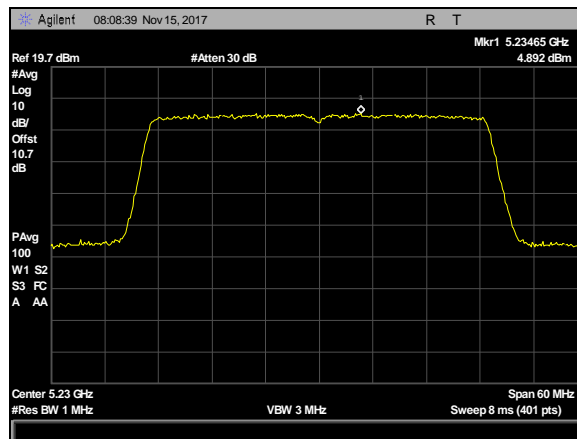
Plot 87. Power Spectral Density, BW 40M, CF 5230M, 19dBi, c0
