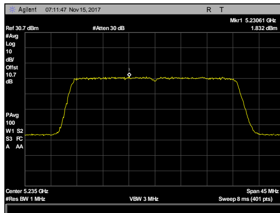
Plot 69. Power Spectral Density, BW 30M, CF 5235M, 27dBi, c0
