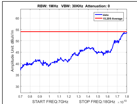
Plot 181. Undesirable Emissions, Average radiated spurious Worst Case 19dBi, 7-18GHz
