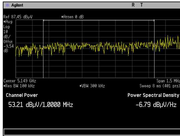
Plot 107. Undesirable Emissions, Average radiated band edge 5150 BW 20M, 5160M, 13dBi, V
