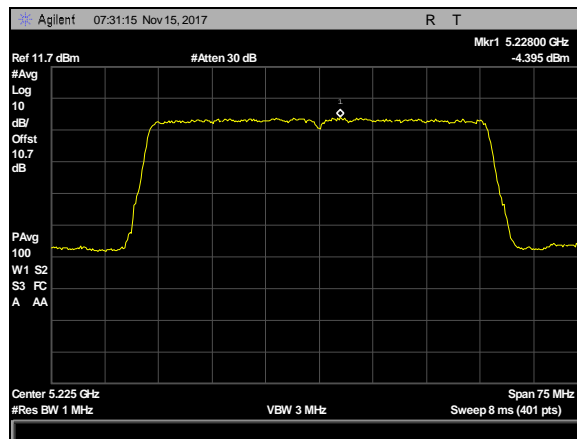
Plot 75. Power Spectral Density, BW 50M, CF 5225M, 27dBi, c0
