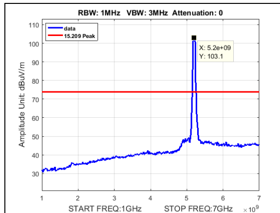
Plot 195. Undesirable Emissions, Peak radiated spurious BW 50M, CF 5200M, 19dBi, 1-7GHz
