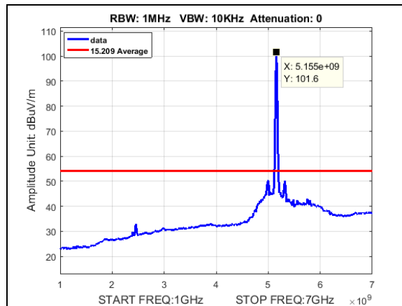
Plot 198. Undesirable Emissions, Average radiated spurious BW 10M, CF 5155M, 27dBi, 1-7GHz
