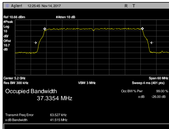
Plot 11. 26 dB - 99% Occupied Bandwidth, BW 40M, CF 5200M
