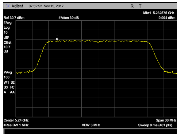
Plot 81. Power Spectral Density, BW 20M, CF 5240M, 19dBi, c0
