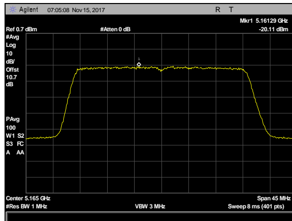
Plot 67. Power Spectral Density, BW 30M, CF 5165M, 27dBm, c0
