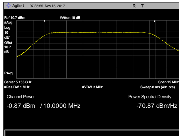
Plot 31. Conducted Transmitter Output Power, BW 10M, CF 5155M, 19dBi, c0
