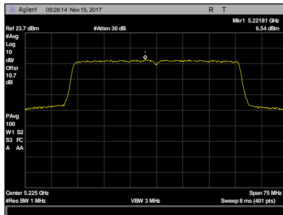
Plot 105. Power Spectral Density, BW 50M, CF 5225M, 13dBi, c0
