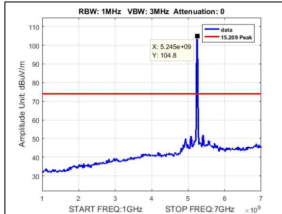
Plot 184. Undesirable Emissions, Peak radiated spurious BW 10M, CF 5245M, 19dBi, 1-7GHz
