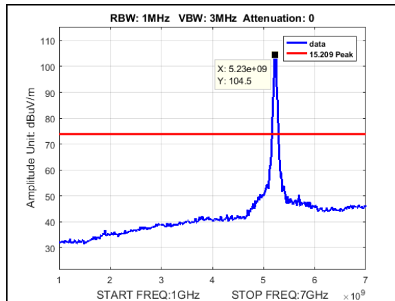
Plot 225. Undesirable Emissions, Peak radiated spurious BW 40M, CF 5230M, 27dBi, 1-7GHz
