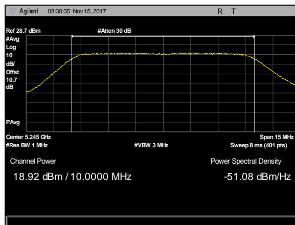
Plot 18. Conducted Transmitter Output Power, BW 10M, CF 5245M, 13dBi, c0
