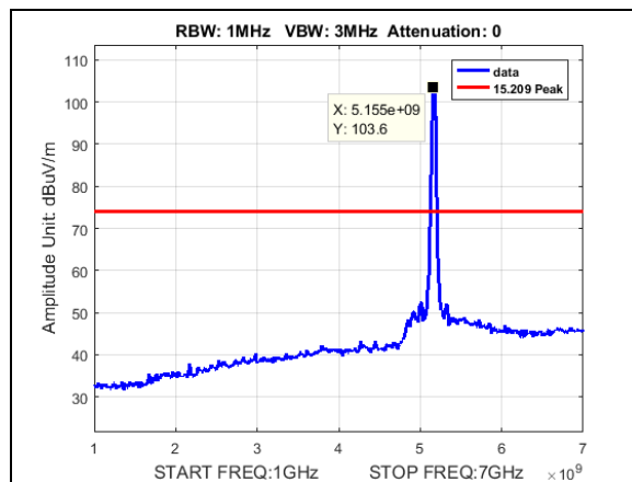
Plot 188. Undesirable Emissions, Peak radiated spurious BW 30M, CF 5165M, 19dBi, 1-7GHz
