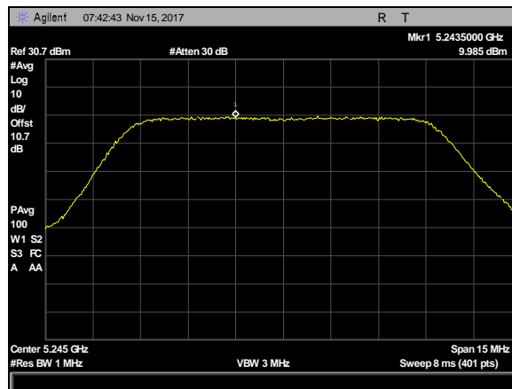
Plot 78. Power Spectral Density, BW 10M, CF 5245M, 19dBi, c0
