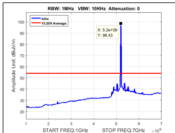
Plot 167. Undesirable Emissions, Average radiated spurious BW 10M, CF 5200M, 19dBi, 1-7GHz
