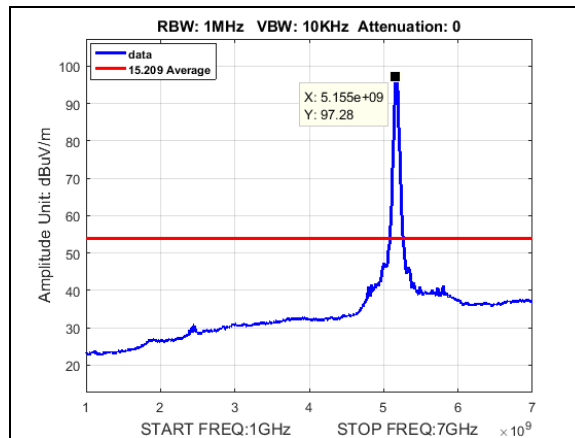
Plot 207. Undesirable Emissions, Average radiated spurious BW 40M, CF 5170M, 27dBi, 1-7GHz
