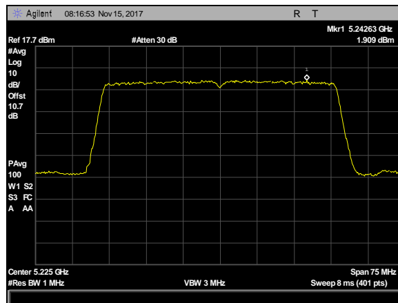
Plot 90. Power Spectral Density, BW 50M, CF 5225M, 19dBi, c0
