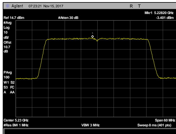
Plot 72. Power Spectral Density, BW 40M, CF 5230M, 27dBi, c0
