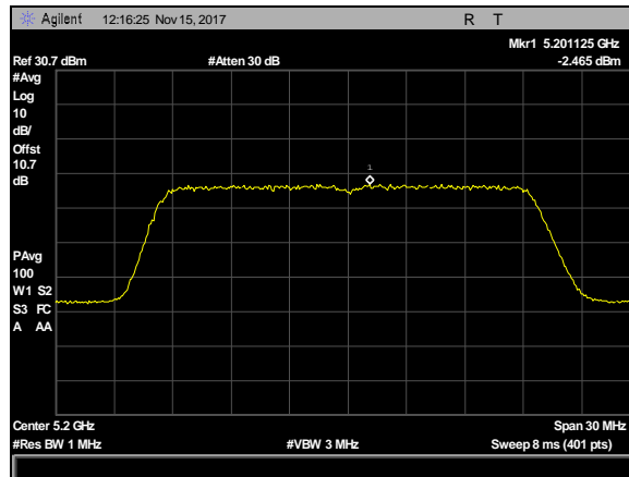
Plot 65. Power Spectral Density, BW 20M, CF 5200M, 27dBm, c0
