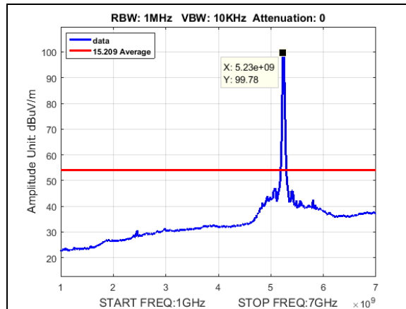
Plot 203. Undesirable Emissions, Average radiated spurious BW 20M, CF 5240M, 27dBi, 1-7GHz
