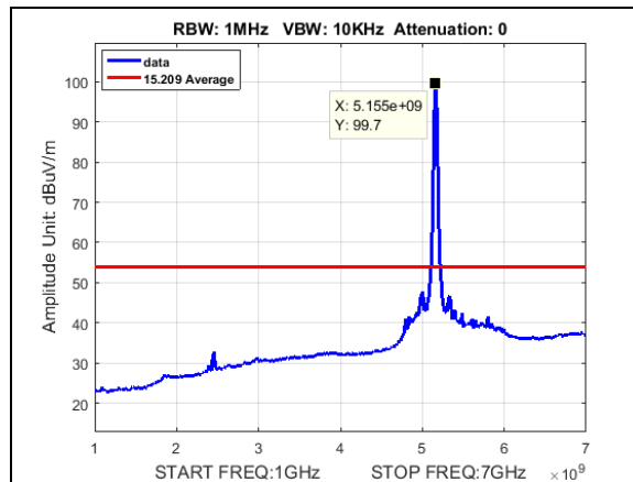
Plot 201. Undesirable Emissions, Average radiated spurious BW 20M, CF 5160M, 27dBi, 1-7GHz
