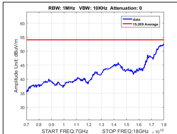
Plot 213. Undesirable Emissions, Average radiated spurious worst case 27dBi, 7-18GHz
