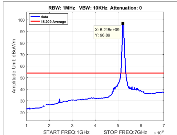
Plot 212. Undesirable Emissions, Average radiated spurious BW 50M, CF 5225M, 27dBi, 1-7GHz
