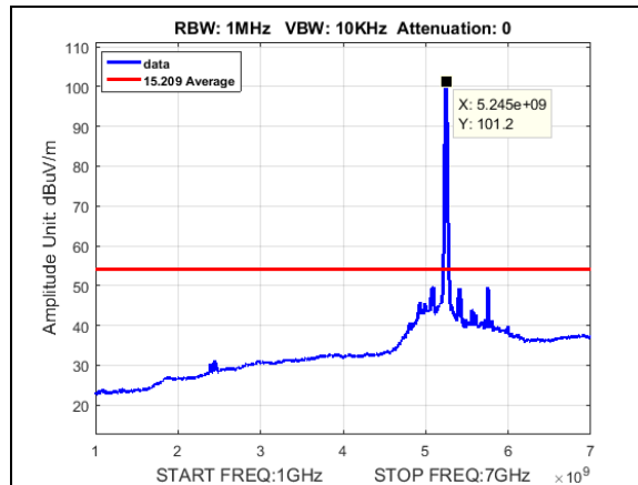
Plot 200. Undesirable Emissions, Average radiated spurious BW 10M, CF 5245M, 27dBi, 1-7GHz
