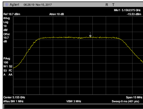
Plot 61. Power Spectral Density, BW 10M, CF 5155M, 27dBi, c0
