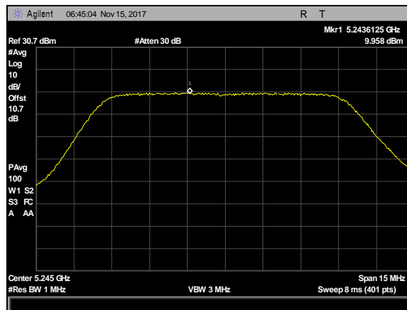
Plot 63. Power Spectral Density, BW 10M, CF 5245M, 27dBi, c0
