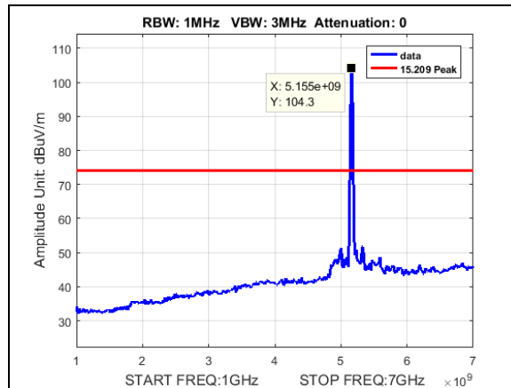
Plot 185. Undesirable Emissions, Peak radiated spurious BW 20M, CF 5160M, 19dBi, 1-7GHz
