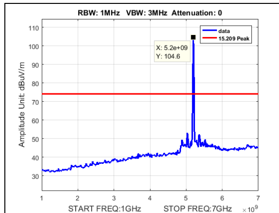
Plot 183. Undesirable Emissions, Peak radiated spurious BW 10M, CF 5200M, 19dBi, 1-7GHz
