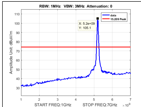
Plot 224. Undesirable Emissions, Peak radiated spurious BW 40M, CF 5200M, 27dBi, 1-7GHz
