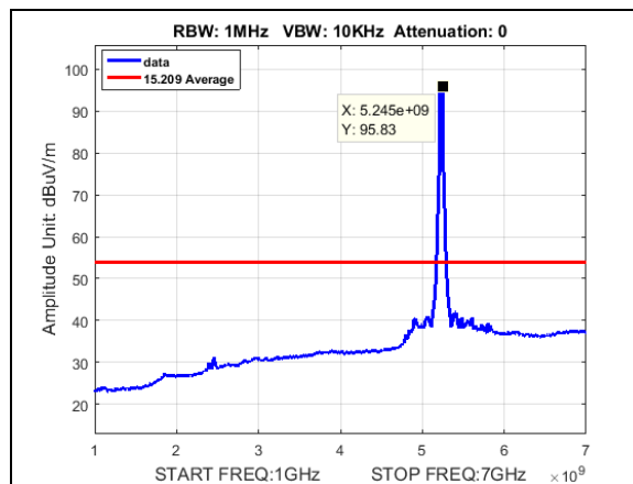
Plot 177. Undesirable Emissions, Average radiated spurious BW 40M, CF 5230M, 19dBi, 1-7GHz
