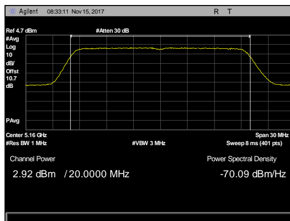
Plot 19. Conducted Transmitter Output Power, BW 20M, CF 5160M, 13dBi, c0
