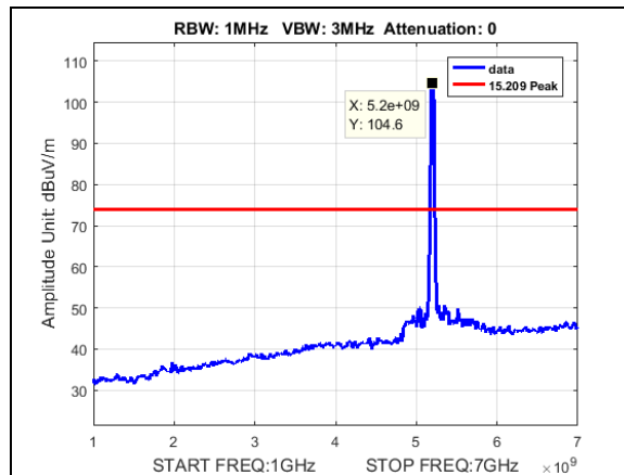
Plot 186. Undesirable Emissions, Peak radiated spurious BW 20M, CF 5200M, 19dBi, 1-7GHz
