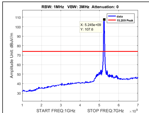
Plot 219. Undesirable Emissions, Peak radiated spurious BW 20M, CF 5240M, 27dBi, 1-7GHz
