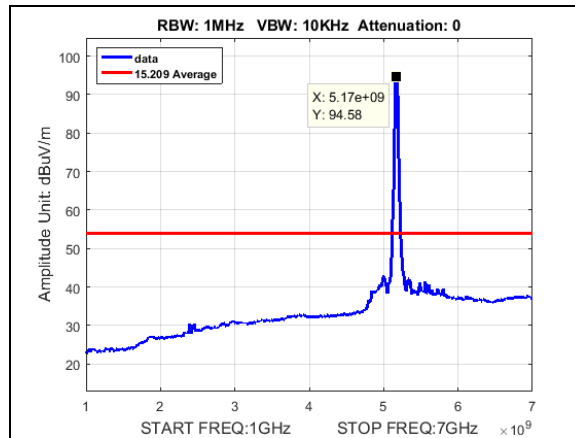
Plot 175. Undesirable Emissions, Average radiated spurious BW 40M, CF 5170M, 19dBi, 1-7GHz
