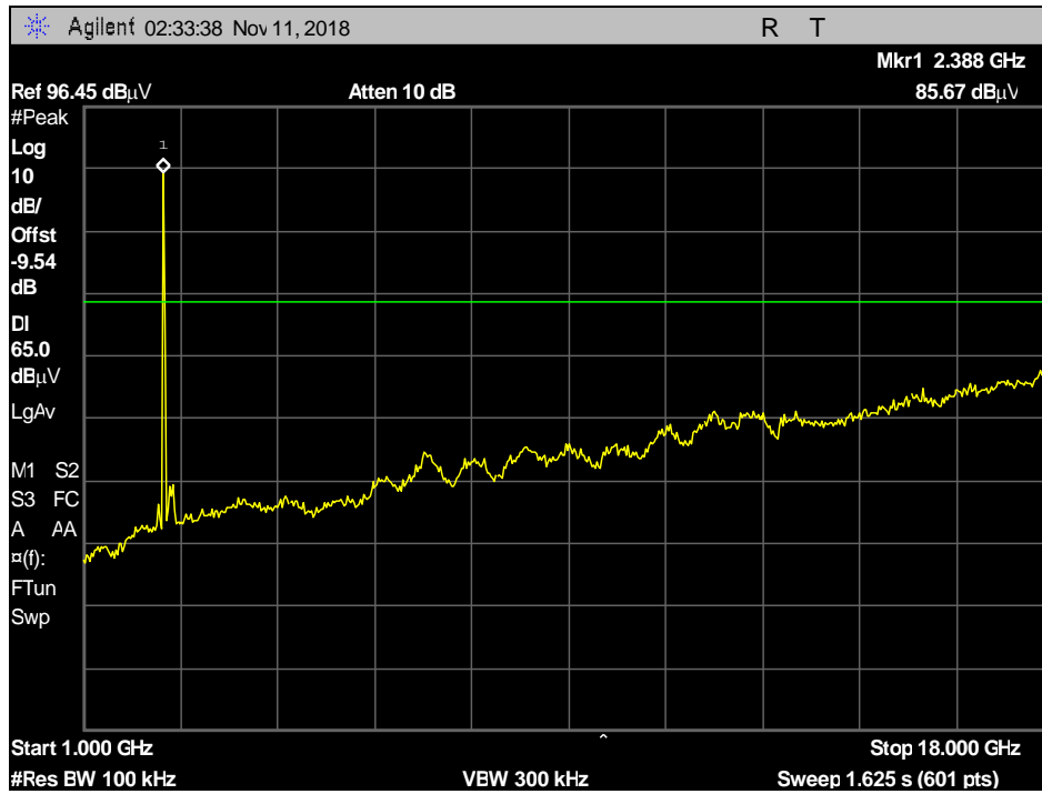
Plot 107. Conducted Spurious Emissions, Nonhopping, 2402MHz, DH1, 1 GHz – 18 GHz
