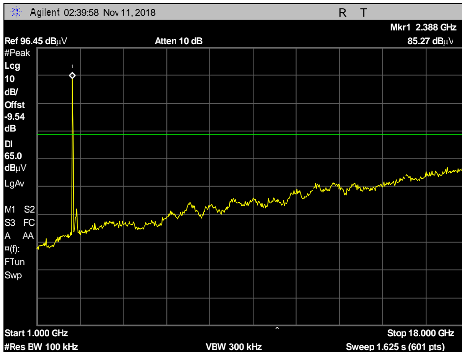
Plot 108. Conducted Spurious Emissions, Nonhopping, 2402MHz, DH5, 1 GHz – 18 GHz
