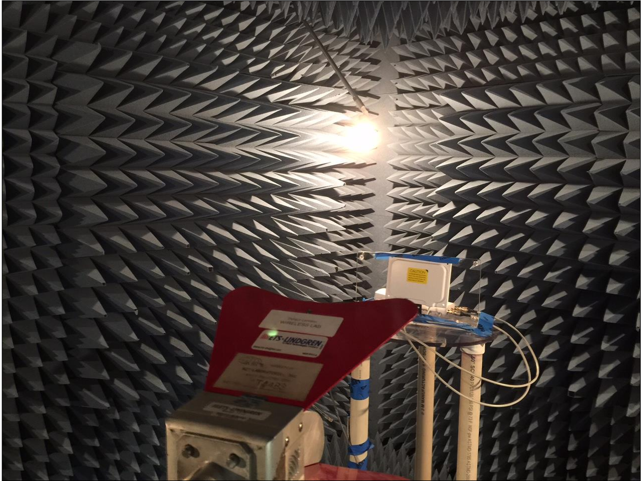
Photograph 2. Radiated Spurious Emissions, Test Setup
