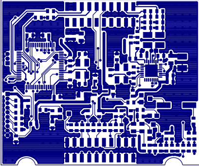
2009.01.23 TOP B'D NAME : DE-620
