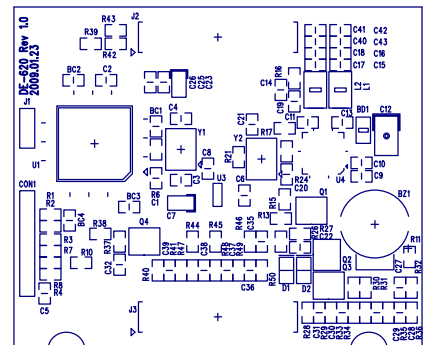
2009.01.23 SILK1 B'D NAME : DE-620
