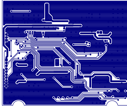
2009.01.23 BOTTOM B'D NAME : DE-620
