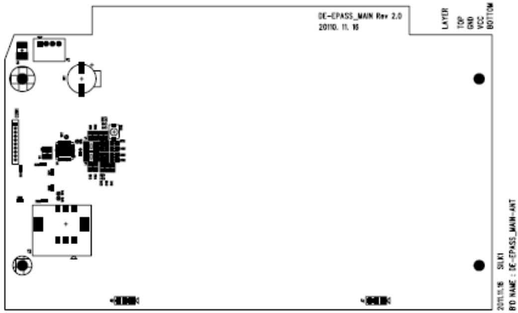
DE-EPASS_MAIN TOP side Part Location Diagram
