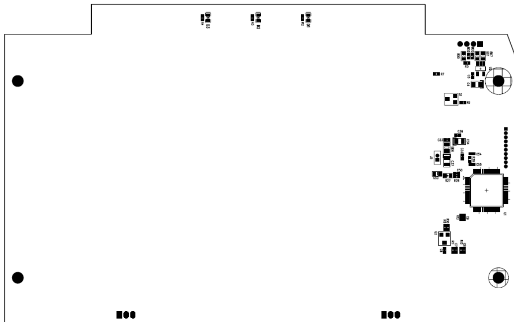
DE-EPASS_MAIN BOTTOM side Part Location Diagram
