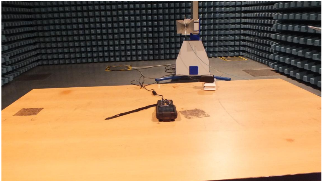
FCC Part 22H/24E Radiated Emission above 1GHz -Front
