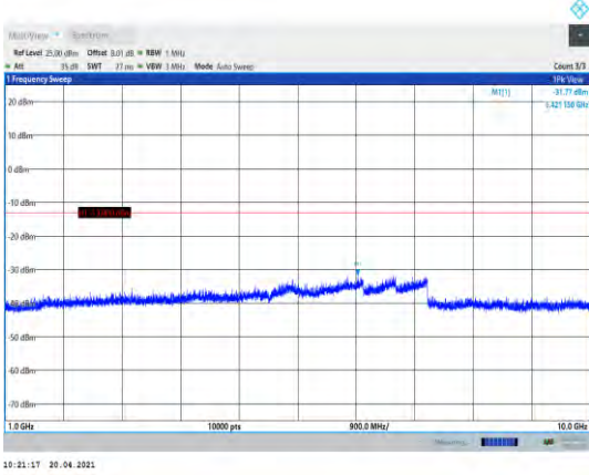
Band26-5MHz-16QAM-26715-1RB#0- Range2:1000~10000MHz
