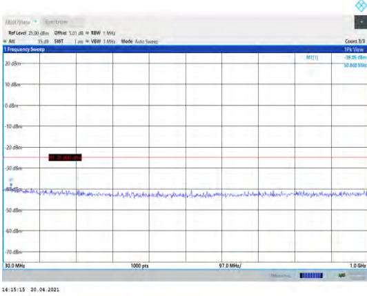
Band38-10MHz-16QAM-37800-1RB#0- Range1:30~1000MHz
