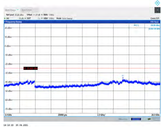
Band38-10MHz-QPSK-38000-1RB#0- Range3:3000~26000MHz
