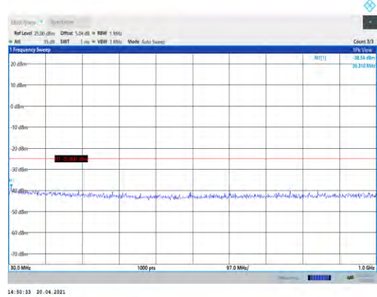
Band41-20MHz-QPSK-40340-1RB#0- Range1:30~1000MHz
