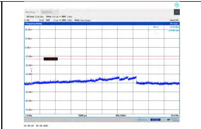
Band12-5MHz-16QAM-23095-1RB#0-Range2:1000~10000MHz
