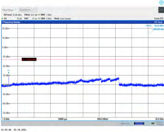
Band12-3MHz-16QAM-23025-1RB#0- Range2:1000~10000MHz
