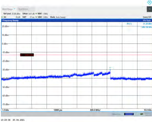
Band26-3MHz-QPSK-26705-1RB#0- Range2:1000~10000MHz
