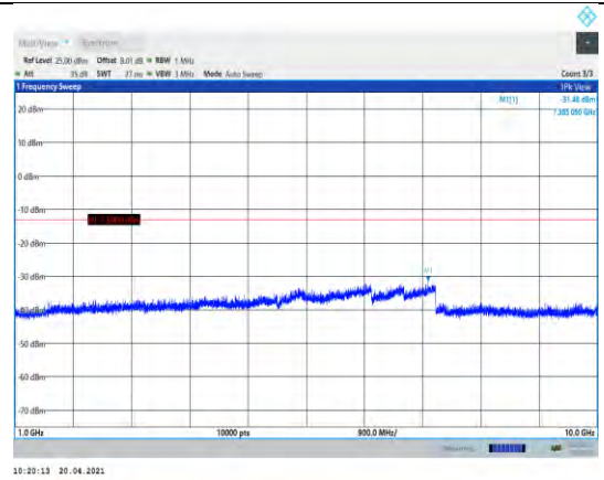
Band26-10MHz-16QAM-26740-1RB#0- Range2:1000~10000MHz
