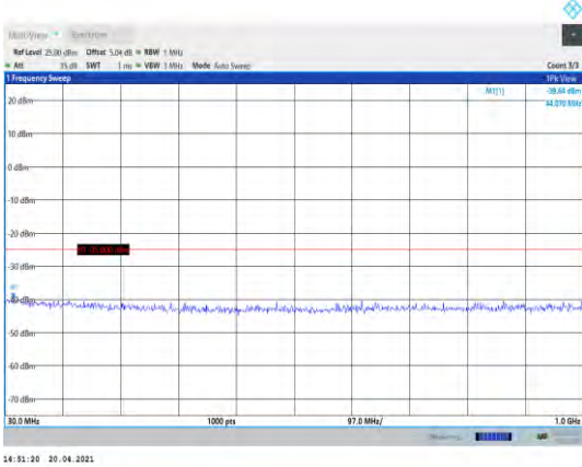
Band41-20MHz-16QAM-40340-1RB#0- Range1:30~1000MHz
