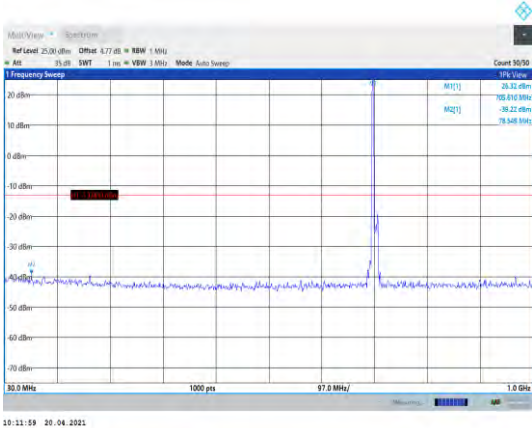
Band17-10MHz-16QAM-23790-1RB#0- Range1:30~1000MHz
