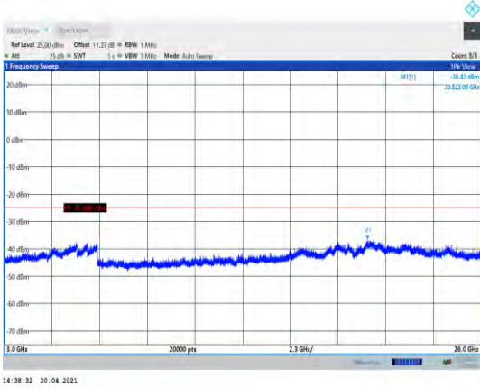
Band41-5MHz-16QAM-40740-1RB#0- Range3:3000~26000MHz
