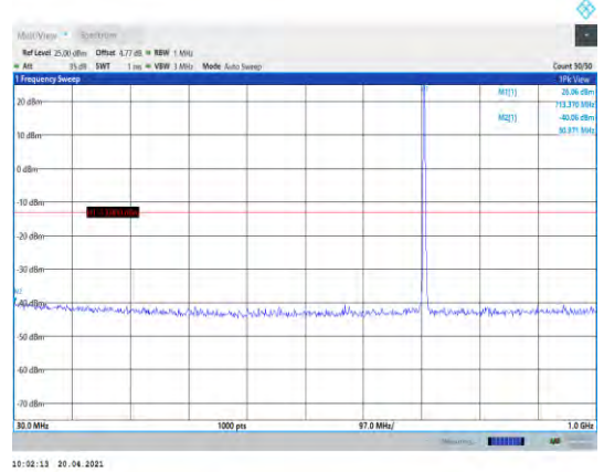
Band12-3MHz-16QAM-23165-1RB#0- Range1:30~1000MHz
