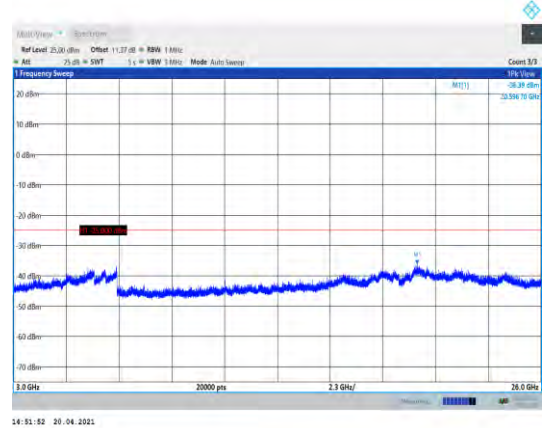
Band41-20MHz-16QAM-40340-1RB#0- Range3:3000~26000MHz
