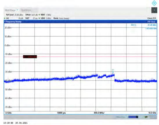
Band26-1.4MHz-QPSK-26783-1RB#0- Range2:1000~10000MHz
