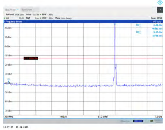
Band12-10MHz-16QAM-23130-1RB#0- Range1:30~1000MHz
