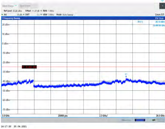
Band38-10MHz-16QAM-38000-1RB#0- Range3:3000~26000MHz
