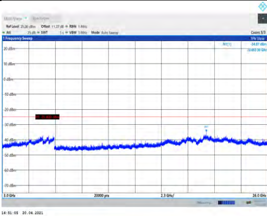
Band41-20MHz-QPSK-40340-1RB#0- Range3:3000~26000MHz
