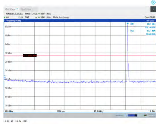
Band26-5MHz-16QAM-26765-1RB#0- Range1:30~1000MHz
