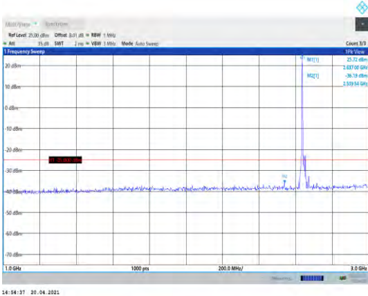
Band41-20MHz-16QAM-41140-1RB#0- Range2:1000~3000MHz
