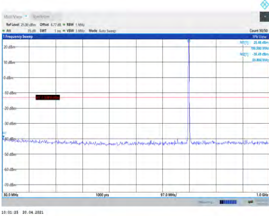
Band12-3MHz-16QAM-23095-1RB#0- Range1:30~1000MHz
