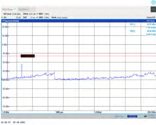
Band66-1.4MHz-QPSK-132322-1RB#0- Range2:1000~20000MHz
