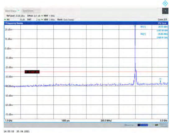
Band41-20MHz-16QAM-40740-1RB#0- Range2:1000~3000MHz
