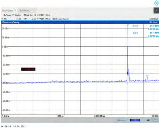
Band38-20MHz-16QAM-38150-1RB#0- Range2:1000~3000MHz
