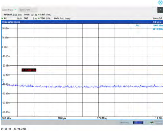
Band38-5MHz-QPSK-38000-1RB#0- Range1:30~1000MHz
