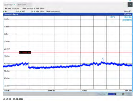
Band38-10MHz-16QAM-38200-1RB#0- Range3:3000~26000MHz
