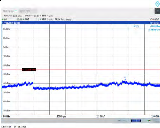
Band41-15MHz-16QAM-40740-1RB#0- Range3:3000~26000MHz
