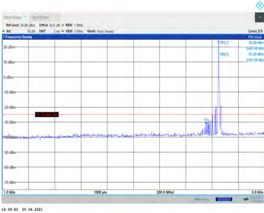
Band41-5MHz-16QAM-41215-1RB#0- Range2:1000~3000MHz
