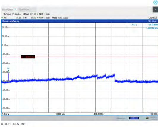
Band12-5MHz-QPSK-23035-1RB#0- Range2:1000~10000MHz
