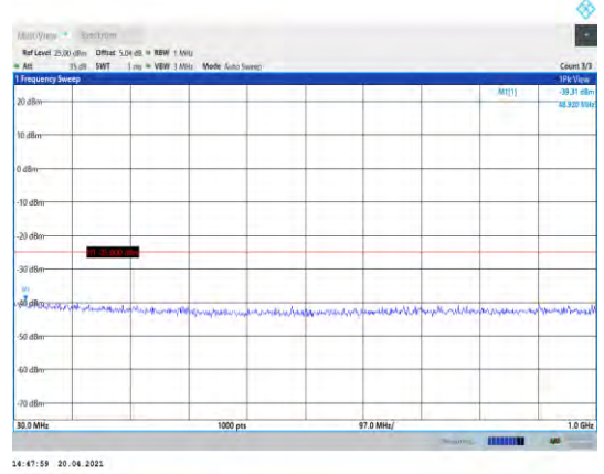
Band41-15MHz-16QAM-40740-1RB#0- Range1:30~1000MHz
