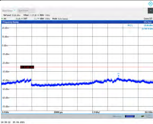
Band41-5MHz-QPSK-40265-1RB#0- Range3:3000~26000MHz
