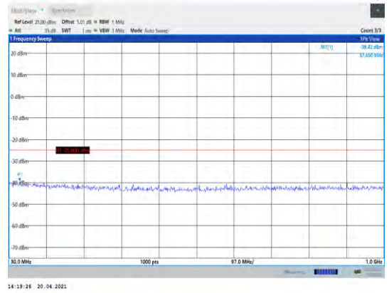
Band38-15MHz-QPSK-37825-1RB#0- Range1:30~1000MHz
