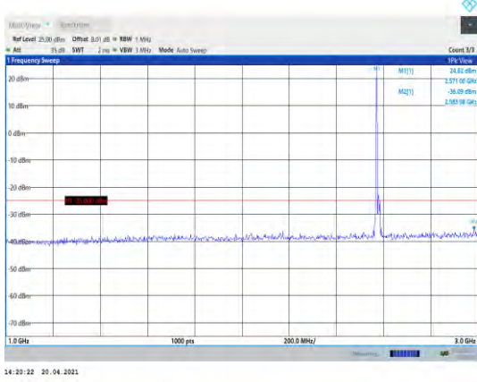
Band38-15MHz-16QAM-37825-1RB#0- Range2:1000~3000MHz
