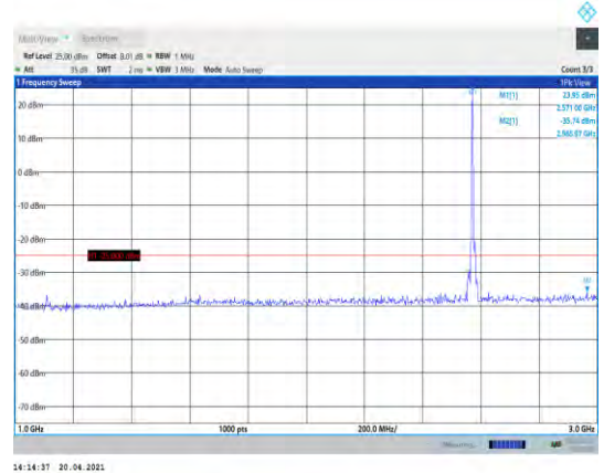
Band38-10MHz-QPSK-37800-1RB#0- Range2:1000~3000MHz
