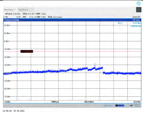
Band26-3MHz-QPSK-26740-1RB#0- Range2:1000~10000MHz
