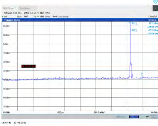
Band41-15MHz-16QAM-41165-1RB#0- Range2:1000~3000MHz
