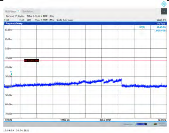
Band12-5MHz-QPSK-23095-1RB#0- Range2:1000~10000MHz
