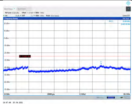
Band41-15MHz-QPSK-40740-1RB#0- Range3:3000~26000MHz
