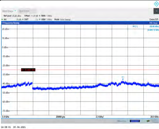
Band38-5MHz-QPSK-37775-1RB#0- Range3:3000~26000MHz
