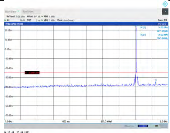
Band38-10MHz-QPSK-38200-1RB#0- Range2:1000~3000MHz
