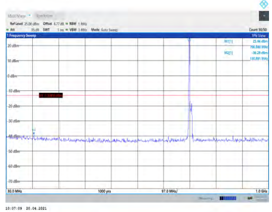
Band12-10MHz-QPSK-23130-1RB#0- Range1:30~1000MHz
