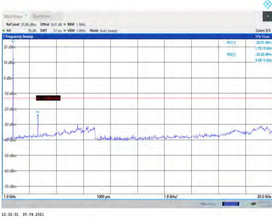
Band66-1.4MHz-16QAM-132322-1RB#0- Range2:1000~20000MHz
