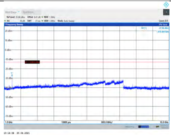
Band17-5MHz-QPSK-23790-1RB#0-Range2:1000~10000MHz
