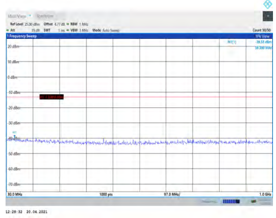
Band66-5MHz-QPSK-131997-1RB#0- Range1:30~1000MHz
