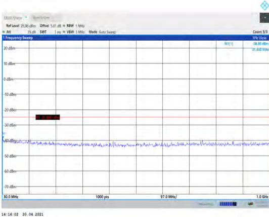
Band38-10MHz-QPSK-38000-1RB#0- Range1:30~1000MHz
