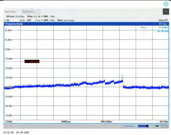
Band26-5MHz-QPSK-26740-1RB#0- Range2:1000~10000MHz
