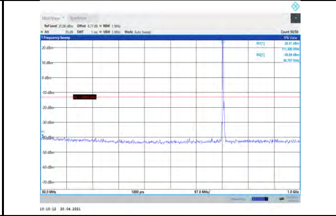
Band12-5MHz-16QAM-23155-1RB#0-Range1:30~1000MHz
