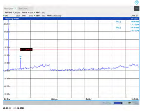
Band66-5MHz-16QAM-131997-1RB#0- Range2:1000~20000MHz
