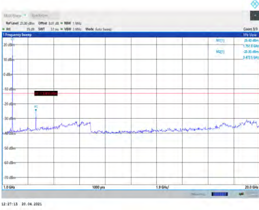
Band66-3MHz-16QAM-132322-1RB#0- Range2:1000~20000MHz
