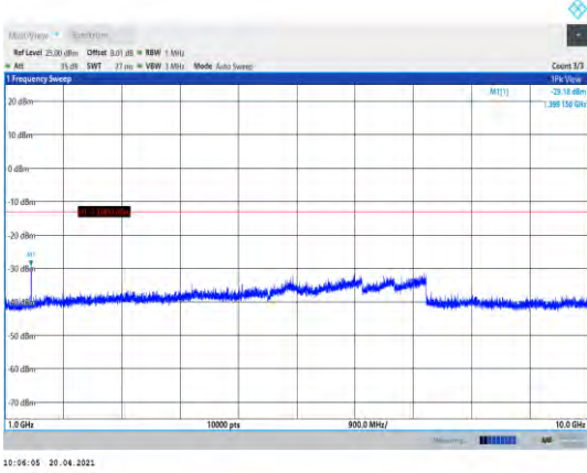
Band12-10MHz-16QAM-23060-1RB#0- Range2:1000~10000MHz
