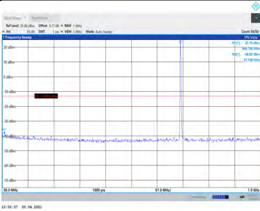
Band12-3MHz-16QAM-23025-1RB#0- Range1:30~1000MHz
