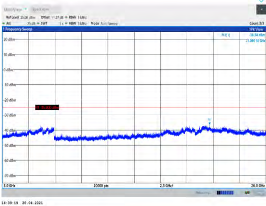
Band41-5MHz-QPSK-41215-1RB#0- Range3:3000~26000MHz
