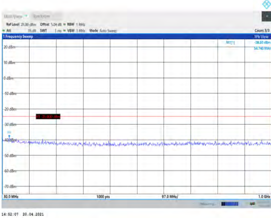
Band41-20MHz-QPSK-40740-1RB#0- Range1:30~1000MHz
