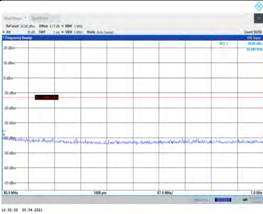
Band66-1.4MHz-16QAM-132322-1RB#0- Range1:30~1000MHz
