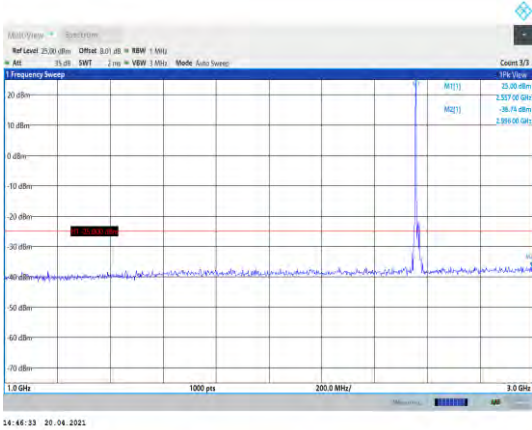
Band41-15MHz-16QAM-40315-1RB#0- Range2:1000~3000MHz
