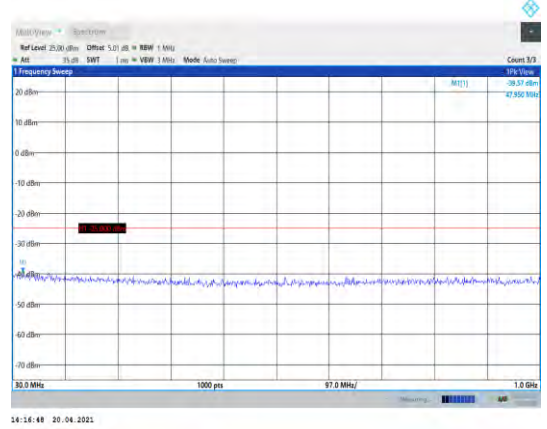
Band38-10MHz-16QAM-38000-1RB#0- Range1:30~1000MHz
