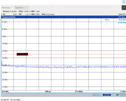
Band41-20MHz-16QAM-41140-1RB#0- Range1:30~1000MHz
