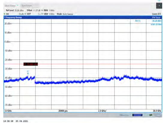
Band41-5MHz-16QAM-40265-1RB#0- Range3:3000~26000MHz
