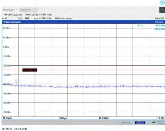
Band41-15MHz-16QAM-41165-1RB#0- Range1:30~1000MHz
