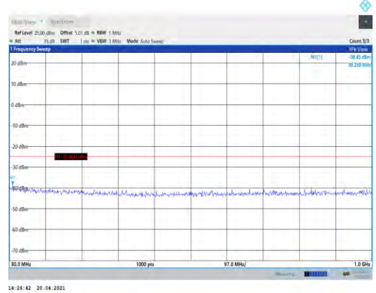
Band38-20MHz-16QAM-38000-1RB#0- Range1:30~1000MHz
