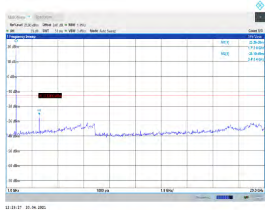
Band66-3MHz-16QAM-131987-1RB#0- Range2:1000~20000MHz
