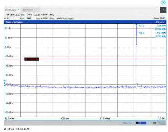
Band26-1.4MHz-16QAM-26783-1RB#0- Range1:30~1000MHz
