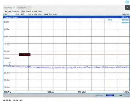
Band41-20MHz-QPSK-41140-1RB#0- Range1:30~1000MHz
