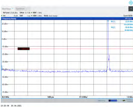
Band26-10MHz-16QAM-26740-1RB#0- Range1:30~1000MHz
