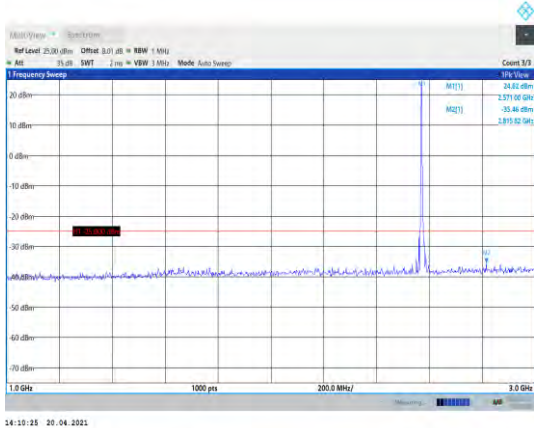
Band38-5MHz-16QAM-37775-1RB#0- Range2:1000~3000MHz
