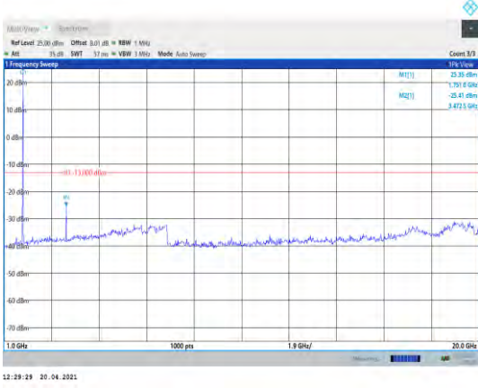
Band66-5MHz-QPSK-132322-1RB#0- Range2:1000~20000MHz
