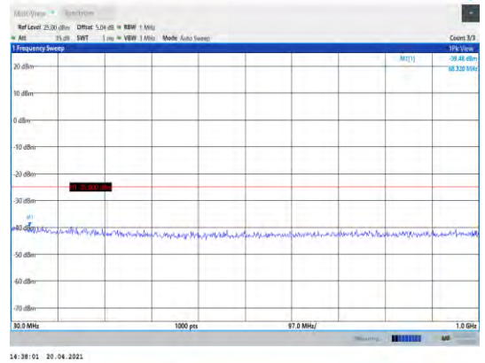
Band41-5MHz-16QAM-40740-1RB#0- Range1:30~1000MHz
