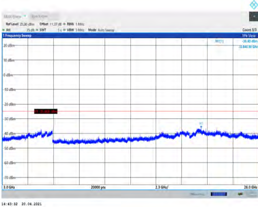
Band41-10MHz-16QAM-40740-1RB#0- Range3:3000~26000MHz
