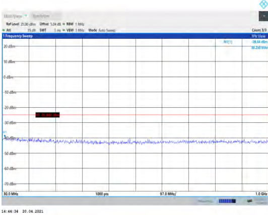
Band41-10MHz-16QAM-41190-1RB#0- Range1:30~1000MHz
