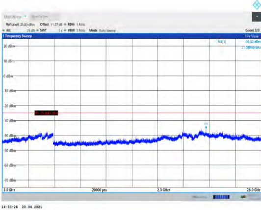
Band41-20MHz-16QAM-40740-1RB#0- Range3:3000~26000MHz
