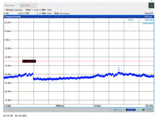
Band38-5MHz-16QAM-37775-1RB#0- Range3:3000~26000MHz
