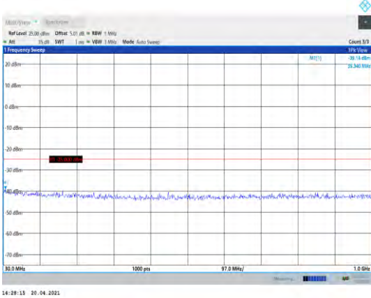
Band38-20MHz-16QAM-38150-1RB#0- Range1:30~1000MHz
