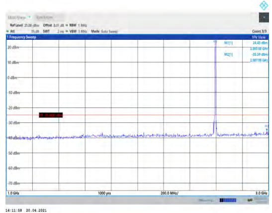
Band38-5MHz-16QAM-38000-1RB#0- Range2:1000~3000MHz
