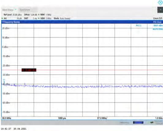
Band41-10MHz-16QAM-40290-1RB#0- Range1:30~1000MHz
