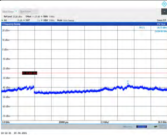
Band38-5MHz-16QAM-38000-1RB#0- Range3:3000~26000MHz
