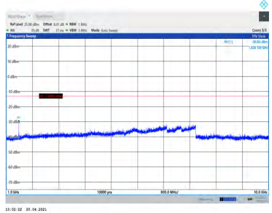
Band12-3MHz-16QAM-23165-1RB#0- Range2:1000~10000MHz
