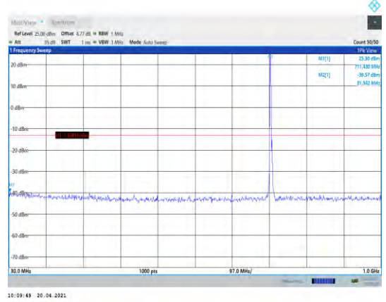
Band12-5MHz-QPSK-23155-1RB#0- Range1:30~1000MHz
