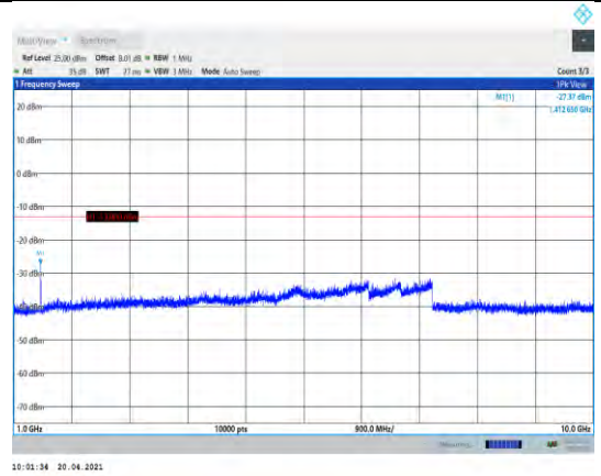
Band12-3MHz-16QAM-23095-1RB#0- Range2:1000~10000MHz
