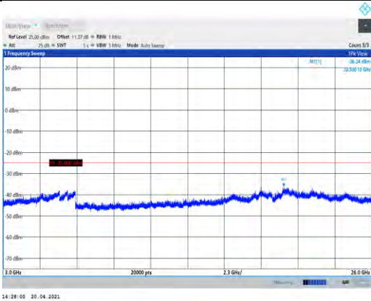
Band38-20MHz-QPSK-38150-1RB#0- Range3:3000~26000MHz
