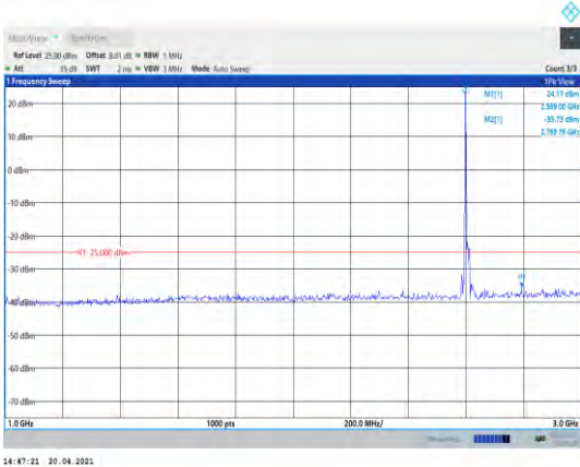
Band41-15MHz-QPSK-40740-1RB#0- Range2:1000~3000MHz
