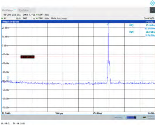
Band12-10MHz-QPSK-23095-1RB#0- Range1:30~1000MHz
