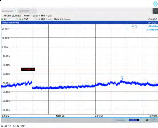
Band41-15MHz-QPSK-41165-1RB#0- Range3:3000~26000MHz
