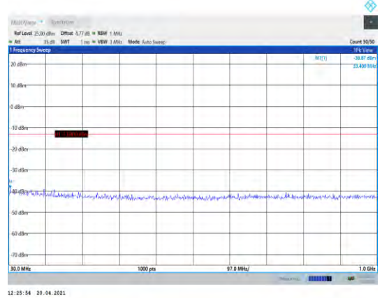
Band66-3MHz-QPSK-131987-1RB#0- Range1:30~1000MHz
