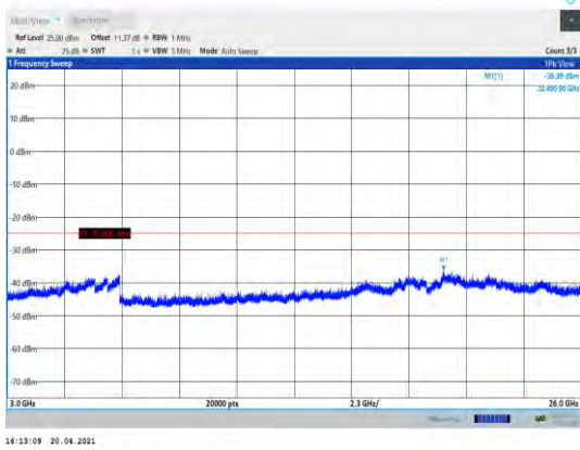
Band38-5MHz-QPSK-38225-1RB#0- Range3:3000~26000MHz
