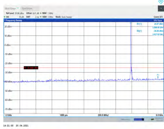
Band38-15MHz-16QAM-38000-1RB#0- Range2:1000~3000MHz
