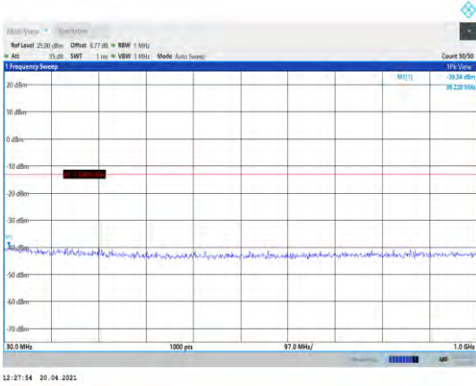
Band66-3MHz-16QAM-132657-1RB#0- Range1:30~1000MHz
