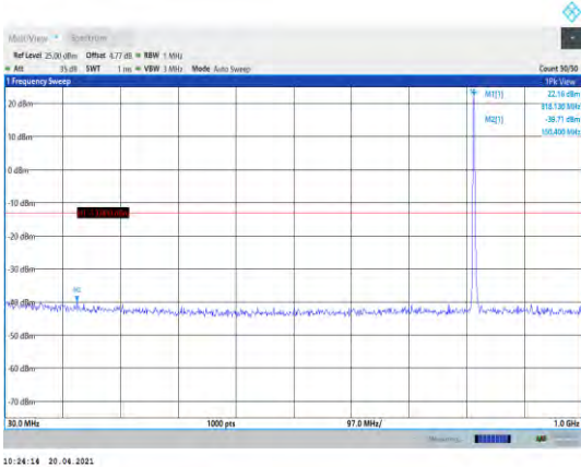
Band26-3MHz-QPSK-26740-1RB#0- Range1:30~1000MHz
