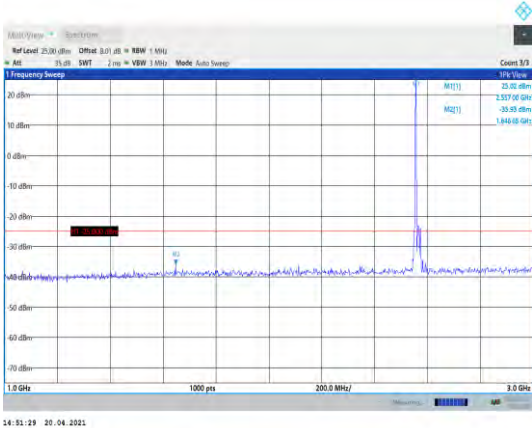
Band41-20MHz-16QAM-40340-1RB#0- Range2:1000~3000MHz
