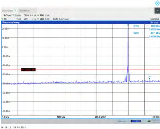
Band38-5MHz-QPSK-38000-1RB#0- Range2:1000~3000MHz
