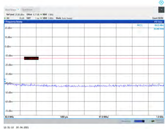
Band66-1.4MHz-QPSK-131979-1RB#0- Range1:30~1000MHz
