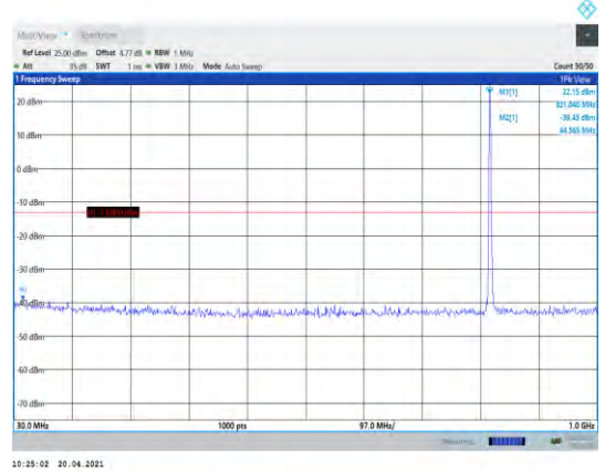
Band26-3MHz-QPSK-26775-1RB#0- Range1:30~1000MHz
