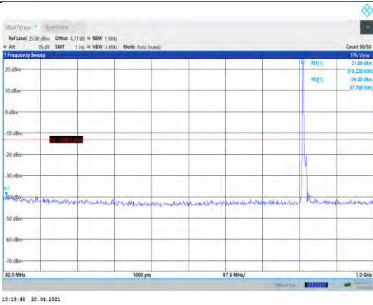
Band26-10MHz-QPSK-26740-1RB#0- Range1:30~1000MHz
