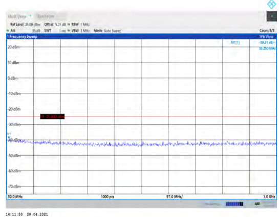
Band38-5MHz-16QAM-38000-1RB#0- Range1:30~1000MHz
