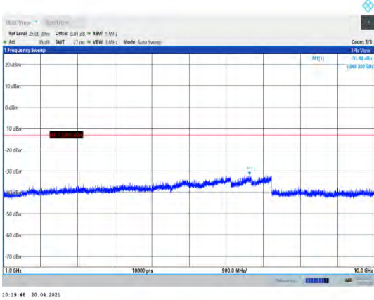
Band26-10MHz-QPSK-26740-1RB#0- Range2:1000~10000MHz
