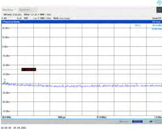
Band38-20MHz-QPSK-38000-1RB#0- Range1:30~1000MHz
