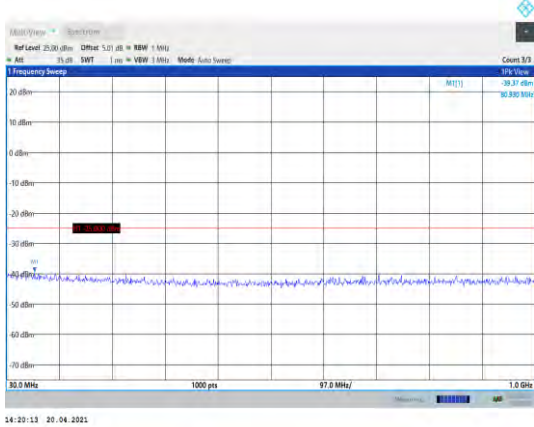
Band38-15MHz-16QAM-37825-1RB#0- Range1:30~1000MHz
