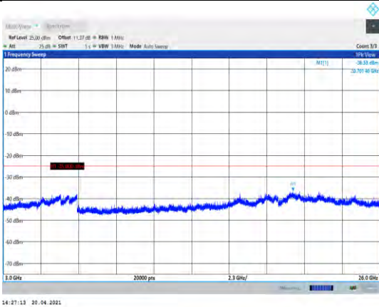
Band38-20MHz-16QAM-38000-1RB#0- Range3:3000~26000MHz
