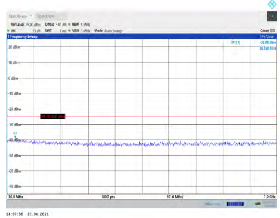
Band38-5MHz-QPSK-37775-1RB#0- Range1:30~1000MHz
