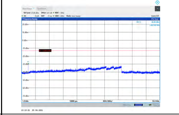
Band12-5MHz-16QAM-23155-1RB#0-Range2:1000~10000MHz
