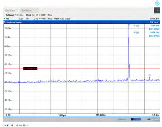
Band41-10MHz-16QAM-40740-1RB#0- Range2:1000~3000MHz
