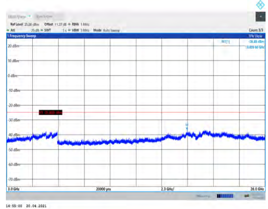
Band41-20MHz-16QAM-41140-1RB#0- Range3:3000~26000MHz
