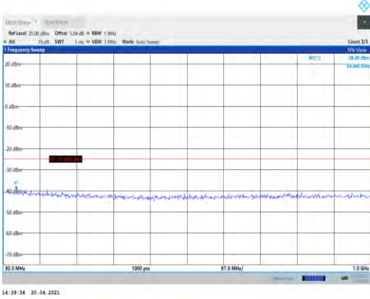
Band41-5MHz-16QAM-41215-1RB#0- Range1:30~1000MHz
