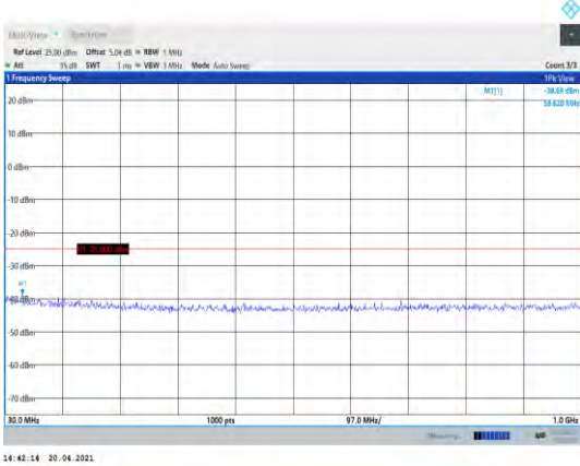
Band41-10MHz-QPSK-40740-1RB#0- Range1:30~1000MHz
