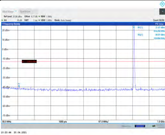
Band26-5MHz-QPSK-26715-1RB#0- Range1:30~1000MHz
