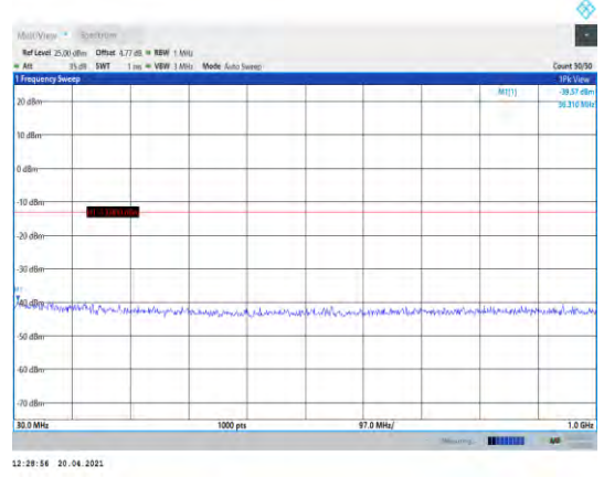
Band66-5MHz-16QAM-131997-1RB#0- Range1:30~1000MHz
