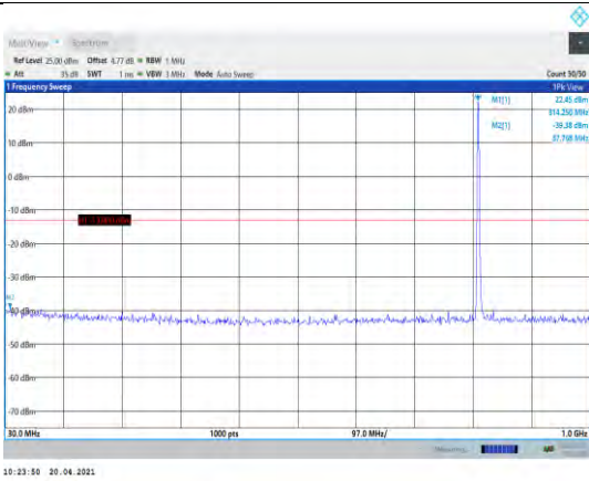
Band26-3MHz-16QAM-26705-1RB#0- Range1:30~1000MHz
