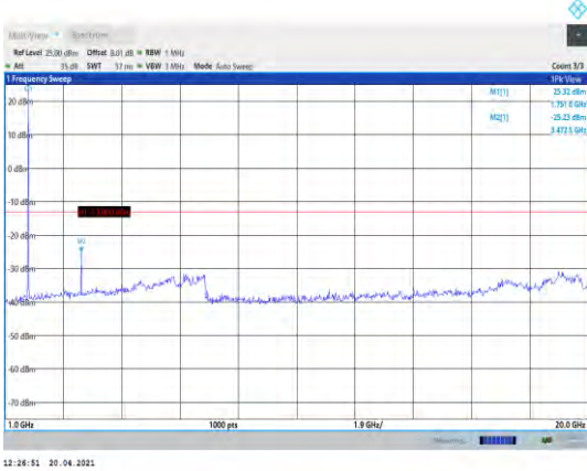
Band66-3MHz-QPSK-132322-1RB#0- Range2:1000~20000MHz
