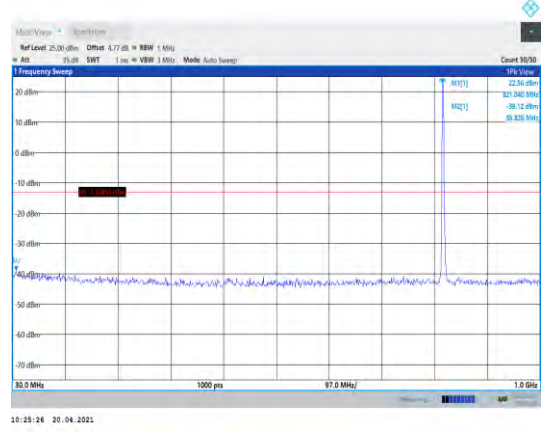
Band26-3MHz-16QAM-26775-1RB#0- Range1:30~1000MHz
