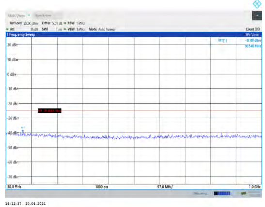
Band38-5MHz-QPSK-38225-1RB#0- Range1:30~1000MHz
