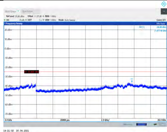
Band38-15MHz-QPSK-38000-1RB#0-Range3:3000~26000MHz
