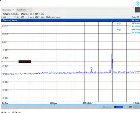
Band38-10MHz-QPSK-38000-1RB#0- Range2:1000~3000MHz
