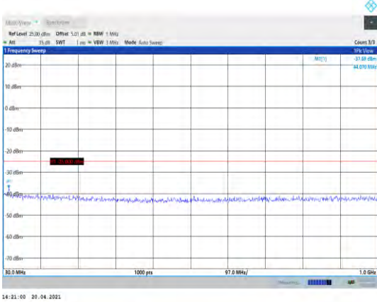
Band38-15MHz-QPSK-38000-1RB#0-Range1:30~1000MHz
