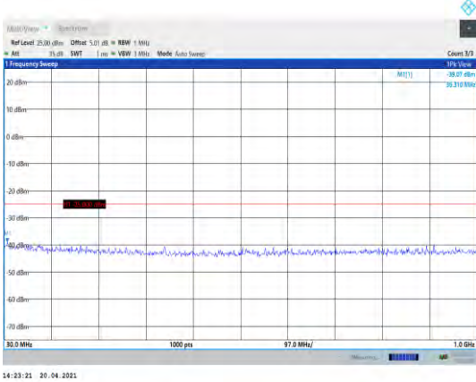
Band38-15MHz-16QAM-38175-1RB#0- Range1:30~1000MHz
