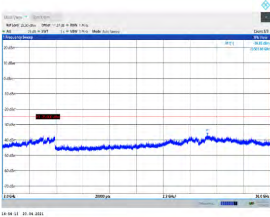
Band41-20MHz-QPSK-41140-1RB#0- Range3:3000~26000MHz
