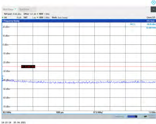
Band38-5MHz-16QAM-37775-1RB#0- Range1:30~1000MHz
