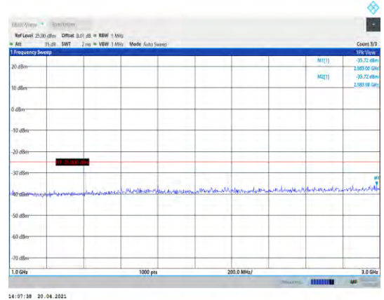
Band38-5MHz-QPSK-37775-1RB#0- Range2:1000~3000MHz
