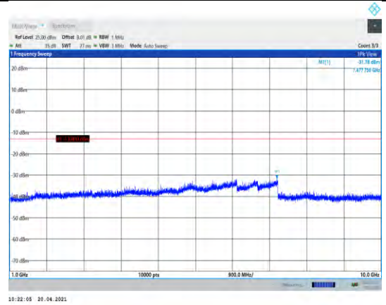
Band26-5MHz-16QAM-26740-1RB#0- Range2:1000~10000MHz
