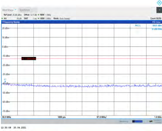
Band66-5MHz-QPSK-132647-1RB#0- Range1:30~1000MHz
