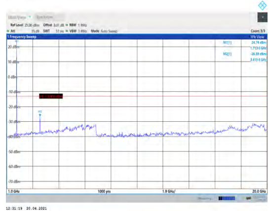
Band66-1.4MHz-QPSK-131979-1RB#0- Range2:1000~20000MHz
