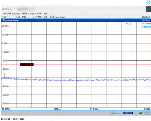
Band38-20MHz-16QAM-37850-1RB#0- Range1:30~1000MHz
