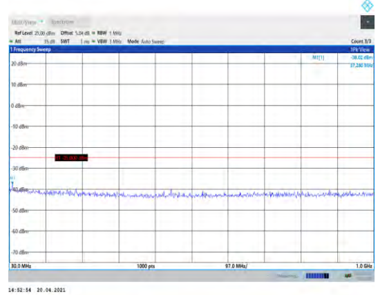
Band41-20MHz-16QAM-40740-1RB#0- Range1:30~1000MHz
