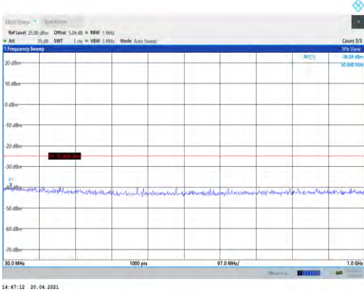
Band41-15MHz-QPSK-40740-1RB#0- Range1:30~1000MHz
