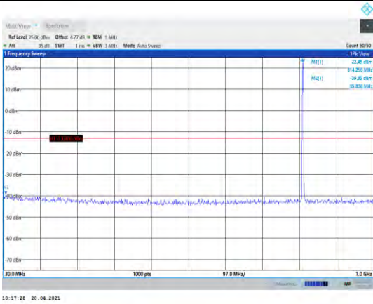
Band26-1.4MHz-16QAM-26697-1RB#0- Range1:30~1000MHz
