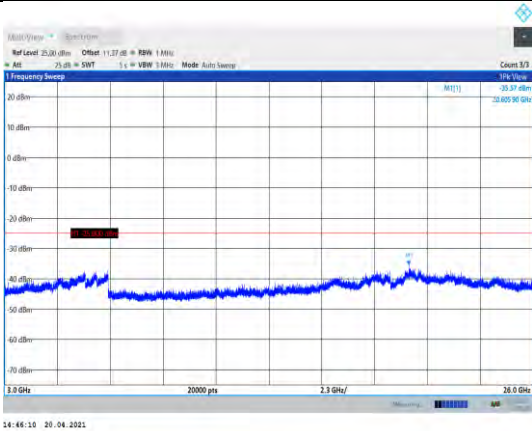
Band41-15MHz-QPSK-40315-1RB#0- Range3:3000~26000MHz
