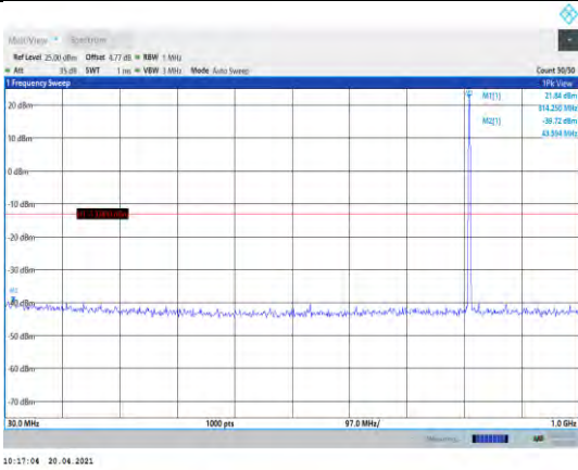
Band26-1.4MHz-QPSK-26697-1RB#0- Range1:30~1000MHz
