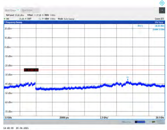
Band41-10MHz-16QAM-41190-1RB#0- Range3:3000~26000MHz
