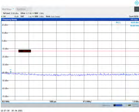
Band66-3MHz-QPSK-132657-1RB#0- Range1:30~1000MHz
