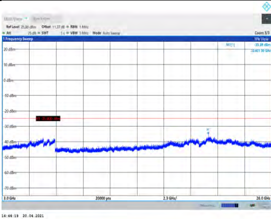
Band41-10MHz-QPSK-41190-1RB#0- Range3:3000~26000MHz
