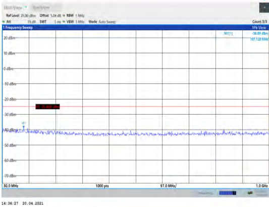
Band41-5MHz-16QAM-40265-1RB#0- Range1:30~1000MHz
