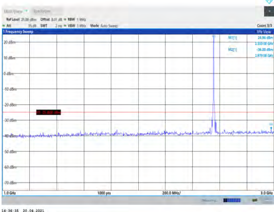
Band41-5MHz-16QAM-40265-1RB#0- Range2:1000~3000MHz
