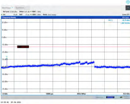
Band12-10MHz-QPSK-23060-1RB#0- Range2:1000~10000MHz
