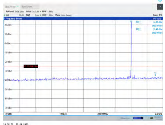
Band41-5MHz-16QAM-40740-1RB#0- Range2:1000~3000MHz
