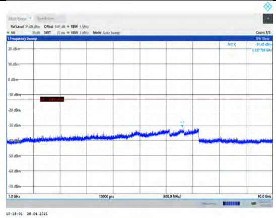
Band26-1.4MHz-QPSK-26740-1RB#0- Range2:1000~10000MHz
