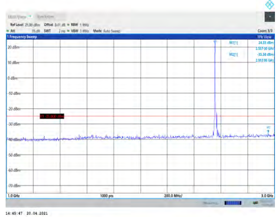
Band41-15MHz-QPSK-40315-1RB#0- Range2:1000~3000MHz
