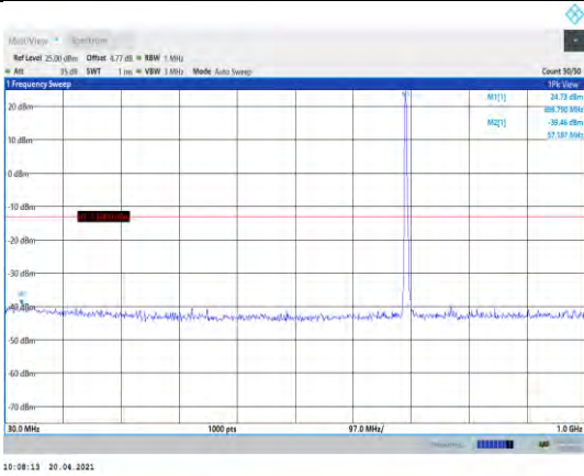
Band12-5MHz-QPSK-23035-1RB#0- Range1:30~1000MHz
