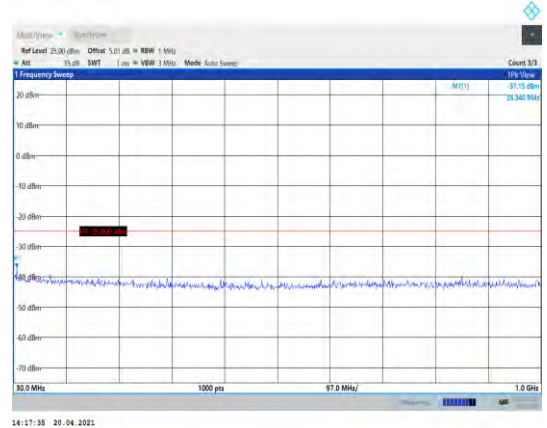
Band38-10MHz-QPSK-38200-1RB#0- Range1:30~1000MHz
