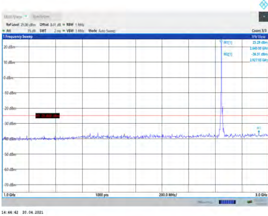
Band41-10MHz-16QAM-41190-1RB#0- Range2:1000~3000MHz
