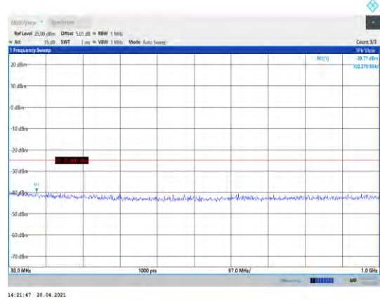
Band38-15MHz-16QAM-38000-1RB#0- Range1:30~1000MHz
