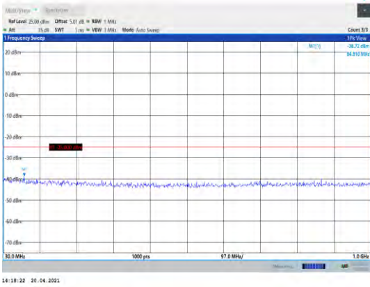
Band38-10MHz-16QAM-38200-1RB#0- Range1:30~1000MHz
