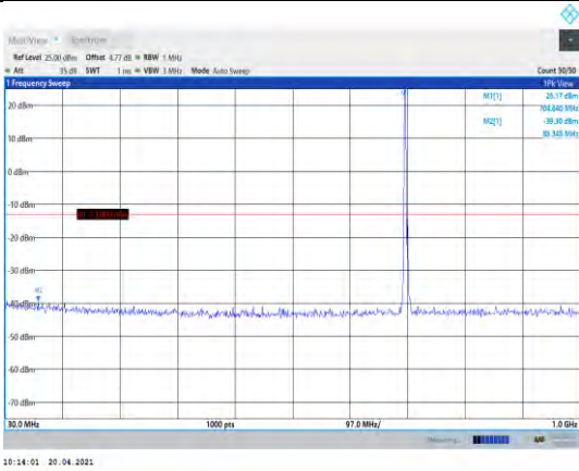
Band17-5MHz-16QAM-23755-1RB#0- Range1:30~1000MHz
