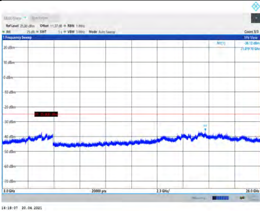
Band38-10MHz-QPSK-38200-1RB#0- Range3:3000~26000MHz
