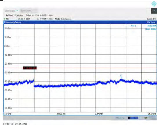
Band38-15MHz-16QAM-37825-1RB#0- Range3:3000~26000MHz
