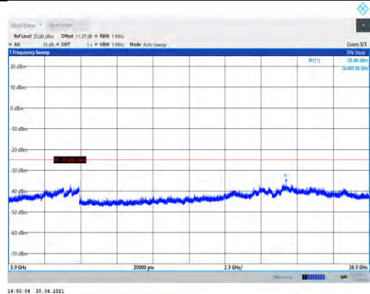
Band41-15MHz-16QAM-41165-1RB#0- Range3:3000~26000MHz
