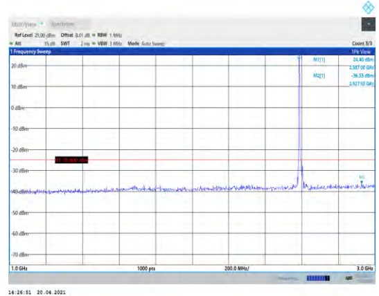
Band38-20MHz-16QAM-38000-1RB#0- Range2:1000~3000MHz
