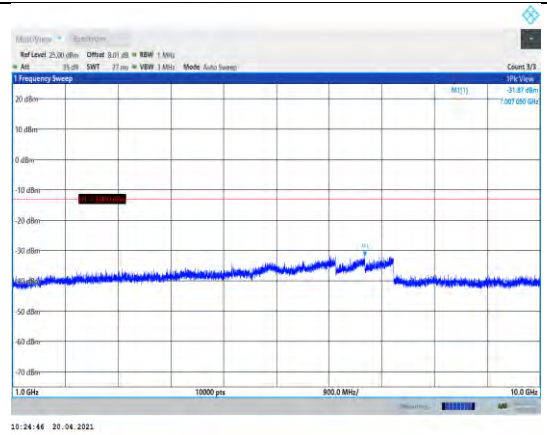
Band26-3MHz-16QAM-26740-1RB#0- Range2:1000~10000MHz
