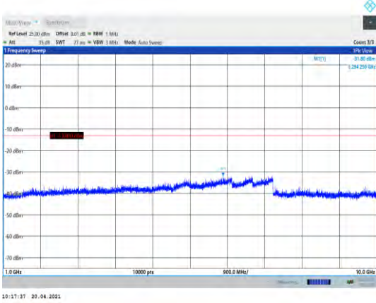
Band26-1.4MHz-16QAM-26697-1RB#0- Range2:1000~10000MHz
