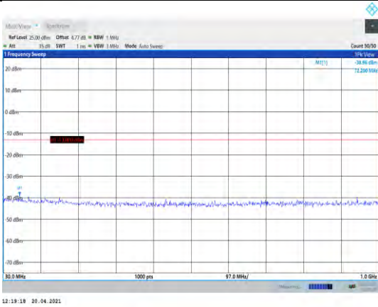
Band4-20MHz-QPSK-20050-1RB#0- Range1:30~1000MHz
