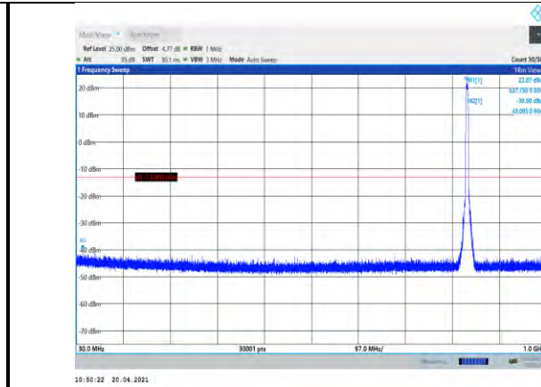
Band5-4182-30~1000MHz
