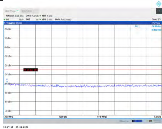
Band7-10MHz-QPSK-21100-1RB#0-Range1:30~1000MHz
