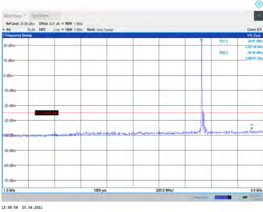
Band7-20MHz-16QAM-21100-1RB#0- Range2:1000~3000MHz
