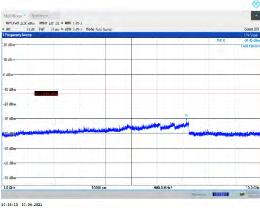
Band5-3MHz-16QAM-20415-1RB#0- Range2:1000~10000MHz
