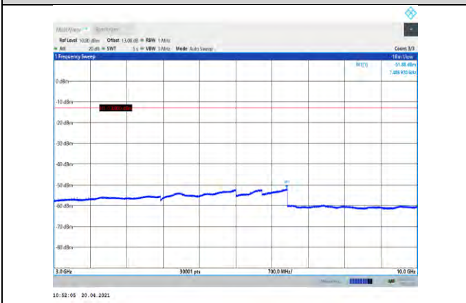
Band5-4233-3000~10000MHz
