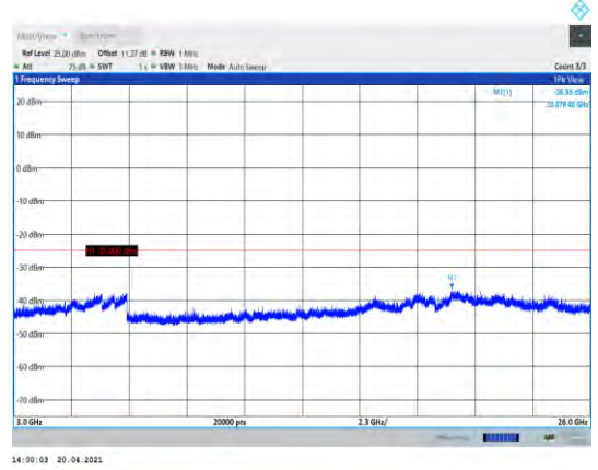
Band7-20MHz-16QAM-21350-1RB#0- Range3:3000~26000MHz
