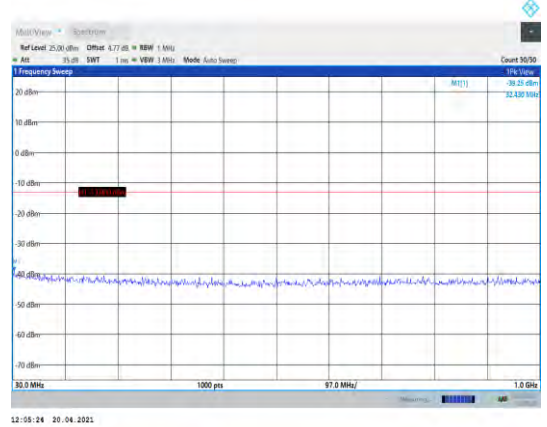
Band4-10MHz-QPSK-20350-1RB#0- Range1:30~1000MHz
