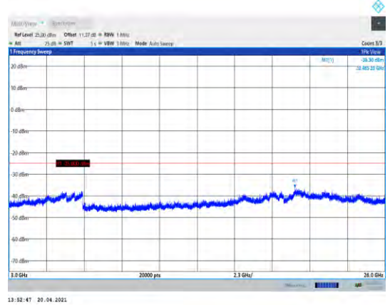
Band7-15MHz-QPSK-21100-1RB#0- Range3:3000~26000MHz
