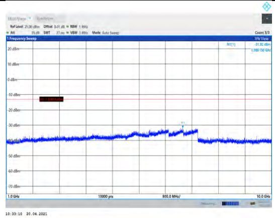
Band5-10MHz-16QAM-20525-1RB#0- Range2:1000~10000MHz
