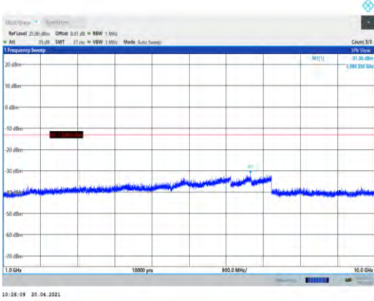
Band5-1.4MHz-QPSK-20407-1RB#0- Range2:1000~10000MHz
