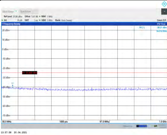
Band7-20MHz-16QAM-21100-1RB#0- Range1:30~1000MHz
