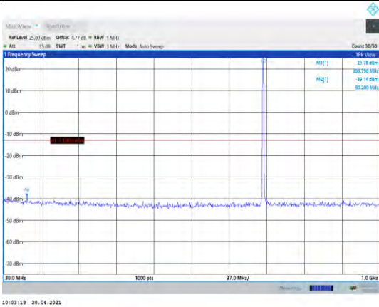
Band12-1.4MHz-16QAM-23017-1RB#0- Range1:30~1000MHz
