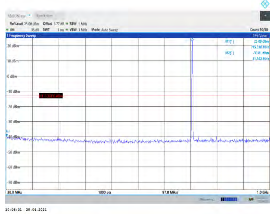
Band12-1.4MHz-QPSK-23173-1RB#0- Range1:30~1000MHz
