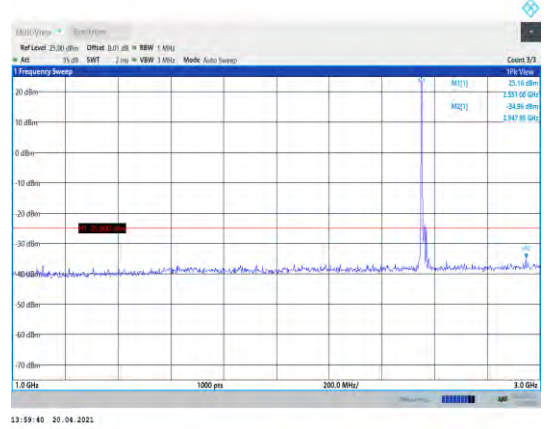
Band7-20MHz-16QAM-21350-1RB#0- Range2:1000~3000MHz
