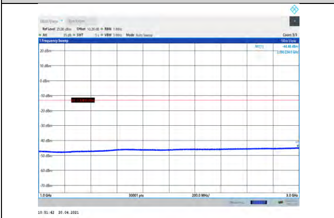
Band5-4233-1000~3000MHz
