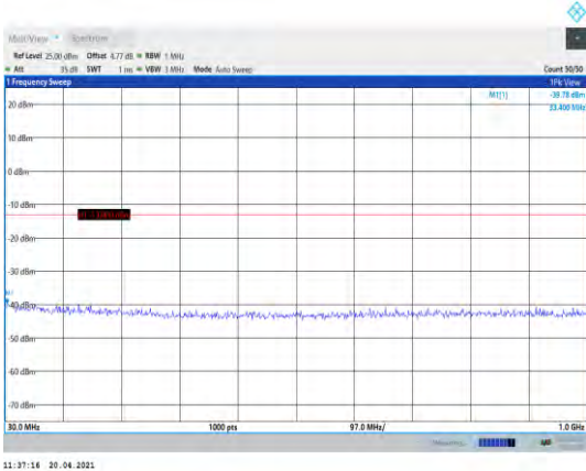
Band2-5MHz-16QAM-18900-1RB#0- Range1:30~1000MHz
