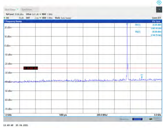
Band7-10MHz-16QAM-21400-1RB#0- Range2:1000~3000MHz
