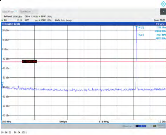
Band5-1.4MHz-QPSK-20407-1RB#0- Range1:30~1000MHz
