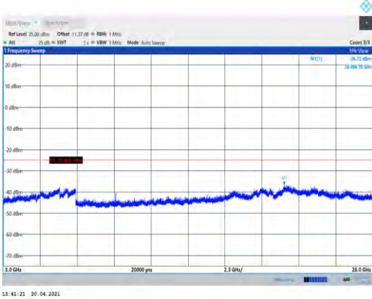
Band7-5MHz-QPSK-20775-1RB#0- Range3:3000~26000MHz
