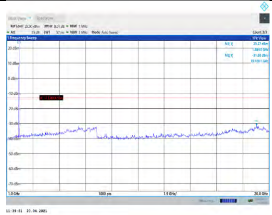
Band2-10MHz-QPSK-18900-1RB#0- Range2:1000~20000MHz
