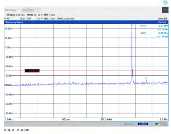
Band7-15MHz-16QAM-21375-1RB#0- Range2:1000~3000MHz
