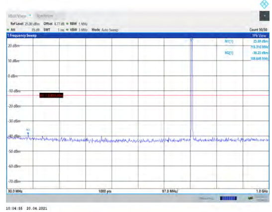
Band12-1.4MHz-16QAM-23173-1RB#0- Range1:30~1000MHz
