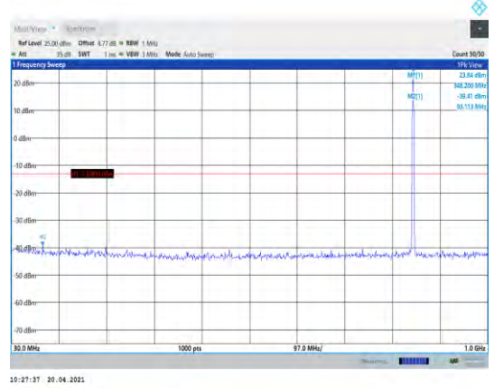
Band5-1.4MHz-QPSK-20643-1RB#0- Range1:30~1000MHz
