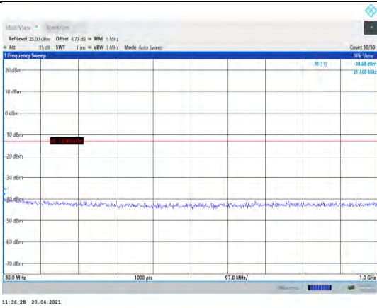
Band2-5MHz-16QAM-18625-1RB#0- Range1:30~1000MHz
