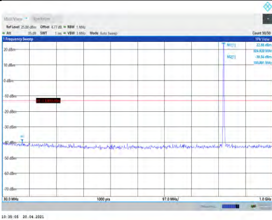
Band5-3MHz-16QAM-20415-1RB#0- Range1:30~1000MHz
