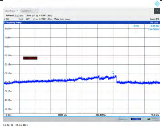
Band5-3MHz-16QAM-20525-1RB#0- Range2:1000~10000MHz
