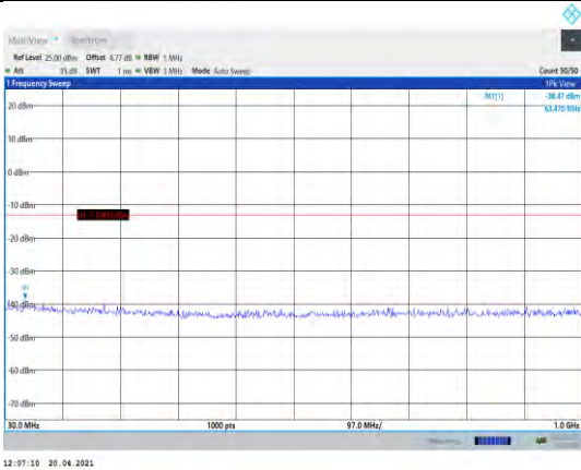
Band4-5MHz-16QAM-19975-1RB#0- Range1:30~1000MHz
