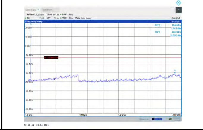
Band4-1.4MHz-16QAM-20393-1RB#0- Range2:1000~20000MHz
