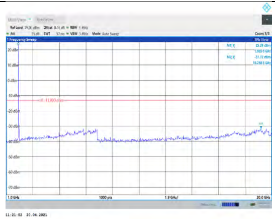
Band2-15MHz-16QAM-18900-1RB#0- Range2:1000~20000MHz
