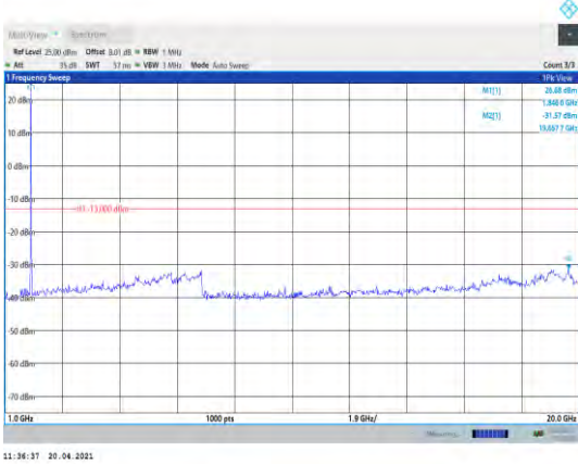
Band2-5MHz-16QAM-18625-1RB#0- Range2:1000~20000MHz
