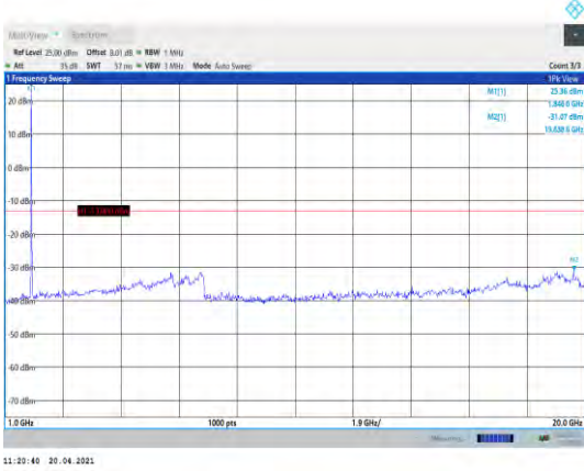
Band2-15MHz-QPSK-18675-1RB#0- Range2:1000~20000MHz
