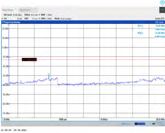
Band2-10MHz-QPSK-18650-1RB#0- Range2:1000~20000MHz
