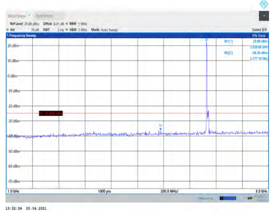
Band7-15MHz-QPSK-21100-1RB#0- Range2:1000~3000MHz
