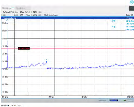
Band2-15MHz-16QAM-18675-1RB#0- Range2:1000~20000MHz
