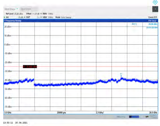
Band7-10MHz-16QAM-21400-1RB#0- Range3:3000~26000MHz
