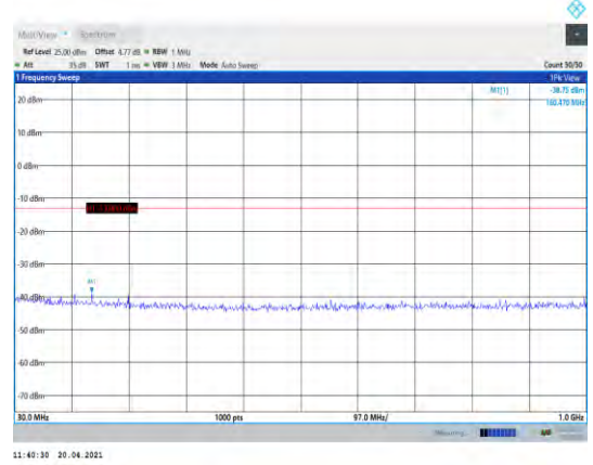
Band2-10MHz-QPSK-19150-1RB#0- Range1:30~1000MHz
