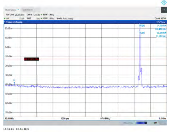
Band5-10MHz-QPSK-20600-1RB#0- Range1:30~1000MHz
