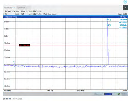
Band5-5MHz-QPSK-20625-1RB#0-Range1:30~1000MHz
