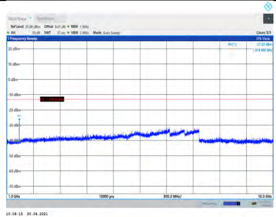
Band12-1.4MHz-16QAM-23095-1RB#0- Range2:1000~10000MHz
