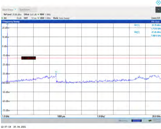
Band4-5MHz-16QAM-19975-1RB#0- Range2:1000~20000MHz
