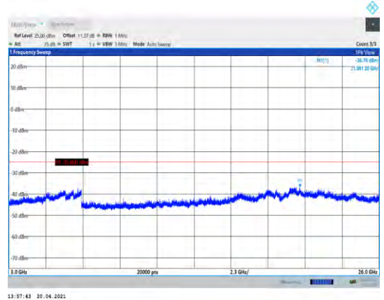
Band7-20MHz-QPSK-21100-1RB#0- Range3:3000~26000MHz
