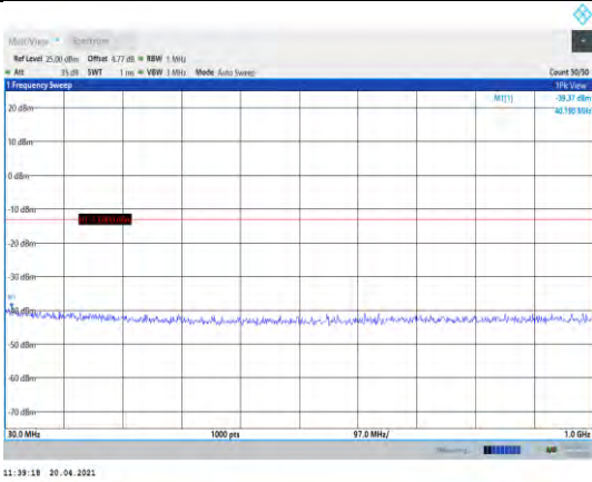
Band2-10MHz-16QAM-18650-1RB#0- Range1:30~1000MHz
