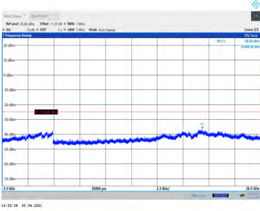
Band7-15MHz-16QAM-21100-1RB#0- Range3:3000~26000MHz
