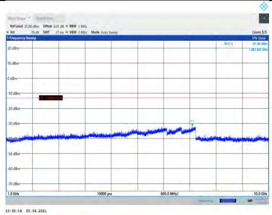
Band5-5MHz-16QAM-20525-1RB#0- Range2:1000~10000MHz
