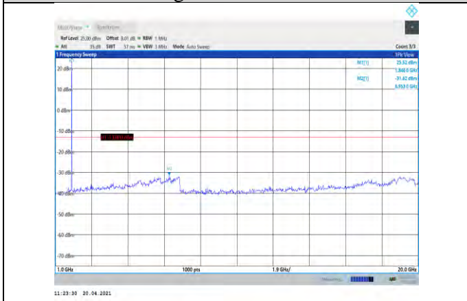
Band2-1.4MHz-QPSK-18607-1RB#0- Range2:1000~20000MHz
