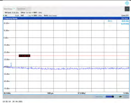
Band7-15MHz-QPSK-21100-1RB#0- Range1:30~1000MHz
