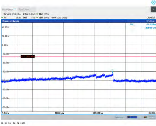
Band5-10MHz-QPSK-20450-1RB#0- Range2:1000~10000MHz
