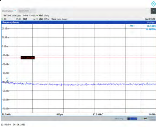
Band4-15MHz-QPSK-20025-1RB#0- Range1:30~1000MHz
