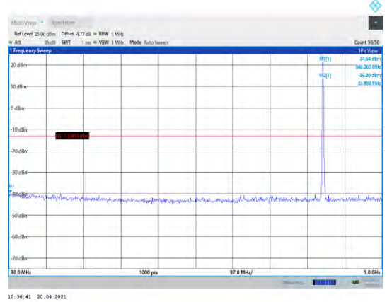
Band5-3MHz-16QAM-20635-1RB#0- Range1:30~1000MHz
