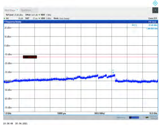
Band5-3MHz-16QAM-20635-1RB#0- Range2:1000~10000MHz
