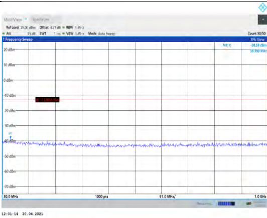
Band4-15MHz-16QAM-20025-1RB#0- Range1:30~1000MHz
