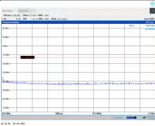
Band4-1.4MHz-QPSK-19957-1RB#0- Range1:30~1000MHz
