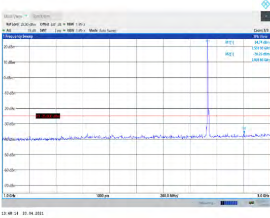
Band7-10MHz-16QAM-21100-1RB#0- Range2:1000~3000MHz
