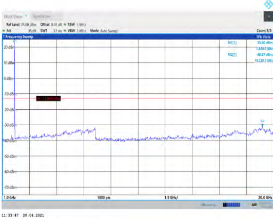
Band2-3MHz-16QAM-18615-1RB#0- Range2:1000~20000MHz
