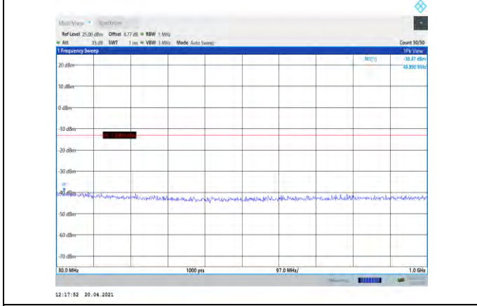
Band4-1.4MHz-16QAM-20175-1RB#0- Range1:30~1000MHz
