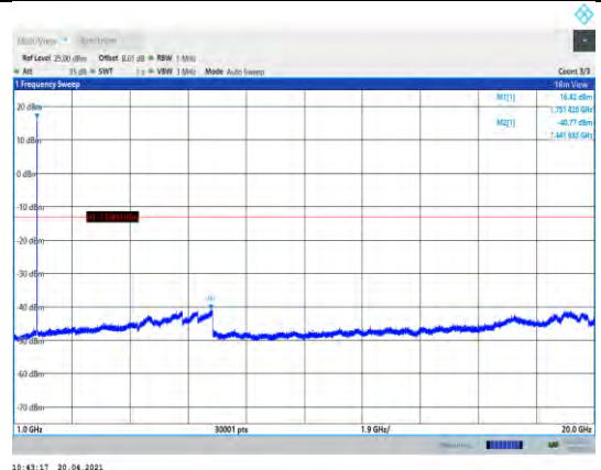
Band4-1513-1000~20000MHz
