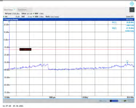
Band2-5MHz-16QAM-18900-1RB#0- Range2:1000~20000MHz
