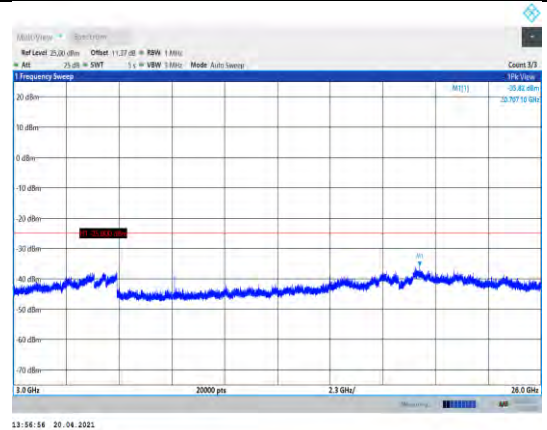
Band7-20MHz-16QAM-20850-1RB#0- Range3:3000~26000MHz
