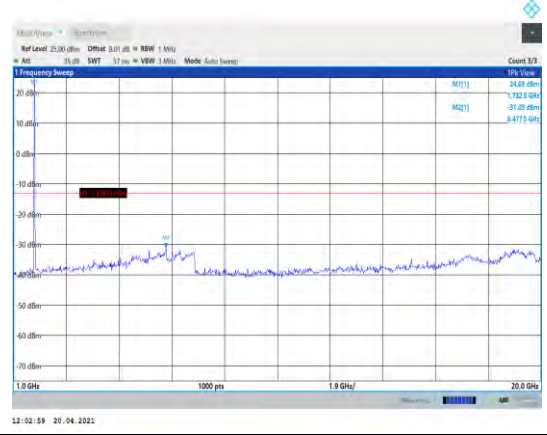
Band4-15MHz-16QAM-20325-1RB#0- Range2:1000~20000MHz
