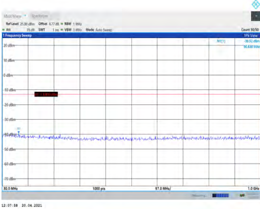
Band4-5MHz-16QAM-20175-1RB#0- Range1:30~1000MHz
