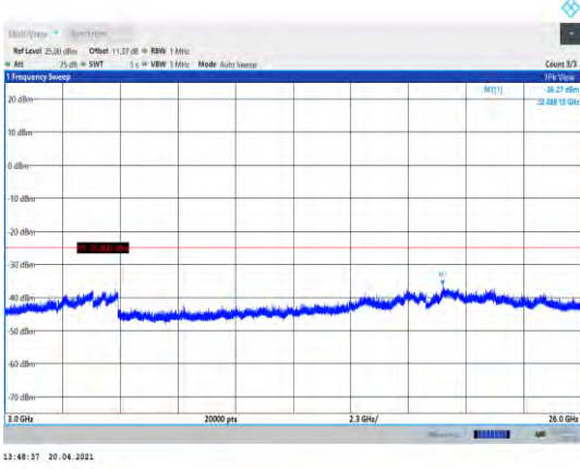
Band7-10MHz-16QAM-21100-1RB#0- Range3:3000~26000MHz
