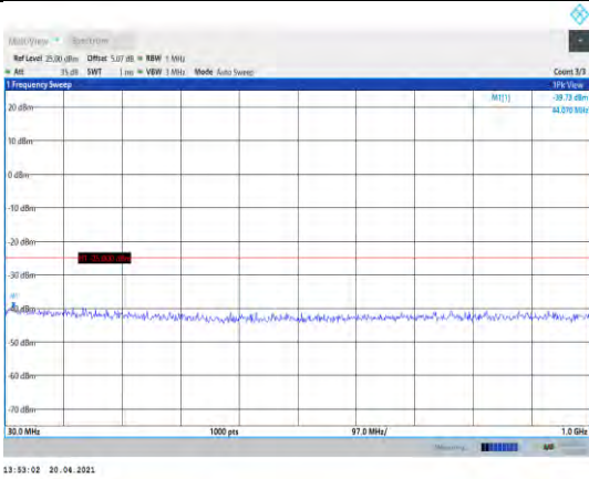
Band7-15MHz-16QAM-21100-1RB#0- Range1:30~1000MHz
