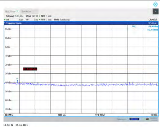
Band7-20MHz-16QAM-20850-1RB#0- Range1:30~1000MHz
