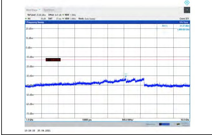
Band5-1.4MHz-16QAM-20407-1RB#0- Range2:1000~10000MHz
