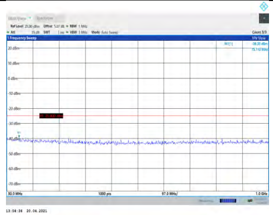
Band7-15MHz-16QAM-21375-1RB#0- Range1:30~1000MHz
