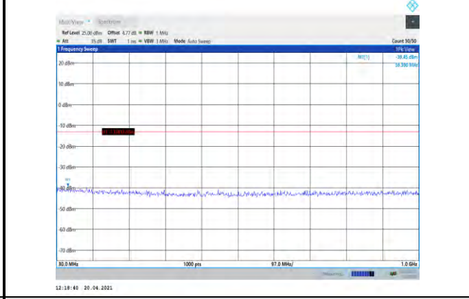
Band4-1.4MHz-16QAM-20393-1RB#0- Range1:30~1000MHz
