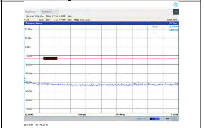
Band2-1.4MHz-QPSK-19193-1RB#0- Range1:30~1000MHz
