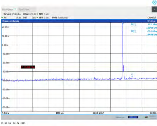
Band7-15MHz-QPSK-21375-1RB#0- Range2:1000~3000MHz
