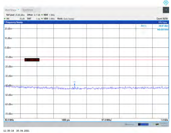
Band2-3MHz-16QAM-19185-1RB#0- Range1:30~1000MHz
