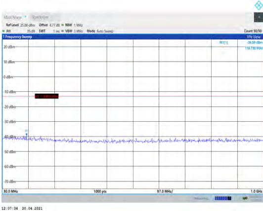
Band4-5MHz-QPSK-20175-1RB#0- Range1:30~1000MHz
