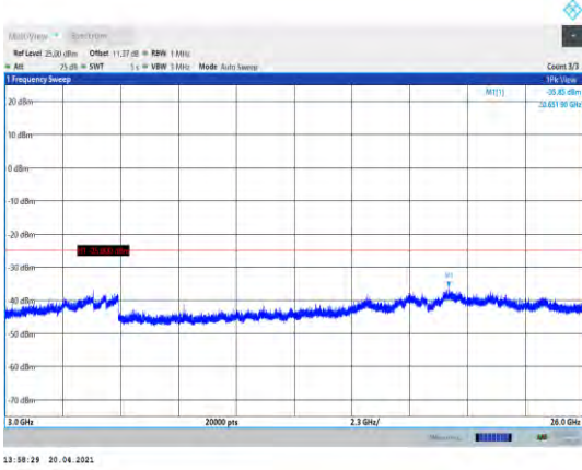
Band7-20MHz-16QAM-21100-1RB#0- Range3:3000~26000MHz
