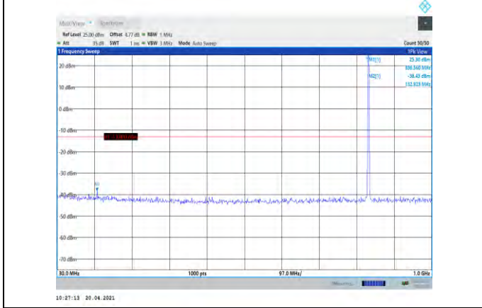
Band5-1.4MHz-16QAM-20525-1RB#0- Range1:30~1000MHz
