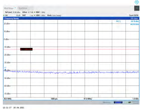
Band4-3MHz-QPSK-20385-1RB#0- Range1:30~1000MHz
