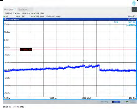
Band5-5MHz-QPSK-20525-1RB#0-Range2:1000~10000MHz
