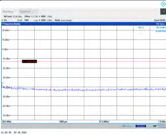
Band2-15MHz-QPSK-18675-1RB#0- Range1:30~1000MHz
