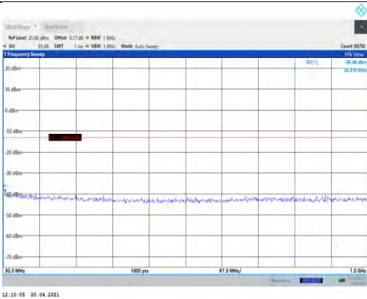
Band4-3MHz-16QAM-19965-1RB#0- Range1:30~1000MHz
