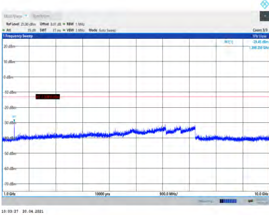
Band12-1.4MHz-16QAM-23017-1RB#0- Range2:1000~10000MHz
