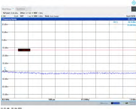
Band2-15MHz-16QAM-18900-1RB#0- Range1:30~1000MHz
