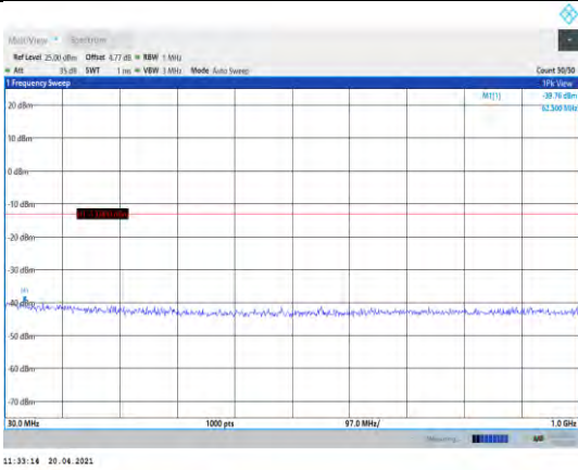
Band2-3MHz-QPSK-18615-1RB#0- Range1:30~1000MHz
