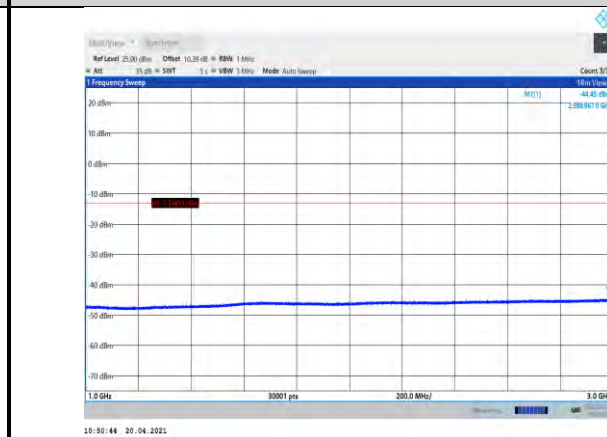
Band5-4182-1000~3000MHz
