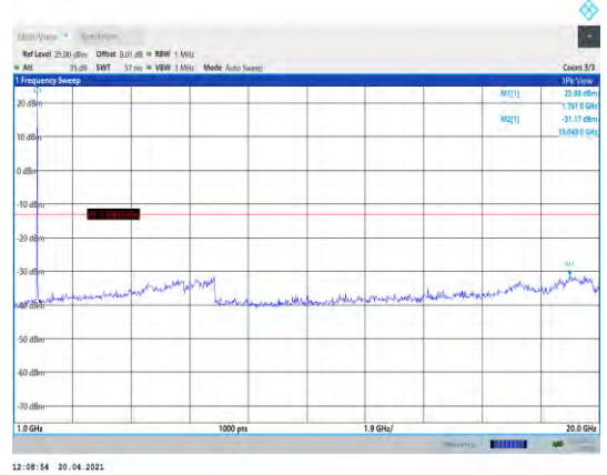
Band4-5MHz-16QAM-20375-1RB#0- Range2:1000~20000MHz
