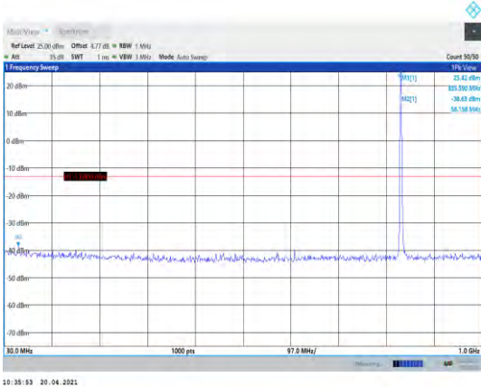
Band5-3MHz-16QAM-20525-1RB#0- Range1:30~1000MHz
