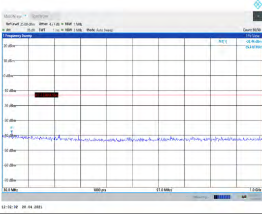
Band4-15MHz-16QAM-20175-1RB#0- Range1:30~1000MHz
