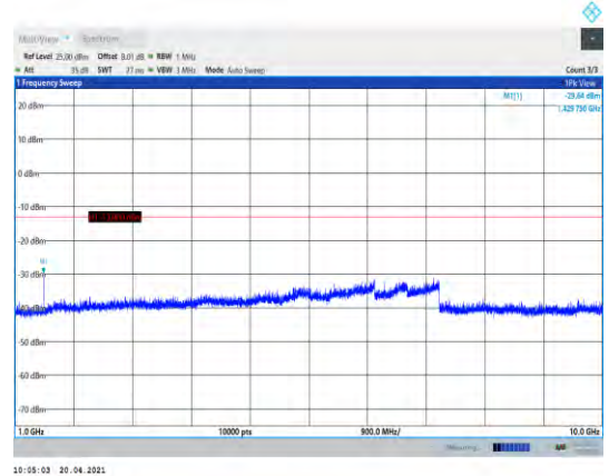
Band12-1.4MHz-16QAM-23173-1RB#0- Range2:1000~10000MHz
