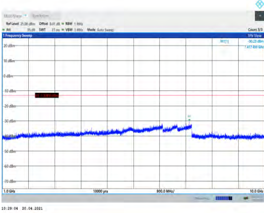
Band5-5MHz-QPSK-20425-1RB#0-Range2:1000~10000MHz
