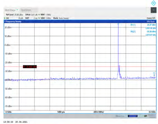
Band7-20MHz-16QAM-20850-1RB#0- Range2:1000~3000MHz
