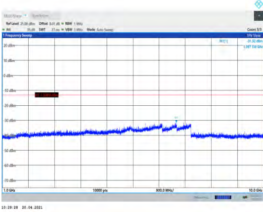
Band5-5MHz-16QAM-20425-1RB#0- Range2:1000~10000MHz
