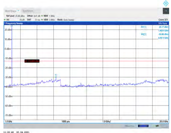
Band2-15MHz-16QAM-19125-1RB#0- Range2:1000~20000MHz
