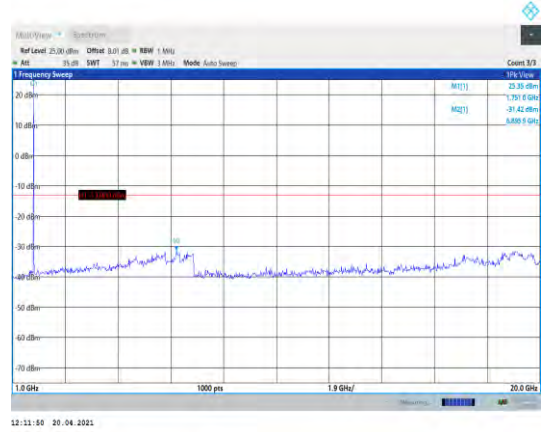
Band4-3MHz-16QAM-20385-1RB#0- Range2:1000~20000MHz
