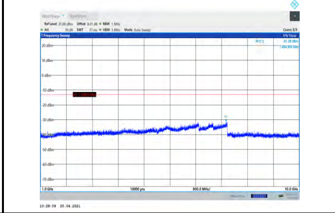
Band5-1.4MHz-16QAM-20643-1RB#0- Range2:1000~10000MHz
