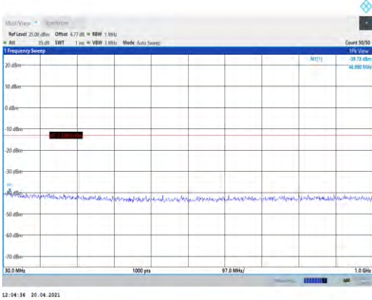
Band4-10MHz-QPSK-20175-1RB#0- Range1:30~1000MHz
