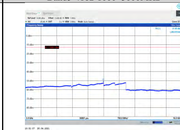
Band5-4182-3000~10000MHz
