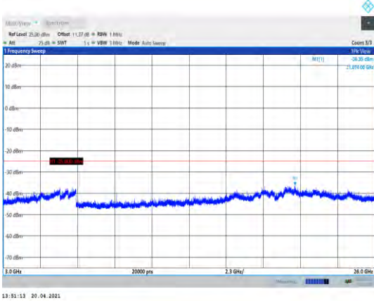
Band7-15MHz-QPSK-20825-1RB#0- Range3:3000~26000MHz
