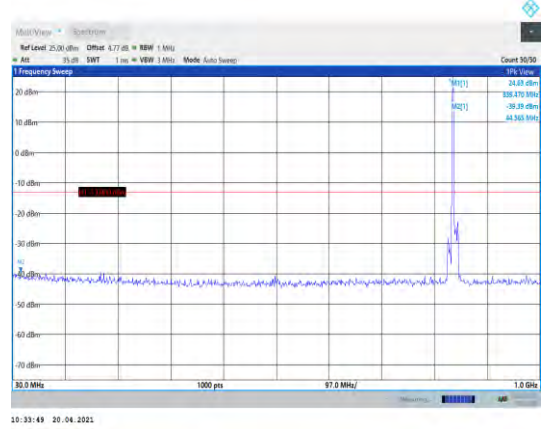
Band5-10MHz-16QAM-20600-1RB#0- Range1:30~1000MHz
