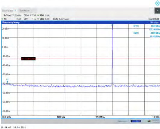
Band12-1.4MHz-16QAM-23095-1RB#0- Range1:30~1000MHz
