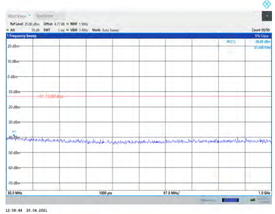
Band4-5MHz-16QAM-20375-1RB#0- Range1:30~1000MHz
