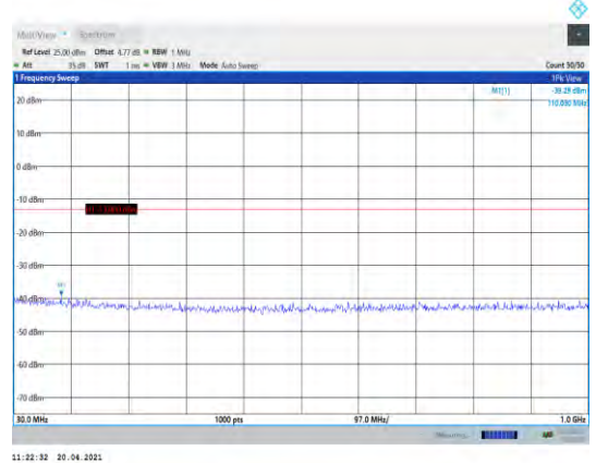
Band2-15MHz-16QAM-19125-1RB#0- Range1:30~1000MHz
