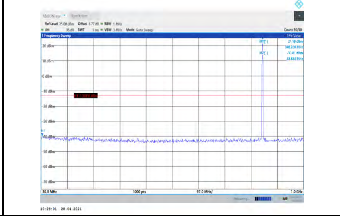
Band5-1.4MHz-16QAM-20643-1RB#0- Range1:30~1000MHz
