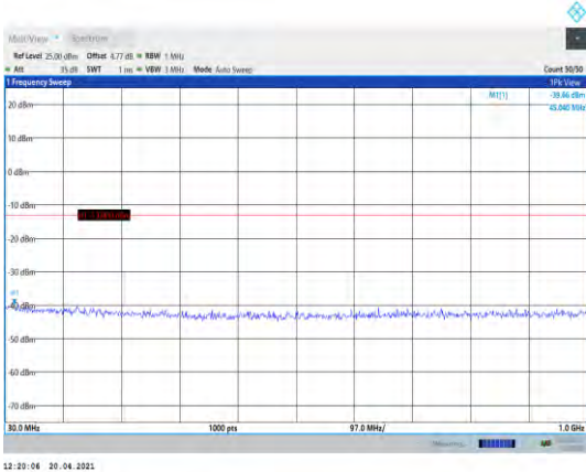
Band4-20MHz-QPSK-20175-1RB#0- Range1:30~1000MHz
