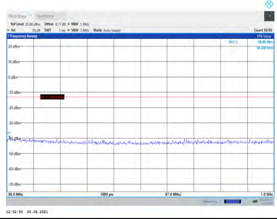
Band4-15MHz-16QAM-20325-1RB#0- Range1:30~1000MHz
