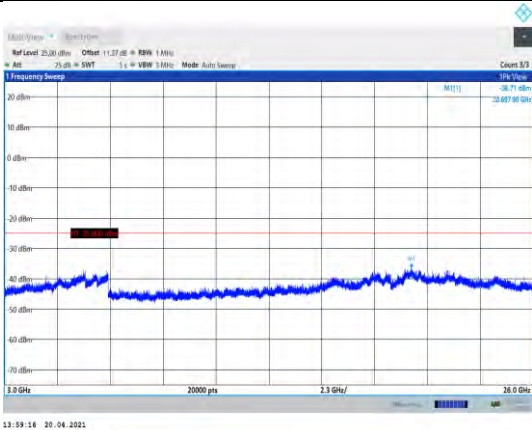
Band7-20MHz-QPSK-21350-1RB#0- Range3:3000~26000MHz
