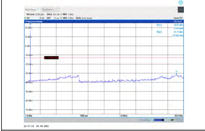
Band4-1.4MHz-16QAM-19957-1RB#0- Range2:1000~20000MHz
