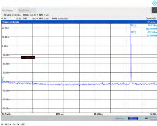
Band5-3MHz-QPSK-20525-1RB#0- Range1:30~1000MHz
