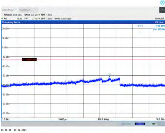
Band5-10MHz-16QAM-20450-1RB#0- Range2:1000~10000MHz
