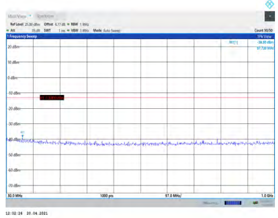
Band4-15MHz-QPSK-20325-1RB#0- Range1:30~1000MHz
