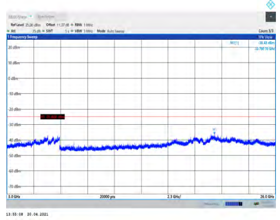
Band7-15MHz-16QAM-21375-1RB#0- Range3:3000~26000MHz
