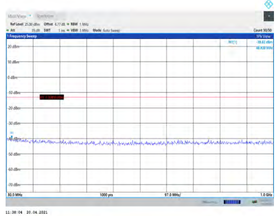
Band2-5MHz-16QAM-19175-1RB#0- Range1:30~1000MHz
