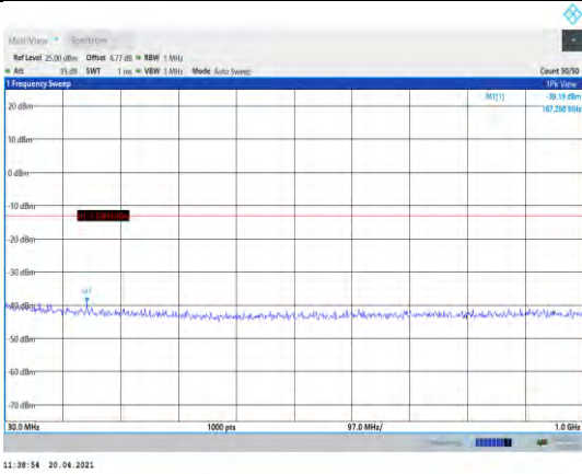
Band2-10MHz-QPSK-18650-1RB#0- Range1:30~1000MHz
