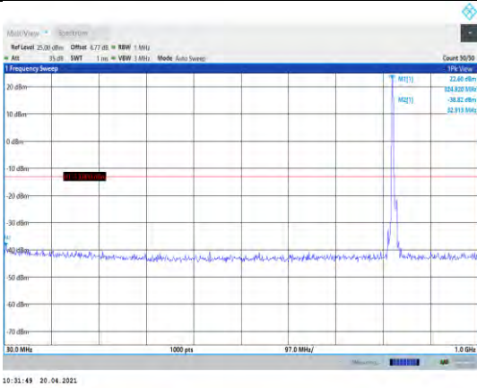
Band5-10MHz-QPSK-20450-1RB#0- Range1:30~1000MHz
