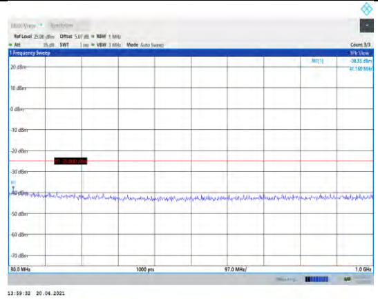
Band7-20MHz-16QAM-21350-1RB#0- Range1:30~1000MHz
