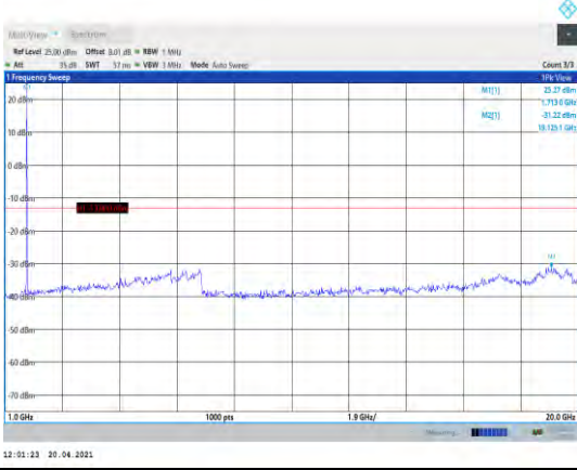
Band4-15MHz-16QAM-20025-1RB#0- Range2:1000~20000MHz
