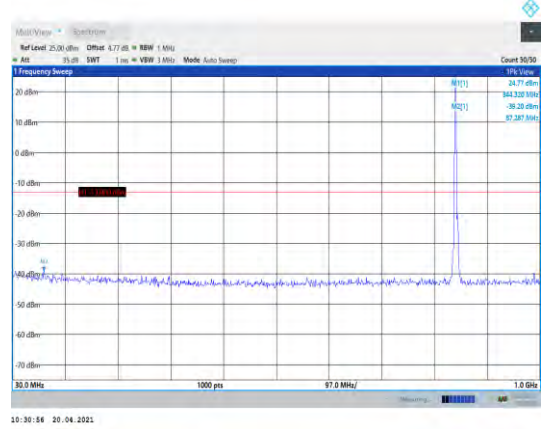
Band5-5MHz-16QAM-20625-1RB#0- Range1:30~1000MHz
