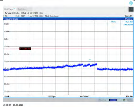
Band5-1.4MHz-QPSK-20525-1RB#0- Range2:1000~10000MHz
