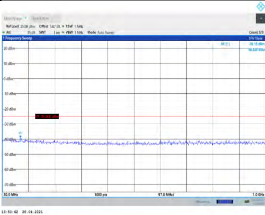
Band7-15MHz-QPSK-20825-1RB#0- Range1:30~1000MHz
