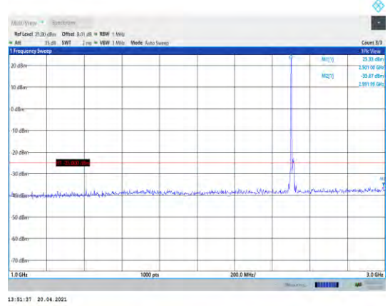
Band7-15MHz-16QAM-20825-1RB#0- Range2:1000~3000MHz
