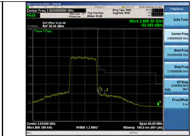
Band41-20MHz-16QAM-41140-100RB#0
