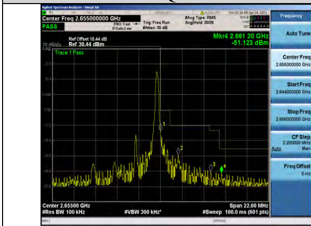
Band41-5MHz-16QAM-41215-1RB#24
