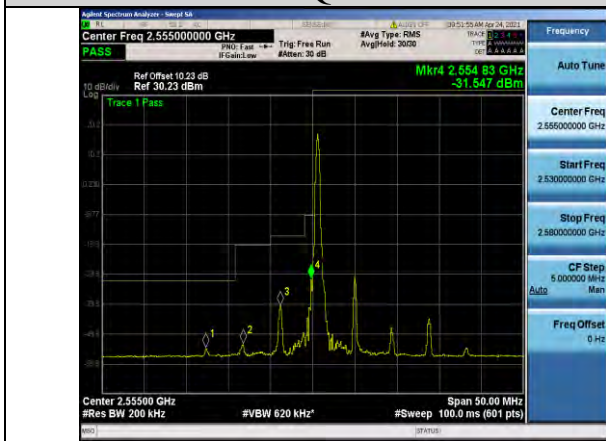
Band41-10MHz-16QAM-40290-1RB#0
