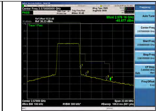
Band7-5MHz-16QAM-21425-25RB#0
