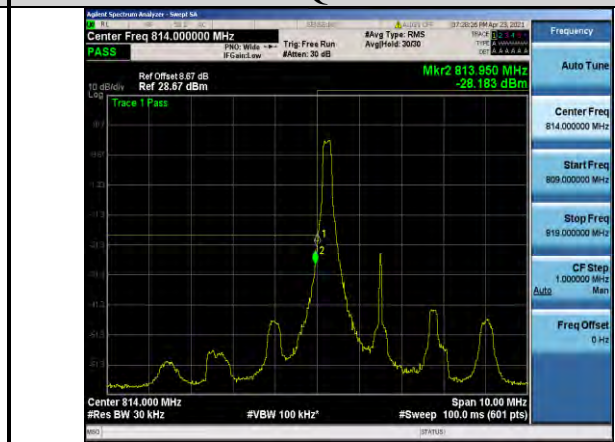
Band26-3MHz-16QAM-26705-1RB#0
