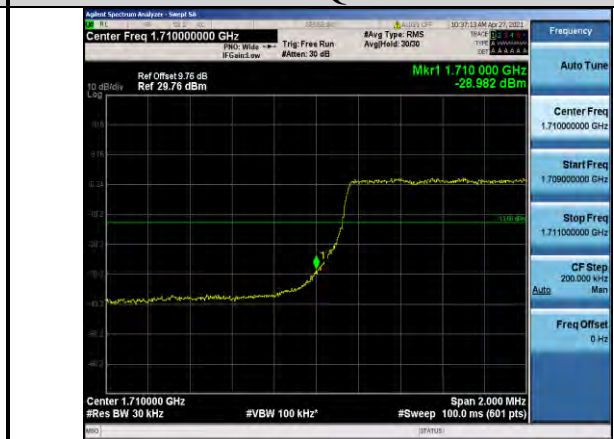
Band66-3MHz-16QAM-131987-15RB#0
