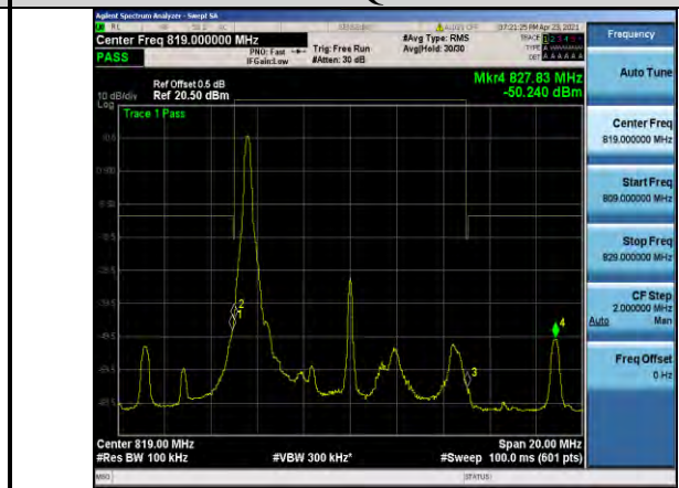
Band26-10MHz-QPSK-26740_Left-1RB#0
