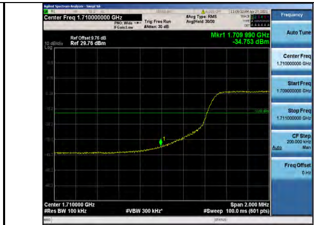
Band66-10MHz-16QAM-132022-50RB#0
