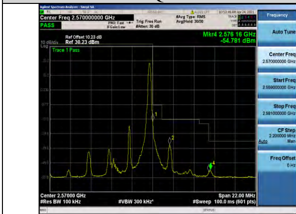
Band7-5MHz-16QAM-21425-1RB#24
