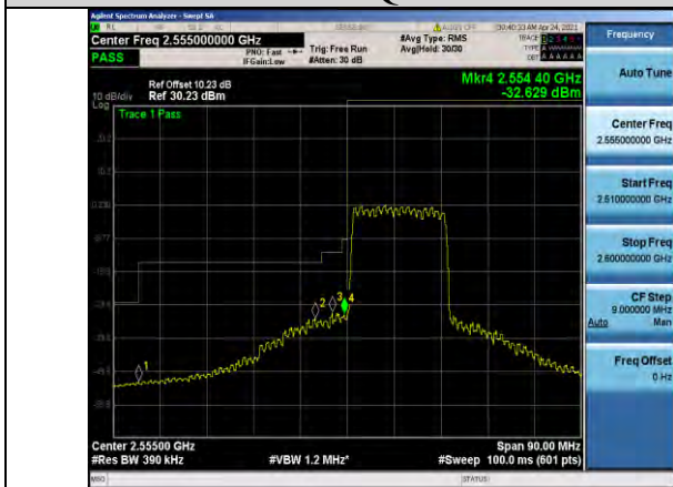
Band41-20MHz-16QAM-40340-100RB#0
