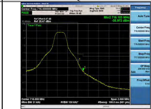
Band12-5MHz-QPSK-23155-1RB#24
