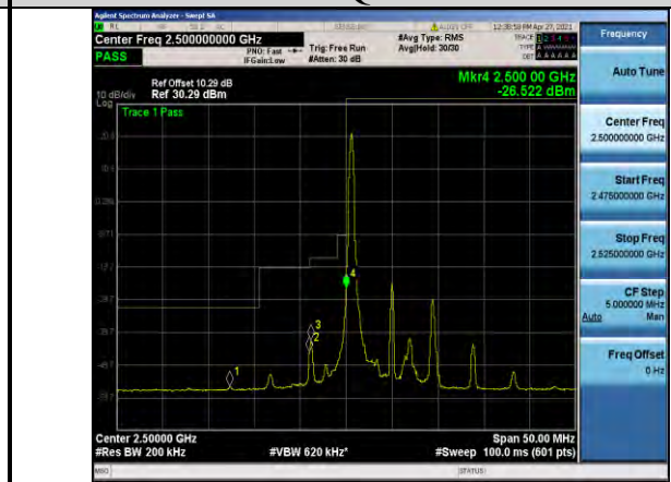
Band7-10MHz-QPSK-20800-1RB#0
