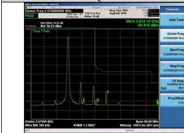
Band7-20MHz-16QAM-21350-1RB#0
