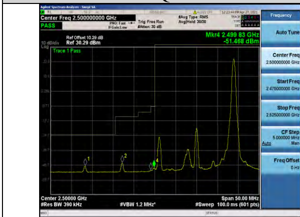
Band7-20MHz-QPSK-20850-1RB#99
