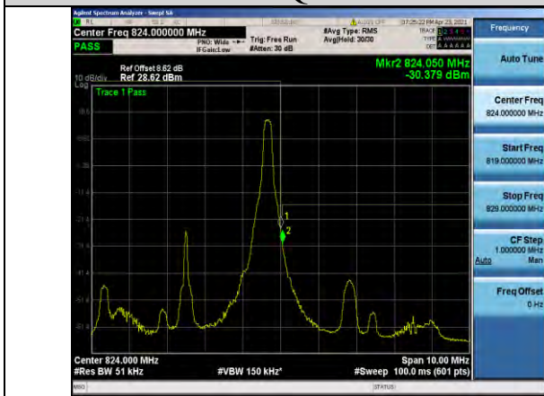
Band26-5MHz-16QAM-26765-1RB#24
