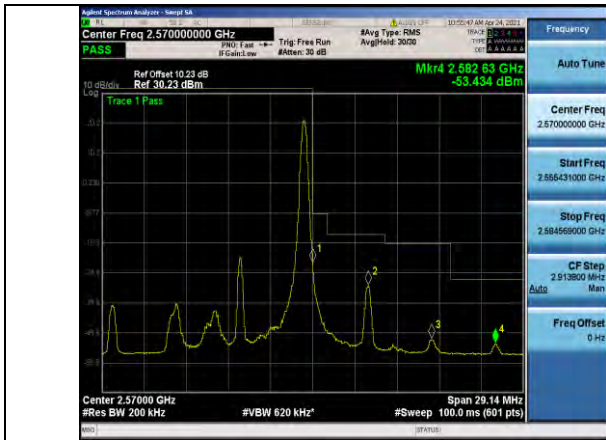
Band7-10MHz-QPSK-21400-1RB#49
