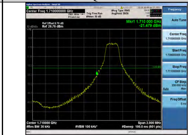
Band66-3MHz-16QAM-131987-1RB#0
