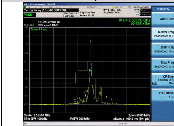
Band41-5MHz-QPSK-40265-1RB#0
