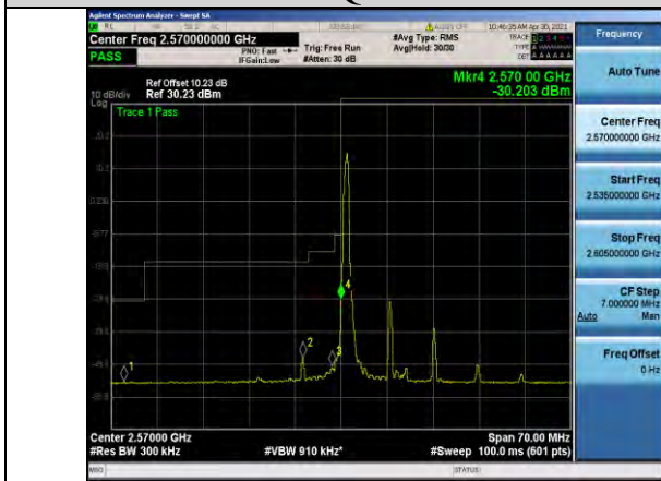
Band38-15MHz-16QAM-37825-1RB#0
