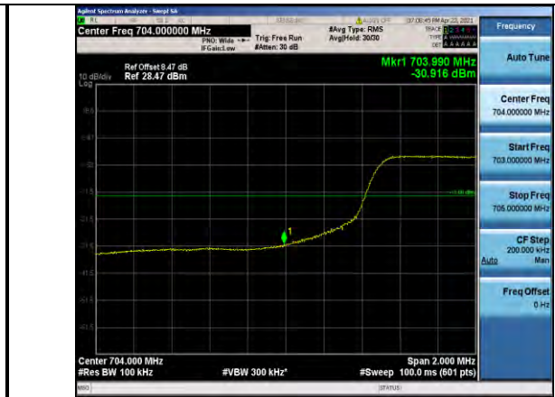
Band17-10MHz-QPSK-23780-50RB#0
