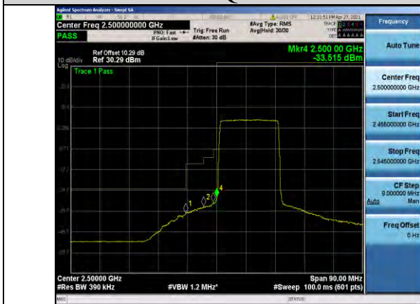
Band7-20MHz-16QAM-20850-100RB#0
