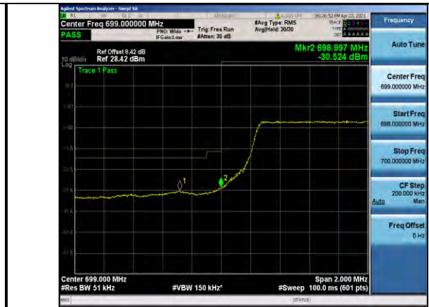
Band12-5MHz-QPSK-23035-25RB#0
