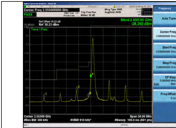
Band41-15MHz-QPSK-40315-1RB#0
