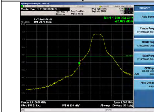
Band66-5MHz-QPSK-131997-1RB#0
