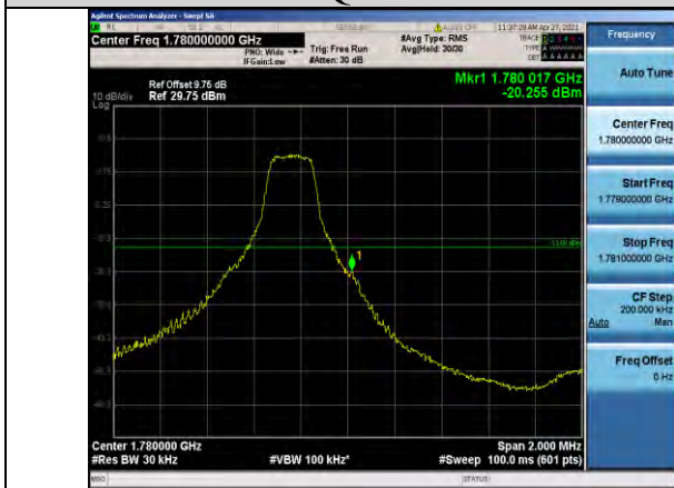
Band66-3MHz-QPSK-132657-1RB#14
