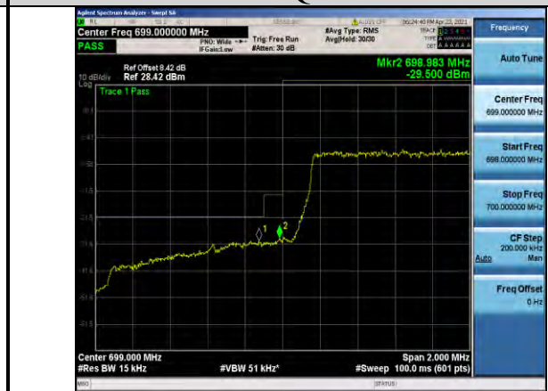
Band12-1.4MHz-QPSK-23017-6RB#0
