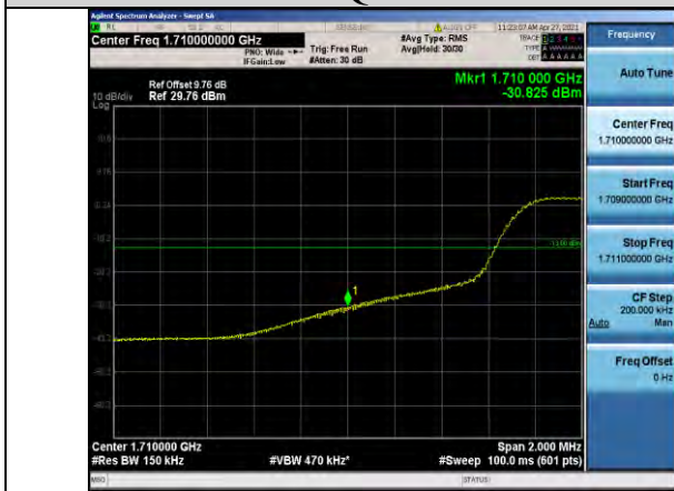
Band66-15MHz-QPSK-132047-75RB#0
