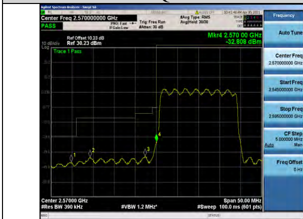
Band38-20MHz-QPSK-37850-100RB#0
