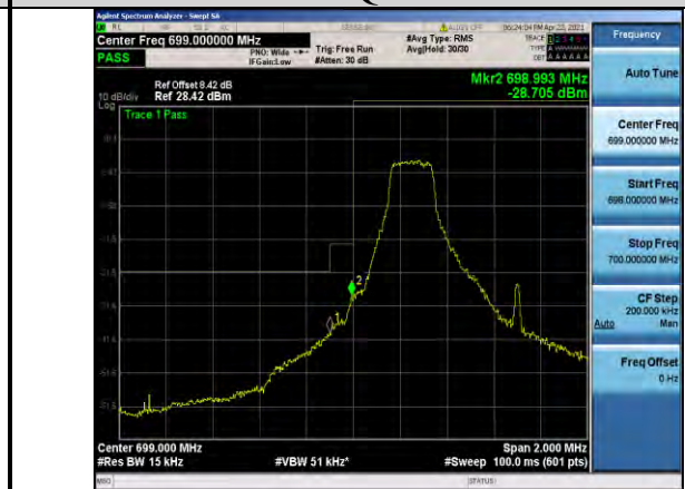
Band12-1.4MHz-QPSK-23017-1RB#0
