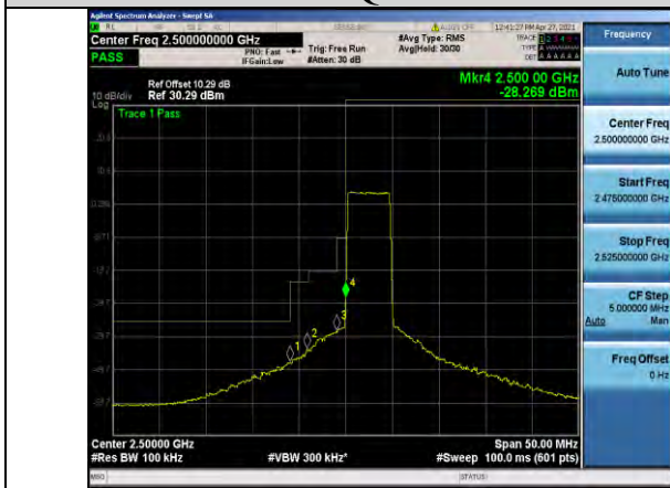
Band7-5MHz-16QAM-20775-25RB#0
