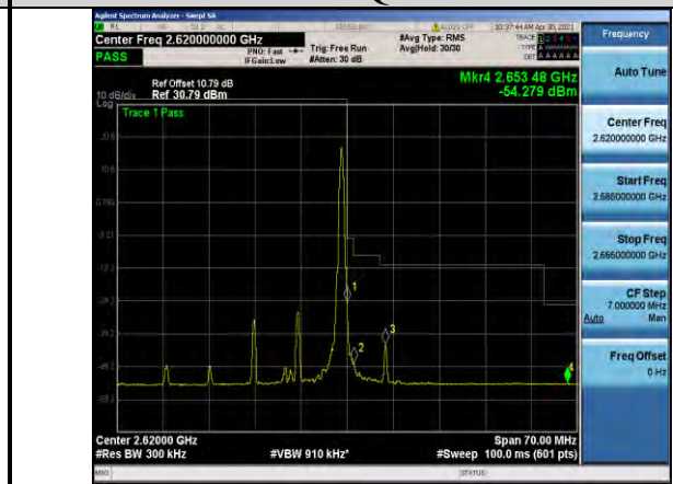
Band38-15MHz-16QAM-38175-1RB#74
