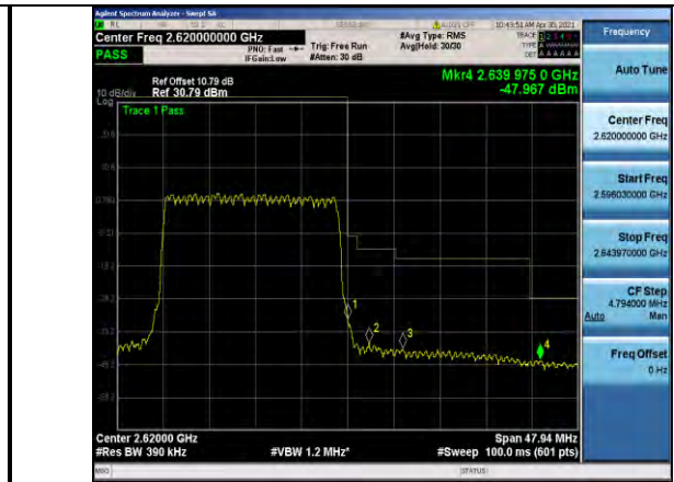
Band38-20MHz-QPSK-38150-100RB#0
