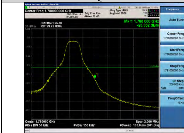
Band66-5MHz-16QAM-132647-1RB#24
