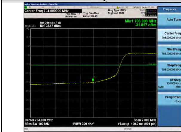
Band17-10MHz-16QAM-23780-50RB#0
