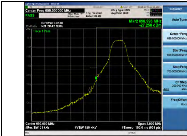
Band12-5MHz-16QAM-23035-1RB#0
