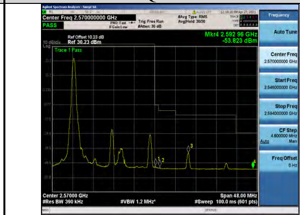
Band7-20MHz-QPSK-21350-1RB#0
