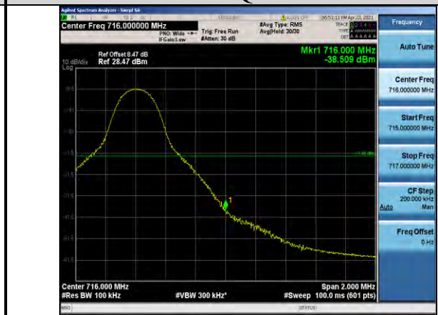
Band12-10MHz-16QAM-23130-1RB#49
