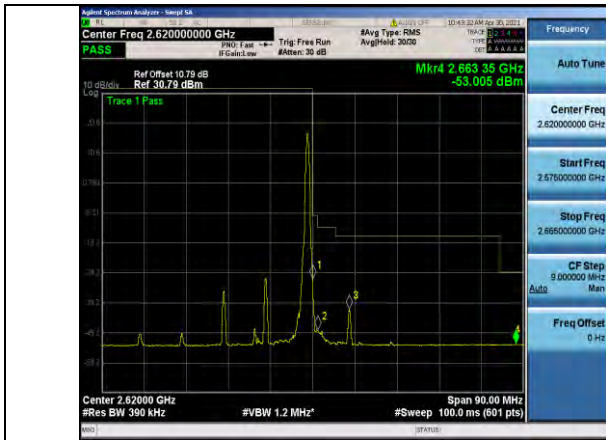
Band38-20MHz-16QAM-38150-1RB#99
