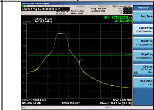
Band66-5MHz-QPSK-132647-1RB#24
