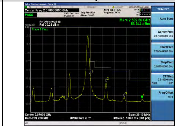
Band7-10MHz-16QAM-21400-1RB#49
