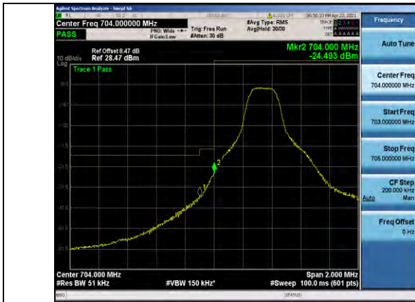
Band17-5MHz-QPSK-23755-1RB#0
