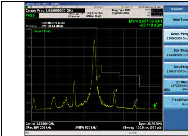
Band41-10MHz-QPSK-41190-1RB#49
