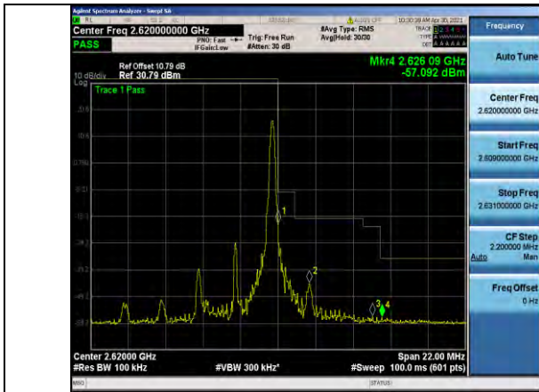
Band38-5MHz-16QAM-38225-1RB#24
