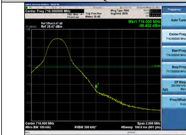
Band17-10MHz-16QAM-23800-1RB#49
