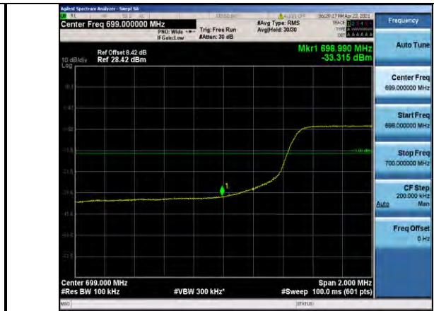
Band12-10MHz-16QAM-23060-50RB#0
