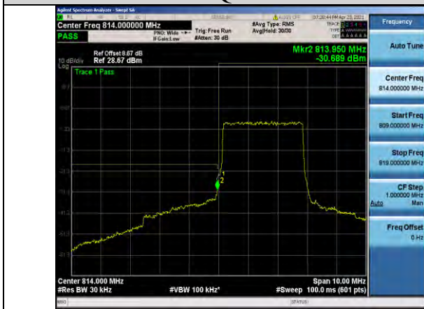
Band26-3MHz-QPSK-26705-15RB#0
