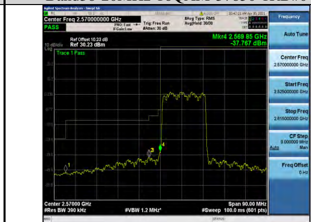
Band38-20MHz-16QAM-37850-100RB#0
