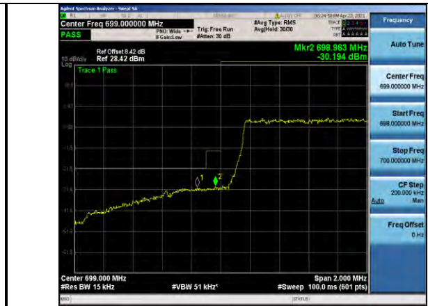
Band12-1.4MHz-16QAM-23017-6RB#0
