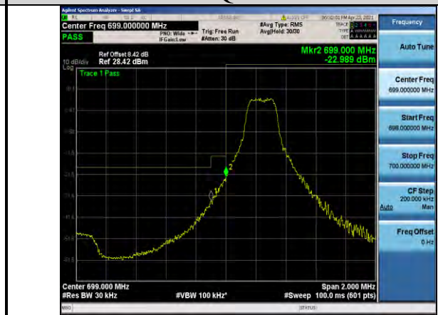
Band12-3MHz-16QAM-23025-1RB#0
