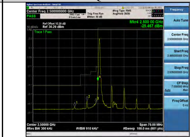
Band7-15MHz-16QAM-20825-1RB#0
