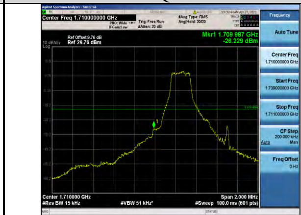
Band66-1.4MHz-QPSK-131979-1RB#0
