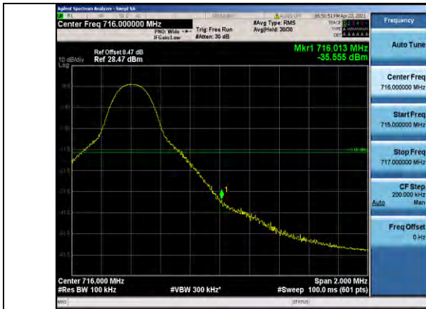
Band12-10MHz-QPSK-23130-1RB#49
