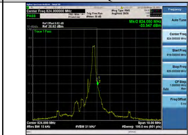
Band26-1.4MHz-16QAM-26783-1RB#5
