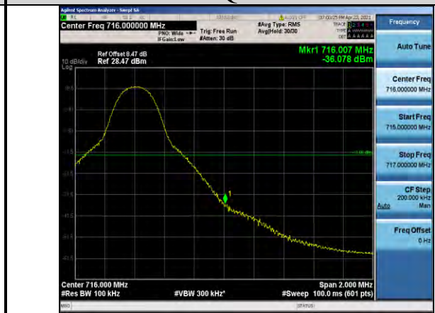
Band17-10MHz-QPSK-23800-1RB#49
