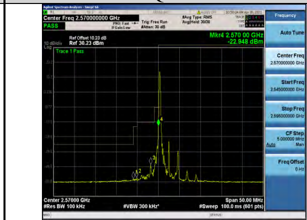
Band38-5MHz-16QAM-37775-1RB#0
