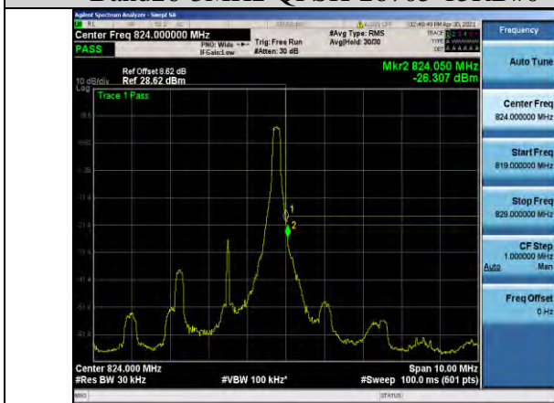
Band26-3MHz-QPSK-26775-1RB#14
