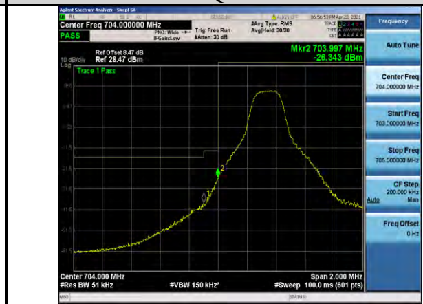
Band17-5MHz-16QAM-23755-1RB#0
