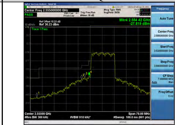
Band41-15MHz-16QAM-40315-75RB#0
