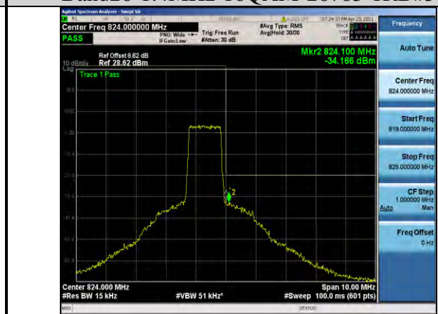
Band26-1.4MHz-16QAM-26783-6RB#0
