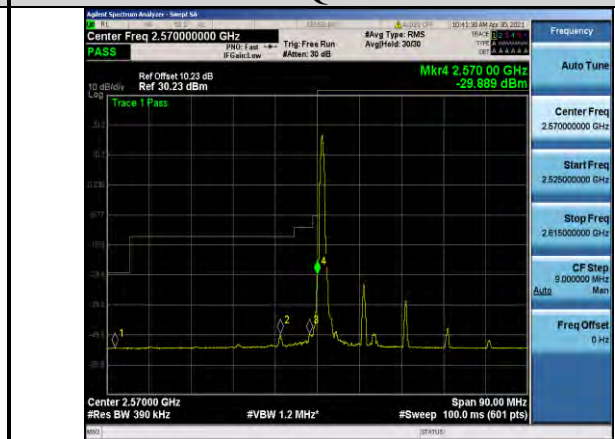
Band38-20MHz-16QAM-37850-1RB#0
