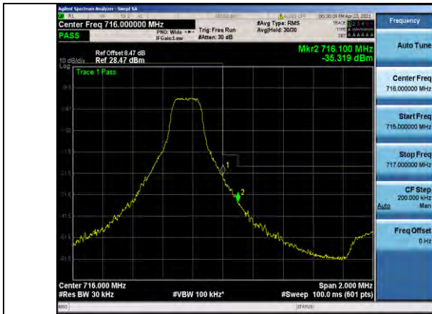
Band12-3MHz-16QAM-23165-1RB#14
