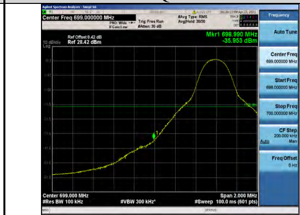
Band12-10MHz-QPSK-23060-1RB#0
