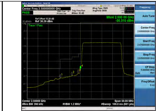
Band7-20MHz-QPSK-20850-100RB#0
