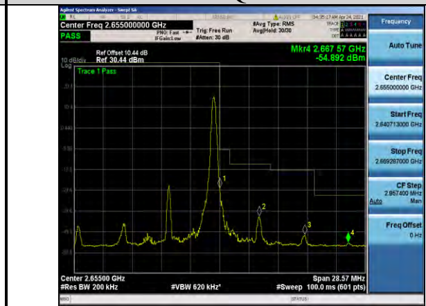
Band41-10MHz-16QAM-41190-1RB#49
