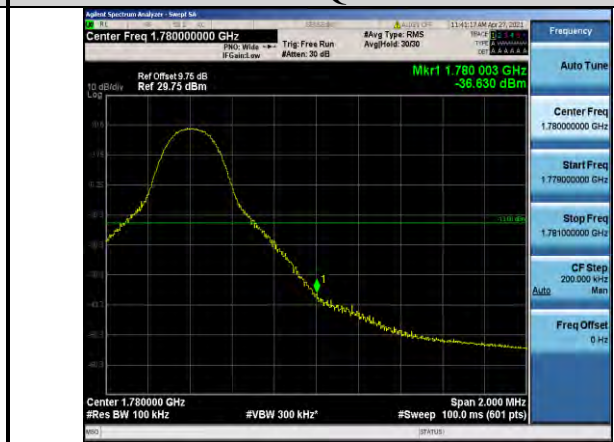
Band66-10MHz-16QAM-132622-1RB#49
