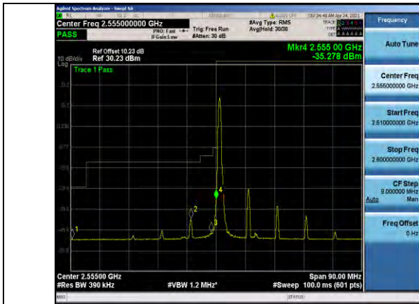
Band41-20MHz-16QAM-40340-1RB#0
