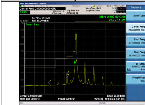
Band7-10MHz-16QAM-20800-1RB#0
