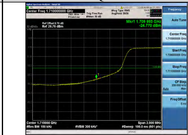
Band66-10MHz-QPSK-132022-1RB#0
