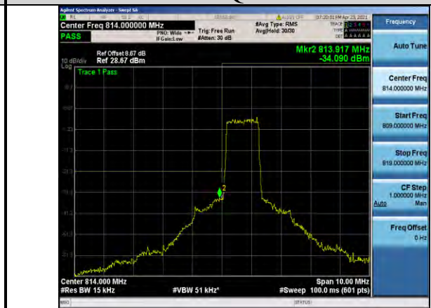
Band26-1.4MHz-QPSK-26697-6RB#0
