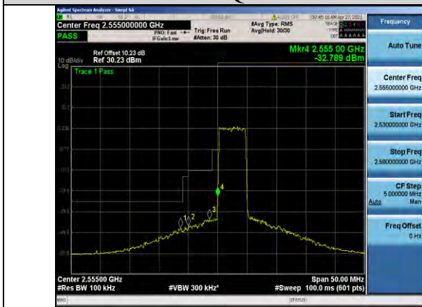
Band41-5MHz-16QAM-40265-25RB#0
