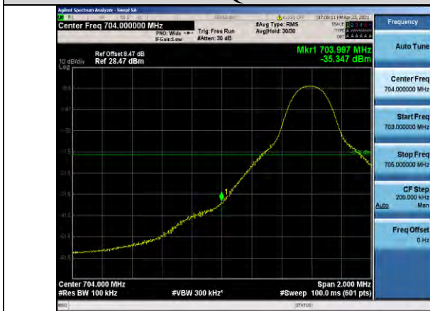
Band17-10MHz-QPSK-23780-1RB#0
