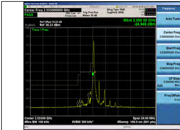
Band41-5MHz-16QAM-40265-1RB#0
