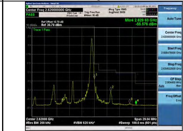
Band38-10MHz-QPSK-38200-1RB#49
