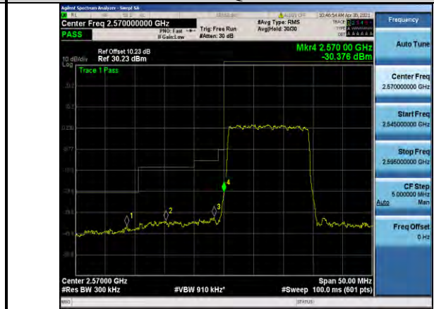
Band38-15MHz-QPSK-37825-75RB#0
