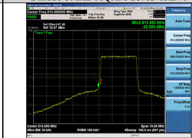
Band26-3MHz-16QAM-26705-15RB#0
