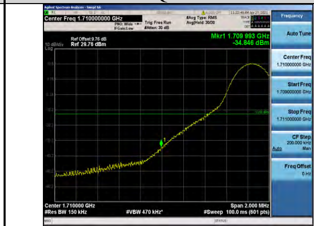
Band66-15MHz-16QAM-132047-1RB#0
