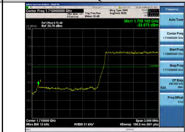
Band66-1.4MHz-QPSK-131979-6RB#0
