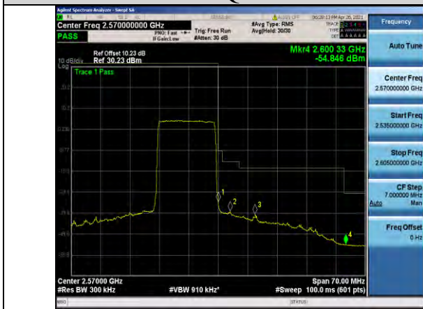
Band7-15MHz-16QAM-21375-75RB#0
