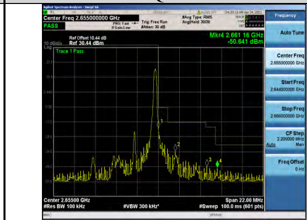
Band41-5MHz-QPSK-41215-1RB#24
