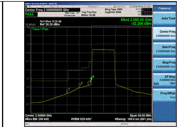
Band7-10MHz-16QAM-20800-50RB#0
