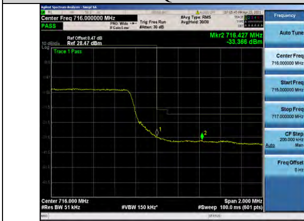
Band17-5MHz-16QAM-23825-25RB#0
