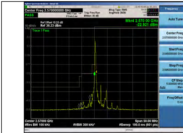
Band38-5MHz-QPSK-37775-1RB#0
