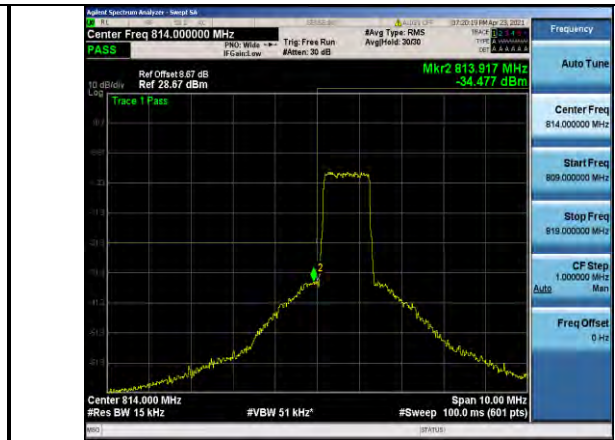
Band26-1.4MHz-16QAM-26697-6RB#0
