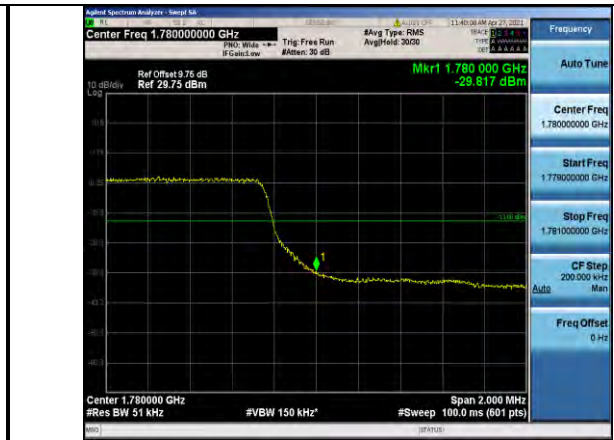
Band66-5MHz-16QAM-132647-25RB#0
