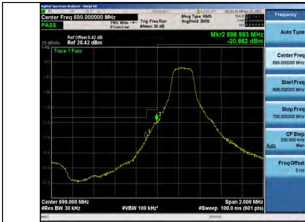
Band12-3MHz-QPSK-23025-1RB#0
