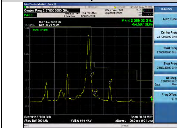
Band7-15MHz-QPSK-21375-1RB#74
