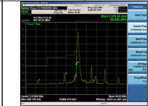
Band38-15MHz-QPSK-37825-1RB#0
