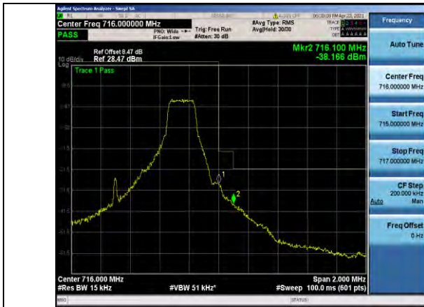
Band12-1.4MHz-QPSK-23173-1RB#5
