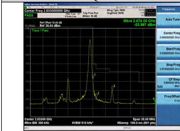
Band41-15MHz-QPSK-41165-1RB#74
