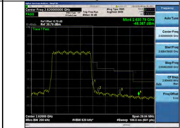
Band38-10MHz-QPSK-38200-50RB#0
