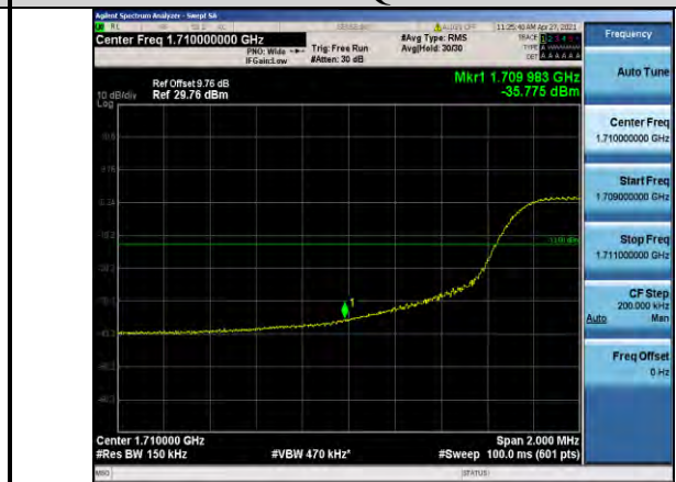
Band66-15MHz-16QAM-132047-75RB#0
