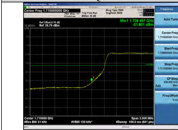
Band66-5MHz-16QAM-131997-25RB#0
