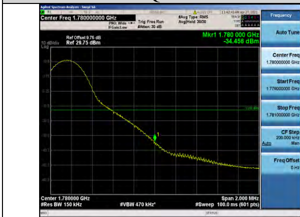
Band66-15MHz-QPSK-132597-1RB#74
