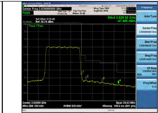
Band38-10MHz-16QAM-38200-50RB#0
