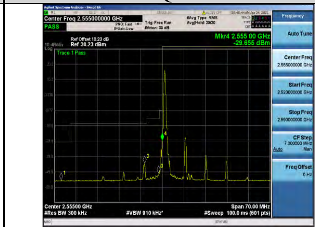
Band41-15MHz-16QAM-40315-1RB#0
