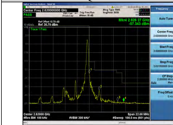
Band38-5MHz-QPSK-38225-1RB#24
