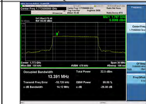
Band66-15MHz-QPSK-132597-75RB#0-13.391
