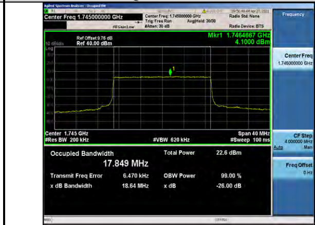
Band66-20MHz-QPSK-132322-100RB#0-17.849
