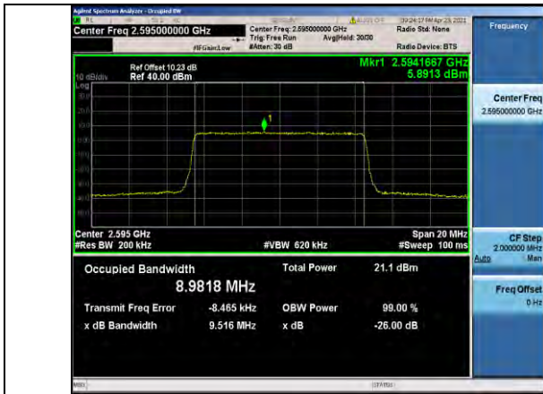
Band38-10MHz-16QAM-38000-50RB#0-8.9818
