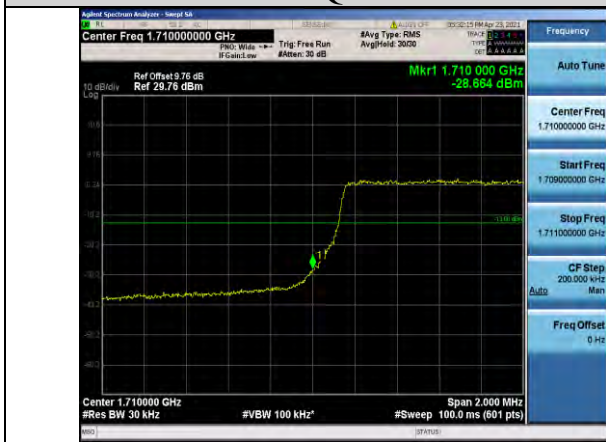
Band4-3MHz-16QAM-19965-15RB#0
