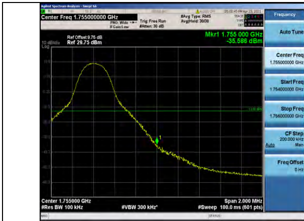
Band4-10MHz-16QAM-20350-1RB#49
