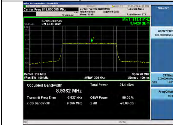
Band26-10MHz-16QAM-26740-50RB#0-8.9362
