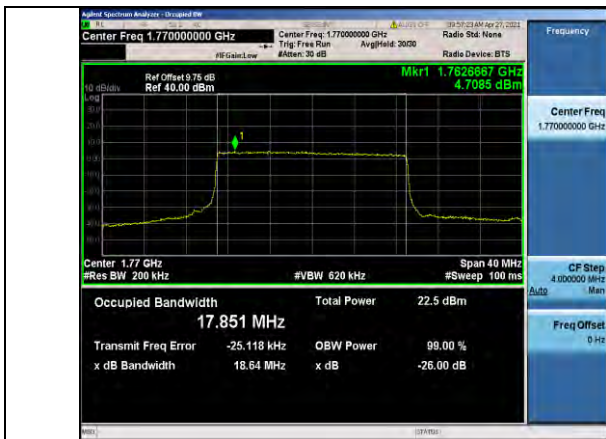
Band66-20MHz-QPSK-132572-100RB#0-17.851
