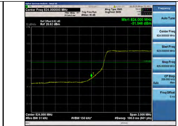
Band5-5MHz-16QAM-20425-25RB#0
