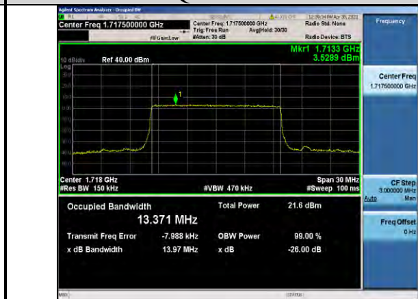
Band66-15MHz-16QAM-132047-75RB#0-13.371
