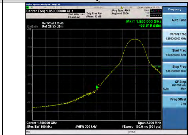
Band2-10MHz-16QAM-18650-1RB#0
