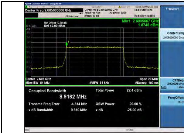
Band41-10MHz-16QAM-40740-50RB#0-8.9162
