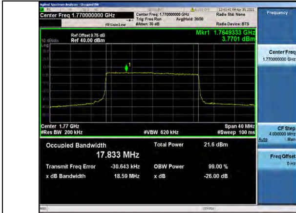
Band66-20MHz-16QAM-132572-100RB#0-17.833
