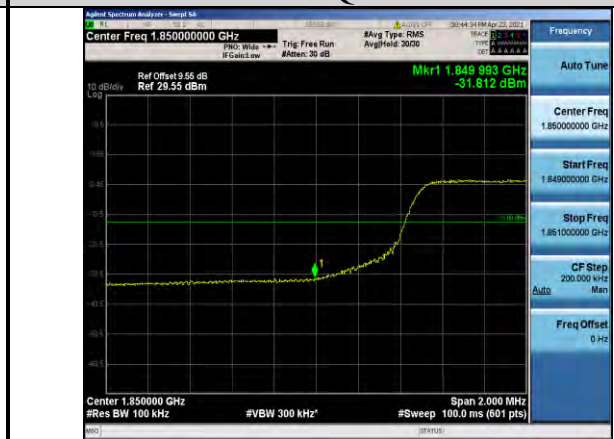
Band2-10MHz-16QAM-18650-50RB#0
