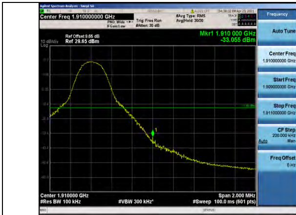
Band2-10MHz-16QAM-19150-1RB#49
