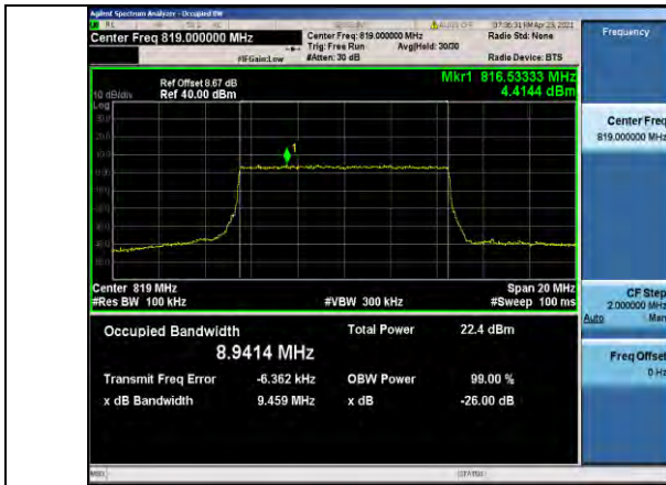
Band26-10MHz-QPSK-26740-50RB#0-8.9414
