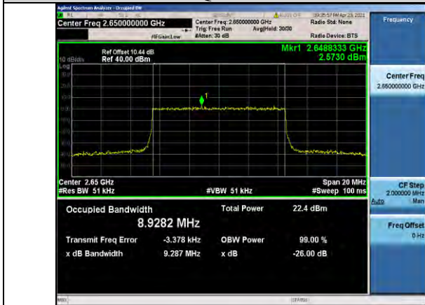
Band41-10MHz-16QAM-41190-50RB#0-8.9282
