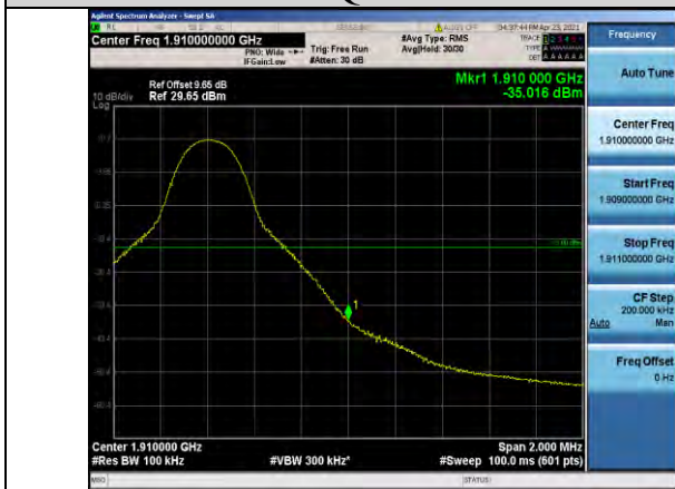
Band2-10MHz-QPSK-19150-1RB#49
