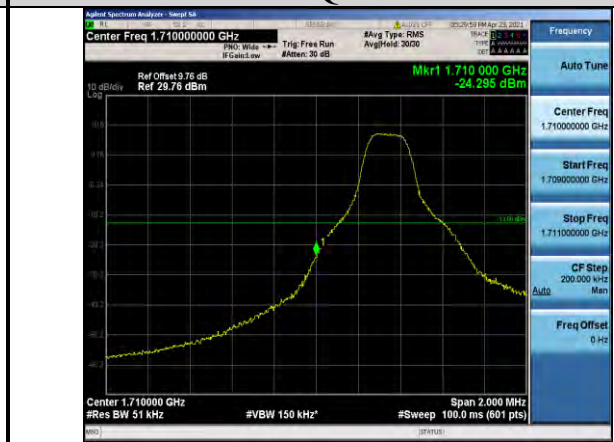
Band4-5MHz-QPSK-19975-1RB#0
