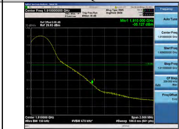
Band2-15MHz-QPSK-19125-1RB#74
