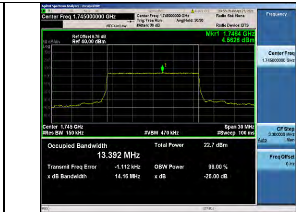
Band66-15MHz-QPSK-132322-75RB#0-13.392
