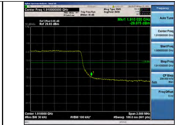
Band2-3MHz-16QAM-19185-15RB#0
