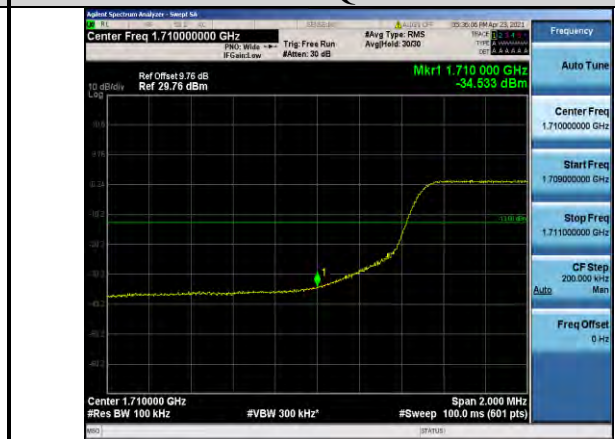
Band4-10MHz-16QAM-20000-50RB#0
