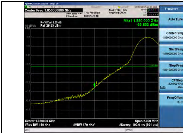
Band2-15MHz-16QAM-18675-1RB#0
