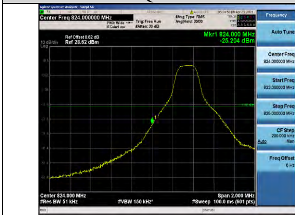
Band5-5MHz-16QAM-20425-1RB#0
