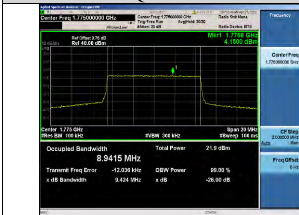
Band66-10MHz-16QAM-132622-50RB#0-8.9415
