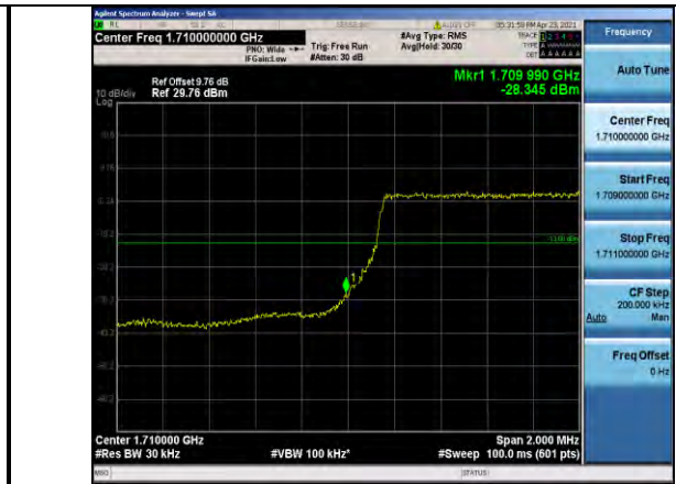
Band4-3MHz-QPSK-19965-15RB#0
