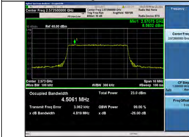
Band38-5MHz-QPSK-37775-25RB#0-4.5061
