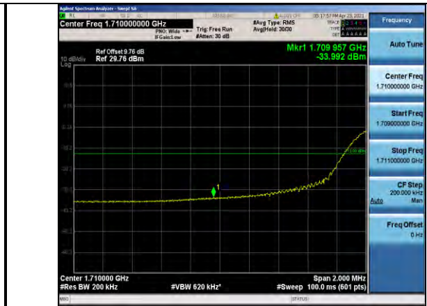
Band4-20MHz-16QAM-20050-100RB#0
