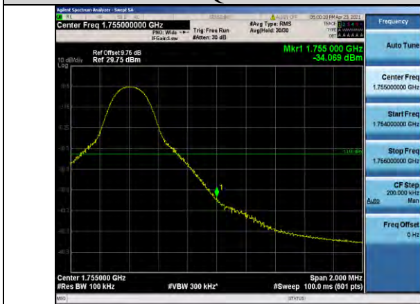
Band4-10MHz-QPSK-20350-1RB#49
