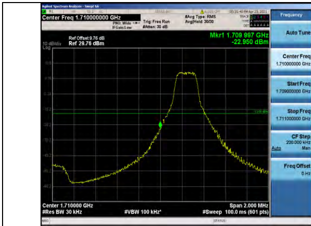
Band4-3MHz-16QAM-19965-1RB#0
