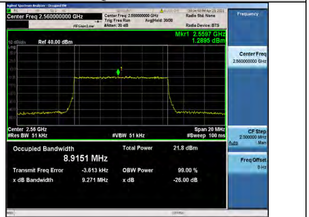
Band41-10MHz-16QAM-40290-50RB#0-8.9151
