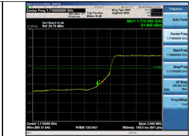
Band4-5MHz-16QAM-19975-25RB#0
