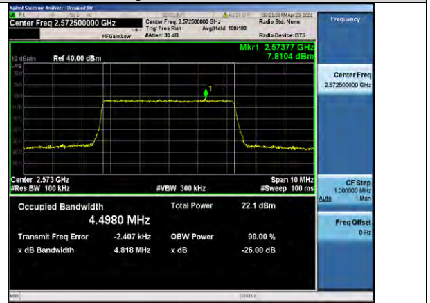
Band38-5MHz-16QAM-37775-25RB#0-4.4980
