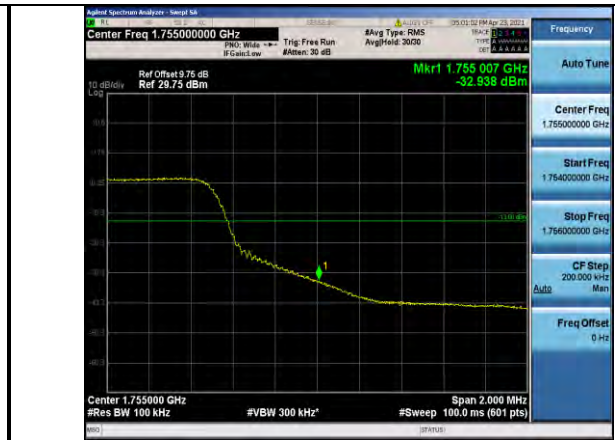
Band4-10MHz-QPSK-20350-50RB#0
