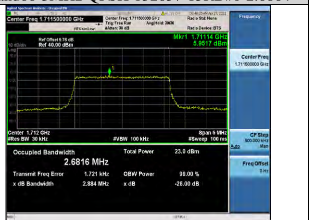
Band66-3MHz-16QAM-131987-15RB#0-2.6816
