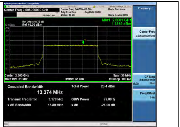
Band41-15MHz-QPSK-40740-75RB#0-13.374
