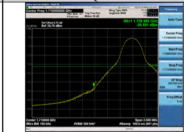
Band4-10MHz-16QAM-20000-1RB#0
