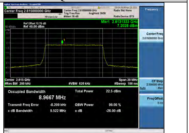
Band38-10MHz-QPSK-38200-50RB#0-8.9667
