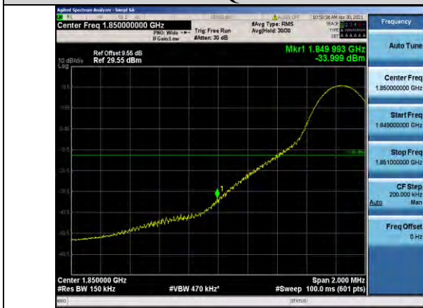
Band2-15MHz-QPSK-18675-1RB#0
