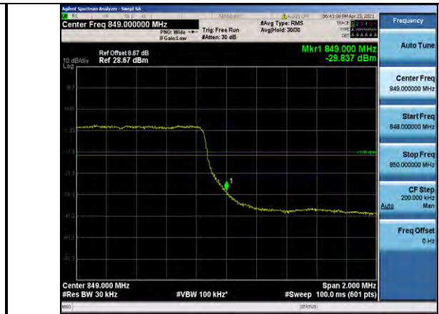
Band5-3MHz-16QAM-20635-15RB#0
