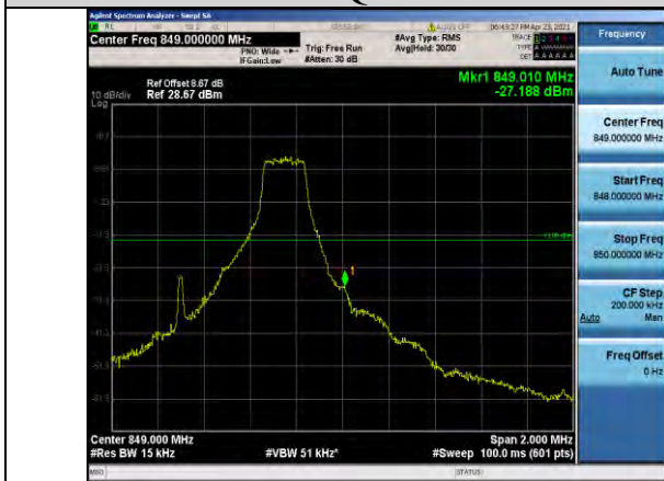
Band5-1.4MHz-QPSK-20643-1RB#5
