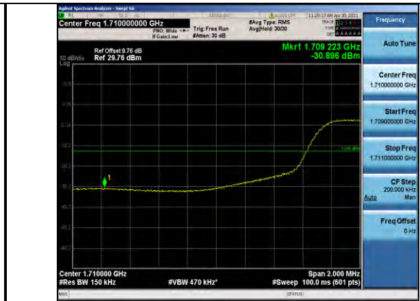
Band4-15MHz-QPSK-20025-75RB#0
