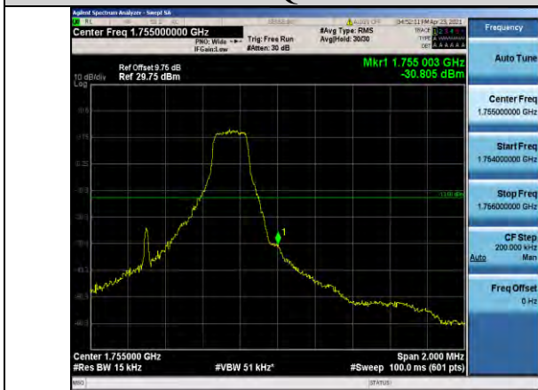
Band4-1.4MHz-QPSK-20393-1RB#5
