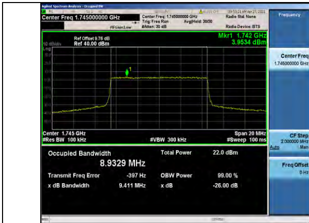
Band66-10MHz-16QAM-132322-50RB#0-8.9329
