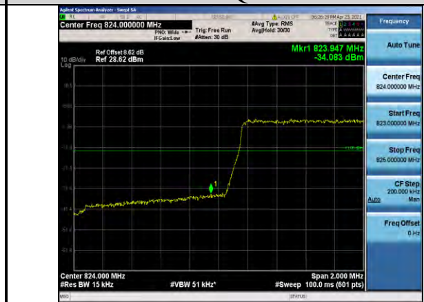
Band5-1.4MHz-16QAM-20407-6RB#0
