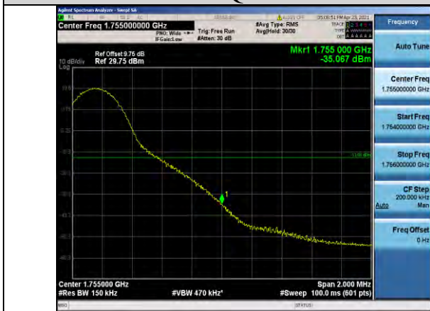
Band4-15MHz-16QAM-20325-1RB#74
