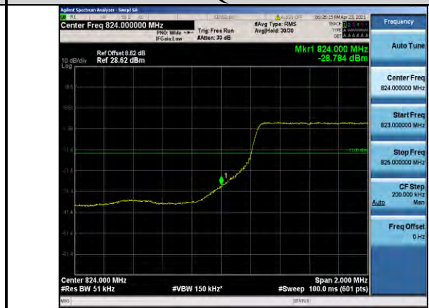
Band5-5MHz-QPSK-20425-25RB#0
