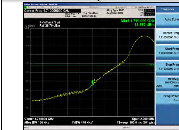
Band4-15MHz-QPSK-20025-1RB#0
