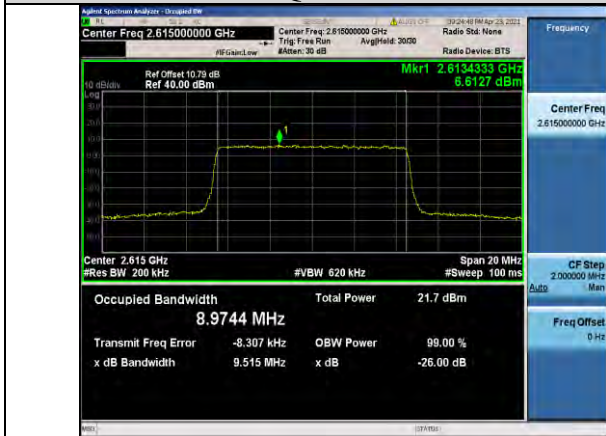
Band38-10MHz-16QAM-38200-50RB#0-8.9744
