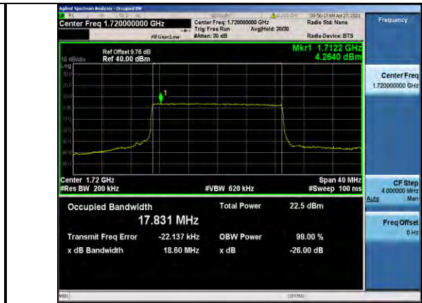
Band66-20MHz-QPSK-132072-100RB#0-17.831
