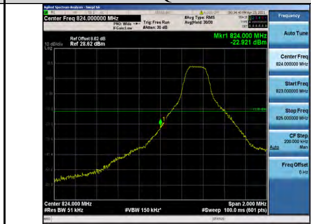
Band5-5MHz-QPSK-20425-1RB#0
