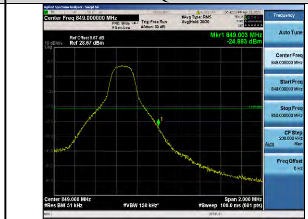
Band5-5MHz-16QAM-20625-1RB#24
