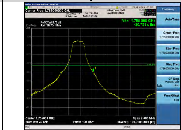
Band4-3MHz-QPSK-20385-1RB#14
