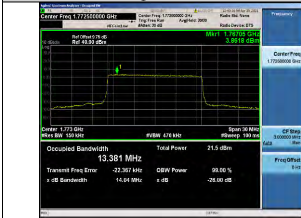
Band66-15MHz-16QAM-132597-75RB#0-13.381
