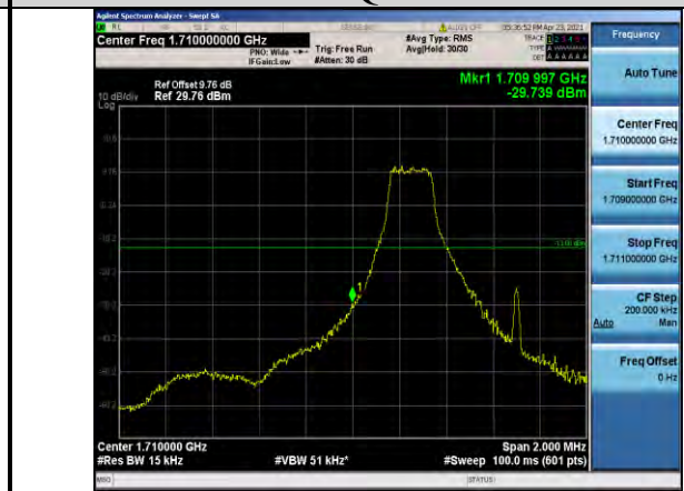
Band4-1.4MHz-16QAM-19957-1RB#0
