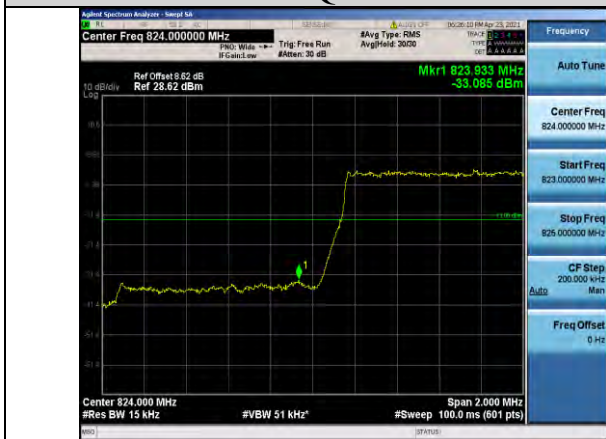
Band5-1.4MHz-QPSK-20407-6RB#0
