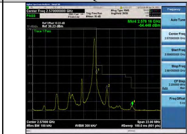
Band7-5MHz-QPSK-21425-1RB#24
