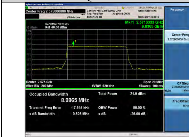
Band38-10MHz-QPSK-37800-50RB#0-8.9865
