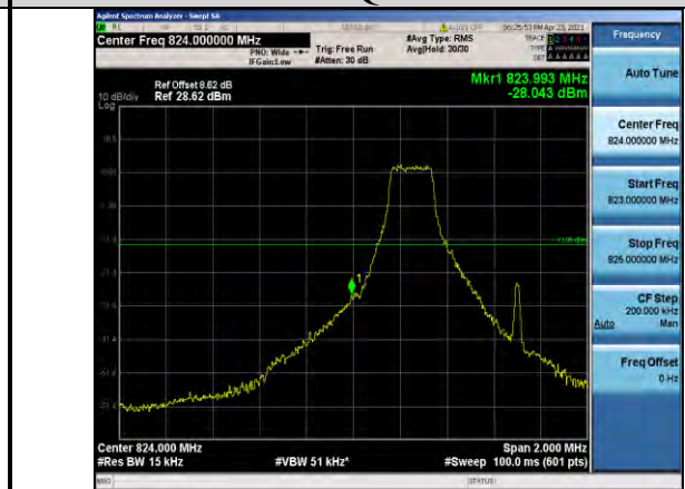
Band5-1.4MHz-16QAM-20407-1RB#0
