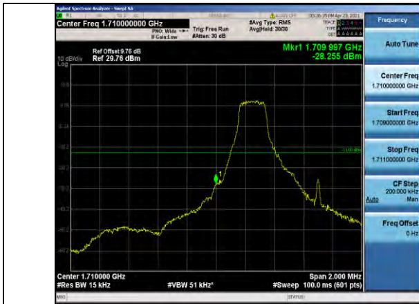
Band4-1.4MHz-QPSK-19957-1RB#0
