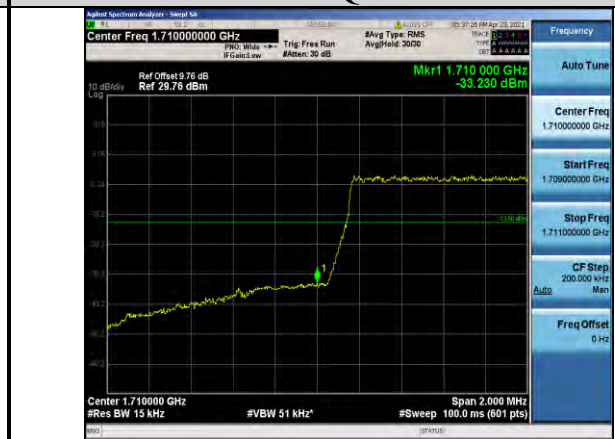
Band4-1.4MHz-16QAM-19957-6RB#0
