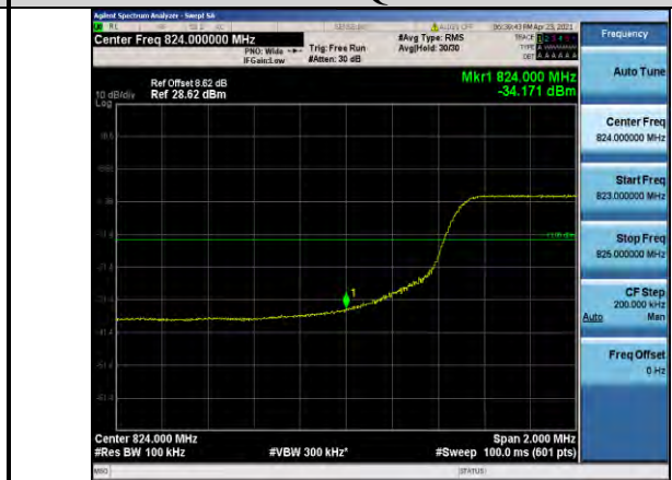
Band5-10MHz-16QAM-20450-50RB#0
