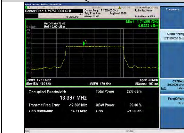
Band66-15MHz-QPSK-132047-75RB#0-13.397
