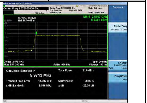
Band38-10MHz-16QAM-37800-50RB#0-8.9713
