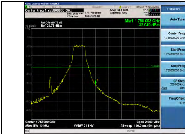
Band4-1.4MHz-16QAM-20393-1RB#5
