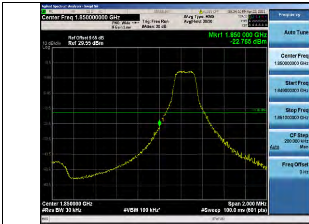
Band2-3MHz-16QAM-18615-1RB#0
