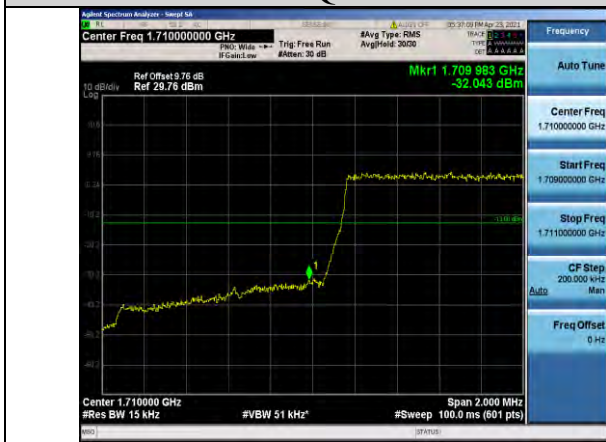
Band4-1.4MHz-QPSK-19957-6RB#0
