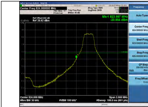
Band5-3MHz-16QAM-20415-1RB#0
