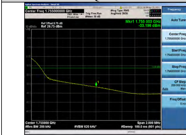
Band4-20MHz-QPSK-20300-100RB#0
