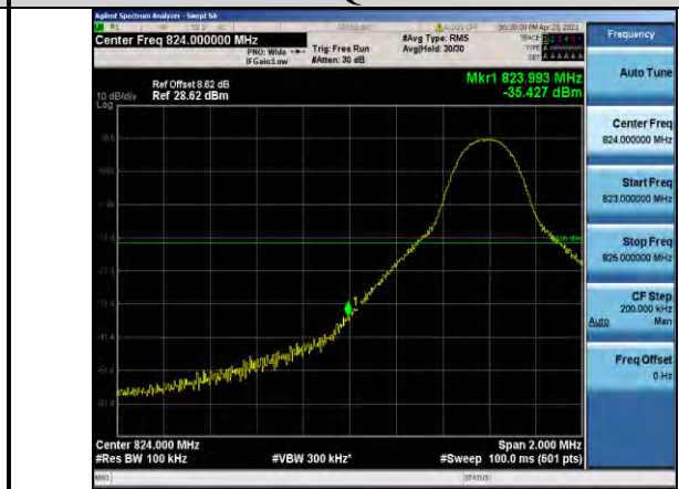
Band5-10MHz-16QAM-20450-1RB#0
