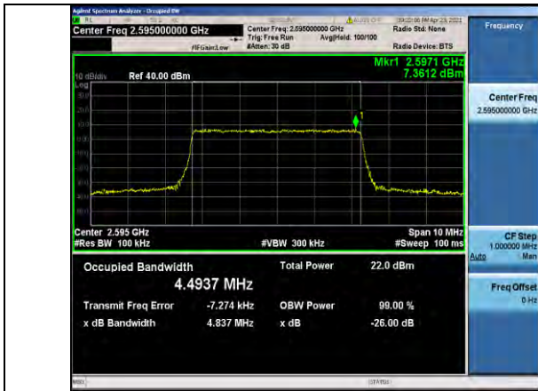
Band38-5MHz-16QAM-38000-25RB#0-4.4937
