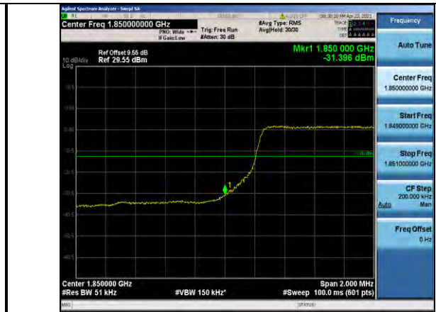
Band2-5MHz-16QAM-18625-25RB#0
