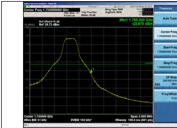
Band4-5MHz-QPSK-20375-1RB#24
