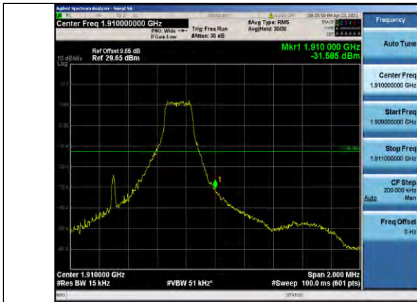
Band2-1.4MHz-16QAM-19193-1RB#5
