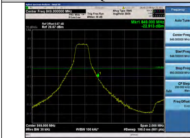
Band5-3MHz-16QAM-20635-1RB#14
