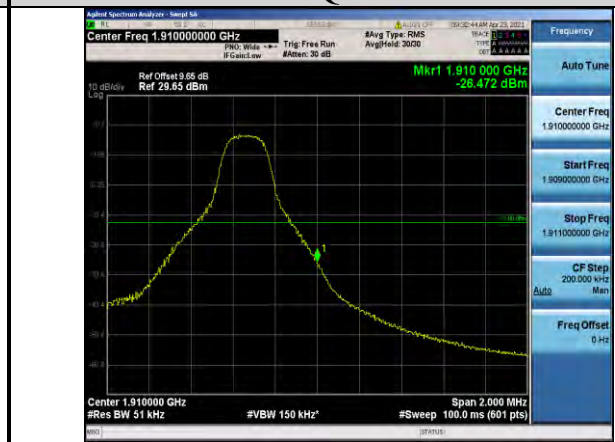
Band2-5MHz-16QAM-19175-1RB#24
