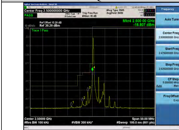
Band7-5MHz-QPSK-20775-1RB#0
