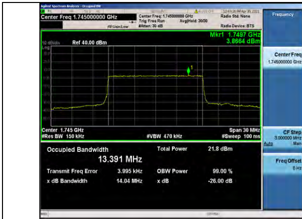
Band66-15MHz-16QAM-132322-75RB#0-13.391
