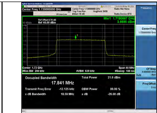
Band66-20MHz-16QAM-132072-100RB#0-17.841
