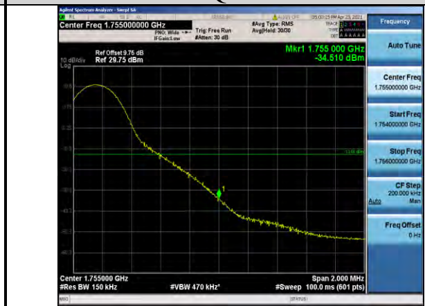
Band4-15MHz-QPSK-20325-1RB#74
