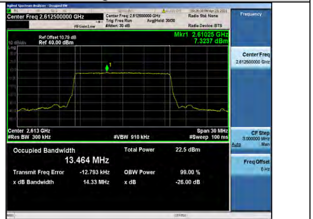
Band38-15MHz-QPSK-38175-75RB#0-13.464
