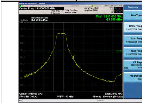
Band2-3MHz-16QAM-19185-1RB#14
