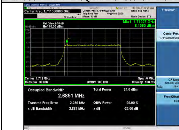
Band66-3MHz-QPSK-131987-15RB#0-2.6851
