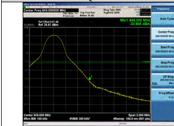
Band5-10MHz-QPSK-20600-1RB#49
