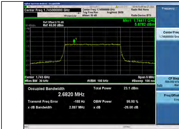
Band66-3MHz-16QAM-132322-15RB#0-2.6820
