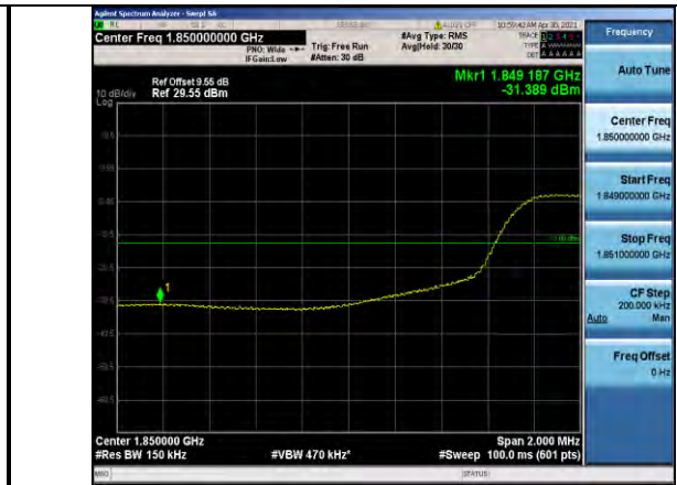
Band2-15MHz-QPSK-18675-75RB#0
