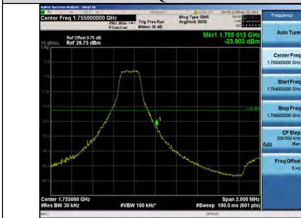
Band4-3MHz-16QAM-20385-1RB#14
