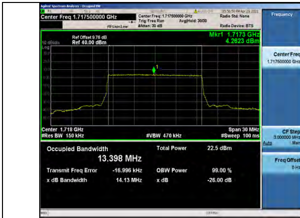
Band4-15MHz-QPSK-20025-75RB#0-13.398
