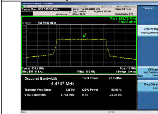
Band5-5MHz-QPSK-20525-25RB#0-4.4747
