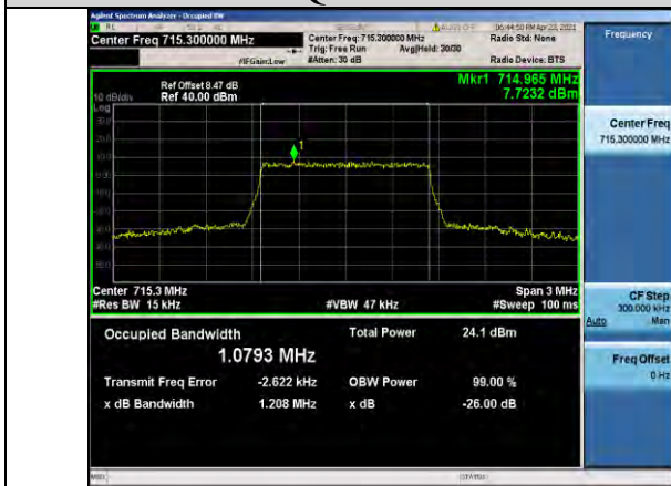
Band12-1.4MHz-QPSK-23173-6RB#0-1.0793
