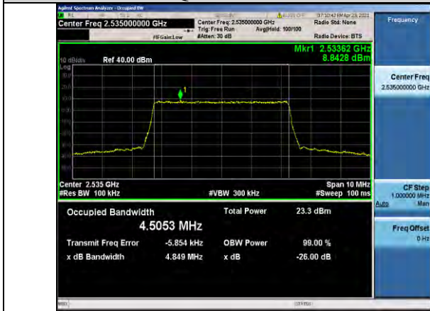
Band7-5MHz-QPSK-21100-25RB#0-4.5053
