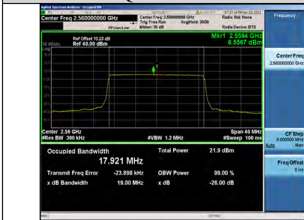
Band7-20MHz-QPSK-21350-100RB#0-17.921
