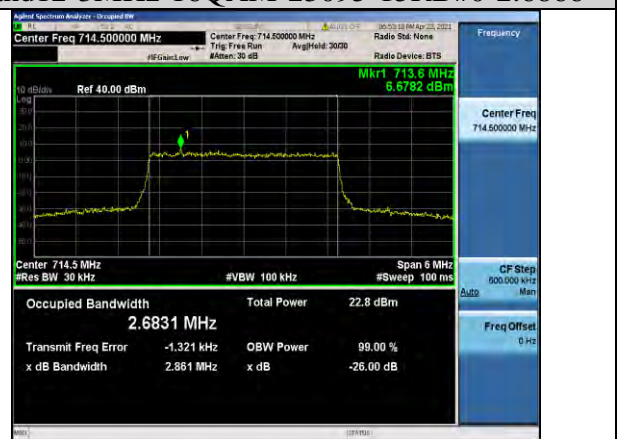
Band12-3MHz-16QAM-23165-15RB#0-2.6831
