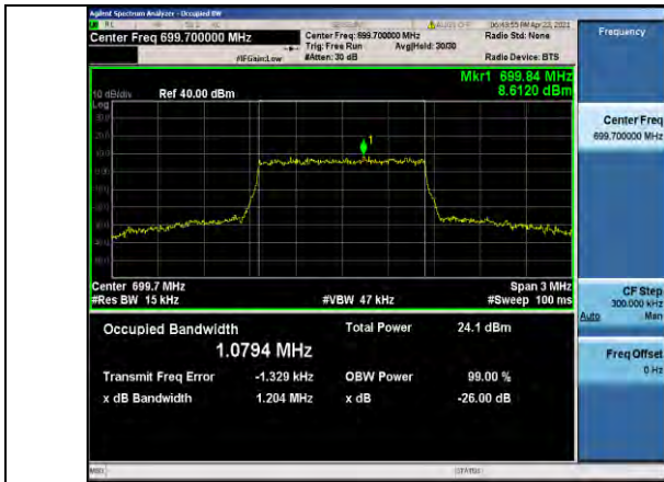
Band12-1.4MHz-QPSK-23017-6RB#0-1.0794
