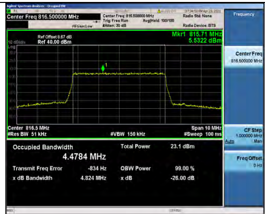
Band26-5MHz-16QAM-26715-25RB#0-4.4784
