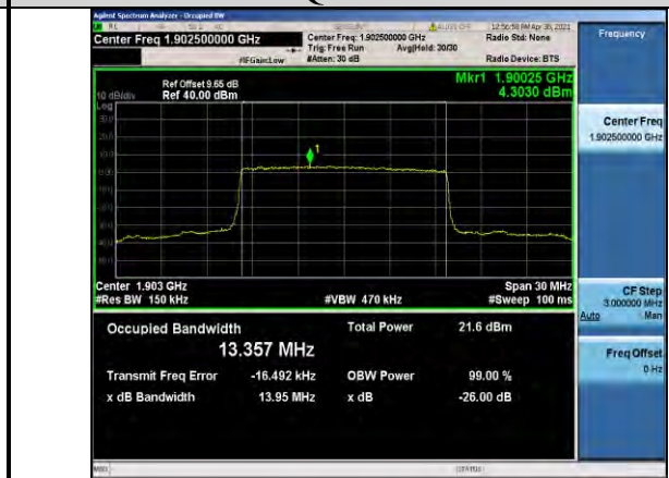
Band2-15MHz-16QAM-19125-75RB#0-13.357
