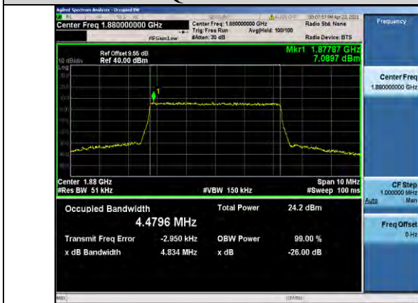
Band2-5MHz-QPSK-18900-25RB#0-4.4796
