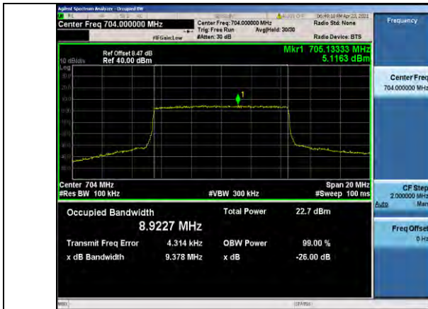
Band12-10MHz-QPSK-23060-50RB#0-8.9227
