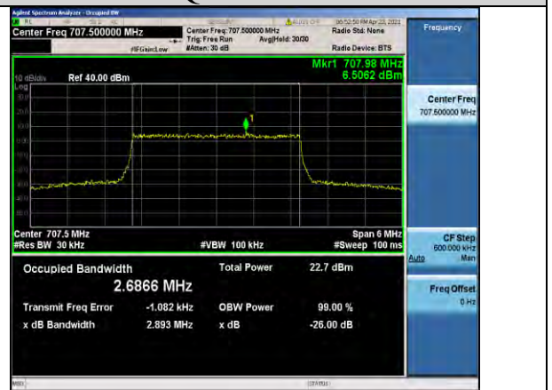
Band12-3MHz-16QAM-23095-15RB#0-2.6866
