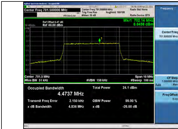
Band12-5MHz-QPSK-23035-25RB#0-4.4737
