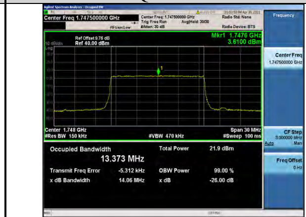
Band4-15MHz-16QAM-20325-75RB#0-13.373
