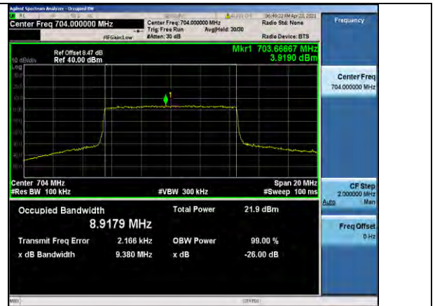
Band12-10MHz-16QAM-23060-50RB#0-8.9179
