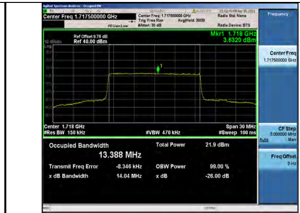
Band4-15MHz-16QAM-20025-75RB#0-13.388
