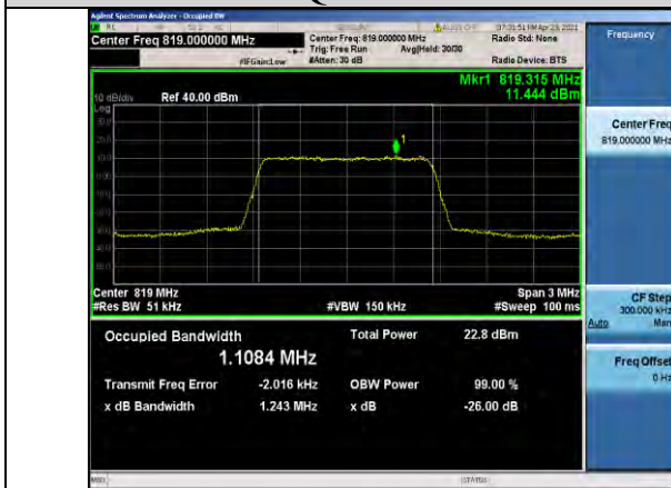
Band26-1.4MHz-QPSK-26740-6RB#0-1.1084
