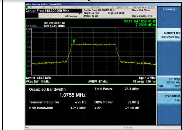
Band5-1.4MHz-16QAM-20643-6RB#0-1.0755
