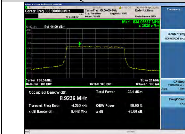
Band5-10MHz-QPSK-20525-50RB#0-8.9236
