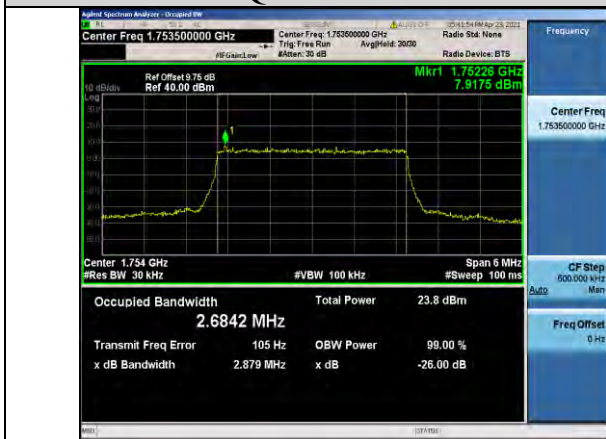
Band4-3MHz-QPSK-20385-15RB#0-2.6842
