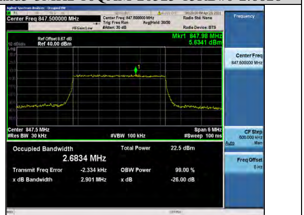
Band5-3MHz-16QAM-20635-15RB#0-2.6834
