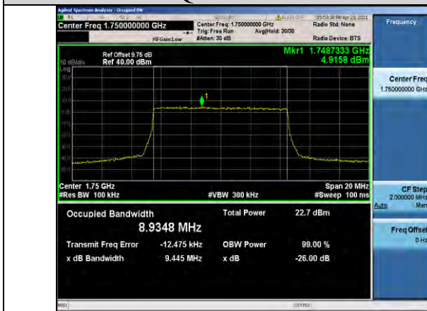
Band4-10MHz-QPSK-20350-50RB#0-8.9348
