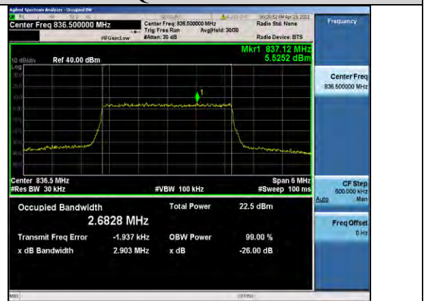
Band5-3MHz-16QAM-20525-15RB#0-2.6828
