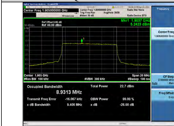
Band2-10MHz-QPSK-19150-50RB#0-8.9313
