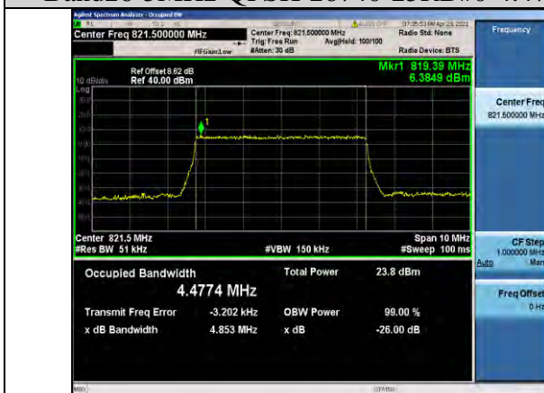
Band26-5MHz-QPSK-26765-25RB#0-4.4774
