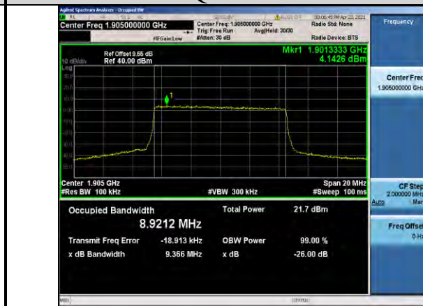
Band2-10MHz-16QAM-19150-50RB#0-8.9212
