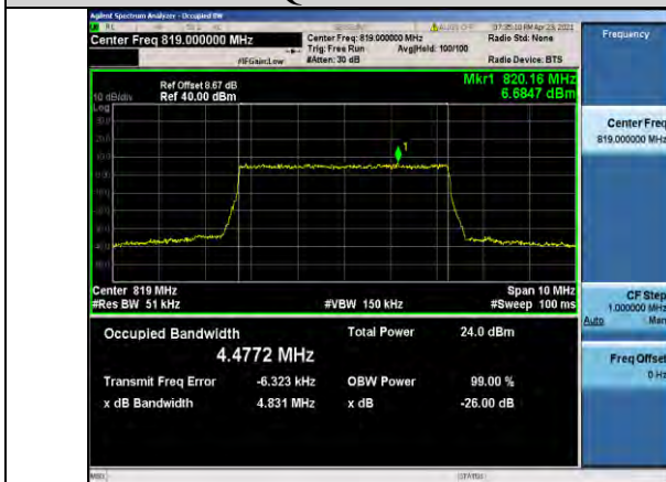
Band26-5MHz-QPSK-26740-25RB#0-4.4772
