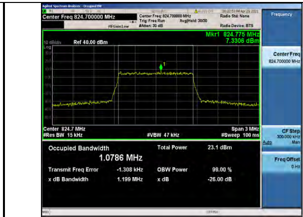
Band5-1.4MHz-16QAM-20407-6RB#0-1.0786
