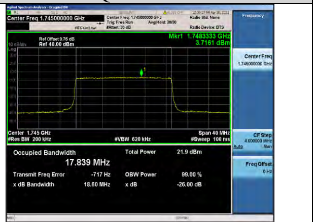
Band4-20MHz-16QAM-20300-100RB#0-17.839
