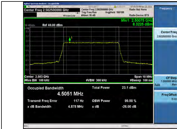
Band7-5MHz-QPSK-20775-25RB#0-4.5051
