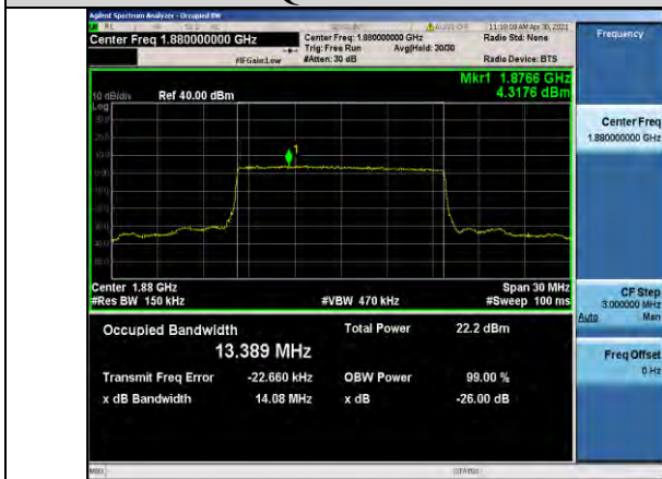
Band2-15MHz-QPSK-18900-75RB#0-13.389
