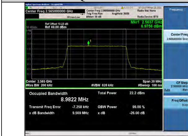
Band7-10MHz-QPSK-21400-50RB#0-8.9822
