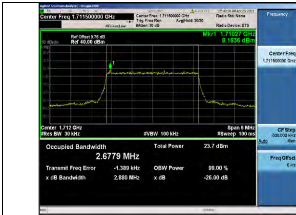
Band4-3MHz-QPSK-19965-15RB#0-2.6779
