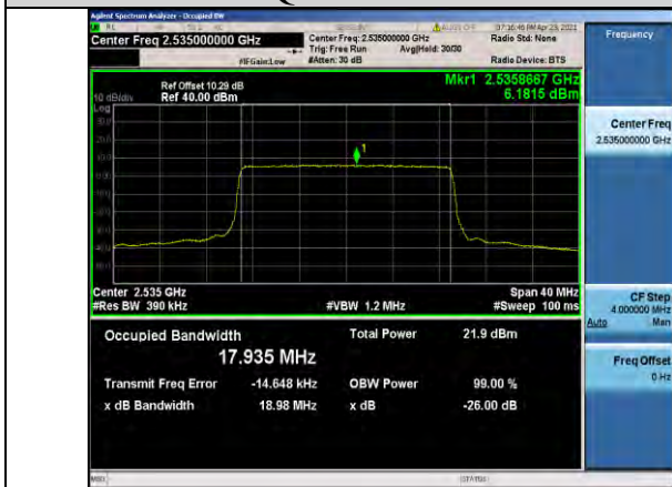
Band7-20MHz-QPSK-21100-100RB#0-17.935
