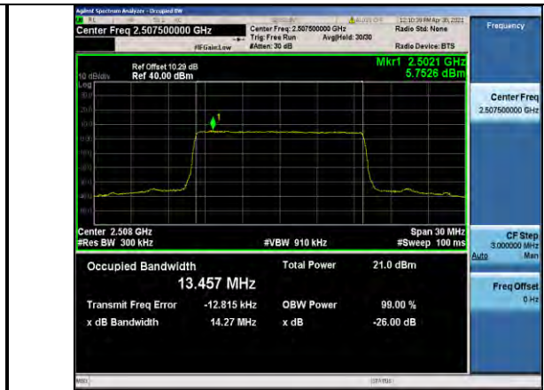
Band7-15MHz-16QAM-20825-75RB#0-13.457
