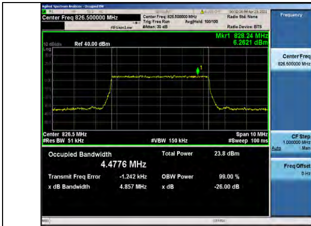
Band5-5MHz-QPSK-20425-25RB#0-4.4776
