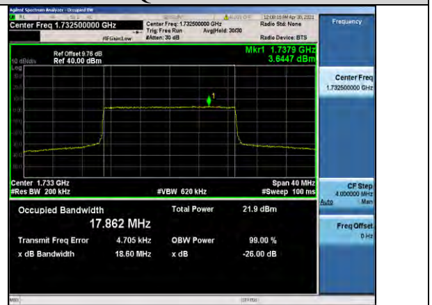
Band4-20MHz-16QAM-20175-100RB#0-17.862
