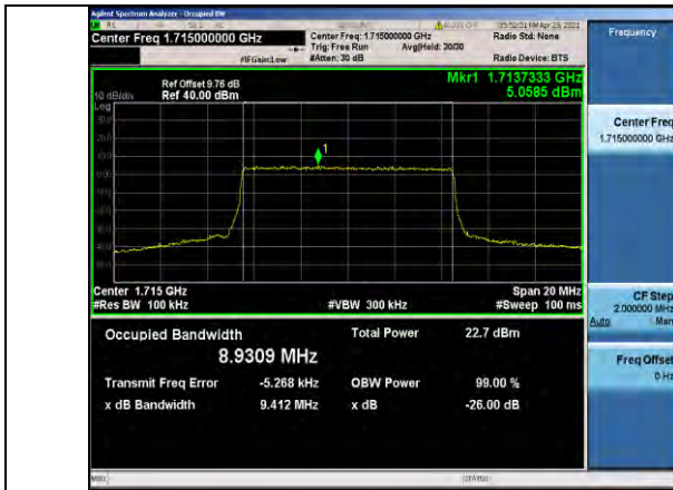
Band4-10MHz-QPSK-20000-50RB#0-8.9309
