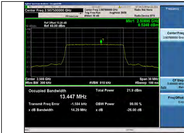
Band7-15MHz-QPSK-20825-75RB#0-13.447
