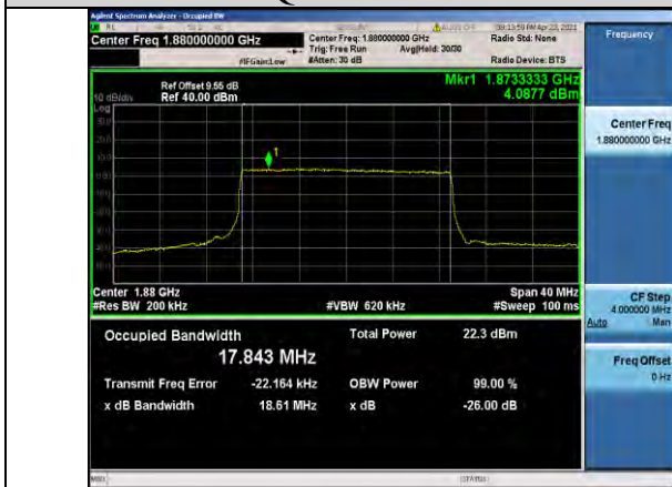
Band2-20MHz-QPSK-18900-100RB#0-17.843
