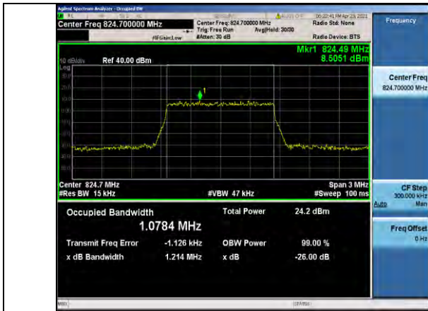
Band5-1.4MHz-QPSK-20407-6RB#0-1.0784
