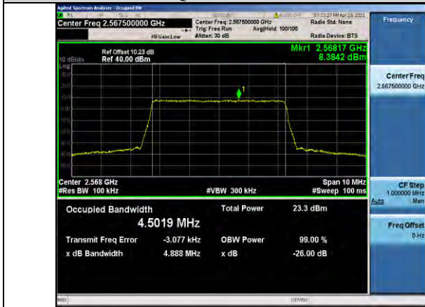
Band7-5MHz-QPSK-21425-25RB#0-4.5019
