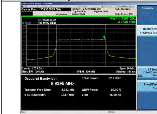
Band4-10MHz-QPSK-20175-50RB#0-8.9395
