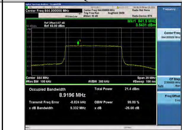
Band5-10MHz-16QAM-20600-50RB#0-8.9196
