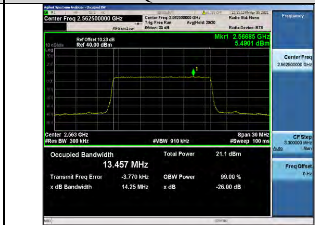
Band7-15MHz-16QAM-21375-75RB#0-13.457
