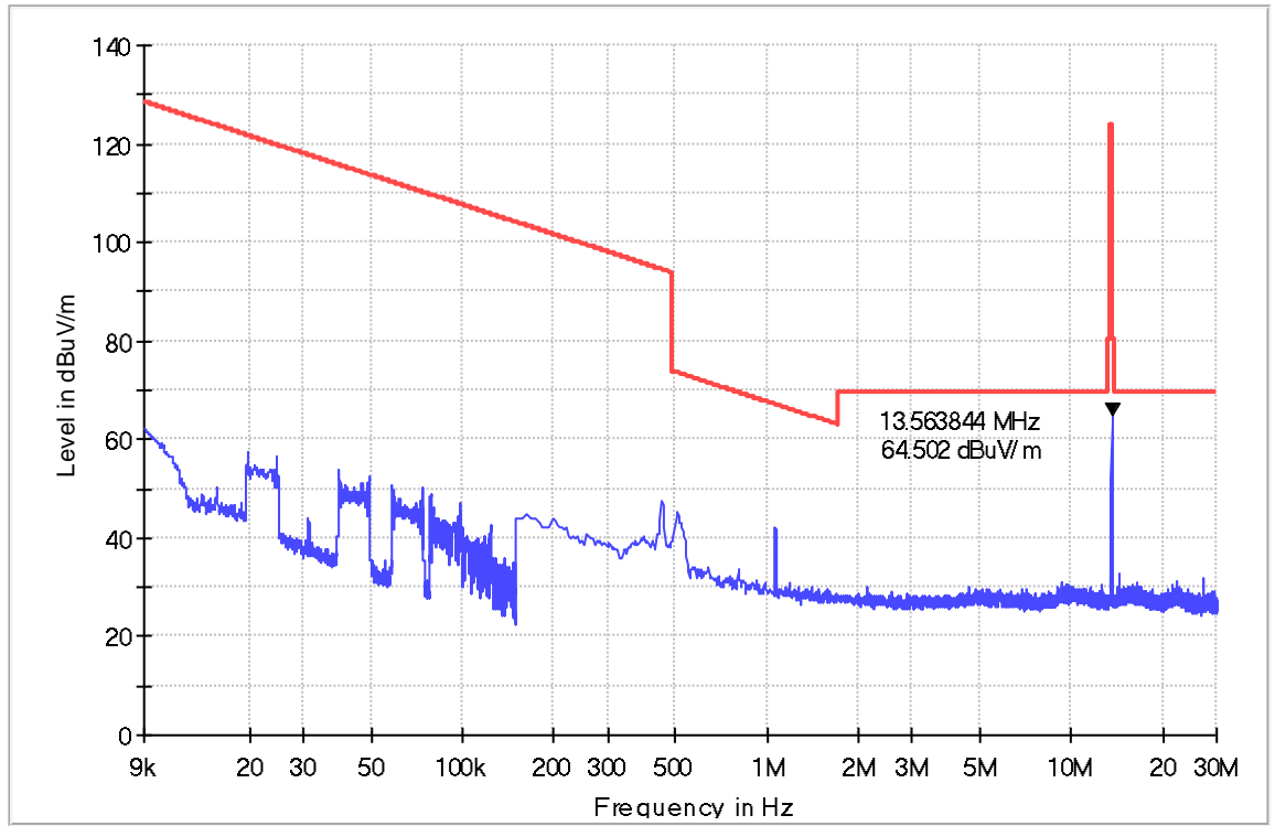
ESR26 Magnetic field dBuV-m
