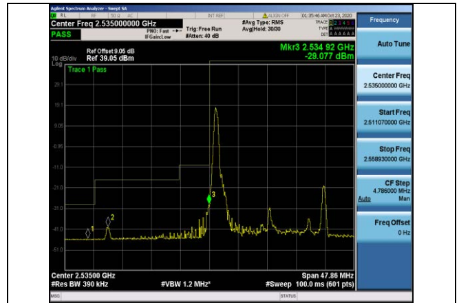
Band41-20MHz-16QAM-40140-1RB#0
