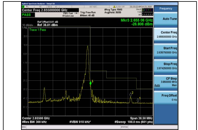
Band41-15MHz-16QAM-41165-1RB#74
