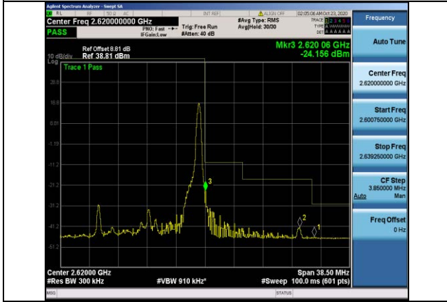
Band38-15MHz-16QAM-38175-1RB#74
