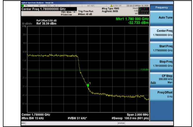
Band66-1.4MHz-QPSK-132665-6RB#0
