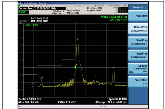
Band41-15MHz-QPSK-40115-1RB#0
