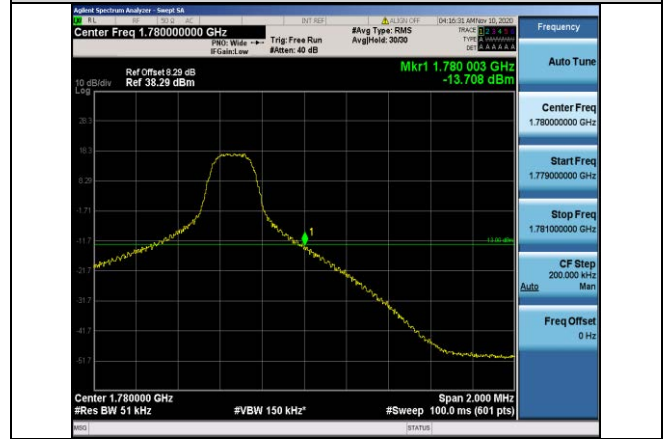
Band66-5MHz-16QAM-132647-1RB#24
