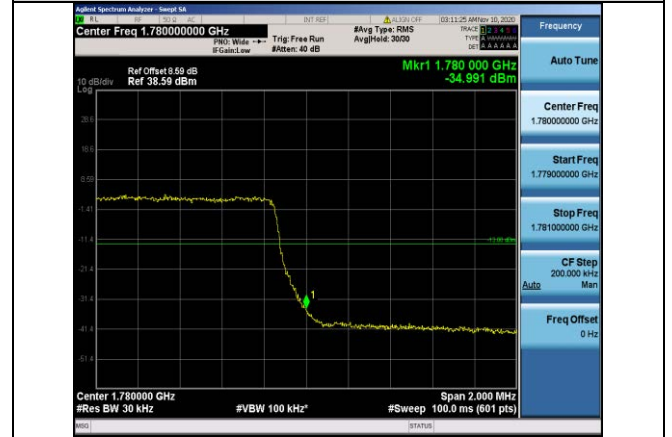
Band66-3MHz-16QAM-132657-15RB#0
