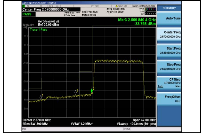
Band38-20MHz-QPSK-37850-100RB#0
