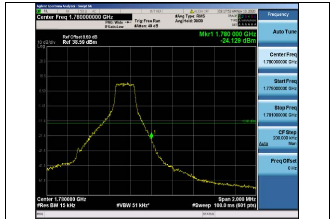
Band66-1.4MHz-QPSK-132665-1RB#5
