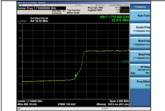
Band66-3MHz-16QAM-131987-15RB#0
