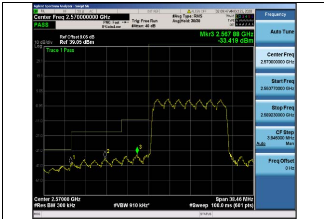
Band38-15MHz-16QAM-37825-75RB#0
