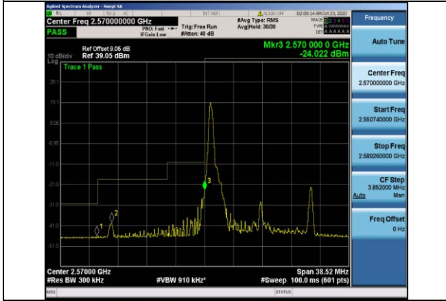
Band38-15MHz-QPSK-37825-1RB#0
