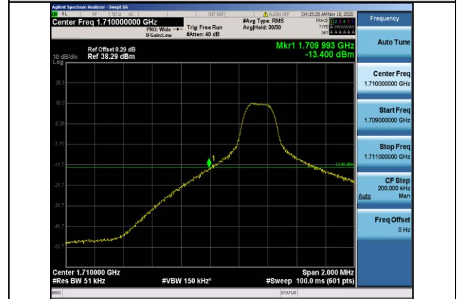
Band66-5MHz-QPSK-131997-1RB#0
