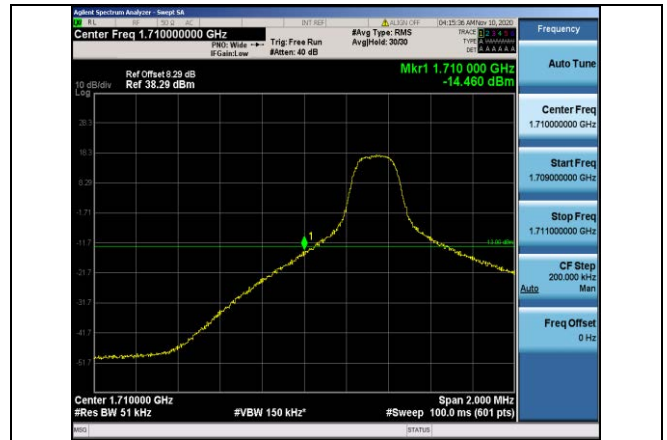
Band66-5MHz-16QAM-131997-1RB#0
