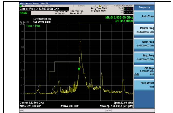
Band41-5MHz-16QAM-40065-1RB#0
