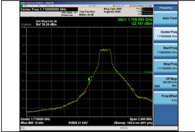
Band66-1.4MHz-QPSK-131979-1RB#0
