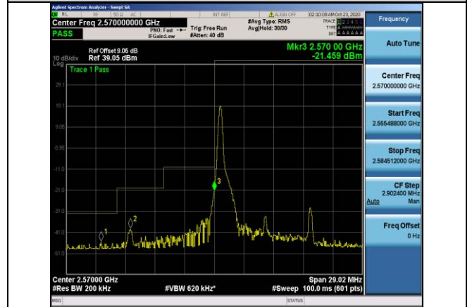
Band38-10MHz-QPSK-37800-1RB#0
