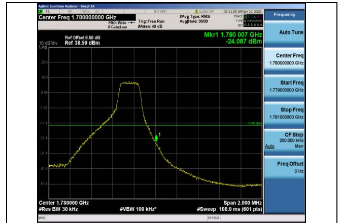
Band66-3MHz-16QAM-132657-1RB#14
