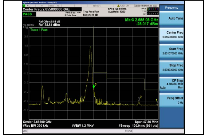
Band41-20MHz-16QAM-41140-1RB#99
