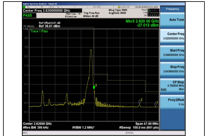
Band38-20MHz-16QAM-38150-1RB#99
