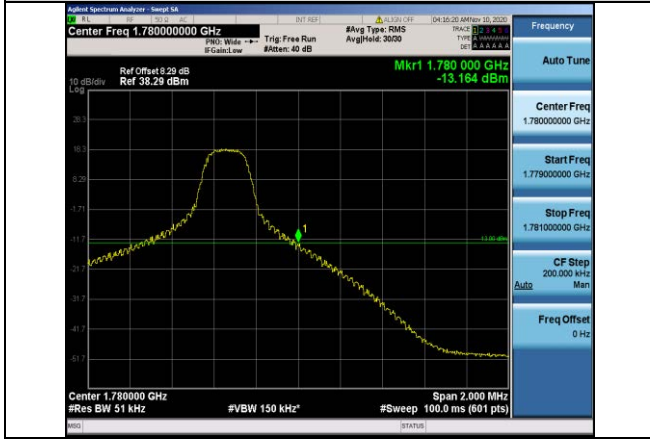
Band66-5MHz-QPSK-132647-1RB#24
