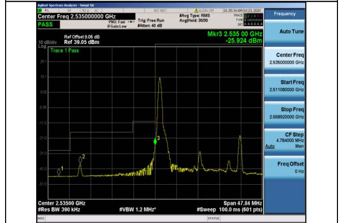
Band41-20MHz-QPSK-40140-1RB#0
