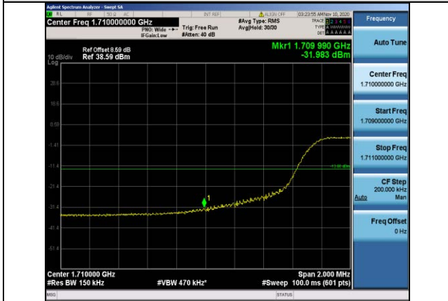
Band66-15MHz-16QAM-132047-75RB#0
