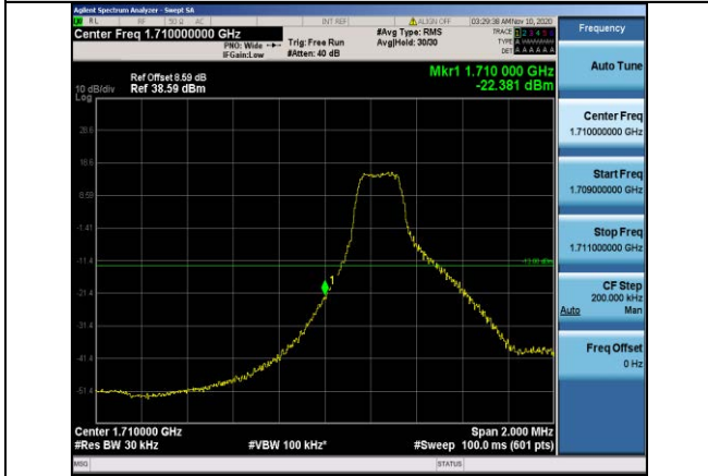
Band66-3MHz-16QAM-131987-1RB#0
