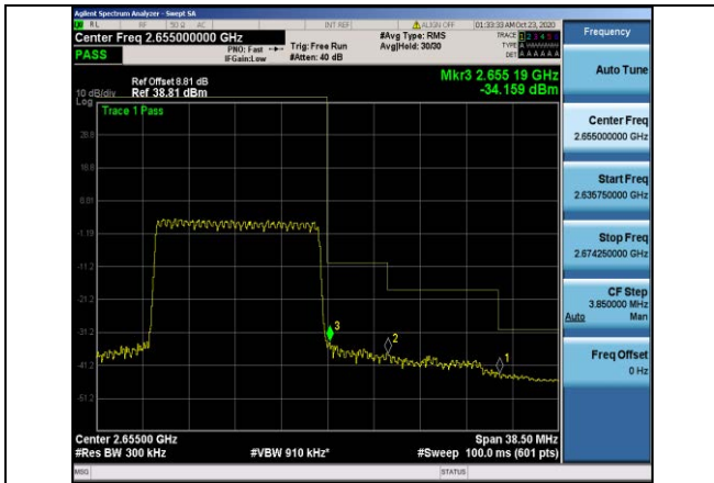
Band41-15MHz-QPSK-41165-75RB#0
