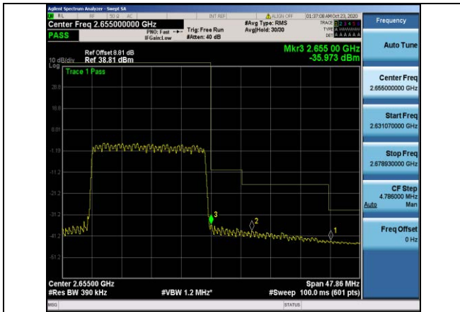
Band41-20MHz-16QAM-41140-100RB#0
