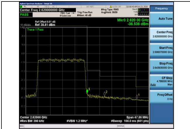
Band38-20MHz-QPSK-38150-100RB#0
