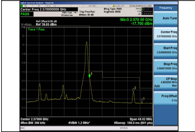
Band7-20MHz-QPSK-21350-1RB#99
