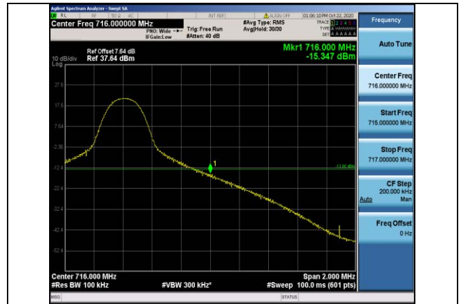
Band12-10MHz-QPSK-23130-1RB#49
