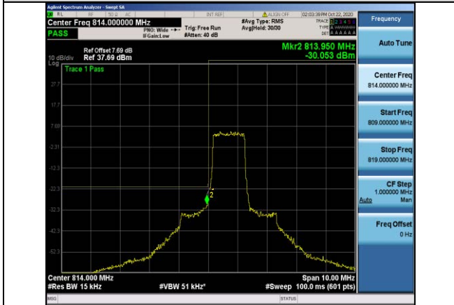
Band26-1.4MHz-QPSK-26697-6RB#0
