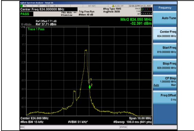
Band26-1.4MHz-16QAM-26783-1RB#5
