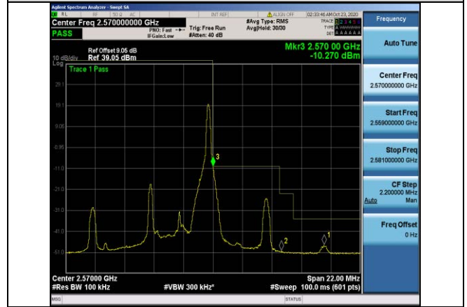
Band7-5MHz-16QAM-21425-1RB#24
