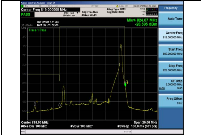
Band26-10MHz-16QAM-26740 Right-1RB#49
