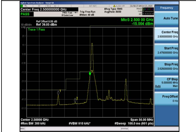
Band7-15MHz-16QAM-20825-1RB#0
