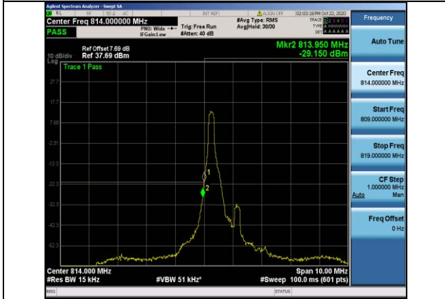
Band26-1.4MHz-QPSK-26697-1RB#0
