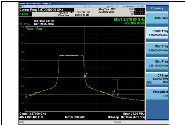
Band7-5MHz-16QAM-21425-25RB#0
