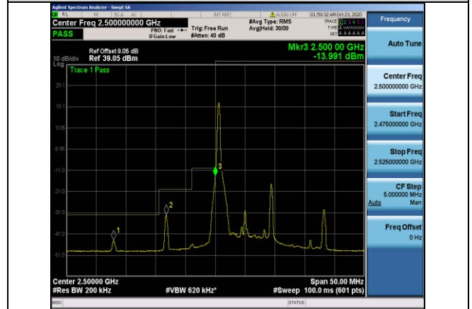
Band7-10MHz-16QAM-20800-1RB#0
