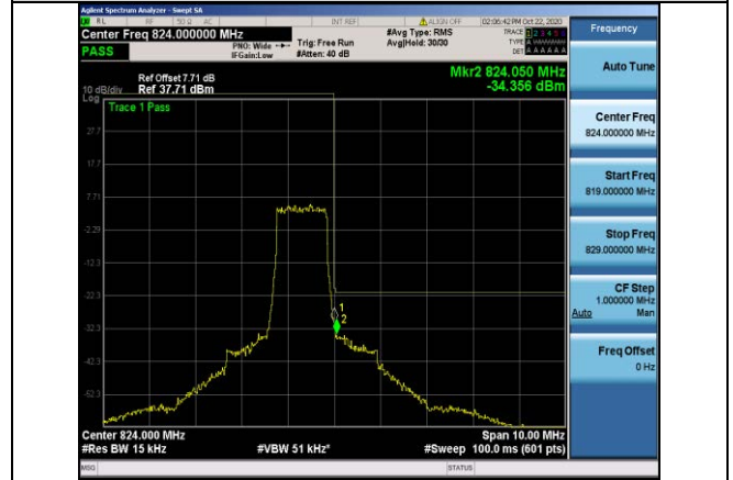
Band26-1.4MHz-QPSK-26783-6RB#0
