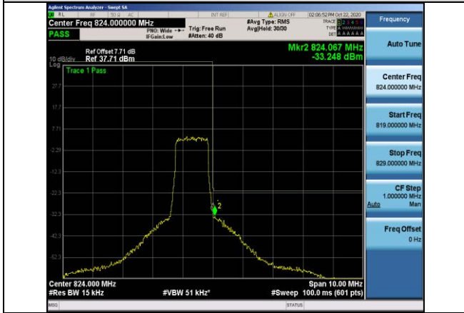
Band26-1.4MHz-16QAM-26783-6RB#0
