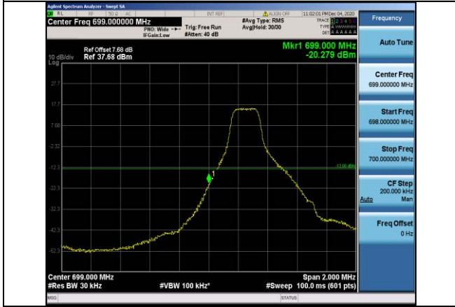
Band12-1.4MHz-QPSK-23017-1RB#0
