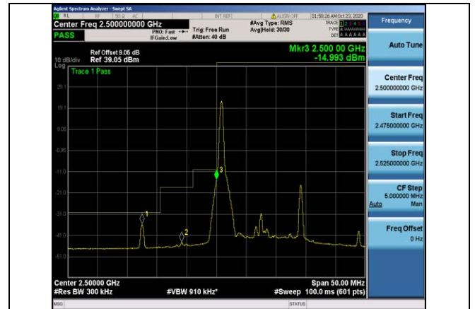
Band7-15MHz-QPSK-20825-1RB#0
