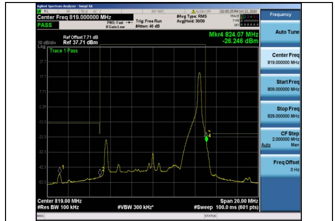
Band26-10MHz-QPSK-26740_Right-1RB#49
