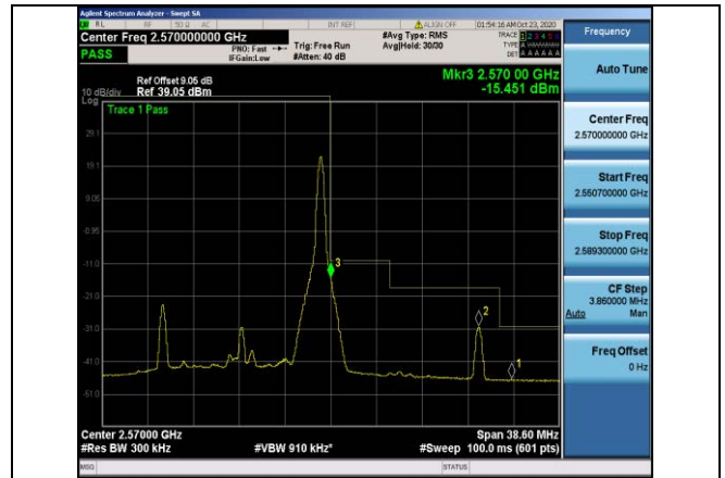
Band7-15MHz-16QAM-21375-1RB#74
