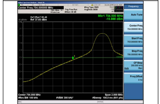
Band17-10MHz-QPSK-23780-1RB#0
