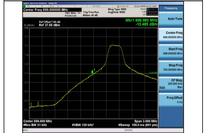
Band12-5MHz-QPSK-23035-1RB#0
