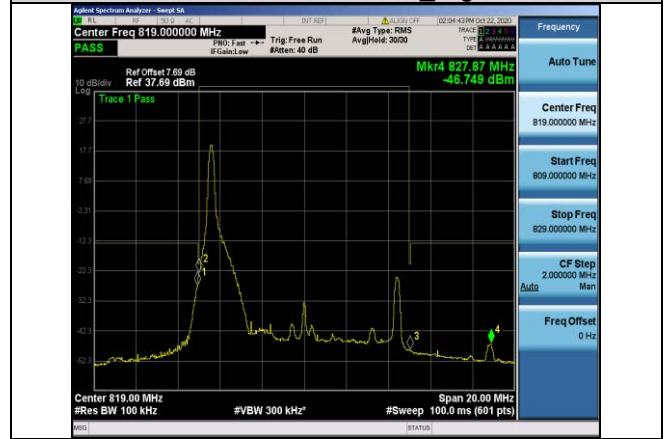
Band26-10MHz-16QAM-26740_Left-1RB#0
