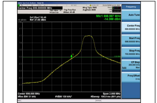
Band12-5MHz-16QAM-23035-1RB#0
