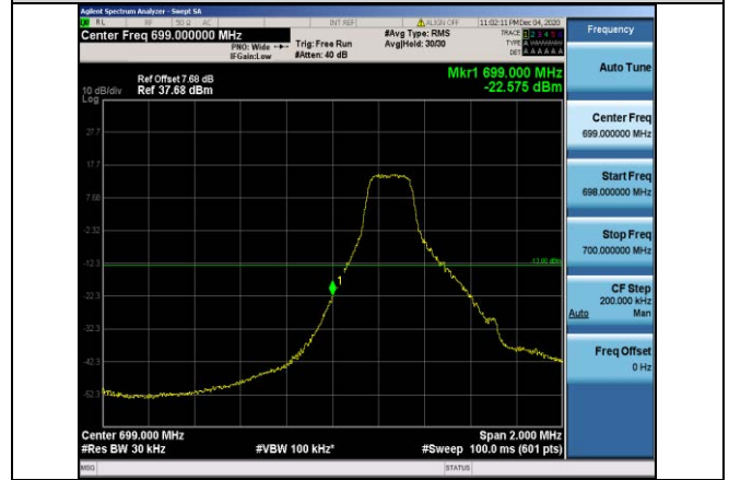
Band12-1.4MHz-16QAM-23017-1RB#0
