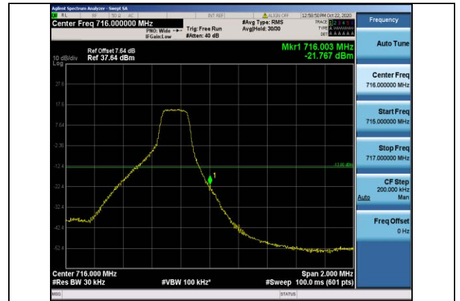
Band12-3MHz-16QAM-23165-1RB#14
