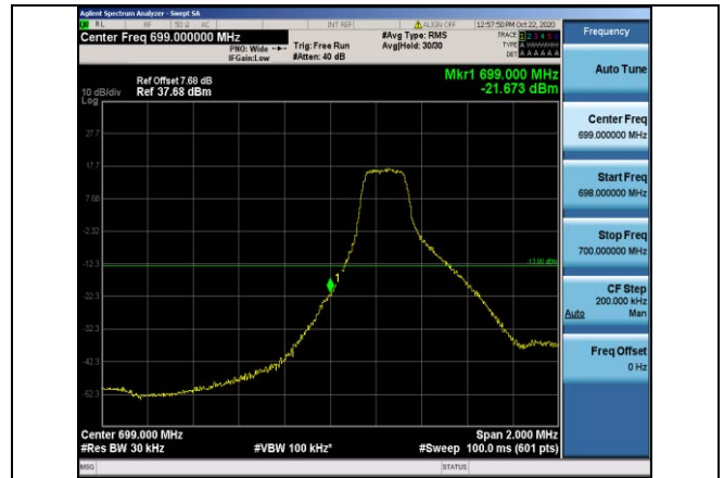
Band12-3MHz-QPSK-23025-1RB#0
