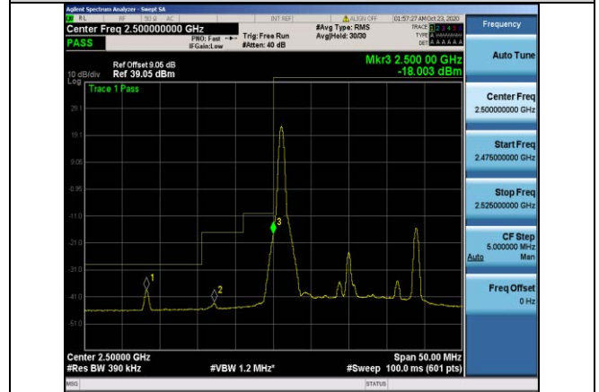
Band7-20MHz-QPSK-20850-1RB#0
