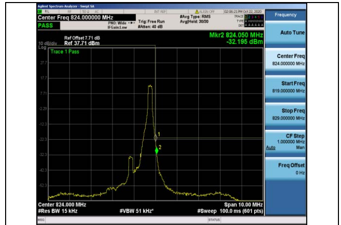
Band26-1.4MHz-QPSK-26783-1RB#5
