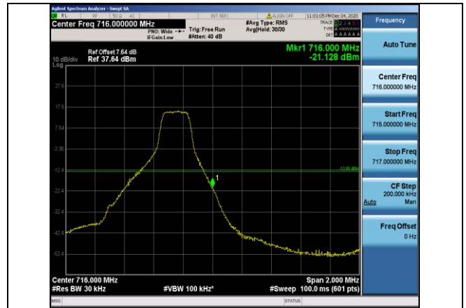
Band12-1.4MHz-QPSK-23173-1RB#5
