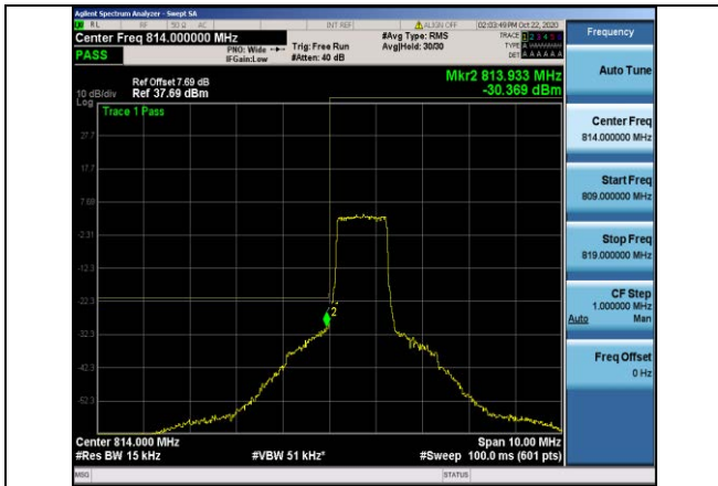
Band26-1.4MHz-16QAM-26697-6RB#0
