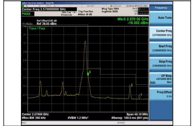
Band7-20MHz-16QAM-21350-1RB#99
