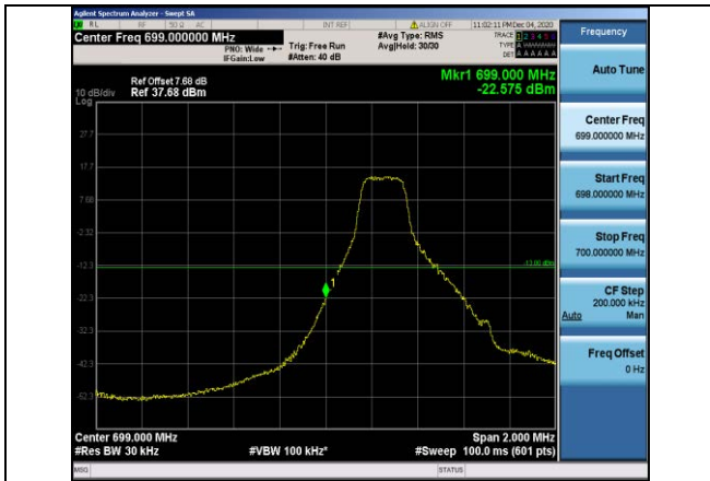
Band12-1.4MHz-16QAM-23017-6RB#0
