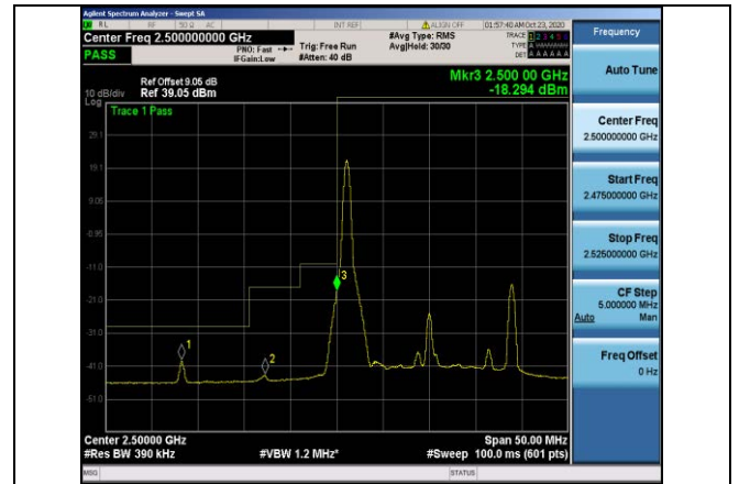
Band7-20MHz-16QAM-20850-1RB#0
