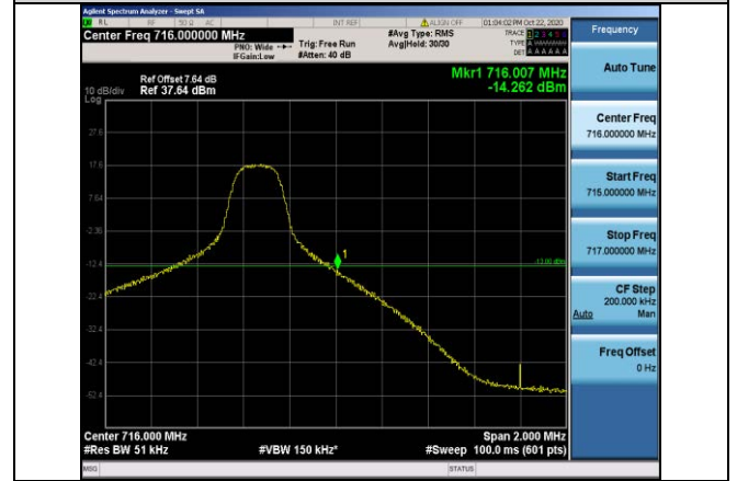
Band12-5MHz-16QAM-23155-1RB#24
