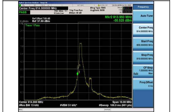
Band26-1.4MHz-16QAM-26697-1RB#0
