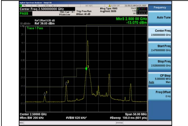
Band7-10MHz-QPSK-20800-1RB#0
