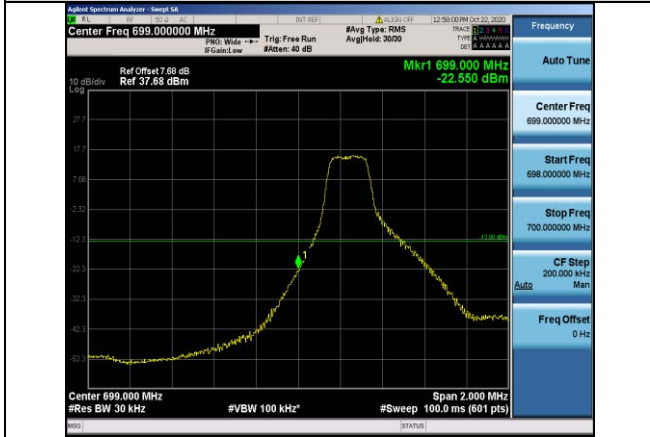
Band12-3MHz-16QAM-23025-1RB#0
