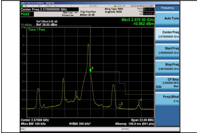
Band7-5MHz-QPSK-21425-1RB#24
