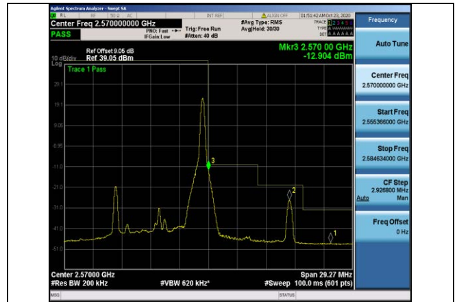
Band7-10MHz-QPSK-21400-1RB#49
