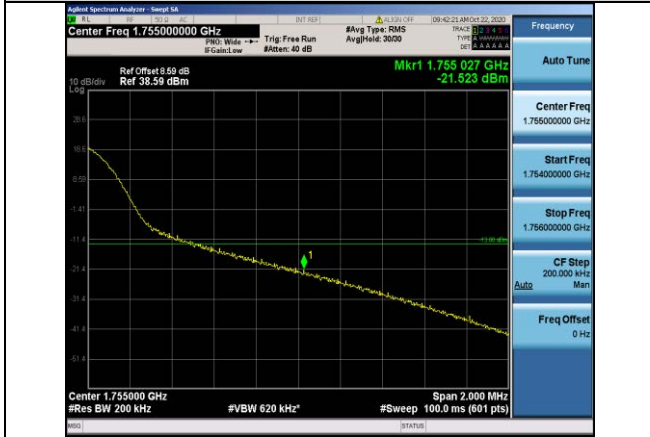
Band4-20MHz-16QAM-20300-1RB#99
