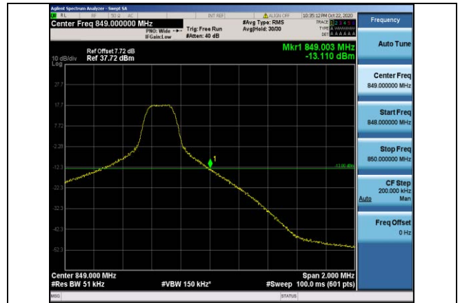
Band5-5MHz-QPSK-20625-1RB#24
