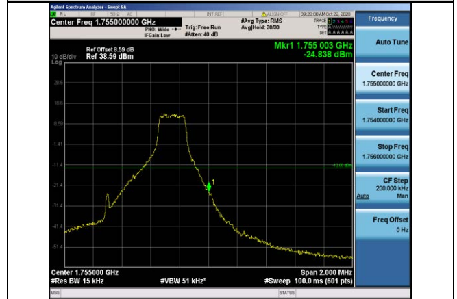
Band4-1.4MHz-QPSK-20393-1RB#5
