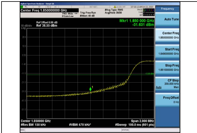
Band2-15MHz-QPSK-18675-75RB#0
