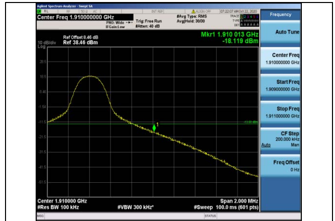
Band2-10MHz-16QAM-19150-1RB#49
