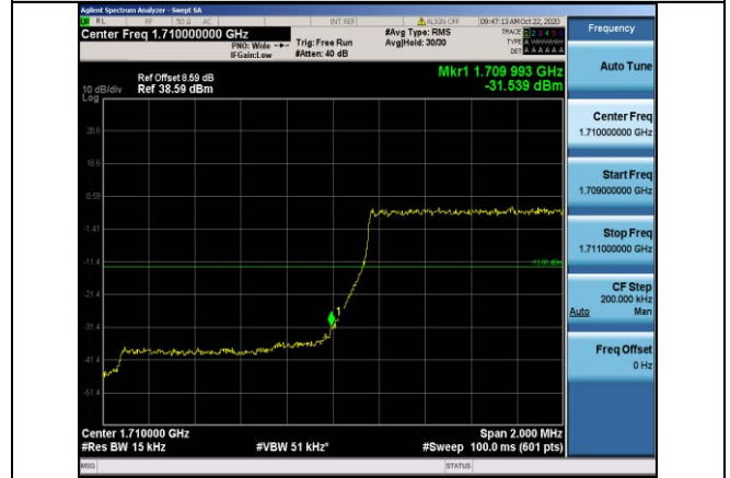
Band4-1.4MHz-QPSK-19957-6RB#0
