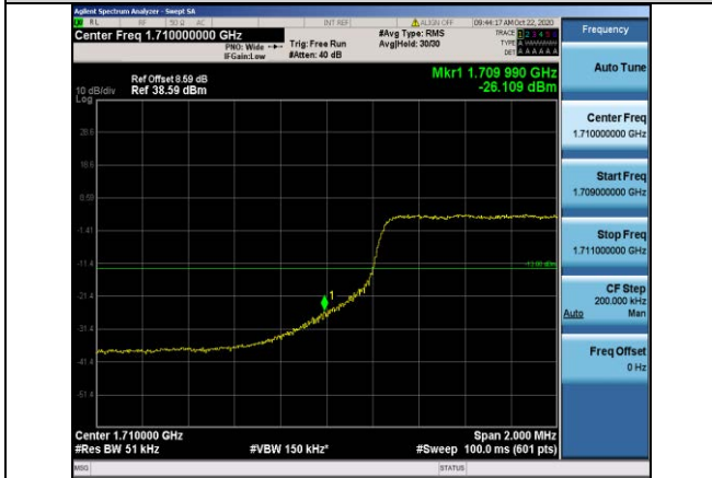
Band4-5MHz-QPSK-19975-25RB#0
