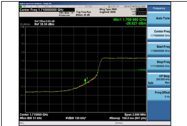
Band4-5MHz-16QAM-19975-25RB#0
