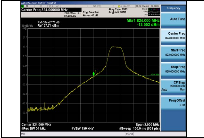
Band5-5MHz-QPSK-20425-1RB#0
