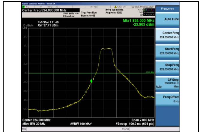
Band5-3MHz-16QAM-20415-1RB#0
