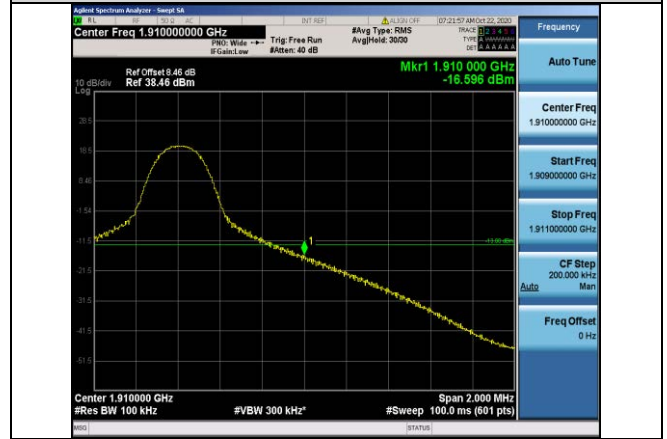
Band2-10MHz-QPSK-19150-1RB#49
