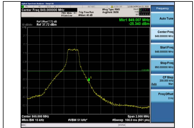
Band5-1.4MHz-16QAM-20643-1RB#5
