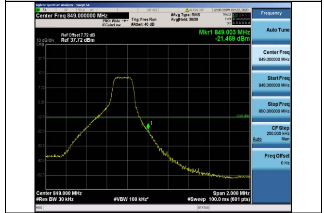
Band5-3MHz-16QAM-20635-1RB#14
