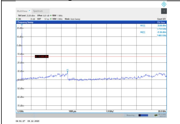
Band66-15MHz-QPSK-132047-1RB#0-Range2:1000~20000MHz
