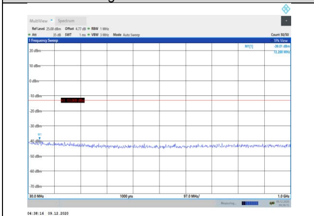
Band66-3MHz-16QAM-132322-1RB#0- Range1:30~1000MHz
