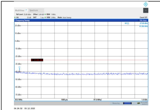
Band41-15MHz-16QAM-40740-1RB#0- Range1:30~1000MHz
