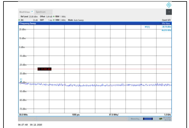
Band41-20MHz-16QAM-40340-1RB#0- Range1:30~1000MHz
