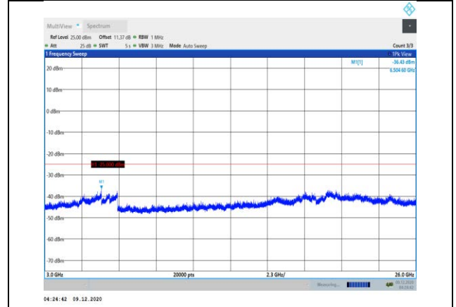
Band41-15MHz-QPSK-40740-1RB#0- Range3:3000~26000MHz
