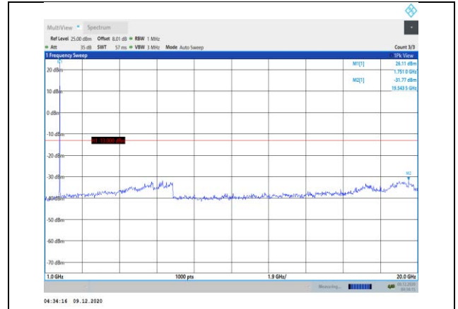
Band66-1.4MHz-QPSK-132322-1RB#0-Range2:1000~20000MHz
