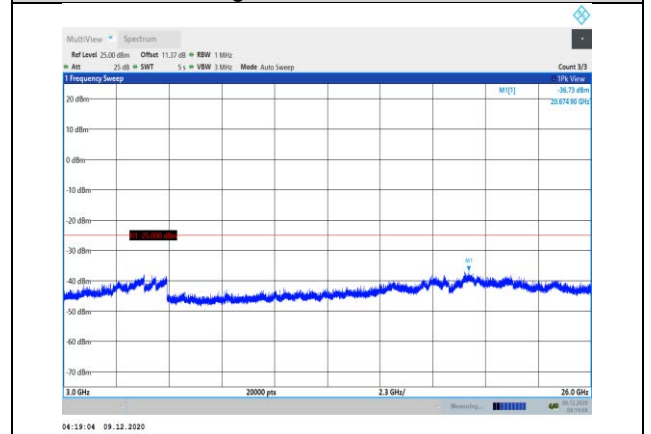
Band41-10MHz-16QAM-40290-1RB#0- Range3:3000~26000MHz
