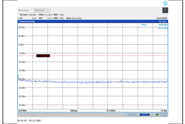
Band66-15MHz-16QAM-132597-1RB#0- Range1:30~1000MHz
