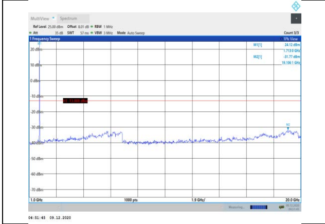
Band66-15MHz-16QAM-132047-1RB#0- Range2:1000~20000MHz
