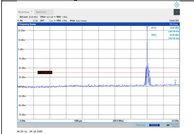
Band41-10MHz-16QAM-40740-1RB#0- Range2:1000~3000MHz
