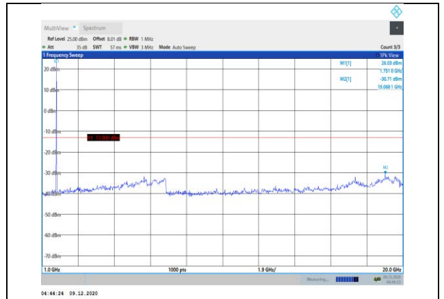
Band66-5MHz-QPSK-132322-1RB#0- Range2:1000~20000MHz
