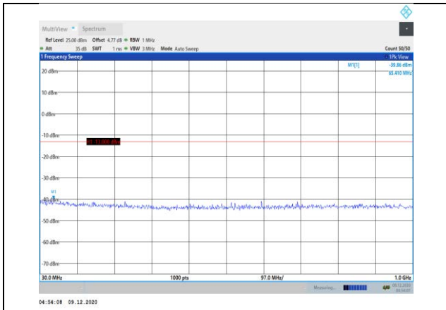
Band66-20MHz-16QAM-132072-1RB#0- Range1:30~1000MHz
