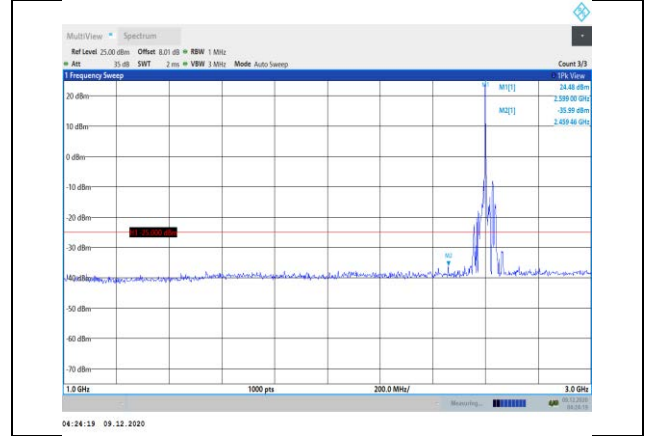
Band41-15MHz-QPSK-40740-1RB#0- Range2:1000~3000MHz
