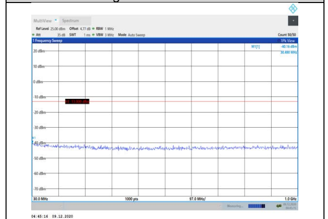
Band66-5MHz-16QAM-132647-1RB#0- Range1:30~1000MHz
