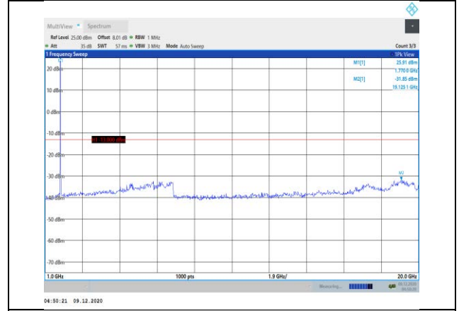
Band66-10MHz-16QAM-132622-1RB#0- Range2:1000~20000MHz
