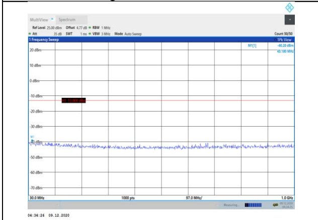
Band66-1.4MHz-16QAM-132322-1RB#0- Range1:30~1000MHz
