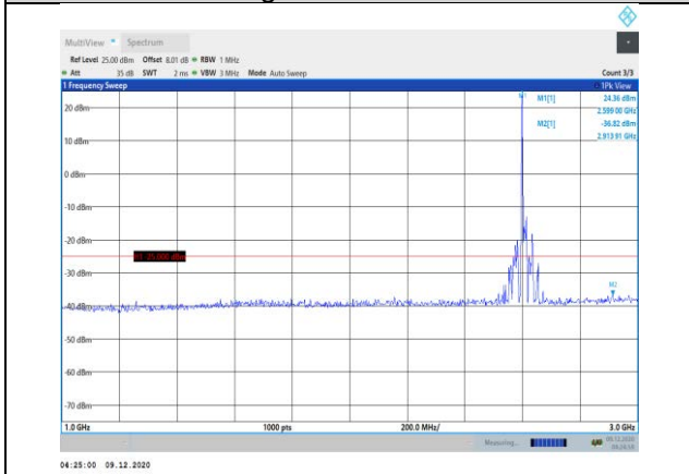
Band41-15MHz-16QAM-40740-1RB#0- Range2:1000~3000MHz
