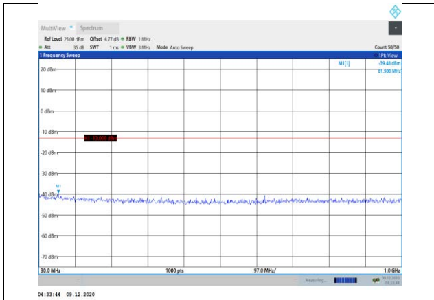
Band66-1.4MHz-16QAM-131979-1RB#0- Range1:30~1000MHz
