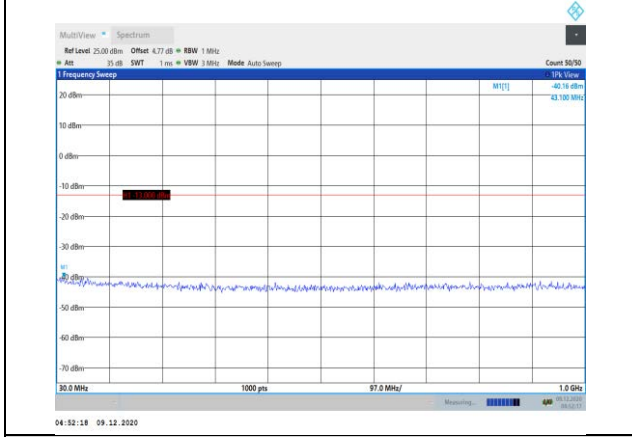
Band66-15MHz-16QAM-132322-1RB#0- Range1:30~1000MHz
