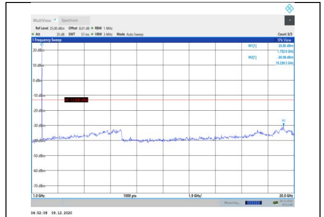
Band66-15MHz-QPSK-132322-1RB#0-Range2:1000~20000MHz
