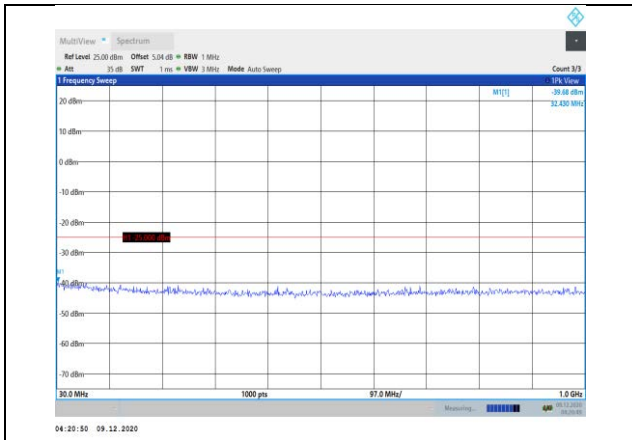
Band41-10MHz-QPSK-41190-1RB#0- Range1:30~1000MHz
