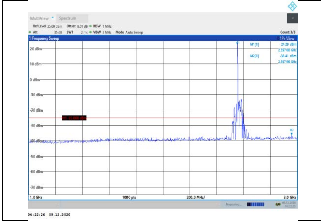
Band41-15MHz-QPSK-40315-1RB#0- Range2:1000~3000MHz
