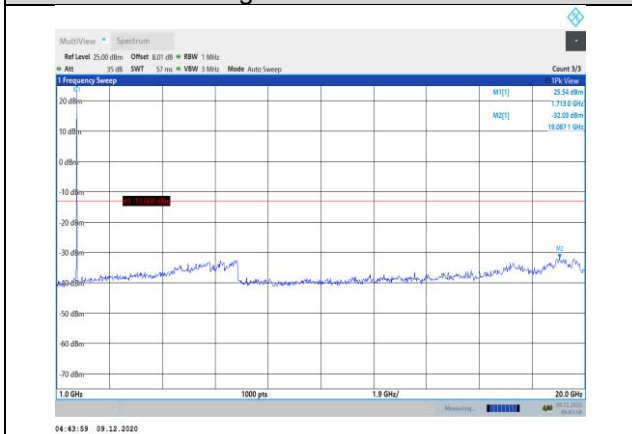
Band66-5MHz-16QAM-131997-1RB#0- Range2:1000~20000MHz
