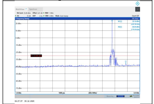
Band41-20MHz-16QAM-40340-1RB#0- Range2:1000~3000MHz
