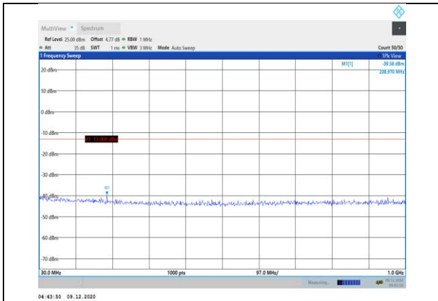
Band66-5MHz-16QAM-131997-1RB#0- Range1:30~1000MHz
