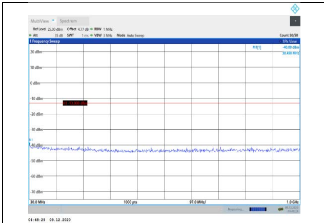
Band66-10MHz-QPSK-132022-1RB#0- Range1:30~1000MHz
