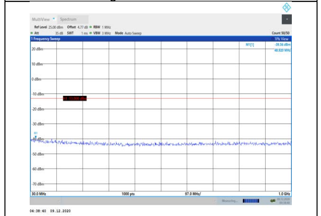
Band66-3MHz-QPSK-132657-1RB#0- Range1:30~1000MHz
