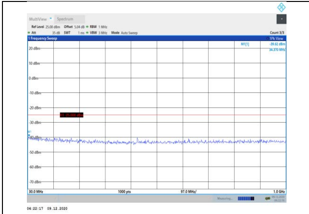
Band41-15MHz-QPSK-40315-1RB#0- Range1:30~1000MHz
