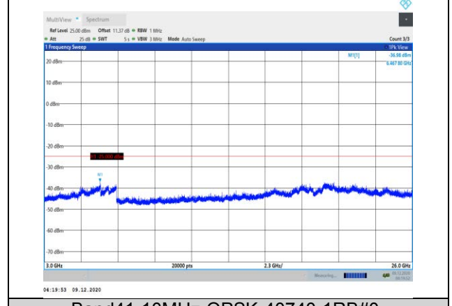
Band41-10MHz-QPSK-40740-1RB#0- Range3:3000~26000MHz
