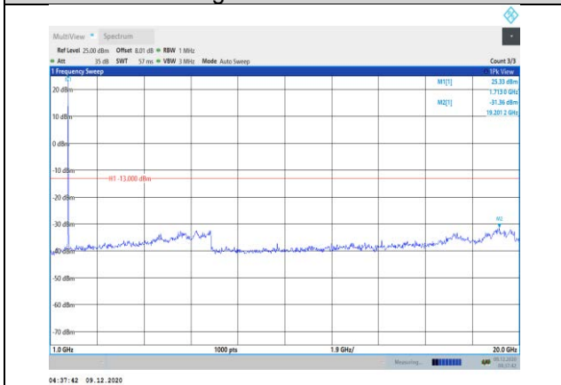
Band66-3MHz-16QAM-131987-1RB#0- Range2:1000~20000MHz
