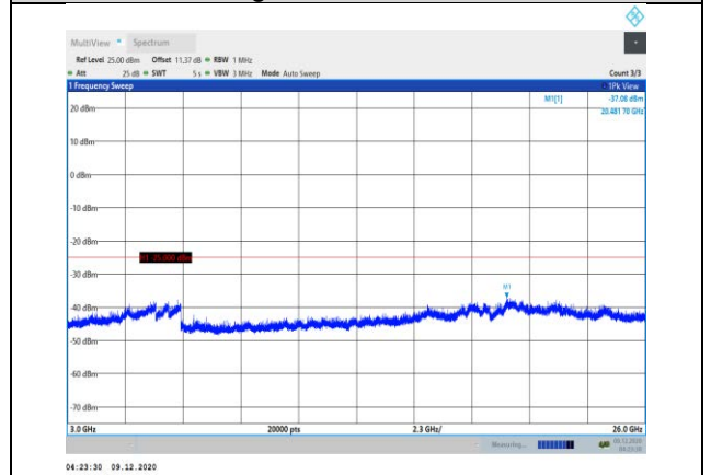
Band41-15MHz-16QAM-40315-1RB#0- Range3:3000~26000MHz
