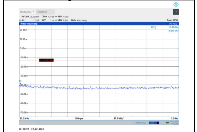
Band66-1.4MHz-16QAM-132665-1RB#0- Range1:30~1000MHz
