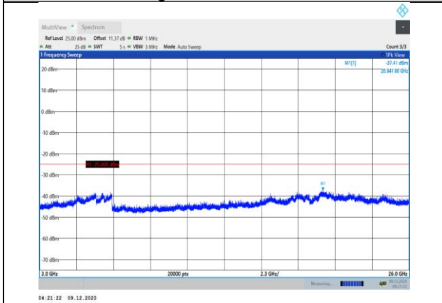
Band41-10MHz-QPSK-41190-1RB#0- Range3:3000~26000MHz
