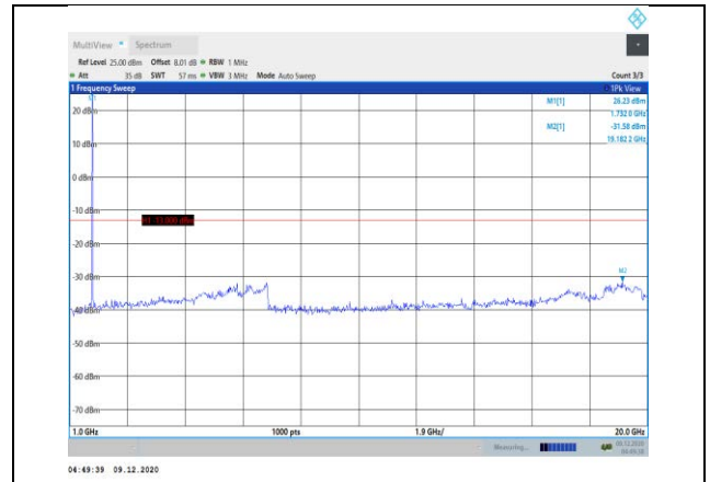
Band66-10MHz-16QAM-132322-1RB#0- Range2:1000~20000MHz
