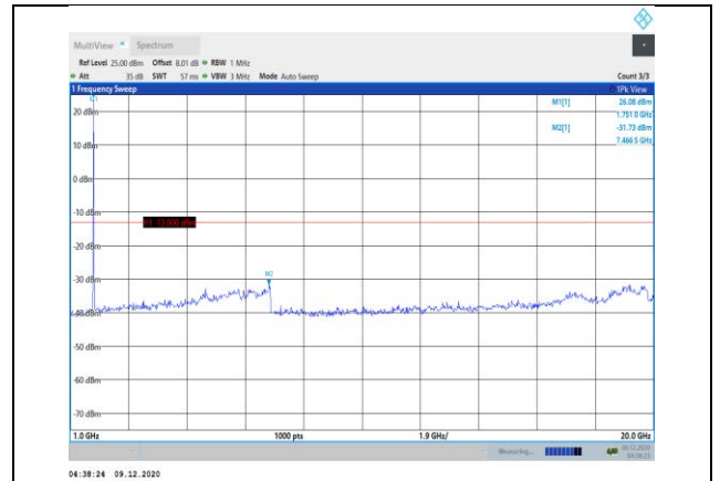
Band66-3MHz-16QAM-132322-1RB#0- Range2:1000~20000MHz
