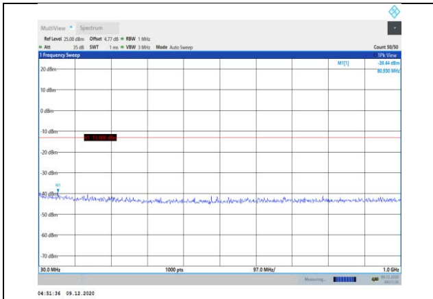
Band66-15MHz-16QAM-132047-1RB#0- Range1:30~1000MHz
