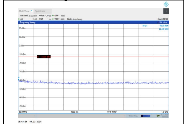
Band66-10MHz-QPSK-132622-1RB#0- Range1:30~1000MHz
