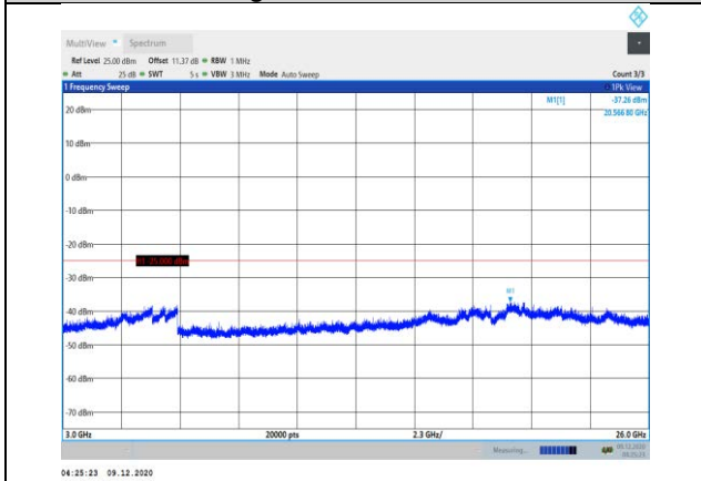
Band41-15MHz-16QAM-40740-1RB#0- Range3:3000~26000MHz
