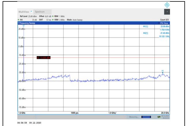
Band66-20MHz-16QAM-132322-1RB#0- Range2:1000~20000MHz
