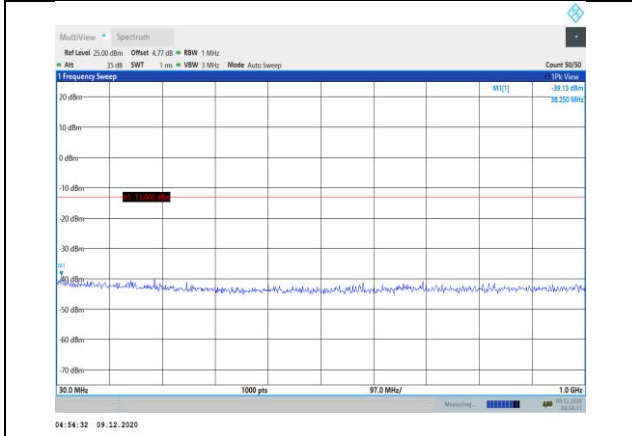
Band66-20MHz-QPSK-132322-1RB#0- Range1:30~1000MHz
