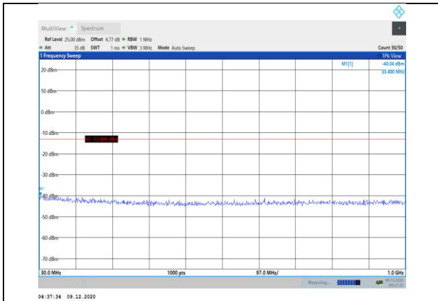
Band66-3MHz-16QAM-131987-1RB#0- Range1:30~1000MHz
