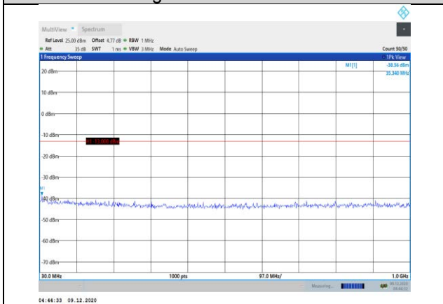
Band66-5MHz-16QAM-132322-1RB#0- Range1:30~1000MHz
