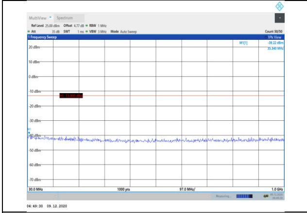
Band66-10MHz-16QAM-132322-1RB#0- Range1:30~1000MHz
