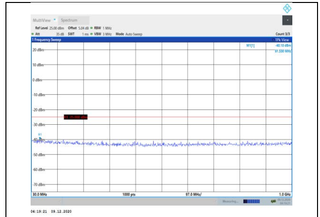
Band41-10MHz-QPSK-40740-1RB#0- Range1:30~1000MHz
