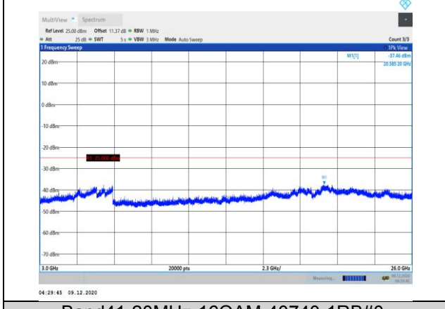
Band41-20MHz-16QAM-40740-1RB#0-Range3:3000~26000MHz
