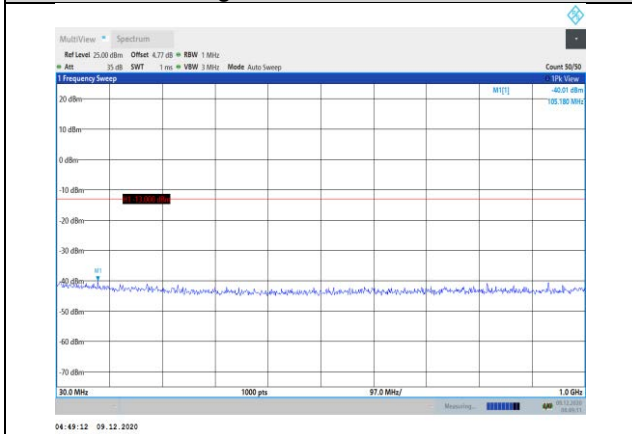
Band66-10MHz-QPSK-132322-1RB#0- Range1:30~1000MHz
