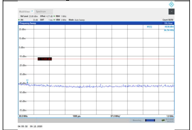
Band66-20MHz-16QAM-132572-1RB#0- Range1:30~1000MHz
