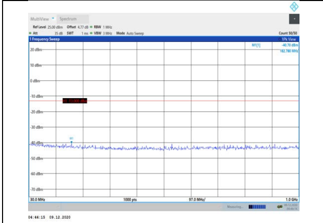
Band66-5MHz-QPSK-132322-1RB#0- Range1:30~1000MHz
