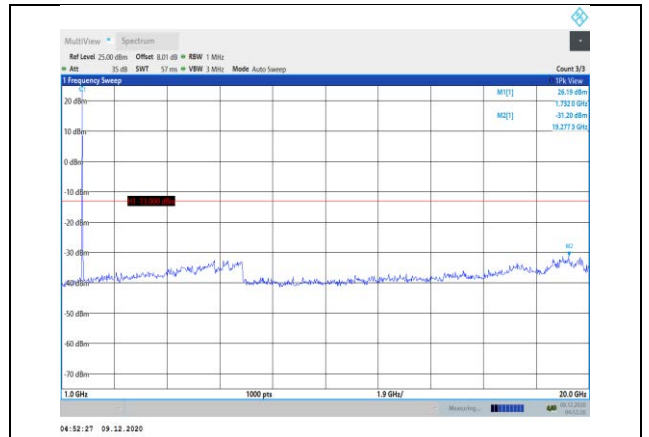
Band66-15MHz-16QAM-132322-1RB#0- Range2:1000~20000MHz
