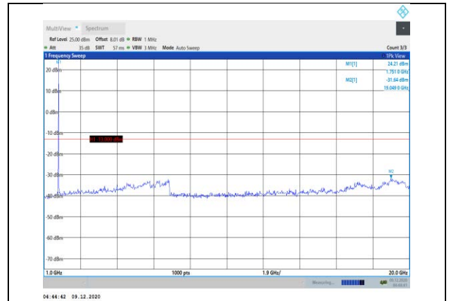
Band66-5MHz-16QAM-132322-1RB#0- Range2:1000~20000MHz
