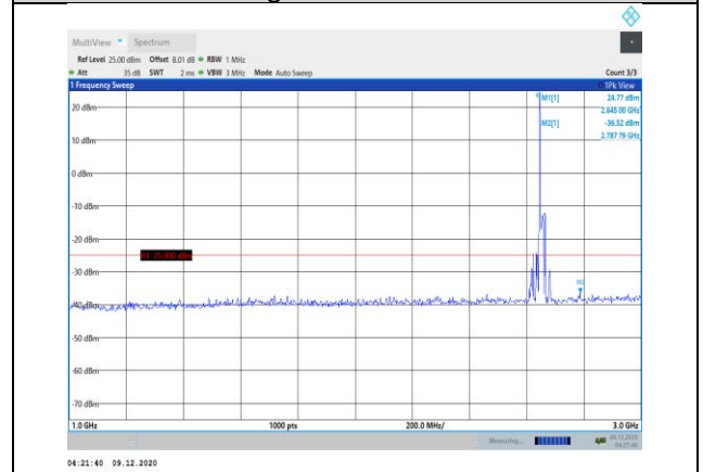
Band41-10MHz-16QAM-41190-1RB#0- Range2:1000~3000MHz
