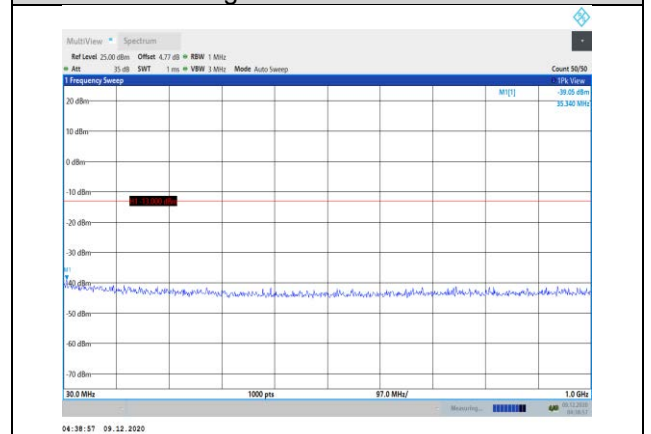
Band66-3MHz-16QAM-132657-1RB#0- Range1:30~1000MHz
