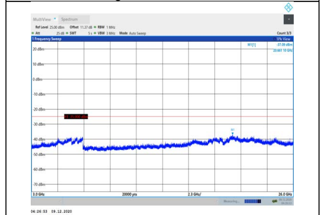
Band41-15MHz-16QAM-41165-1RB#0- Range3:3000~26000MHz
