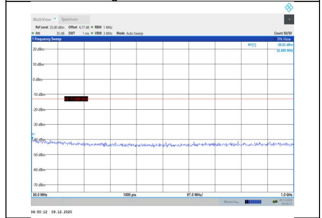
Band66-10MHz-16QAM-132622-1RB#0- Range1:30~1000MHz
