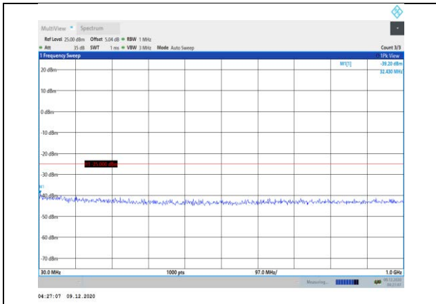
Band41-20MHz-QPSK-40340-1RB#0- Range1:30~1000MHz
