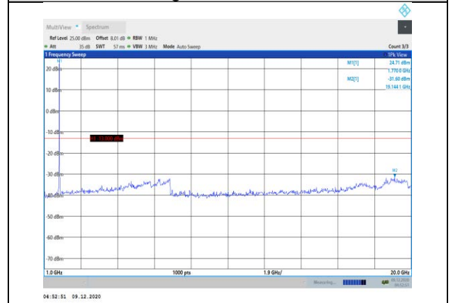
Band66-15MHz-QPSK-132597-1RB#0-Range2:1000~20000MHz
