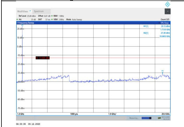
Band66-1.4MHz-QPSK-131979-1RB#0-Range2:1000~20000MHz
