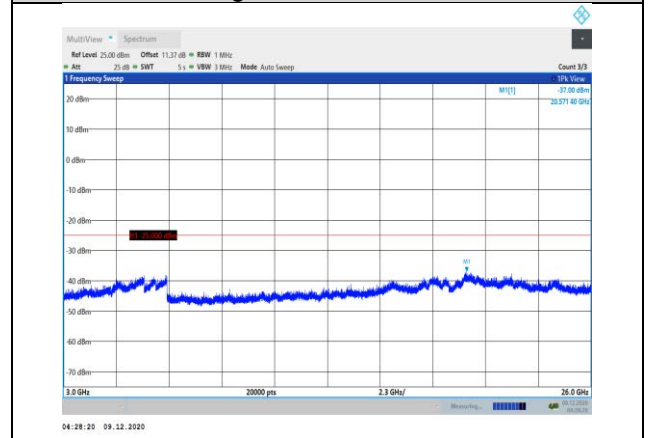
Band41-20MHz-16QAM-40340-1RB#0- Range3:3000~26000MHz
