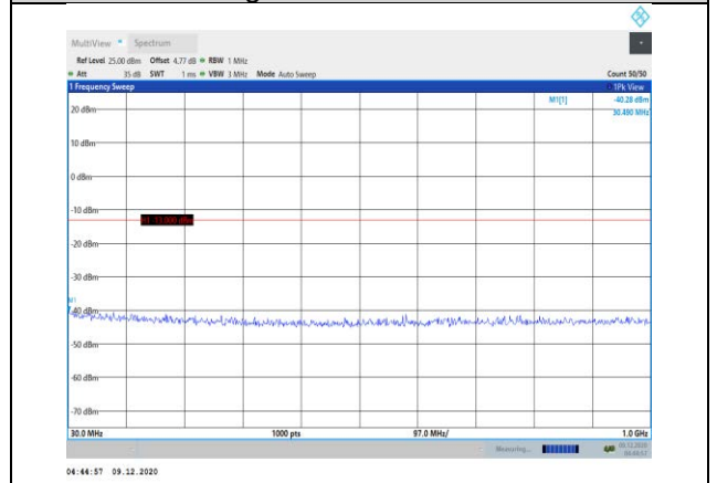
Band66-5MHz-QPSK-132647-1RB#0- Range1:30~1000MHz
