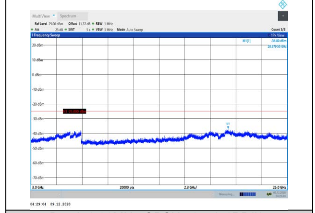
Band41-20MHz-QPSK-40740-1RB#0- Range3:3000~26000MHz
