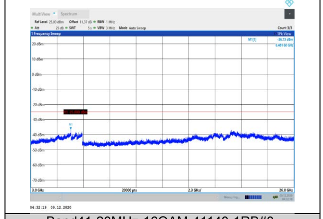
Band41-20MHz-16QAM-41140-1RB#0-Range3:3000~26000MHz
