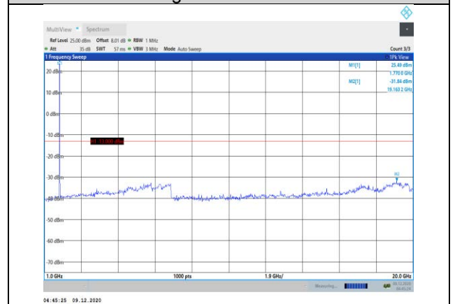
Band66-5MHz-16QAM-132647-1RB#0- Range2:1000~20000MHz
