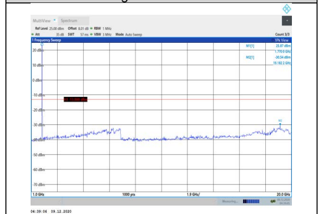
Band66-3MHz-16QAM-132657-1RB#0- Range2:1000~20000MHz
