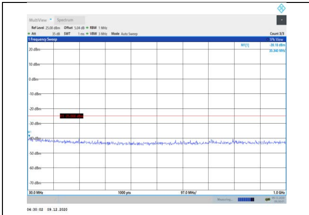
Band41-20MHz-QPSK-41140-1RB#0- Range1:30~1000MHz
