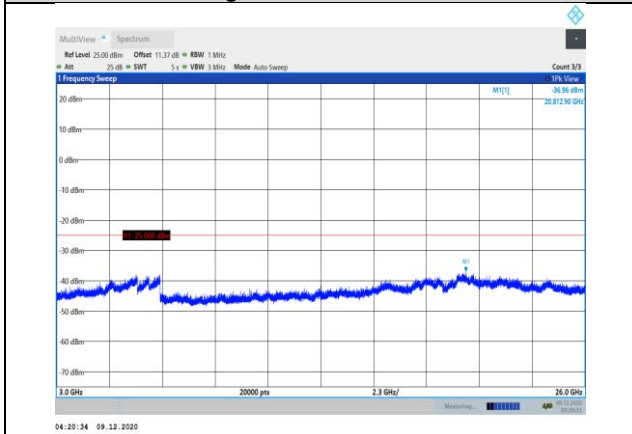
Band41-10MHz-16QAM-40740-1RB#0- Range3:3000~26000MHz
