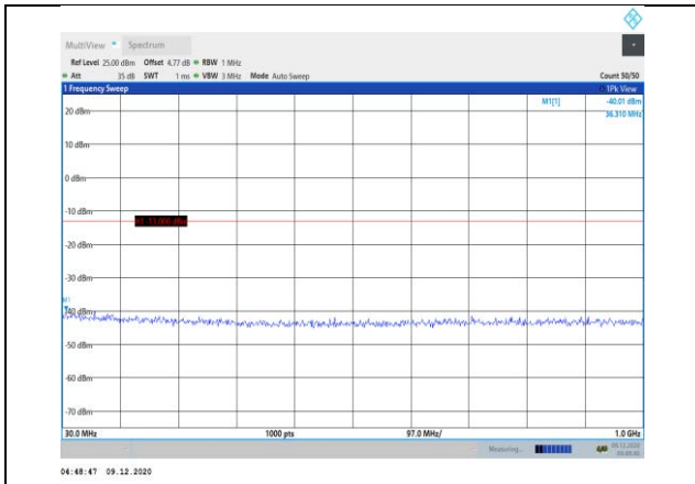
Band66-10MHz-16QAM-132022-1RB#0- Range1:30~1000MHz
