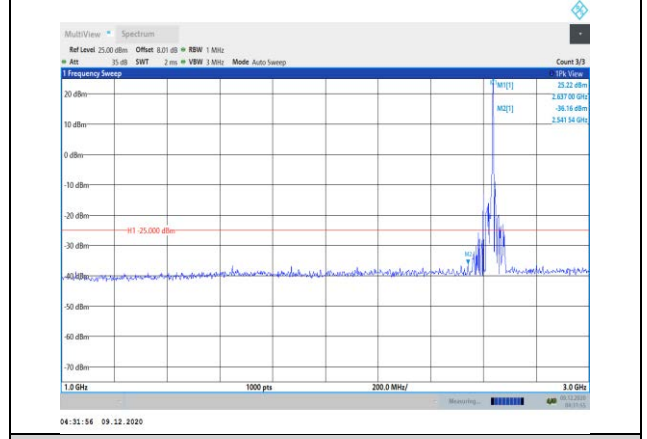
Band41-20MHz-16QAM-41140-1RB#0-Range2:1000~3000MHz
