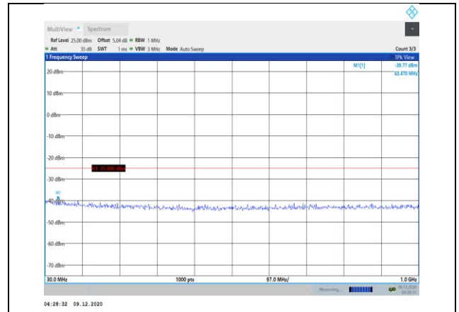
Band41-20MHz-QPSK-40740-1RB#0- Range1:30~1000MHz
