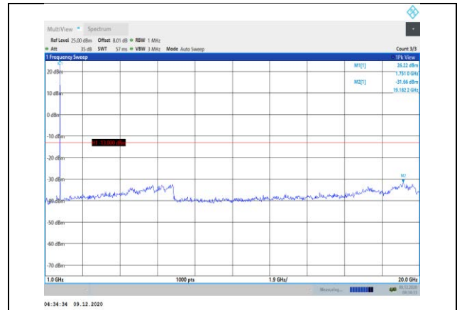
Band66-1.4MHz-16QAM-132322-1RB#0- Range2:1000~20000MHz
