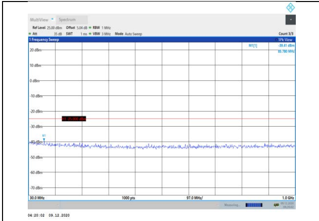
Band41-10MHz-16QAM-40740-1RB#0- Range1:30~1000MHz
