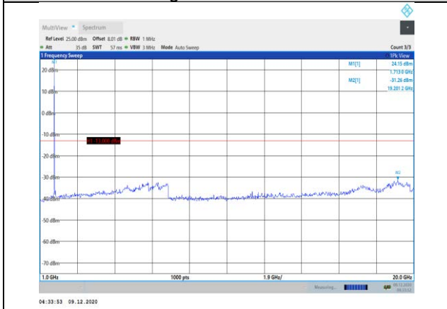
Band66-1.4MHz-16QAM-131979-1RB#0- Range2:1000~20000MHz
