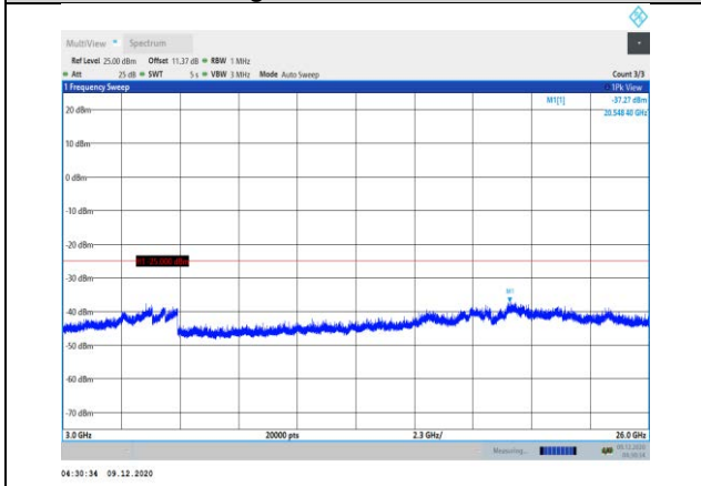
Band41-20MHz-QPSK-41140-1RB#0- Range3:3000~26000MHz
