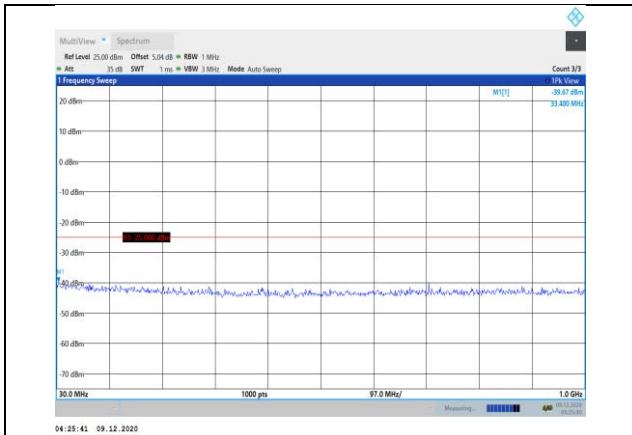
Band41-15MHz-QPSK-41165-1RB#0- Range1:30~1000MHz
