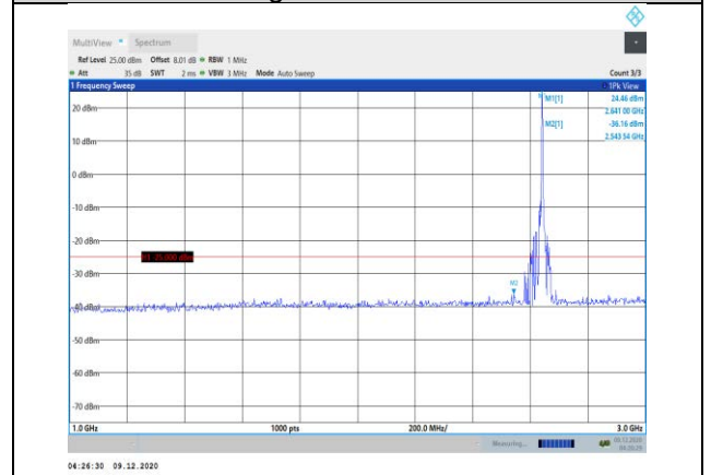
Band41-15MHz-16QAM-41165-1RB#0- Range2:1000~3000MHz
