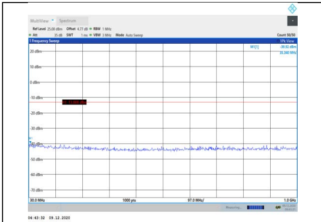
Band66-5MHz-QPSK-131997-1RB#0- Range1:30~1000MHz
