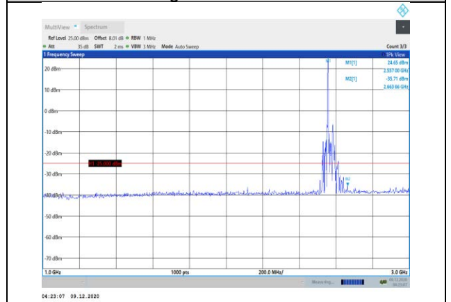
Band41-15MHz-16QAM-40315-1RB#0- Range2:1000~3000MHz
