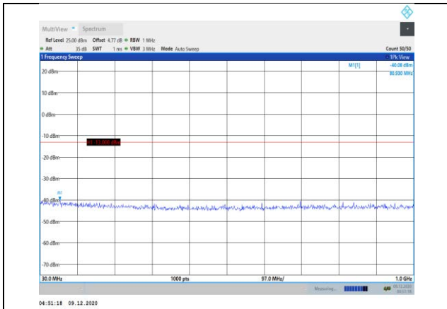
Band66-15MHz-QPSK-132047-1RB#0-Range1:30~1000MHz
