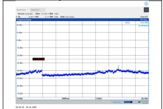
Band41-10MHz-16QAM-41190-1RB#0- Range3:3000~26000MHz
