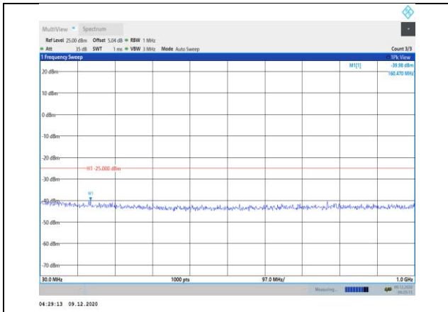
Band41-20MHz-16QAM-40740-1RB#0-Range1:30~1000MHz
