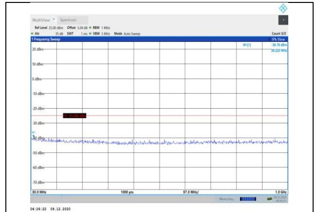
Band41-15MHz-16QAM-41165-1RB#0- Range1:30~1000MHz
