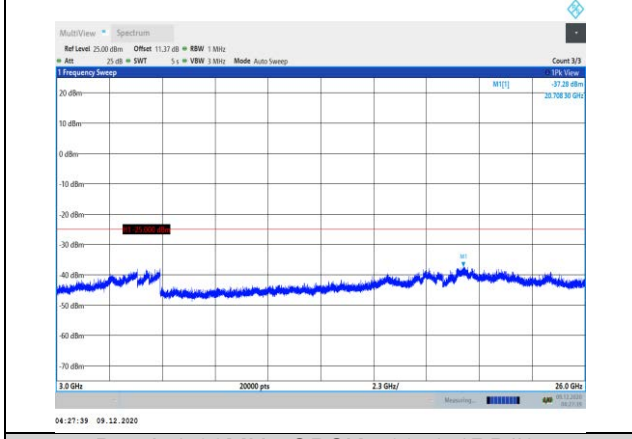
Band41-20MHz-QPSK-40340-1RB#0- Range3:3000~26000MHz
