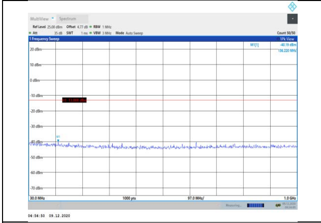
Band66-20MHz-16QAM-132322-1RB#0- Range1:30~1000MHz
