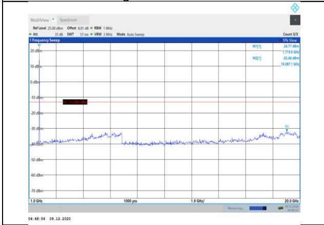
Band66-10MHz-16QAM-132022-1RB#0- Range2:1000~20000MHz
