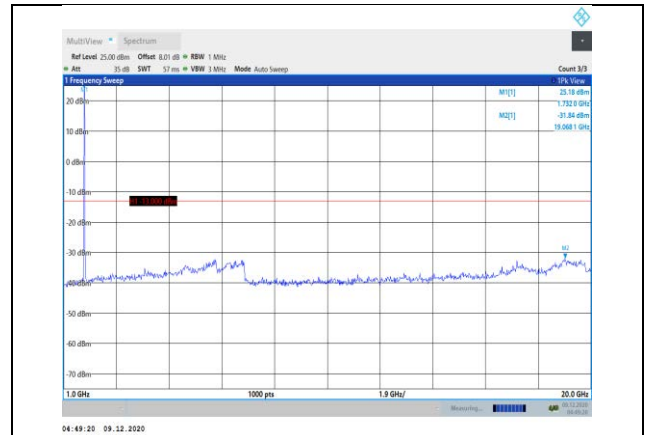
Band66-10MHz-QPSK-132322-1RB#0- Range2:1000~20000MHz
