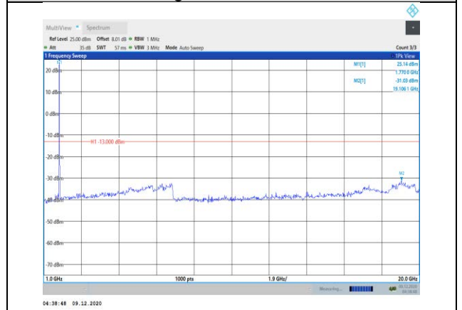
Band66-3MHz-QPSK-132657-1RB#0- Range2:1000~20000MHz
