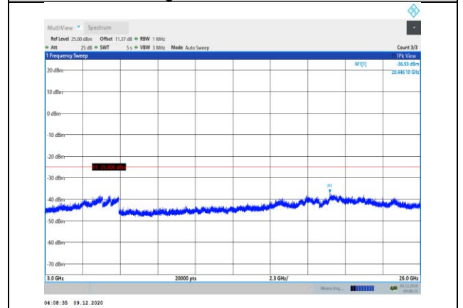
Band38-20MHz-QPSK-38000-1RB#0- Range3:3000~26000MHz
