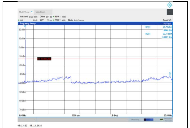
Band25-3MHz-16QAM-26365-1RB#0- Range2:1000~20000MHz
