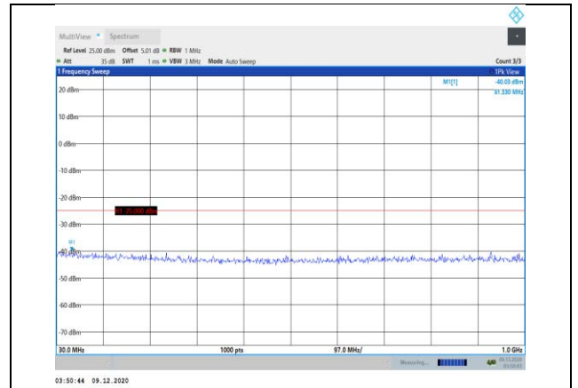
Band38-10MHz-QPSK-38000-1RB#0- Range1:30~1000MHz
