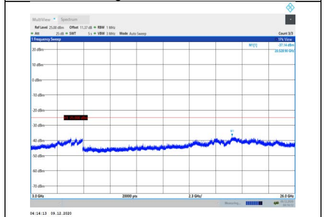
Band41-5MHz-16QAM-40265-1RB#0-Range3:3000~26000MHz
