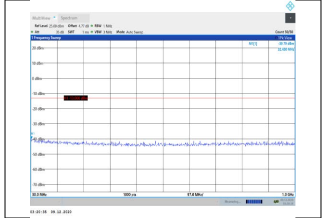
Band25-10MHz-QPSK-26640-1RB#0-Range1:30~1000MHz
