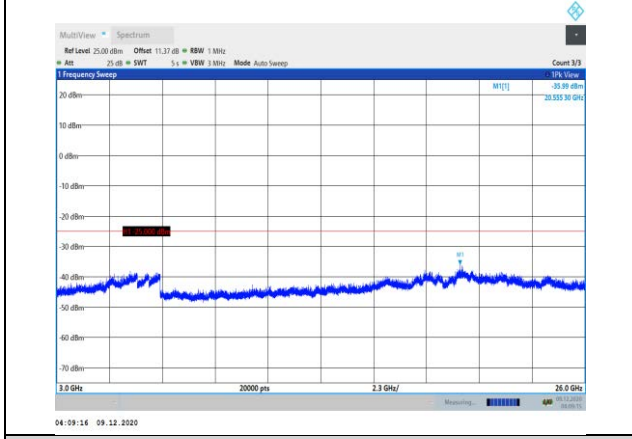
Band38-20MHz-16QAM-38000-1RB#0-Range3:3000~26000MHz
