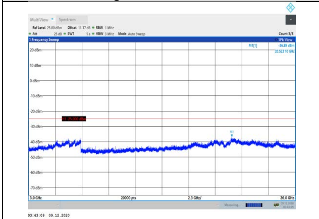
Band38-5MHz-16QAM-38000-1RB#0- Range3:3000~26000MHz
