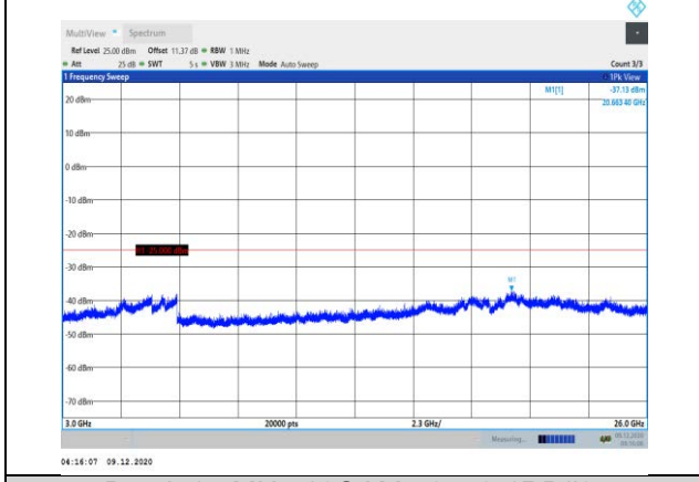
Band41-5MHz-16QAM-40740-1RB#0- Range3:3000~26000MHz
