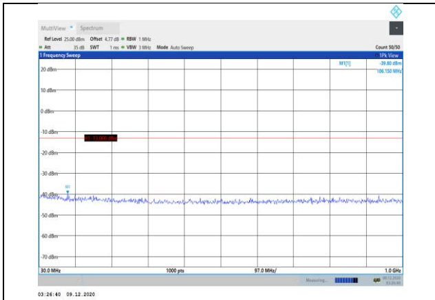
Band25-20MHz-16QAM-26140-1RB#0- Range1:30~1000MHz
