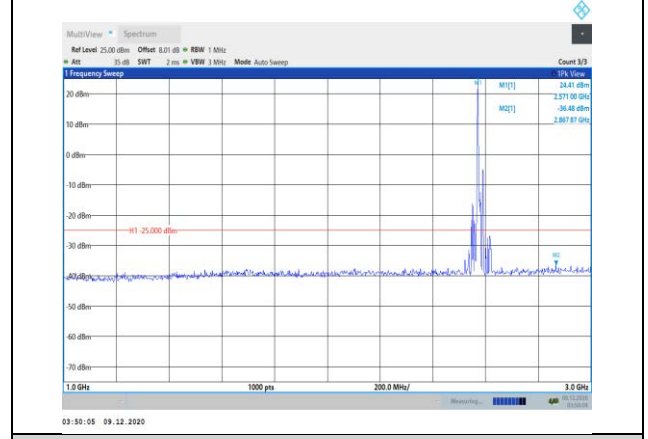
Band38-10MHz-16QAM-37800-1RB#0-Range2:1000~3000MHz
