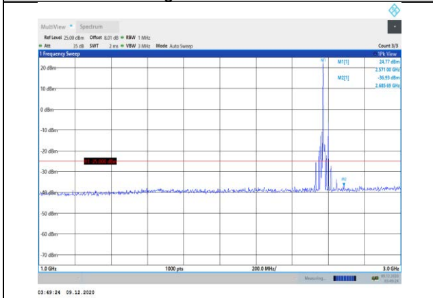
Band38-10MHz-QPSK-37800-1RB#0- Range2:1000~3000MHz
