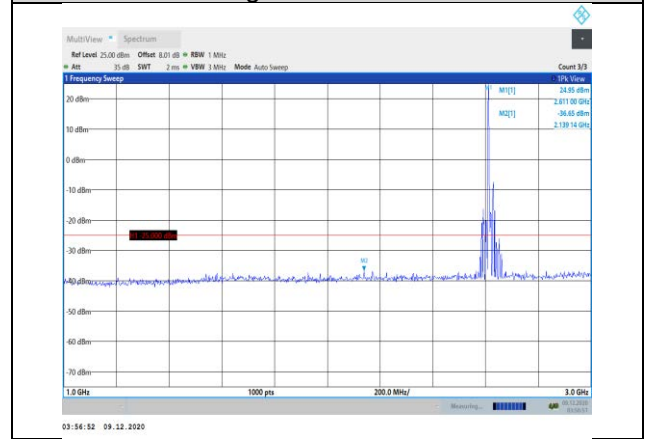
Band38-10MHz-16QAM-38200-1RB#0-Range2:1000~3000MHz
