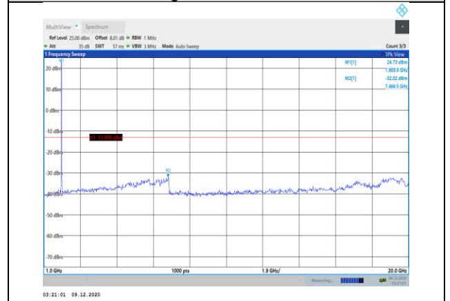
Band25-10MHz-16QAM-26640-1RB#0-Range2:1000~20000MHz
