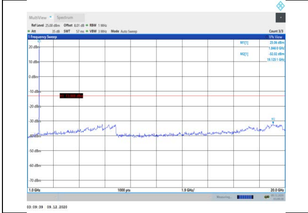
Band25-1.4MHz-16QAM-26047-1RB#0- Range2:1000~20000MHz
