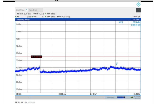
Band38-15MHz-16QAM-37825-1RB#0-Range3:3000~26000MHz
