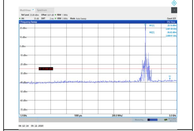
Band38-20MHz-16QAM-38150-1RB#0-Range2:1000~3000MHz
