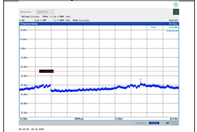
Band41-5MHz-QPSK-40740-1RB#0- Range3:3000~26000MHz
