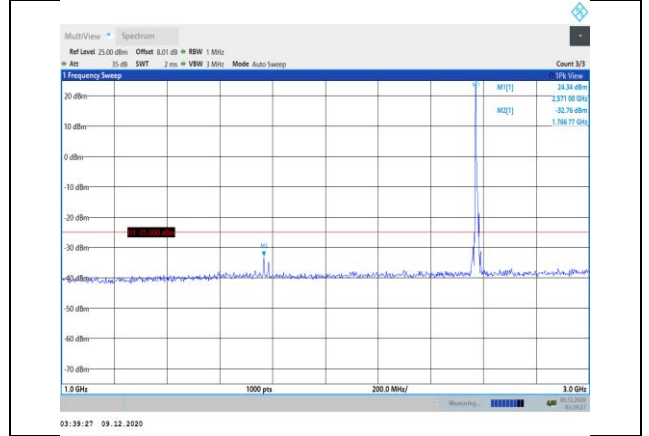
Band38-5MHz-16QAM-37775-1RB#0-Range2:1000~3000MHz
