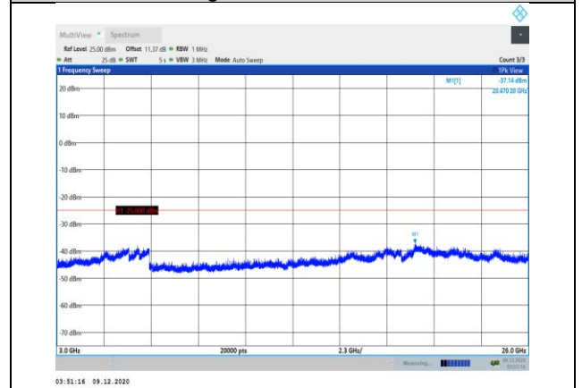
Band38-10MHz-QPSK-38000-1RB#0- Range3:3000~26000MHz
