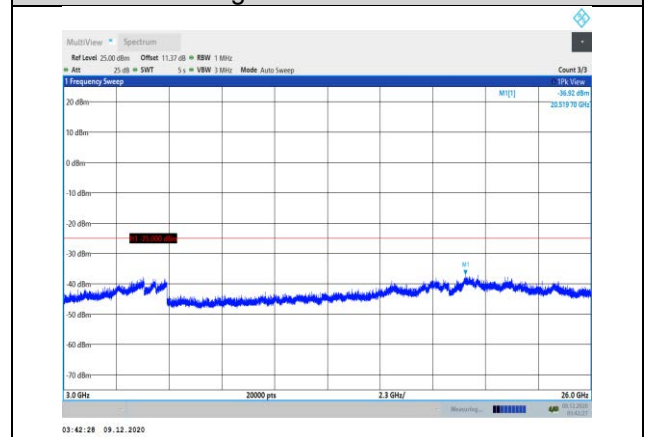
Band38-5MHz-QPSK-38000-1RB#0- Range3:3000~26000MHz
