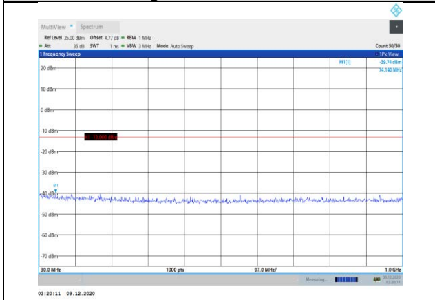
Band25-10MHz-16QAM-26365-1RB#0-Range1:30~1000MHz
