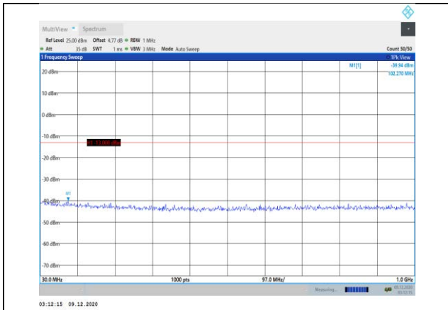
Band25-3MHz-QPSK-26055-1RB#0- Range1:30~1000MHz
