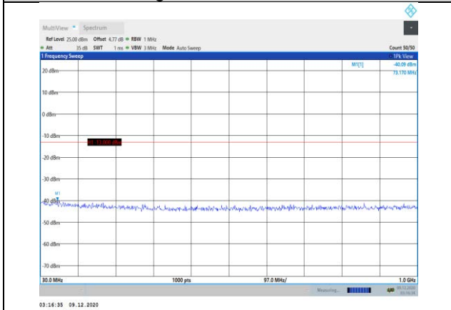
Band25-5MHz-QPSK-26365-1RB#0- Range1:30~1000MHz
