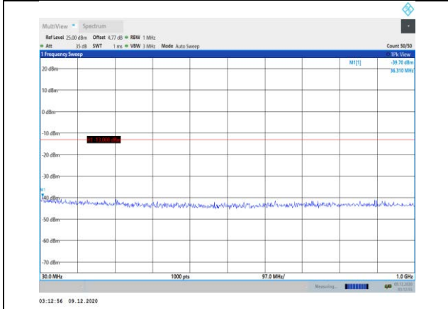
Band25-3MHz-QPSK-26365-1RB#0- Range1:30~1000MHz
