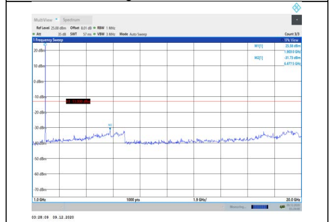
Band25-20MHz-16QAM-26590-1RB#0- Range2:1000~20000MHz
