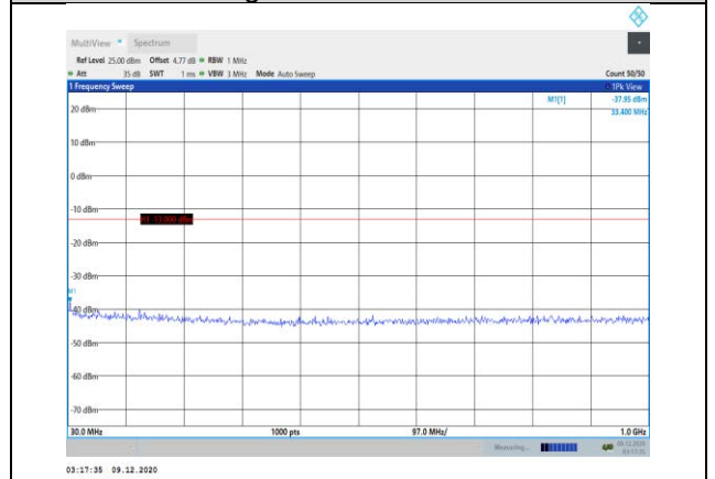
Band25-5MHz-16QAM-26665-1RB#0- Range1:30~1000MHz
