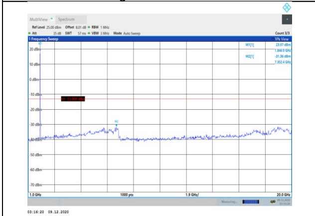
Band25-5MHz-16QAM-26065-1RB#0- Range2:1000~20000MHz
