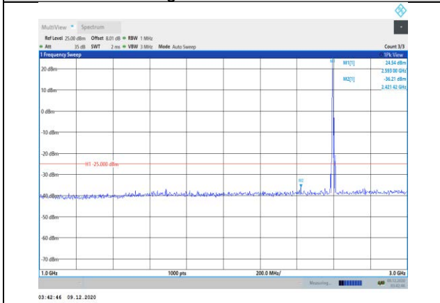
Band38-5MHz-16QAM-38000-1RB#0- Range2:1000~3000MHz
