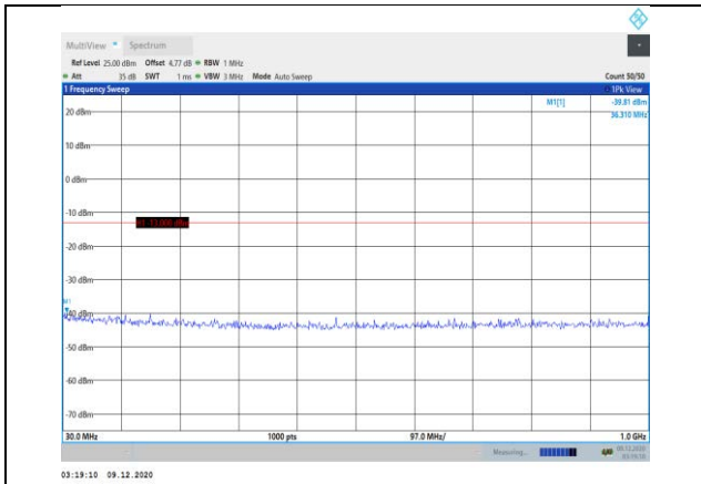
Band25-10MHz-QPSK-26090-1RB#0-Range1:30~1000MHz
