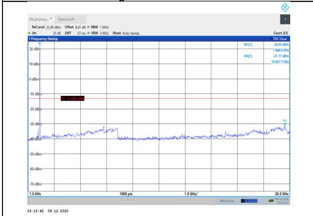
Band25-3MHz-16QAM-26055-1RB#0- Range2:1000~20000MHz
