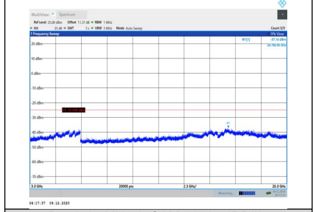
Band41-5MHz-16QAM-41215-1RB#0- Range3:3000~26000MHz
