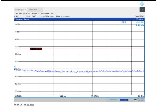
Band25-20MHz-16QAM-26365-1RB#0- Range1:30~1000MHz
