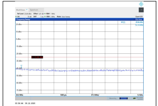
Band38-10MHz-16QAM-38200-1RB#0-Range1:30~1000MHz
