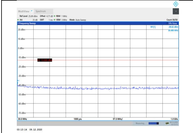
Band25-3MHz-16QAM-26365-1RB#0- Range1:30~1000MHz
