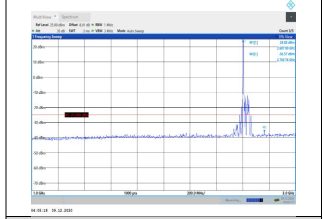
Band38-15MHz-16QAM-38175-1RB#0-Range2:1000~3000MHz
