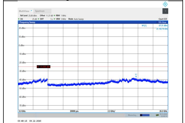
Band38-5MHz-16QAM-38225-1RB#0- Range3:3000~26000MHz
