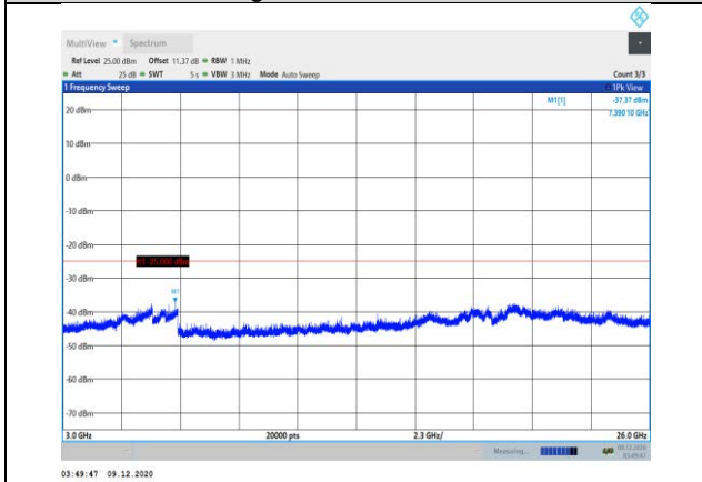
Band38-10MHz-QPSK-37800-1RB#0- Range3:3000~26000MHz
