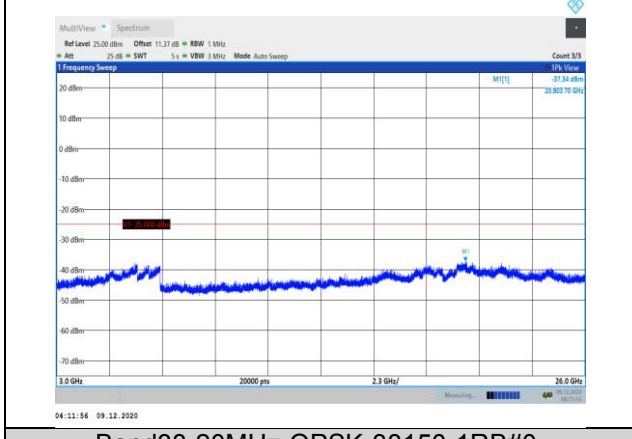
Band38-20MHz-QPSK-38150-1RB#0- Range3:3000~26000MHz
