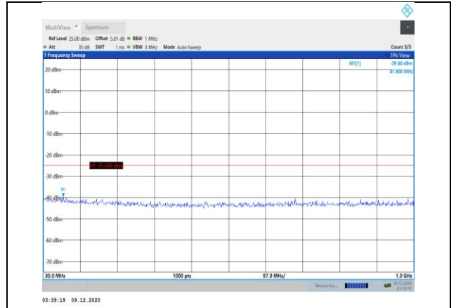
Band38-5MHz-16QAM-37775-1RB#0-Range1:30~1000MHz
