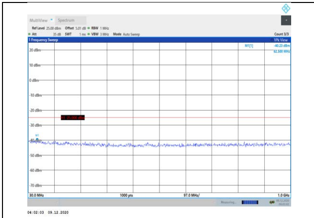
Band38-15MHz-16QAM-38000-1RB#0-Range1:30~1000MHz
