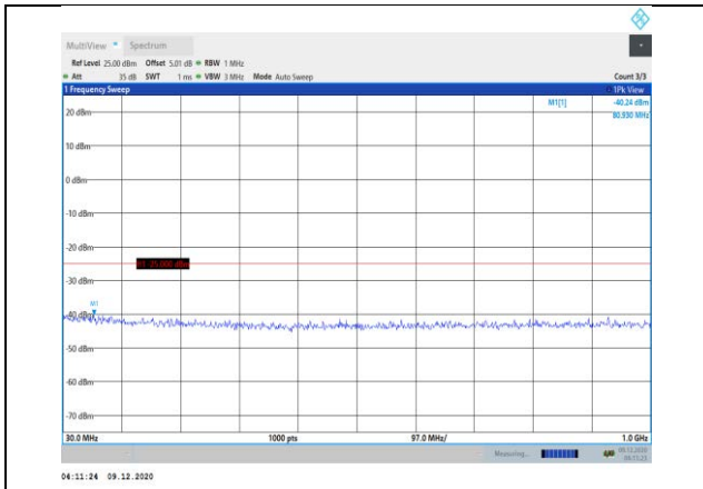
Band38-20MHz-QPSK-38150-1RB#0- Range1:30~1000MHz
