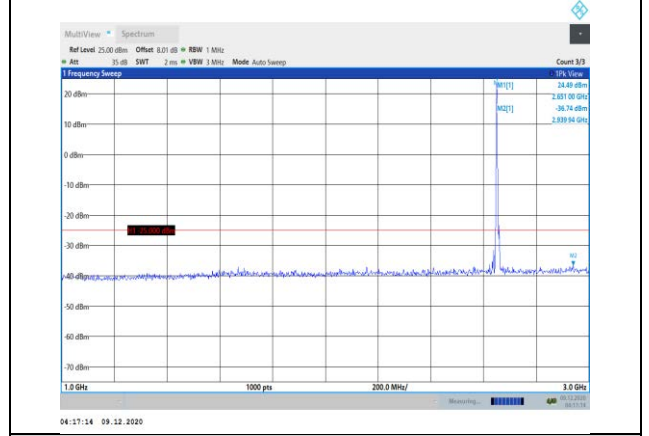
Band41-5MHz-16QAM-41215-1RB#0- Range2:1000~3000MHz
