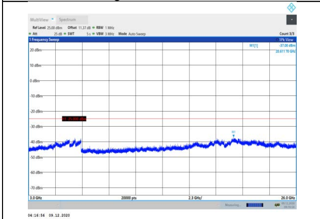
Band41-5MHz-QPSK-41215-1RB#0-Range3:3000~26000MHz
