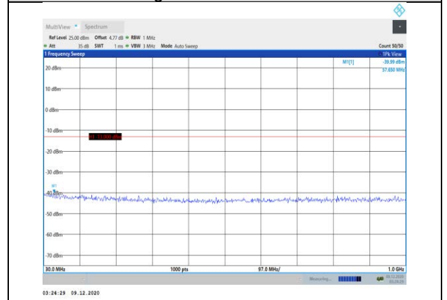
Band25-15MHz-QPSK-26615-1RB#0- Range1:30~1000MHz
