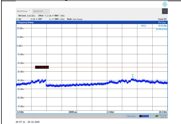
Band38-20MHz-QPSK-37850-1RB#0- Range3:3000~26000MHz
