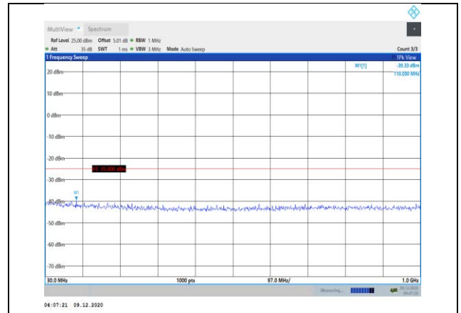
Band38-20MHz-16QAM-37850-1RB#0- Range1:30~1000MHz
