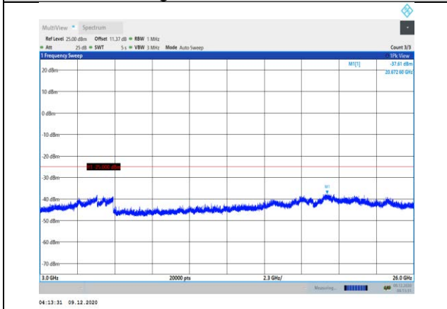
Band41-5MHz-QPSK-40265-1RB#0- Range3:3000~26000MHz
