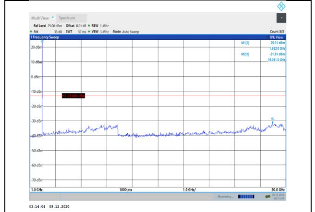
Band25-3MHz-16QAM-26675-1RB#0- Range2:1000~20000MHz
