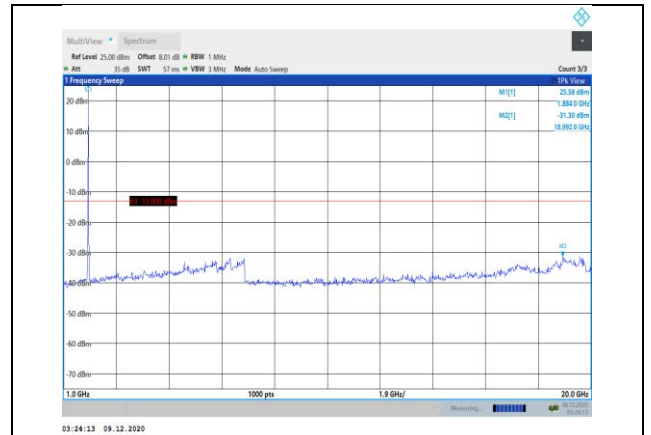
Band25-15MHz-16QAM-26365-1RB#0- Range2:1000~20000MHz
