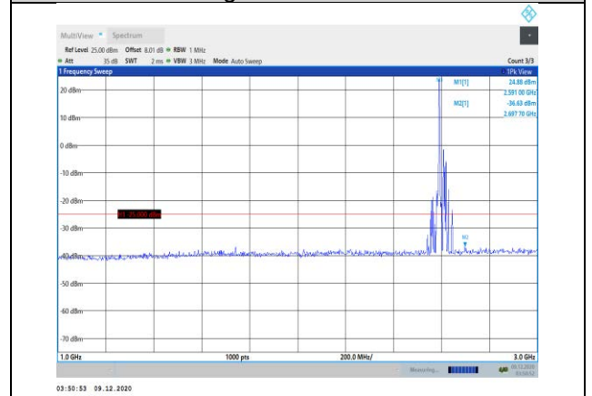
Band38-10MHz-QPSK-38000-1RB#0- Range2:1000~3000MHz
