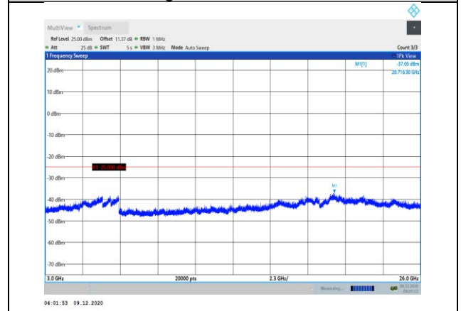
Band38-15MHz-QPSK-38000-1RB#0- Range3:3000~26000MHz
