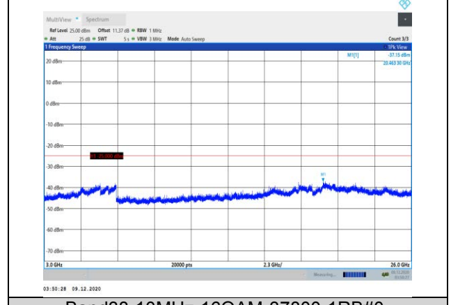
Band38-10MHz-16QAM-37800-1RB#0-Range3:3000~26000MHz
