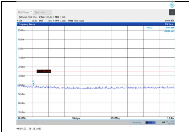
Band38-10MHz-QPSK-38200-1RB#0-Range1:30~1000MHz
