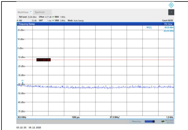
Band25-3MHz-16QAM-26055-1RB#0- Range1:30~1000MHz
