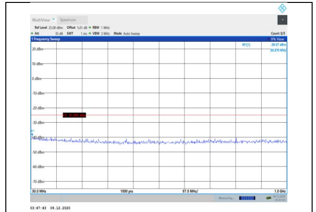
Band38-5MHz-16QAM-38225-1RB#0- Range1:30~1000MHz
