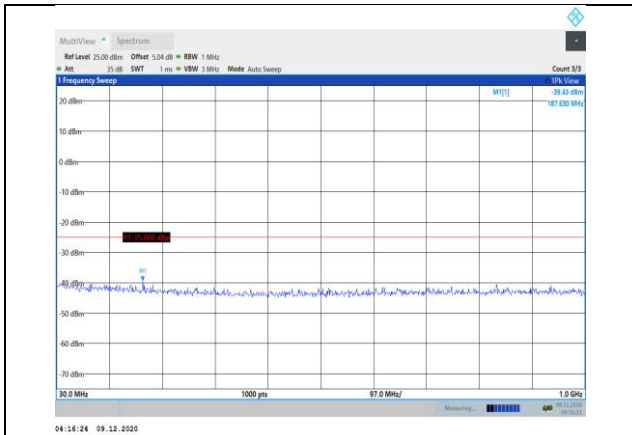
Band41-5MHz-QPSK-41215-1RB#0-Range1:30~1000MHz
