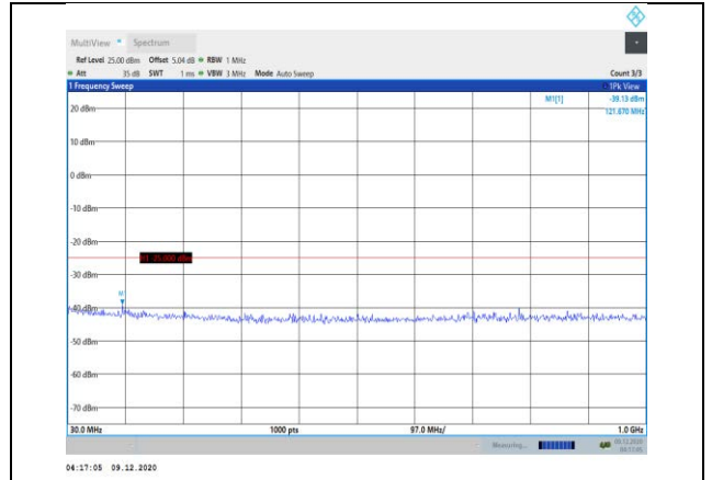
Band41-5MHz-16QAM-41215-1RB#0- Range1:30~1000MHz
