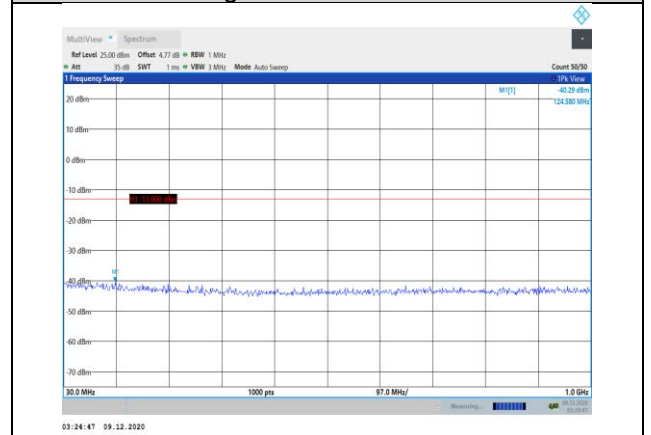
Band25-15MHz-16QAM-26615-1RB#0- Range1:30~1000MHz
