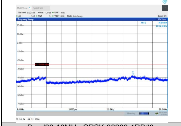
Band38-10MHz-QPSK-38200-1RB#0-Range3:3000~26000MHz
