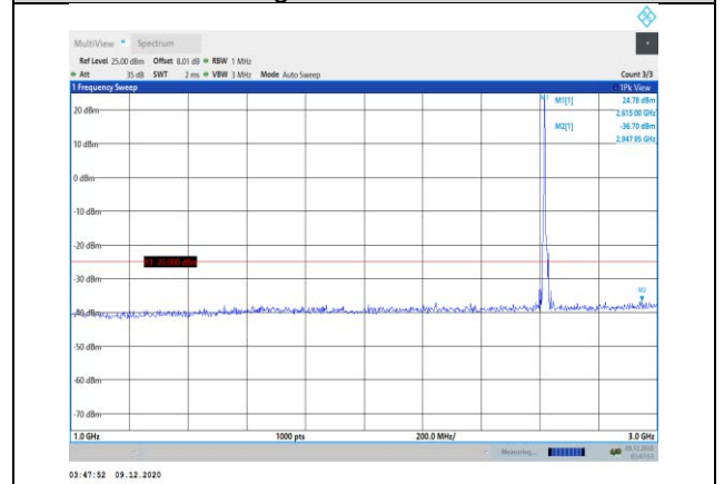
Band38-5MHz-16QAM-38225-1RB#0- Range2:1000~3000MHz
