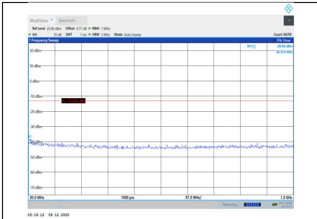
Band25-5MHz-16QAM-26065-1RB#0- Range1:30~1000MHz
