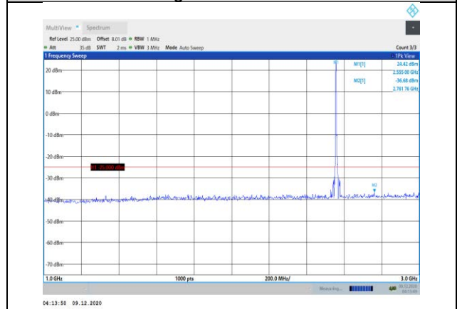
Band41-5MHz-16QAM-40265-1RB#0-Range2:1000~3000MHz
