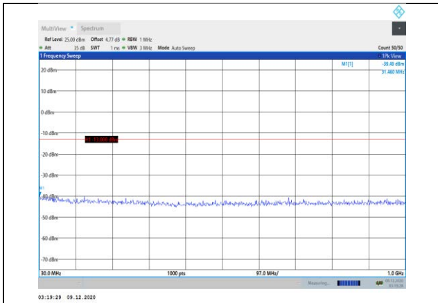
Band25-10MHz-16QAM-26090-1RB#0-Range1:30~1000MHz
