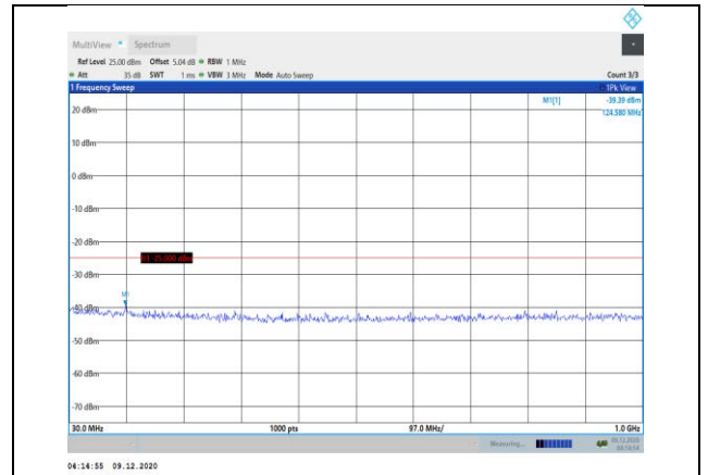
Band41-5MHz-QPSK-40740-1RB#0- Range1:30~1000MHz
