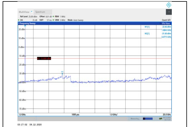
Band25-5MHz-16QAM-26365-1RB#0- Range2:1000~20000MHz
