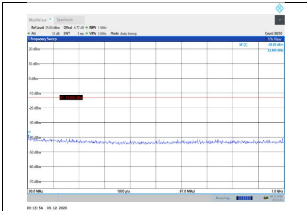
Band25-5MHz-QPSK-26065-1RB#0- Range1:30~1000MHz
