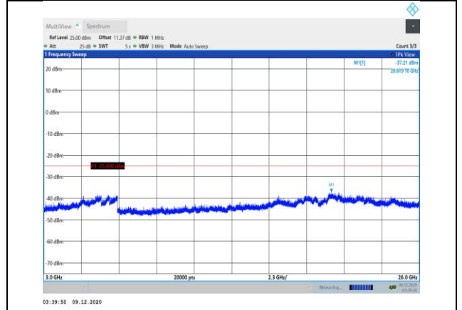
Band38-5MHz-16QAM-37775-1RB#0-Range3:3000~26000MHz
