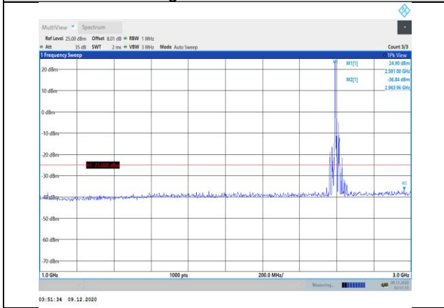
Band38-10MHz-16QAM-38000-1RB#0-Range2:1000~3000MHz
