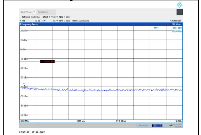
Band25-20MHz-16QAM-26590-1RB#0- Range1:30~1000MHz
