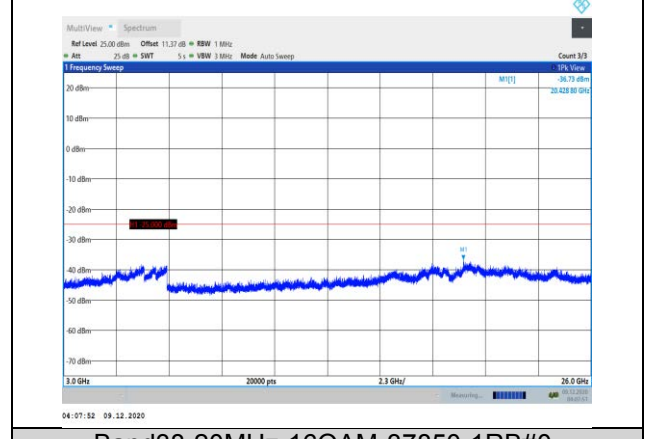
Band38-20MHz-16QAM-37850-1RB#0- Range3:3000~26000MHz
