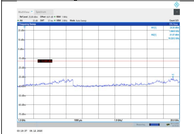
Band25-10MHz-16QAM-26090-1RB#0-Range2:1000~20000MHz
