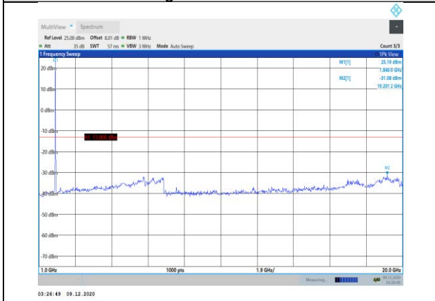
Band25-20MHz-16QAM-26140-1RB#0- Range2:1000~20000MHz
