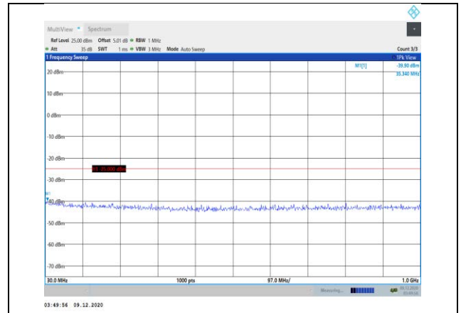
Band38-10MHz-16QAM-37800-1RB#0-Range1:30~1000MHz
