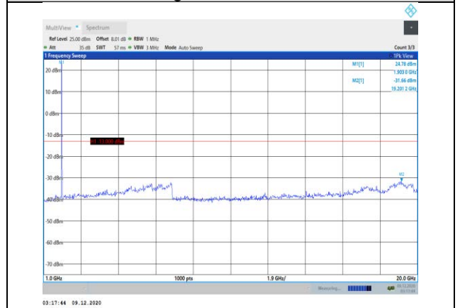
Band25-5MHz-16QAM-26665-1RB#0- Range2:1000~20000MHz
