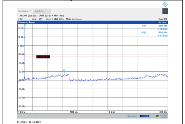
Band25-5MHz-QPSK-26665-1RB#0- Range2:1000~20000MHz
