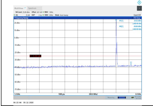
Band41-5MHz-16QAM-40740-1RB#0- Range2:1000~3000MHz
