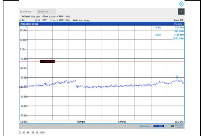
Band25-10MHz-QPSK-26640-1RB#0-Range2:1000~20000MHz
