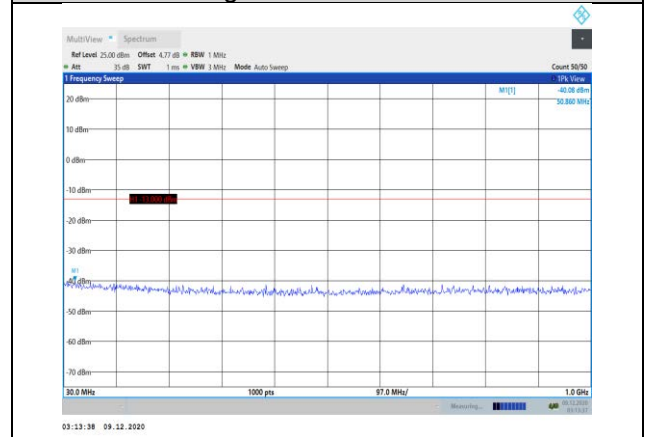
Band25-3MHz-QPSK-26675-1RB#0- Range1:30~1000MHz
