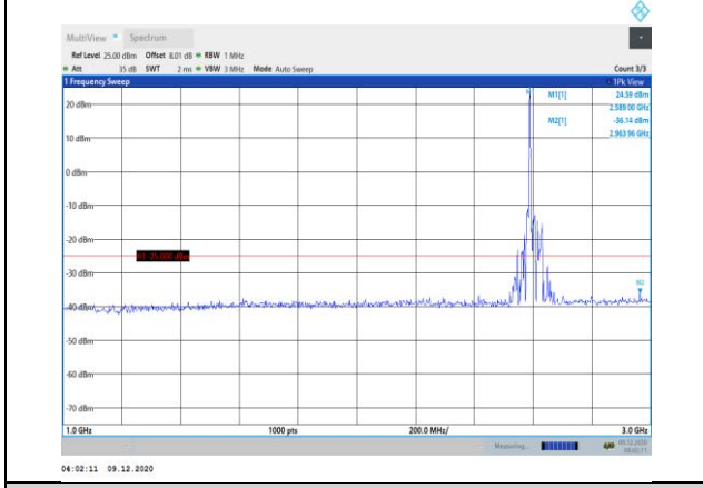
Band38-15MHz-16QAM-38000-1RB#0-Range2:1000~3000MHz
