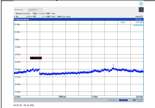
Band38-15MHz-QPSK-37825-1RB#0- Range3:3000~26000MHz
