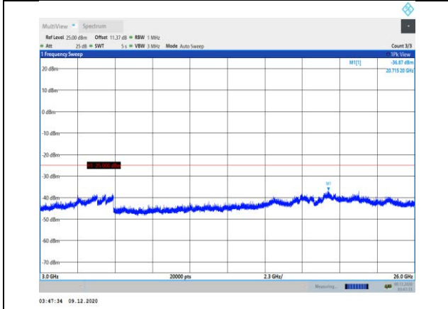
Band38-5MHz-QPSK-38225-1RB#0-Range3:3000~26000MHz
