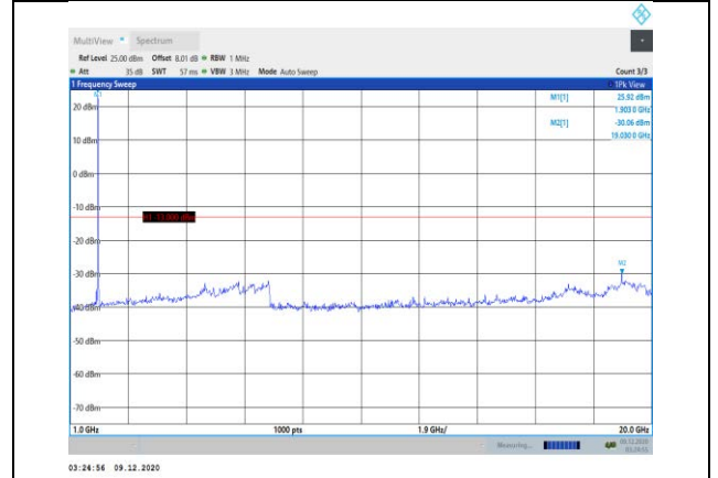
Band25-15MHz-16QAM-26615-1RB#0- Range2:1000~20000MHz
