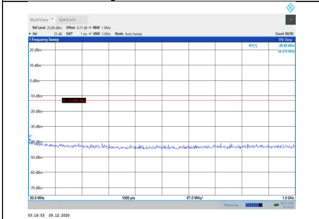
Band25-5MHz-16QAM-26365-1RB#0- Range1:30~1000MHz
