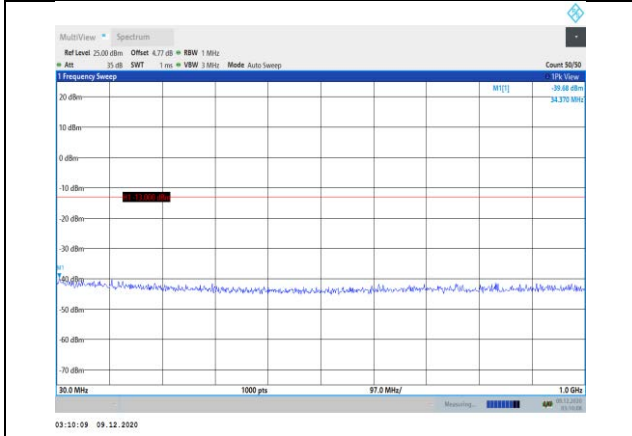
Band25-1.4MHz-16QAM-26365-1RB#0- Range1:30~1000MHz
