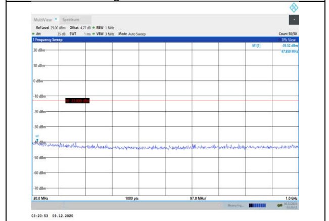
Band25-10MHz-16QAM-26640-1RB#0-Range1:30~1000MHz
