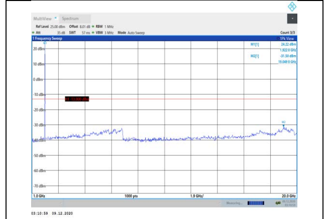
Band25-1.4MHz-16QAM-26683-1RB#0- Range2:1000~20000MHz
