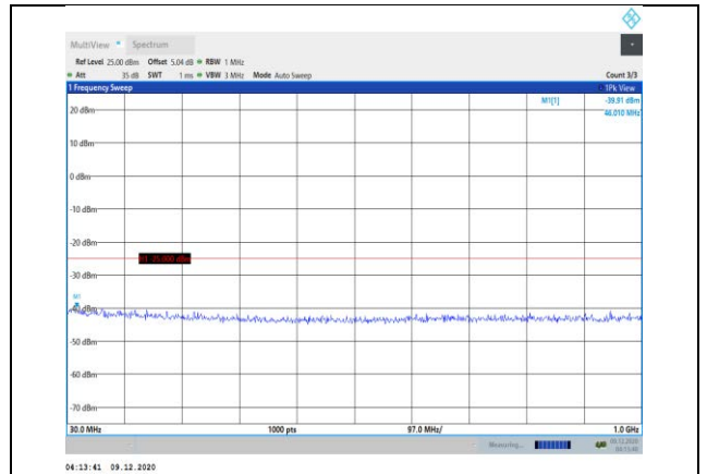
Band41-5MHz-16QAM-40265-1RB#0-Range1:30~1000MHz
