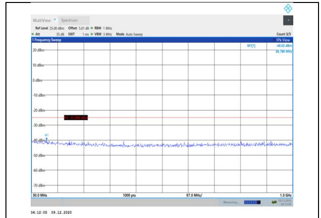
Band38-20MHz-16QAM-38150-1RB#0-Range1:30~1000MHz
