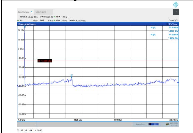
Band25-15MHz-16QAM-26115-1RB#0- Range2:1000~20000MHz
