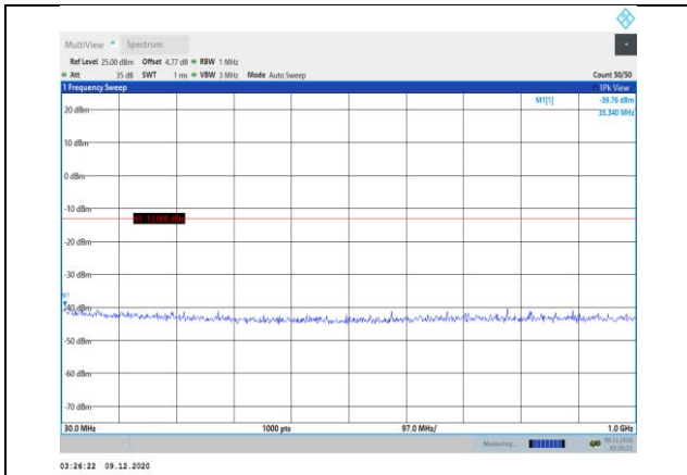
Band25-20MHz-QPSK-26140-1RB#0- Range1:30~1000MHz
