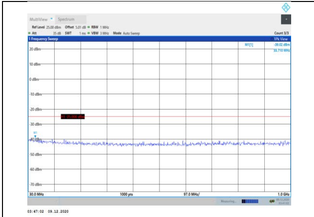
Band38-5MHz-QPSK-38225-1RB#0-Range1:30~1000MHz
