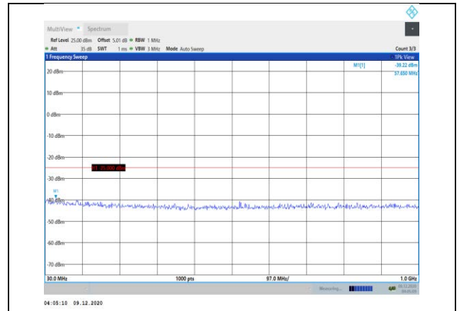
Band38-15MHz-16QAM-38175-1RB#0-Range1:30~1000MHz
