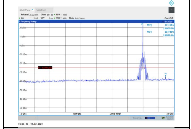
Band38-15MHz-QPSK-38000-1RB#0- Range2:1000~3000MHz
