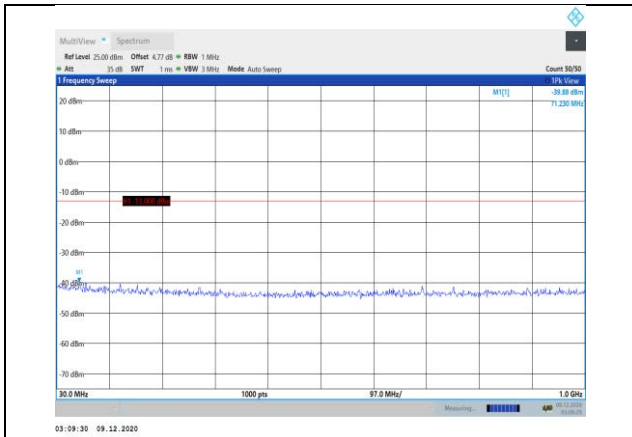
Band25-1.4MHz-16QAM-26047-1RB#0- Range1:30~1000MHz
