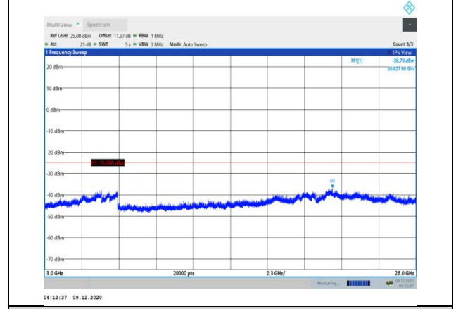
Band38-20MHz-16QAM-38150-1RB#0-Range3:3000~26000MHz
