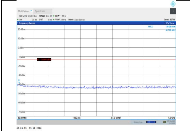
Band25-15MHz-16QAM-26365-1RB#0- Range1:30~1000MHz
