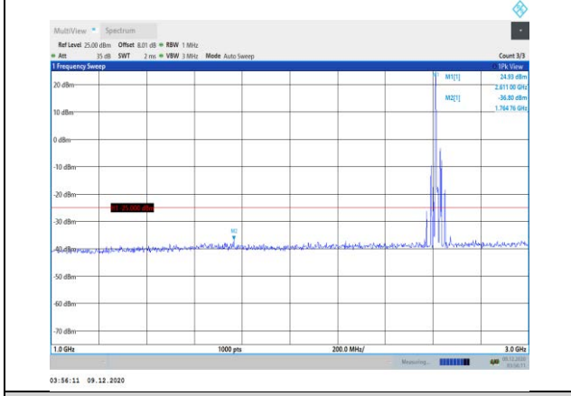
Band38-10MHz-QPSK-38200-1RB#0-Range2:1000~3000MHz
