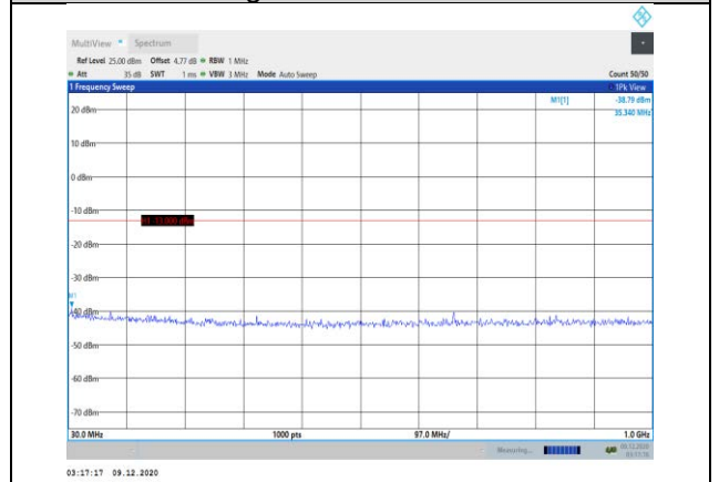
Band25-5MHz-QPSK-26665-1RB#0- Range1:30~1000MHz
