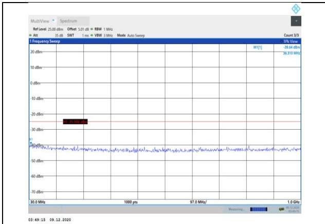
Band38-10MHz-QPSK-37800-1RB#0- Range1:30~1000MHz
