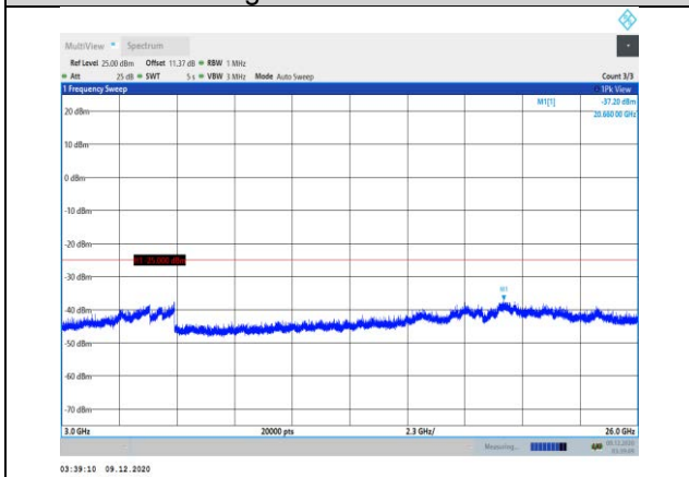
Band38-5MHz-QPSK-37775-1RB#0- Range3:3000~26000MHz
