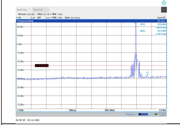
Band38-20MHz-16QAM-38000-1RB#0-Range2:1000~3000MHz
