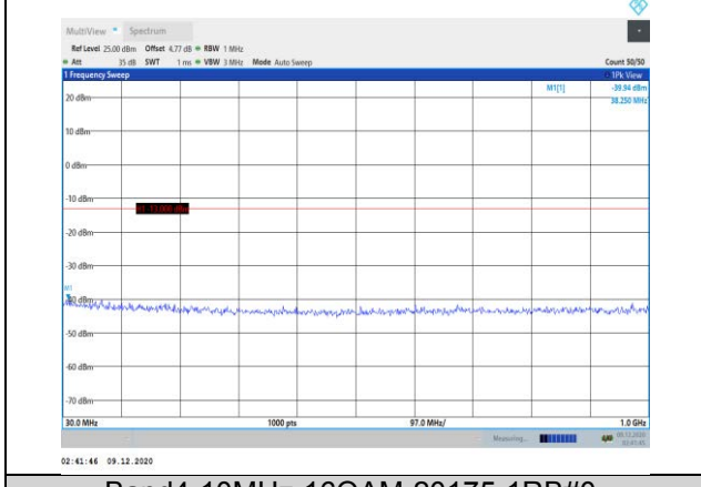
Band4-10MHz-16QAM-20175-1RB#0- Range1:30~1000MHz
