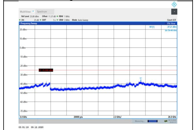
Band7-15MHz-QPSK-21100-1RB#0- Range3:3000~26000MHz
