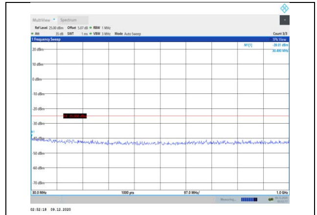
Band7-5MHz-16QAM-21425-1RB#0- Range1:30~1000MHz
