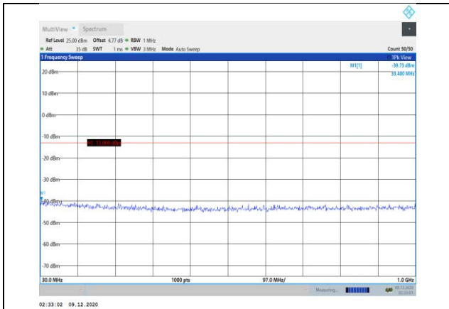
Band4-3MHz-16QAM-19965-1RB#0- Range1:30~1000MHz
