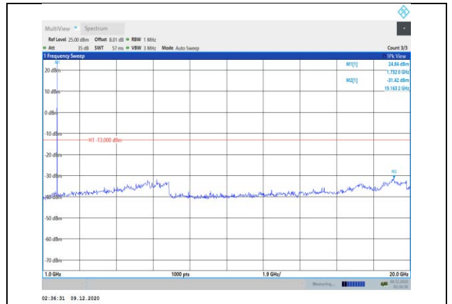
Band4-5MHz-16QAM-20175-1RB#0- Range2:1000~20000MHz
