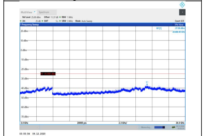
Band7-20MHz-16QAM-20850-1RB#0- Range3:3000~26000MHz
