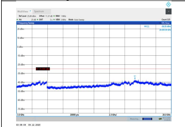
Band7-20MHz-QPSK-21350-1RB#0- Range3:3000~26000MHz
