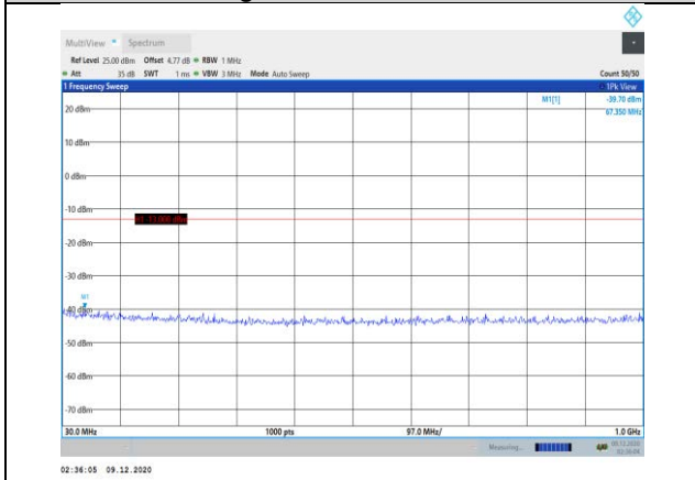
Band4-5MHz-QPSK-20175-1RB#0- Range1:30~1000MHz
