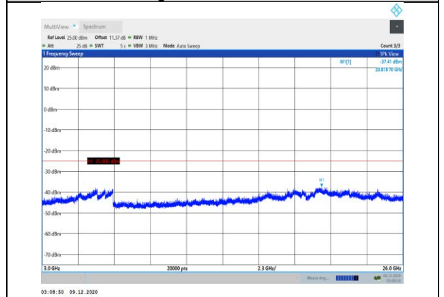
Band7-20MHz-16QAM-21350-1RB#0- Range3:3000~26000MHz
