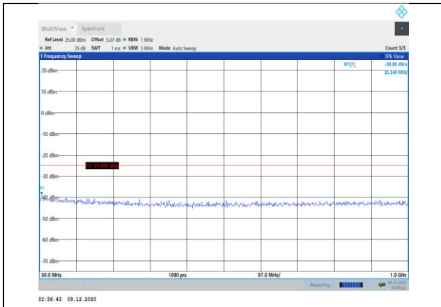
Band7-10MHz-QPSK-21400-1RB#0- Range1:30~1000MHz
