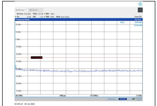
Band7-20MHz-16QAM-21350-1RB#0- Range1:30~1000MHz
