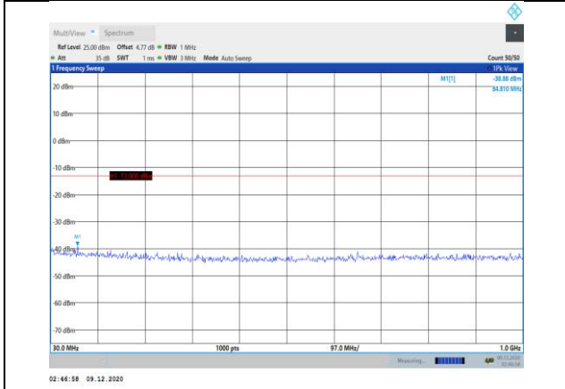
Band4-20MHz-QPSK-20175-1RB#0-Range1:30~1000MHz
