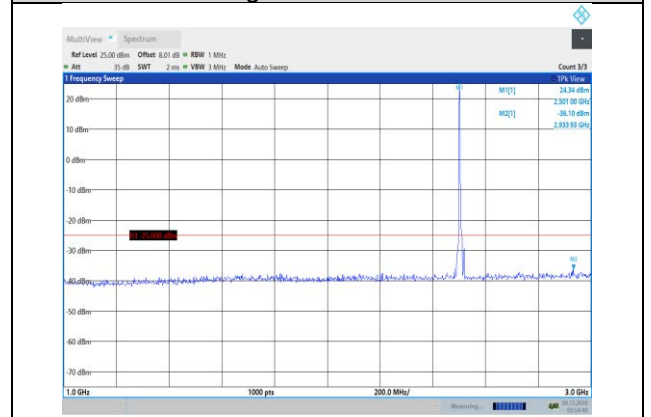
Band7-10MHz-16QAM-20800-1RB#0- Range2:1000~3000MHz
