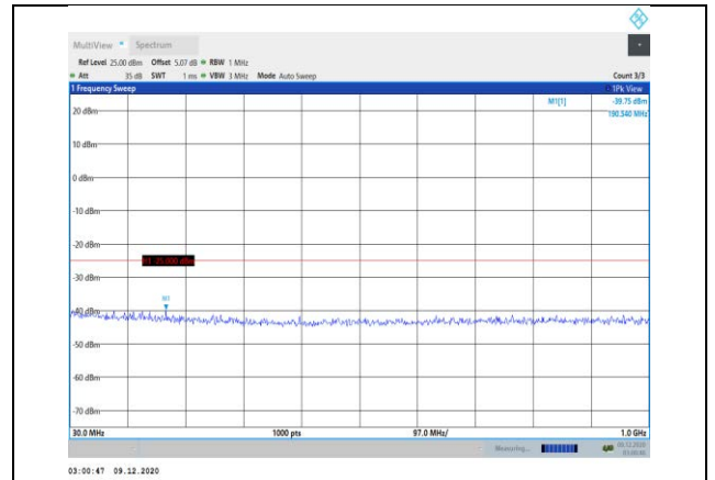
Band7-15MHz-QPSK-21100-1RB#0- Range1:30~1000MHz
