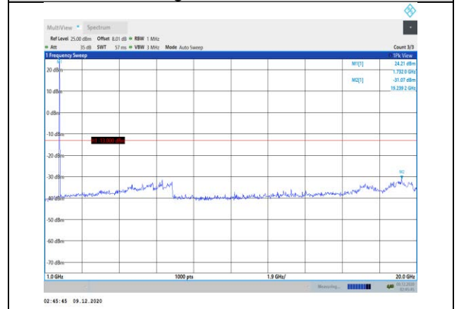
Band4-15MHz-16QAM-20325-1RB#0- Range2:1000~20000MHz
