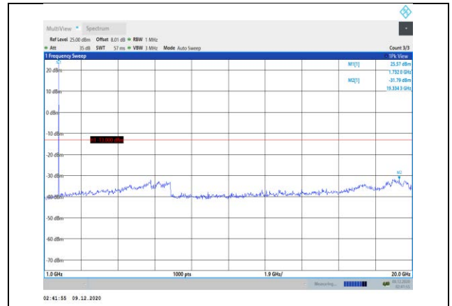
Band4-10MHz-16QAM-20175-1RB#0- Range2:1000~20000MHz
