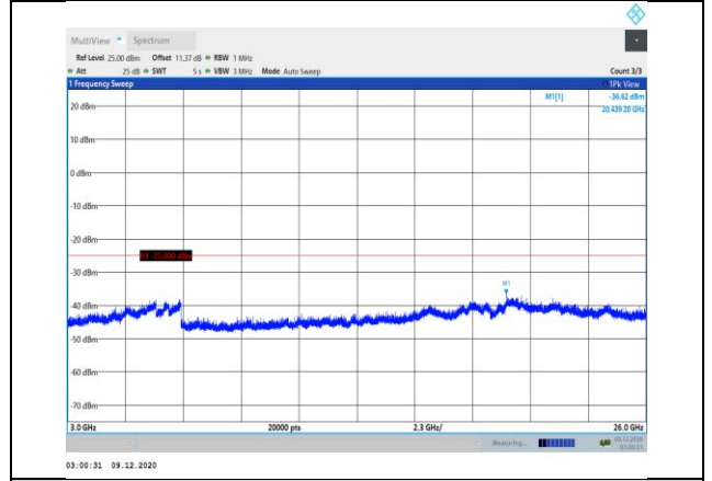
Band7-15MHz-16QAM-20825-1RB#0- Range3:3000~26000MHz
