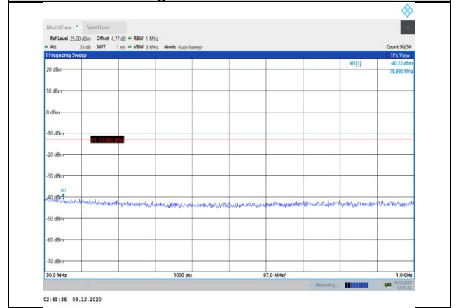
Band4-15MHz-16QAM-20325-1RB#0- Range1:30~1000MHz
