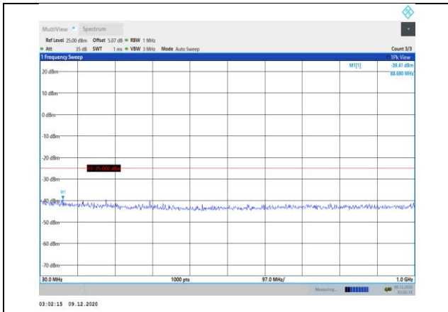
Band7-15MHz-QPSK-21375-1RB#0- Range1:30~1000MHz
