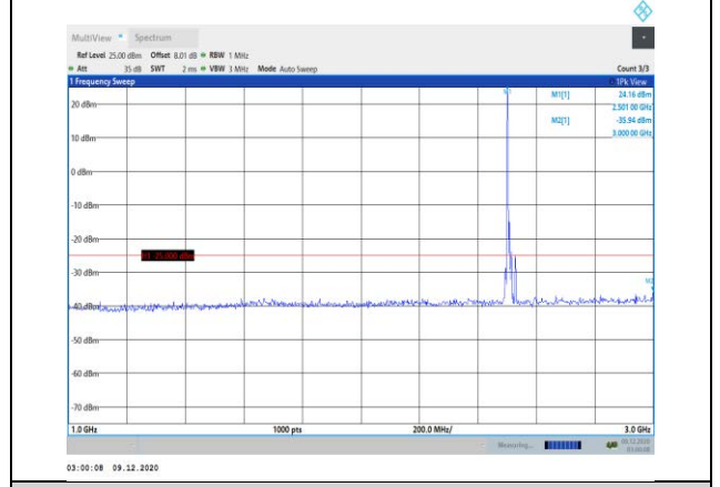
Band7-15MHz-16QAM-20825-1RB#0- Range2:1000~3000MHz
