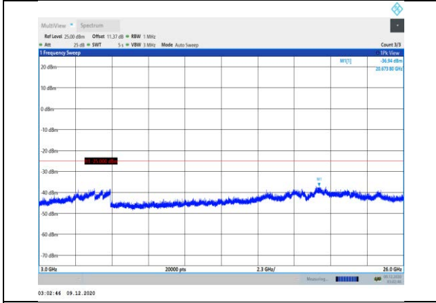
Band7-15MHz-QPSK-21375-1RB#0- Range3:3000~26000MHz
