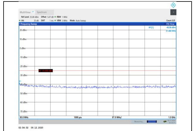
Band7-10MHz-16QAM-20800-1RB#0- Range1:30~1000MHz
