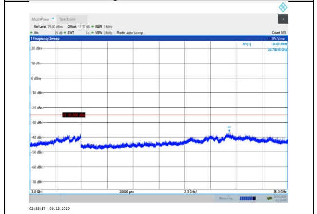
Band7-10MHz-QPSK-21100-1RB#0- Range3:3000~26000MHz
