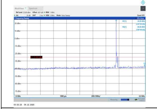
Band7-15MHz-QPSK-21375-1RB#0- Range2:1000~3000MHz
