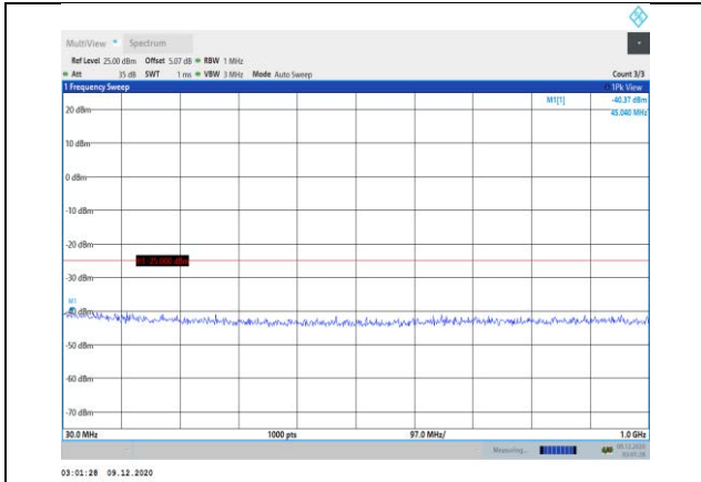
Band7-15MHz-16QAM-21100-1RB#0- Range1:30~1000MHz
