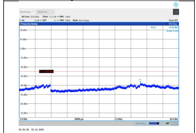
Band7-5MHz-16QAM-21425-1RB#0- Range3:3000~26000MHz
