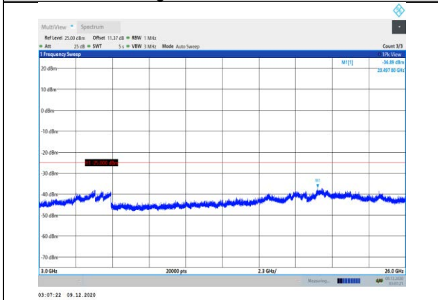
Band7-20MHz-16QAM-21100-1RB#0- Range3:3000~26000MHz
