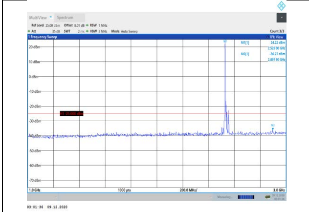
Band7-15MHz-16QAM-21100-1RB#0- Range2:1000~3000MHz
