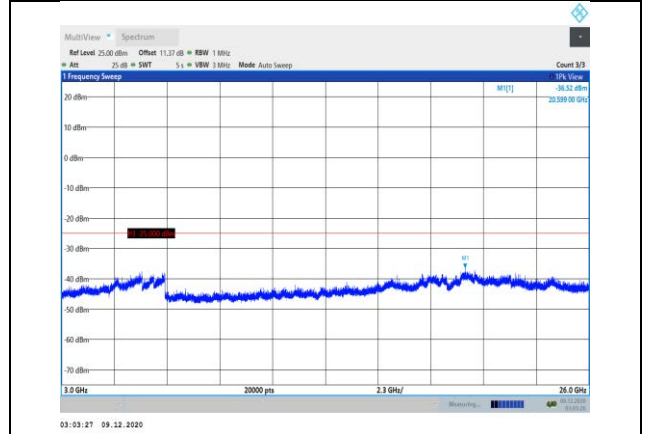
Band7-15MHz-16QAM-21375-1RB#0- Range3:3000~26000MHz
