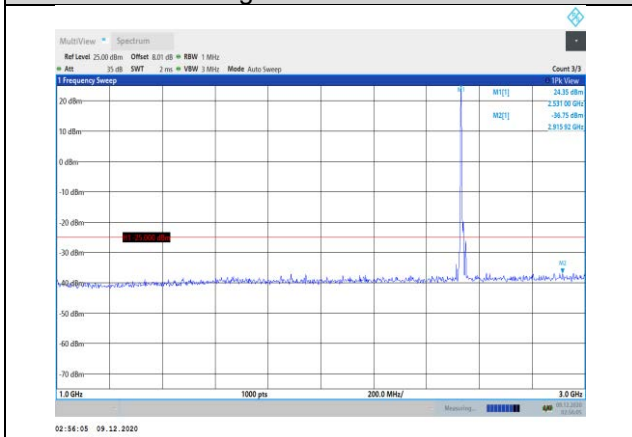
Band7-10MHz-16QAM-21100-1RB#0- Range2:1000~3000MHz
