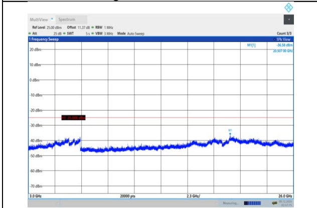
Band7-10MHz-QPSK-21400-1RB#0- Range3:3000~26000MHz
