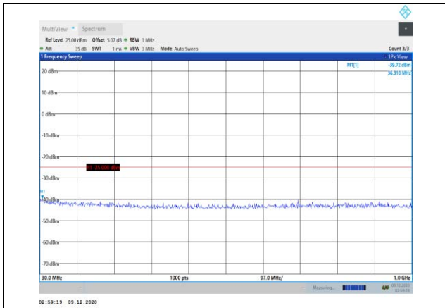
Band7-15MHz-QPSK-20825-1RB#0- Range1:30~1000MHz
