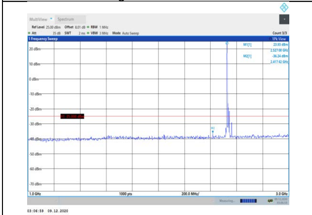
Band7-20MHz-16QAM-21100-1RB#0- Range2:1000~3000MHz
