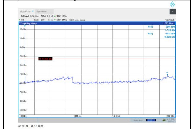
Band4-1.4MHz-16QAM-20393-1RB#0- Range2:1000~20000MHz
