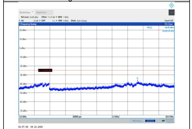
Band7-10MHz-16QAM-21400-1RB#0- Range3:3000~26000MHz
