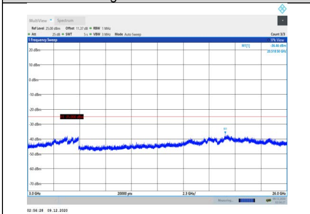
Band7-10MHz-16QAM-21100-1RB#0- Range3:3000~26000MHz
