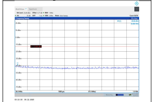
Band25-1.4MHz-QPSK-26683-1RB#0-Range1:30~1000MHz
