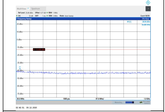
Band4-10MHz-16QAM-20350-1RB#0- Range1:30~1000MHz
