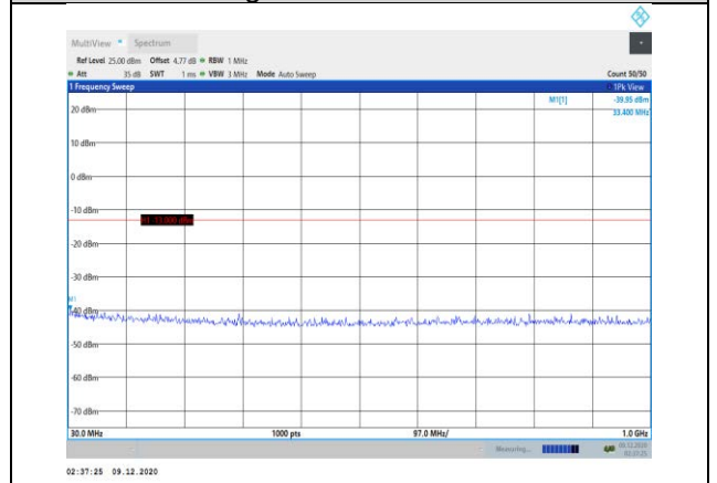
Band4-5MHz-16QAM-20375-1RB#0- Range1:30~1000MHz
