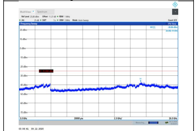
Band7-20MHz-QPSK-21100-1RB#0- Range3:3000~26000MHz
