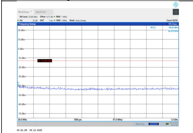
Band4-10MHz-QPSK-20175-1RB#0-Range1:30~1000MHz
