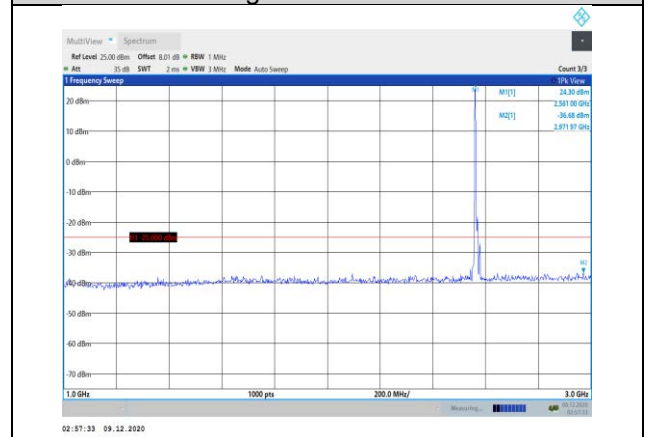
Band7-10MHz-16QAM-21400-1RB#0- Range2:1000~3000MHz
