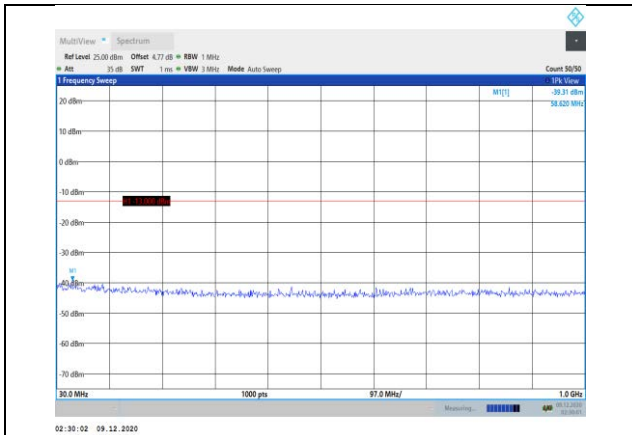
Band4-1.4MHz-QPSK-19957-1RB#0- Range1:30~1000MHz
