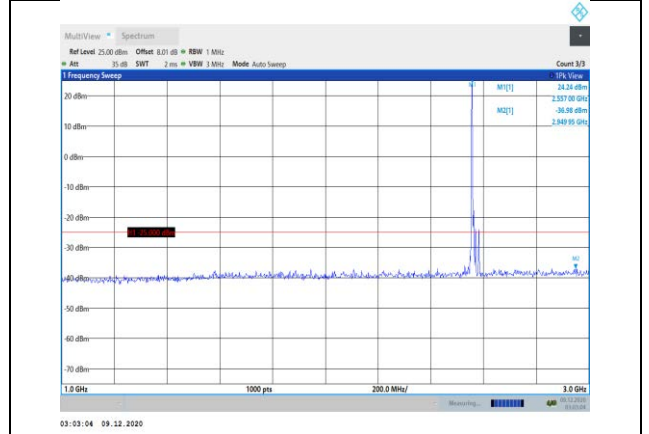
Band7-15MHz-16QAM-21375-1RB#0- Range2:1000~3000MHz
