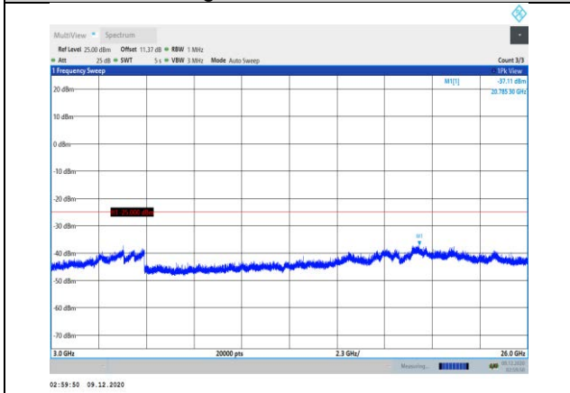
Band7-15MHz-QPSK-20825-1RB#0- Range3:3000~26000MHz
