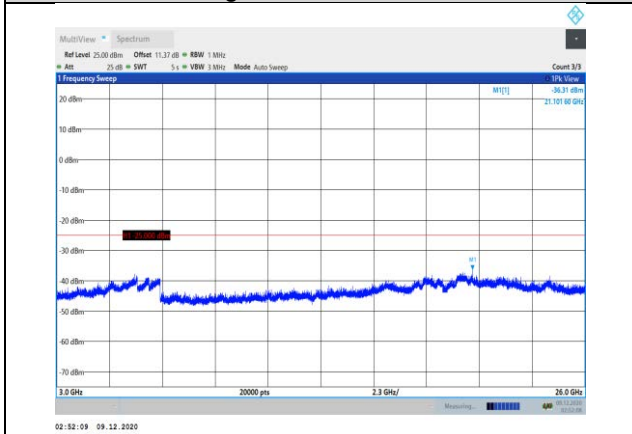
Band7-5MHz-QPSK-21425-1RB#0- Range3:3000~26000MHz
