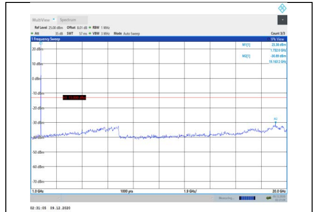
Band4-1.4MHz-16QAM-20175-1RB#0- Range2:1000~20000MHz
