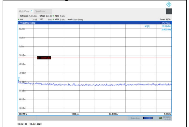
Band4-10MHz-QPSK-20350-1RB#0-Range1:30~1000MHz
