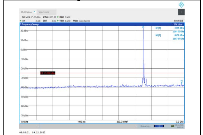
Band7-20MHz-16QAM-20850-1RB#0- Range2:1000~3000MHz
