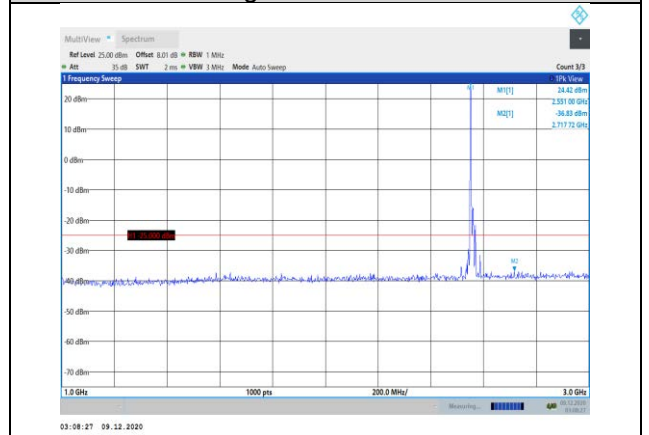
Band7-20MHz-16QAM-21350-1RB#0- Range2:1000~3000MHz
