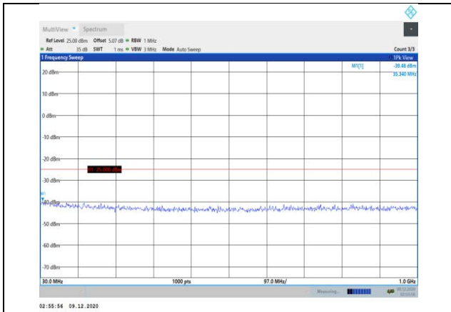
Band7-10MHz-16QAM-21100-1RB#0- Range1:30~1000MHz
