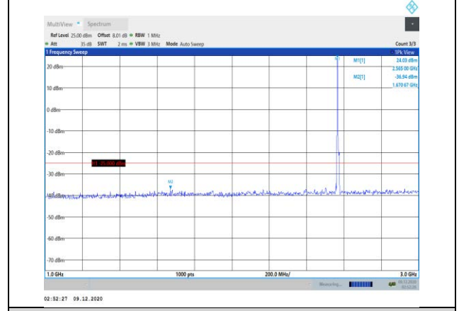
Band7-5MHz-16QAM-21425-1RB#0- Range2:1000~3000MHz
