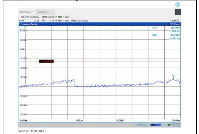
Band4-5MHz-16QAM-20375-1RB#0- Range2:1000~20000MHz
