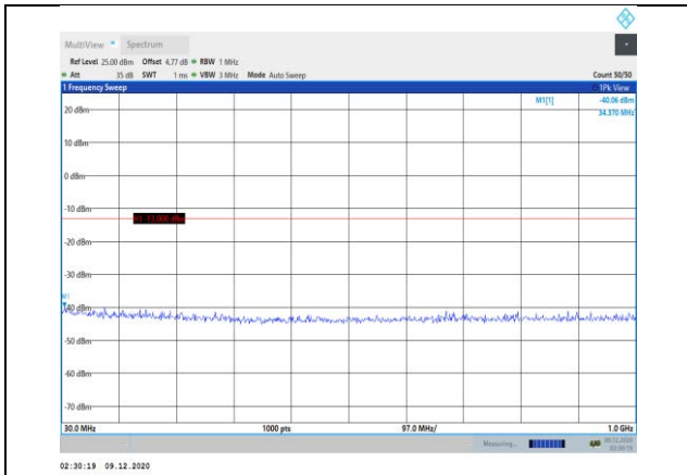
Band4-1.4MHz-16QAM-19957-1RB#0- Range1:30~1000MHz
