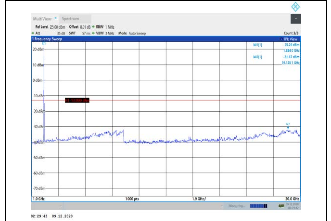
Band2-20MHz-16QAM-19100-1RB#0- Range2:1000~20000MHz
