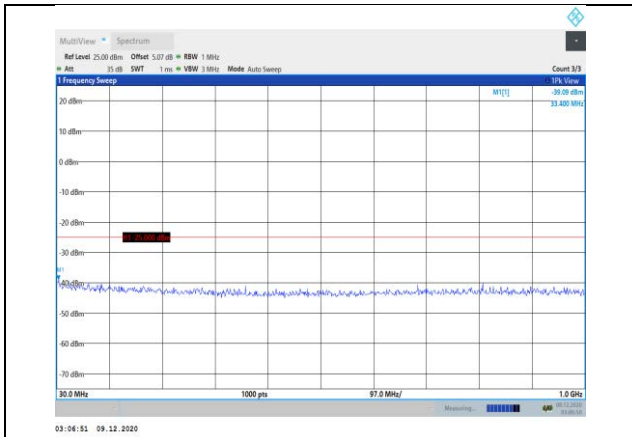
Band7-20MHz-16QAM-21100-1RB#0- Range1:30~1000MHz
