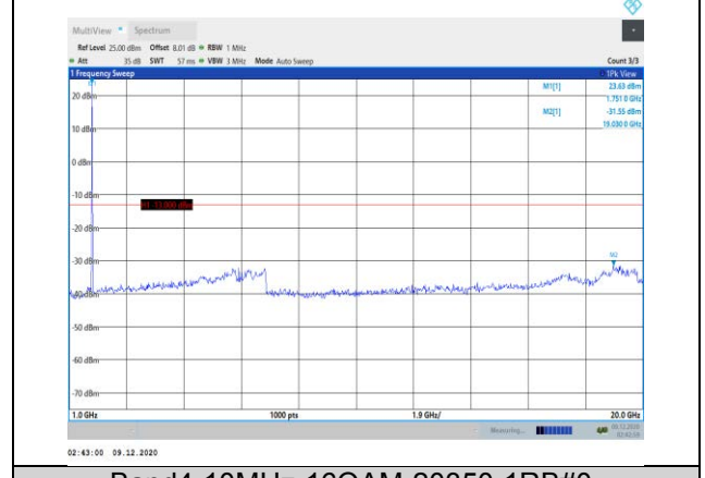
Band4-10MHz-16QAM-20350-1RB#0- Range2:1000~20000MHz
