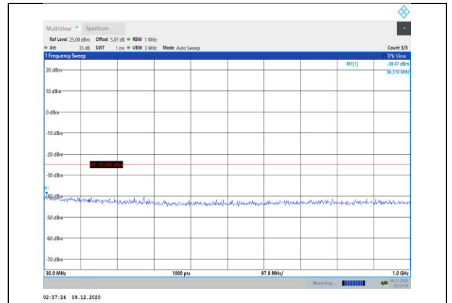
Band7-10MHz-16QAM-21400-1RB#0- Range1:30~1000MHz
