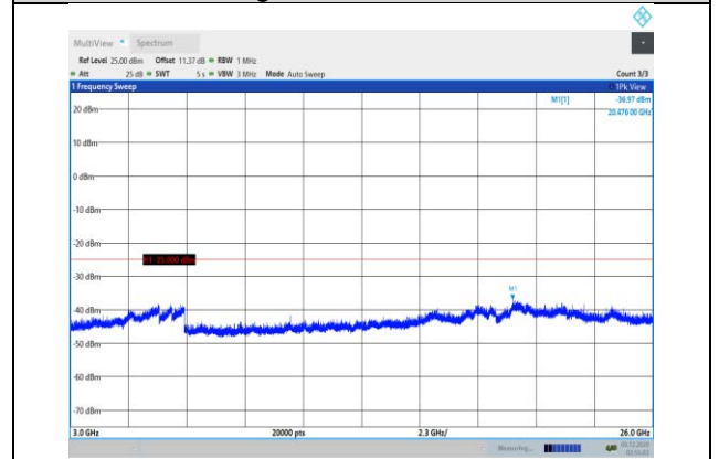
Band7-10MHz-16QAM-20800-1RB#0- Range3:3000~26000MHz
