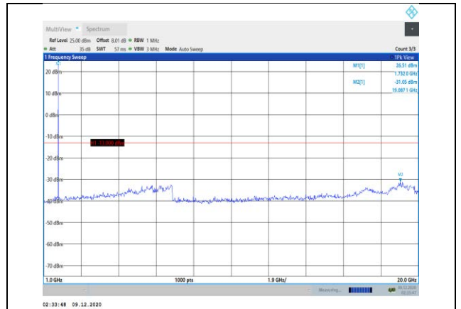
Band4-3MHz-16QAM-20175-1RB#0- Range2:1000~20000MHz
