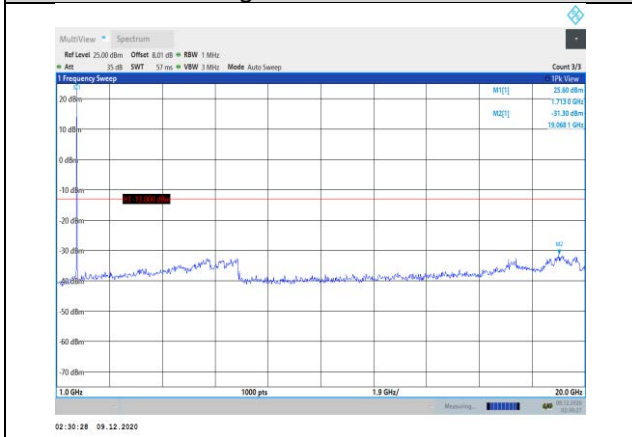
Band4-1.4MHz-16QAM-19957-1RB#0- Range2:1000~20000MHz
