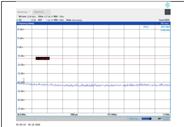
Band25-1.4MHz-QPSK-26047-1RB#0-Range1:30~1000MHz
