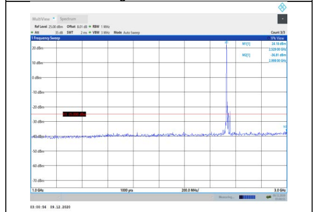
Band7-15MHz-QPSK-21100-1RB#0- Range2:1000~3000MHz
