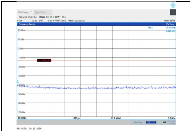
Band4-5MHz-QPSK-19975-1RB#0- Range1:30~1000MHz
