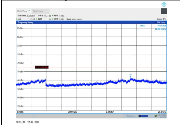
Band7-5MHz-16QAM-21100-1RB#0- Range3:3000~26000MHz
