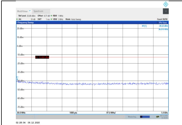
Band2-20MHz-16QAM-18700-1RB#0- Range1:30~1000MHz
