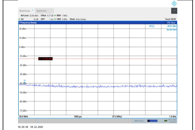
Band2-20MHz-16QAM-19100-1RB#0- Range1:30~1000MHz
