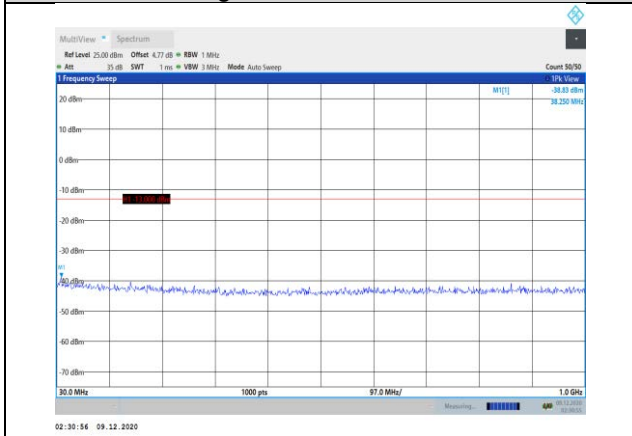
Band4-1.4MHz-16QAM-20175-1RB#0- Range1:30~1000MHz
