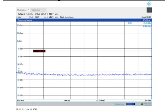
Band4-1.4MHz-16QAM-20393-1RB#0- Range1:30~1000MHz
