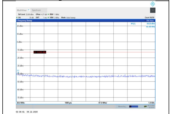
Band4-3MHz-16QAM-20385-1RB#0- Range1:30~1000MHz
