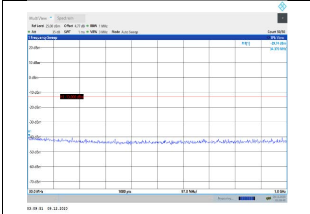
Band25-1.4MHz-QPSK-26365-1RB#0-Range1:30~1000MHz
