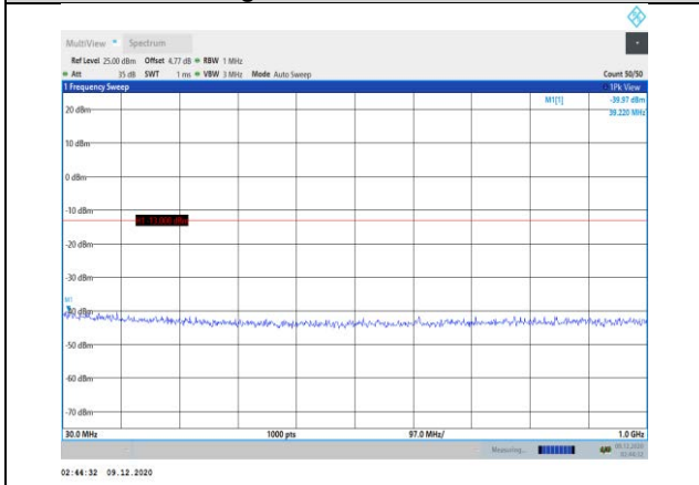
Band4-15MHz-16QAM-20175-1RB#0- Range1:30~1000MHz
