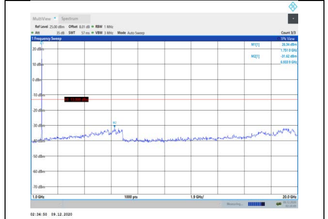
Band4-3MHz-16QAM-20385-1RB#0- Range2:1000~20000MHz
