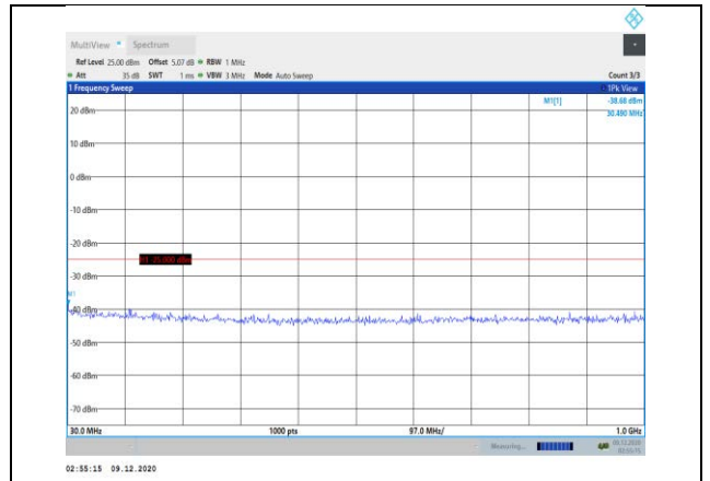
Band7-10MHz-QPSK-21100-1RB#0- Range1:30~1000MHz
