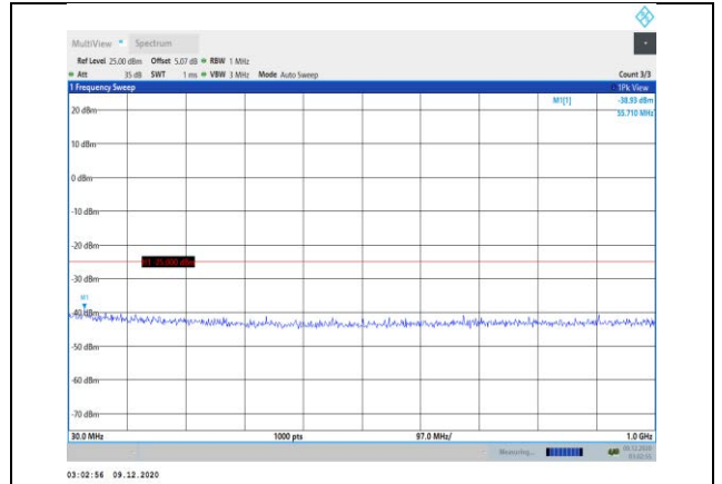
Band7-15MHz-16QAM-21375-1RB#0- Range1:30~1000MHz
