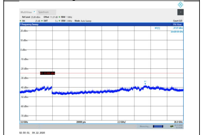
Band7-5MHz-16QAM-20775-1RB#0- Range3:3000~26000MHz
