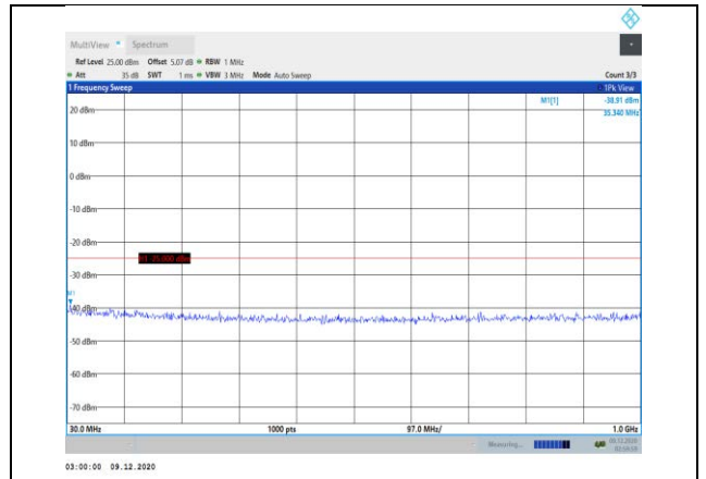
Band7-15MHz-16QAM-20825-1RB#0- Range1:30~1000MHz
