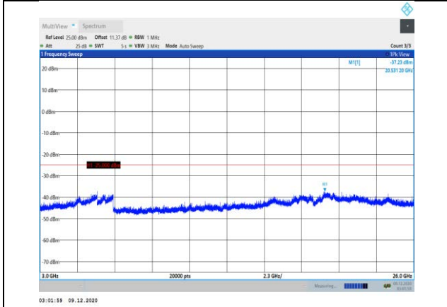
Band7-15MHz-16QAM-21100-1RB#0- Range3:3000~26000MHz
