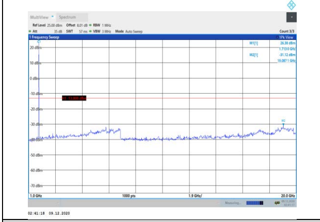
Band4-10MHz-16QAM-20000-1RB#0- Range2:1000~20000MHz
