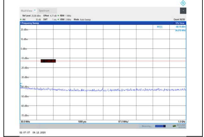
Band2-1.4MHz-QPSK-19193-1RB#0-Range1:30~1000MHz
