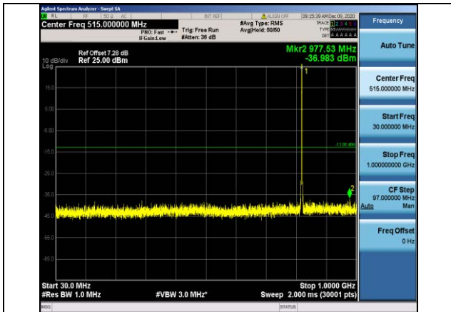
Band26-1.4MHz-16QAM-26783-1RB#0- Range1:30~1000MHz
