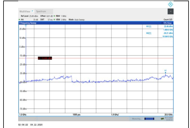
Band2-1.4MHz-QPSK-18900-1RB#0-Range2:1000~20000MHz
