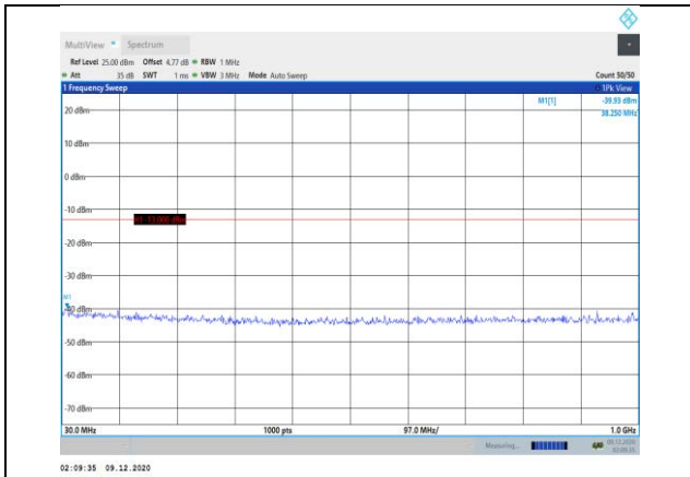
Band2-3MHz-QPSK-18615-1RB#0- Range1:30~1000MHz
