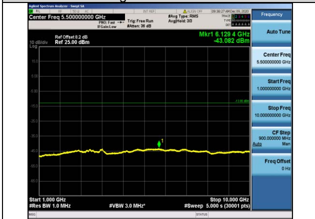
Band26-5MHz-16QAM-26765-1RB#0- Range2:1000~10000MHz
