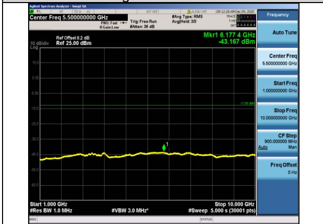
Band26-3MHz-16QAM-26775-1RB#0- Range2:1000~10000MHz
