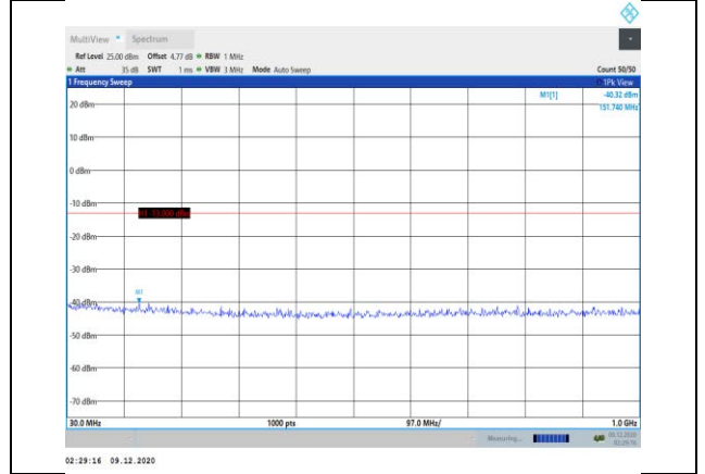
Band2-20MHz-QPSK-19100-1RB#0- Range1:30~1000MHz
