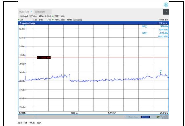
Band2-3MHz-16QAM-18900-1RB#0- Range2:1000~20000MHz
