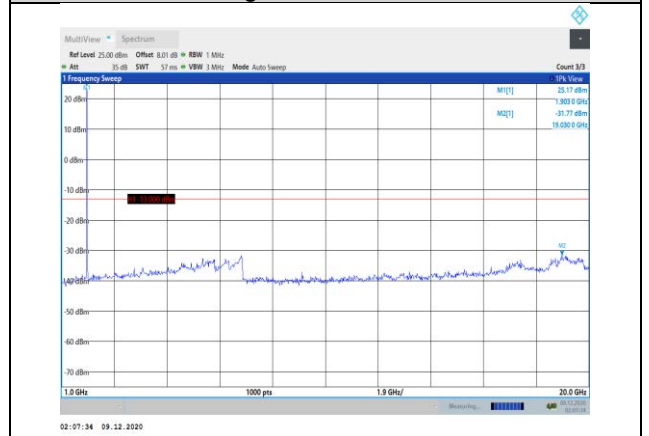
Band2-1.4MHz-16QAM-19193-1RB#0- Range2:1000~20000MHz
