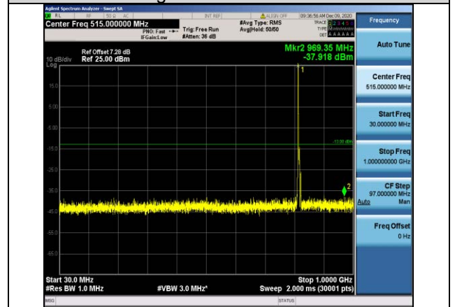
Band26-5MHz-16QAM-26740-1RB#0- Range1:30~1000MHz
