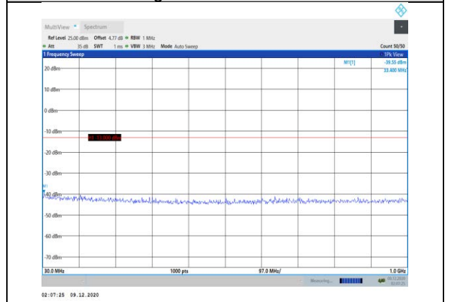
Band2-1.4MHz-16QAM-19193-1RB#0- Range1:30~1000MHz
