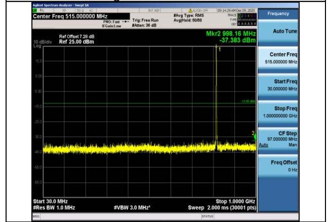
Band26-1.4MHz-16QAM-26740-1RB#0- Range1:30~1000MHz
