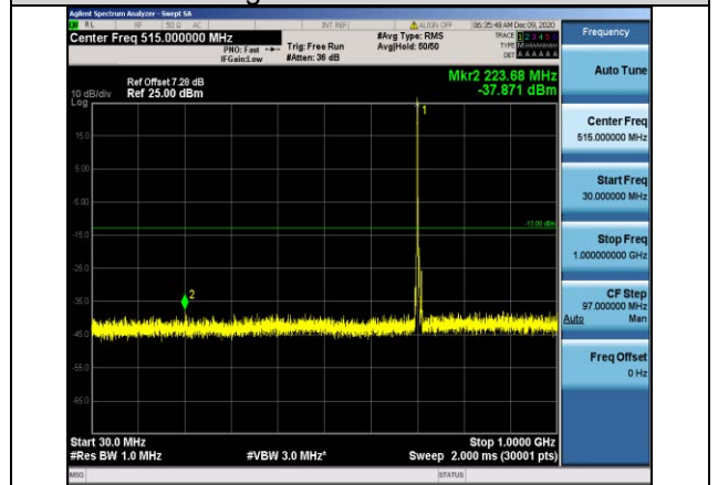
Band17-5MHz-QPSK-23790-1RB#0-Range1:30~1000MHz
