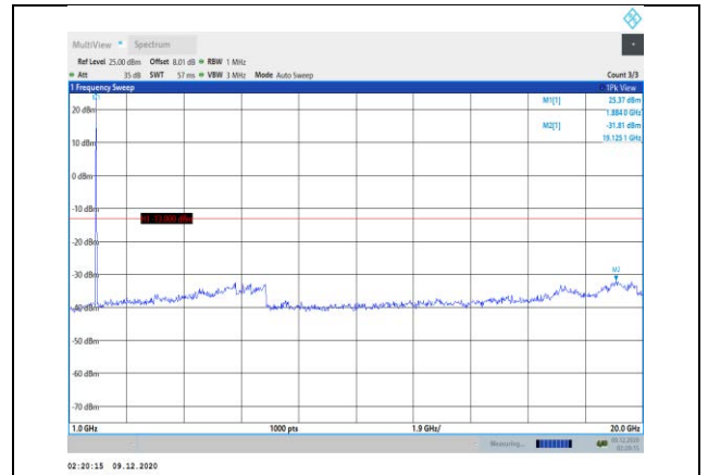
Band2-10MHz-QPSK-18900-1RB#0- Range2:1000~20000MHz
