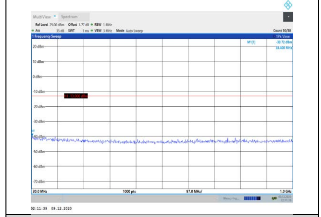
Band2-3MHz-16QAM-19185-1RB#0- Range1:30~1000MHz
