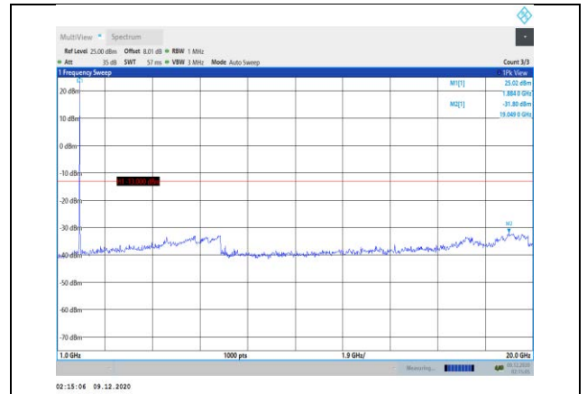
Band2-5MHz-16QAM-18900-1RB#0- Range2:1000~20000MHz
