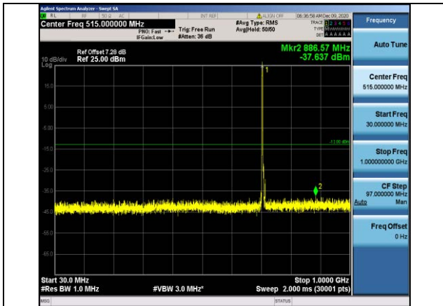
Band17-5MHz-QPSK-23825-1RB#0-Range1:30~1000MHz
