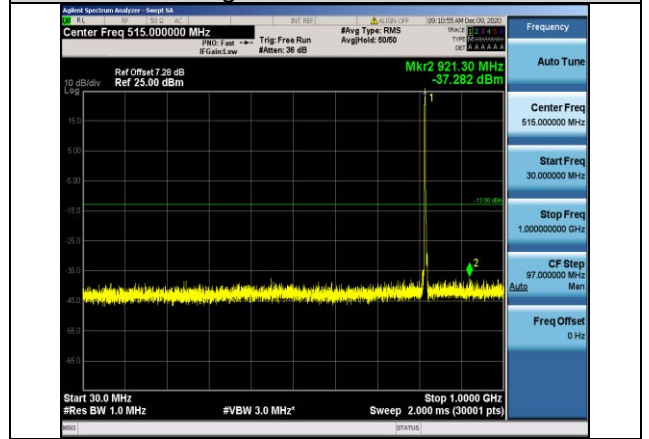
Band26-3MHz-16QAM-26740-1RB#0- Range1:30~1000MHz
