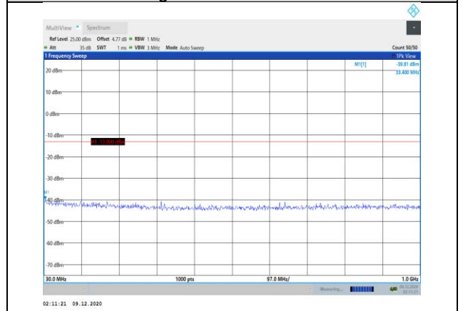
Band2-3MHz-QPSK-19185-1RB#0- Range1:30~1000MHz
