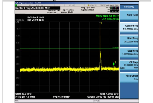
Band26-10MHz-16QAM-26740-1RB#0- Range1:30~1000MHz
