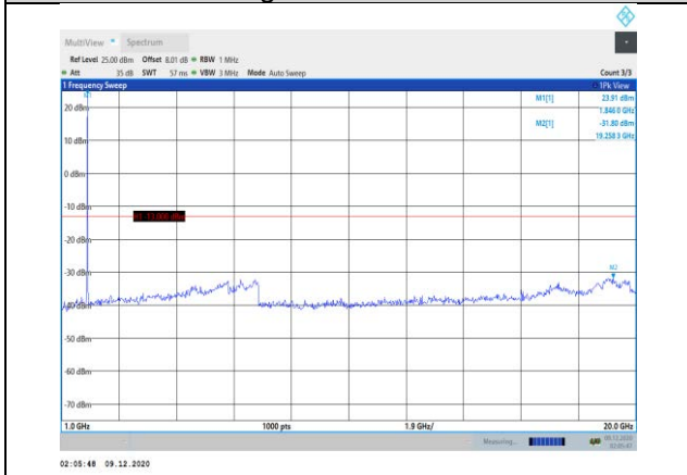
Band2-1.4MHz-16QAM-18607-1RB#0- Range2:1000~20000MHz
