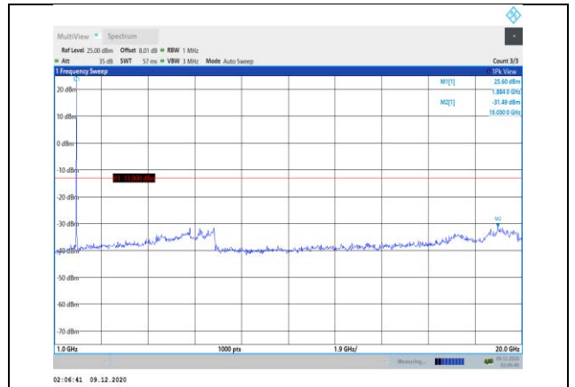
Band2-1.4MHz-16QAM-18900-1RB#0- Range2:1000~20000MHz
