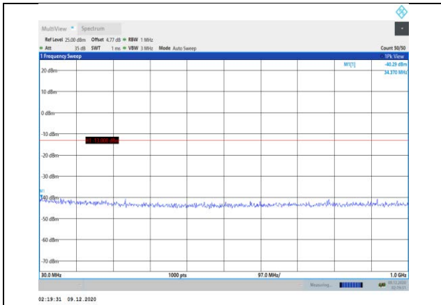
Band2-10MHz-16QAM-18650-1RB#0- Range1:30~1000MHz
