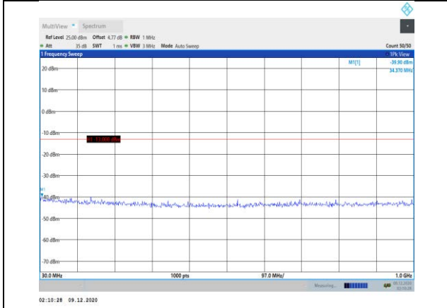
Band2-3MHz-QPSK-18900-1RB#0- Range1:30~1000MHz
