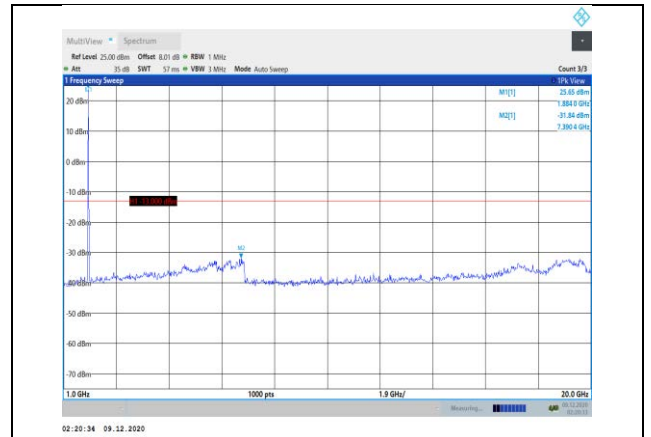
Band2-10MHz-16QAM-18900-1RB#0- Range2:1000~20000MHz
