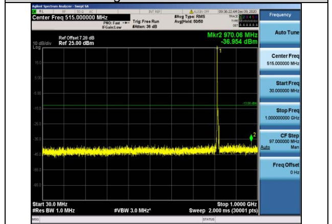
Band26-5MHz-QPSK-26740-1RB#0- Range1:30~1000MHz
