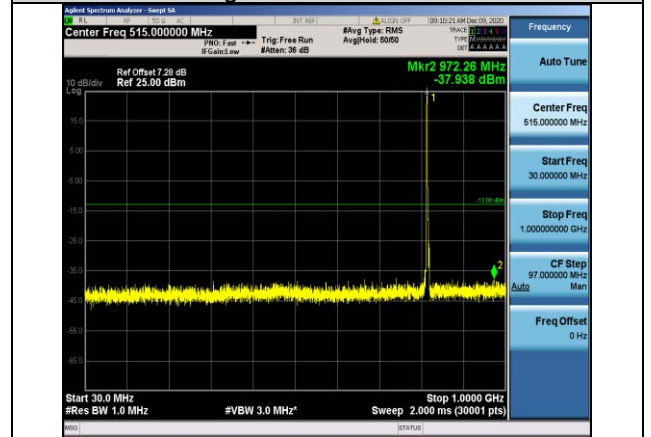
Band26-3MHz-QPSK-26740-1RB#0- Range1:30~1000MHz
