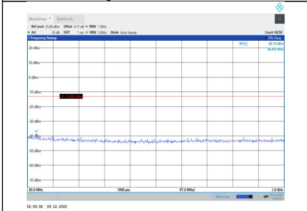
Band2-1.4MHz-16QAM-18900-1RB#0- Range1:30~1000MHz
