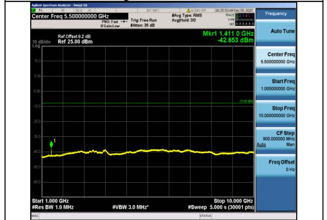
Band17-10MHz-16QAM-23790-1RB#0- Range2:1000~10000MHz
