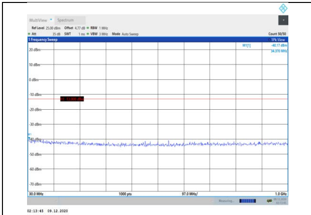
Band2-5MHz-QPSK-18625-1RB#0- Range1:30~1000MHz
