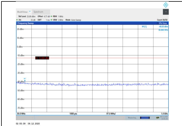
Band2-1.4MHz-16QAM-18607-1RB#0- Range1:30~1000MHz
