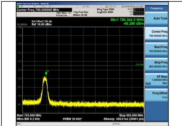
Band13-10MHz-16QAM-23230-1RB#0-Range4:793~805MHz
