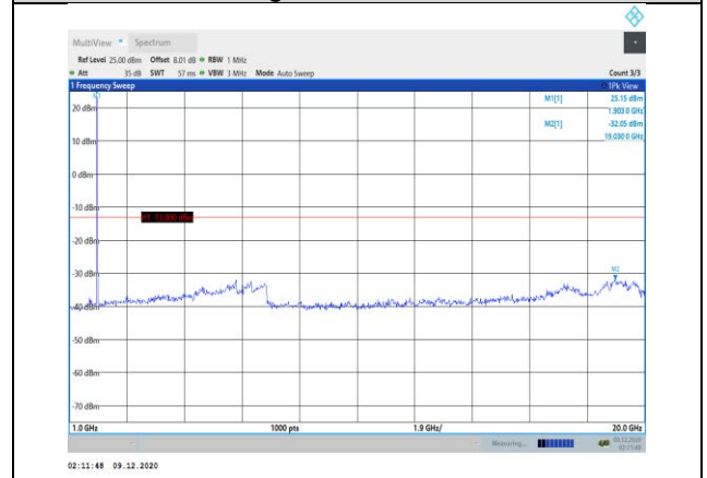
Band2-3MHz-16QAM-19185-1RB#0- Range2:1000~20000MHz
