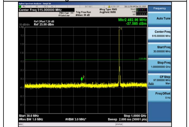
Band13-5MHz-16QAM-23230-1RB#0- Range1:30~1000MHz
