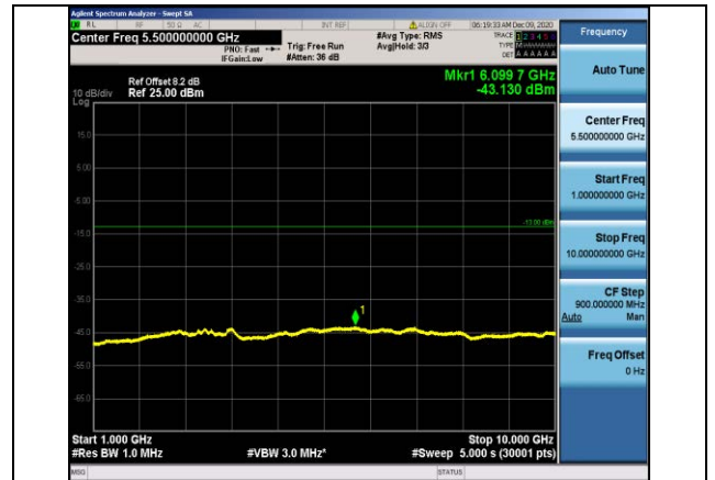
Band5-10MHz-16QAM-20525-1RB#0- Range2:1000~10000MHz
