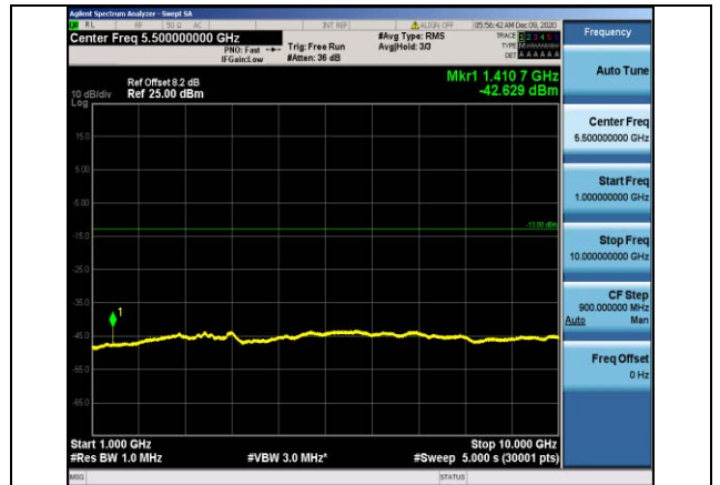
Band12-5MHz-QPSK-23095-1RB#0-Range2:1000~10000MHz
