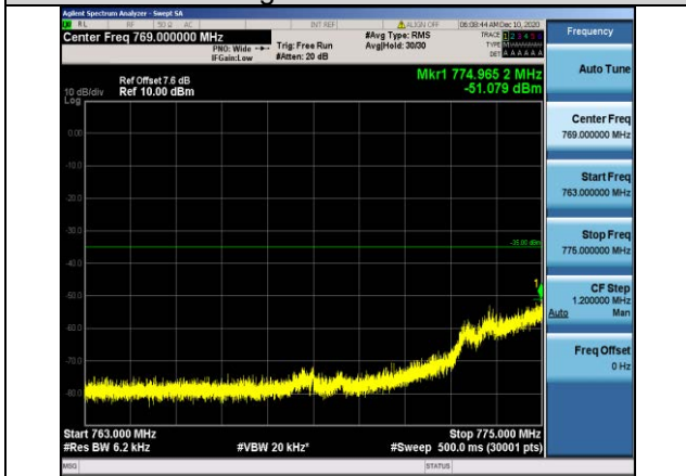
Band13-5MHz-QPSK-23205-1RB#0-Range3:763~775MHz
