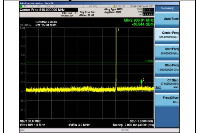
Band12-1.4MHz-16QAM-23173-1RB#0-Range1:30~1000MHz
