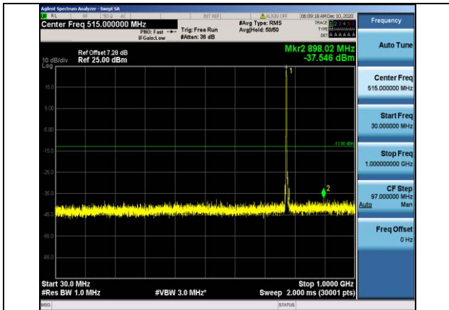
Band13-5MHz-16QAM-23205-1RB#0- Range1:30~1000MHz
