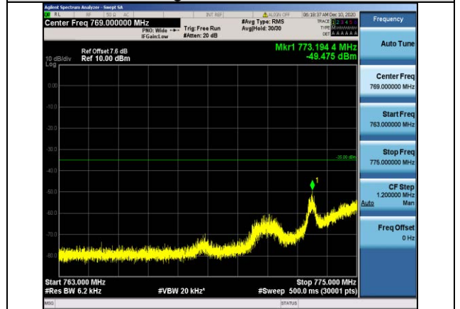
Band13-10MHz-16QAM-23230-1RB#0- Range3:763~775MHz
