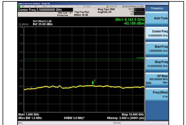
Band13-5MHz-QPSK-23205-1RB#0-Range2:1000~10000MHz
