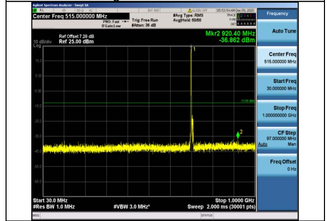
Band12-10MHz-QPSK-23130-1RB#0- Range1:30~1000MHz
