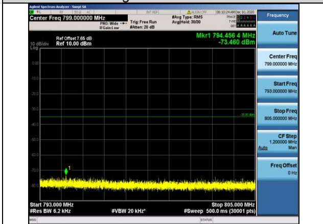
Band13-5MHz-16QAM-23205-1RB#0- Range4:793~805MHz
