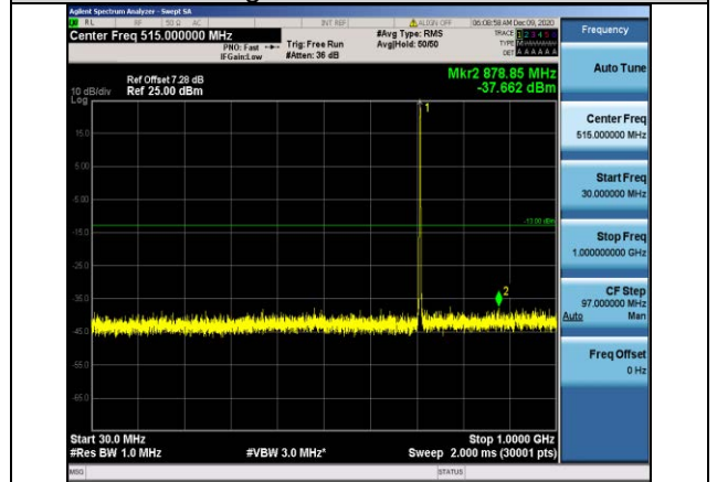
Band12-1.4MHz-QPSK-23173-1RB#0- Range1:30~1000MHz
