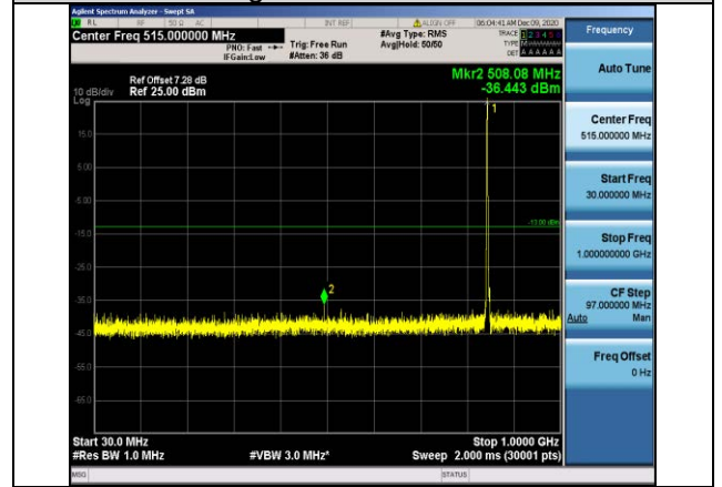
Band5-3MHz-QPSK-20635-1RB#0-Range1:30~1000MHz
