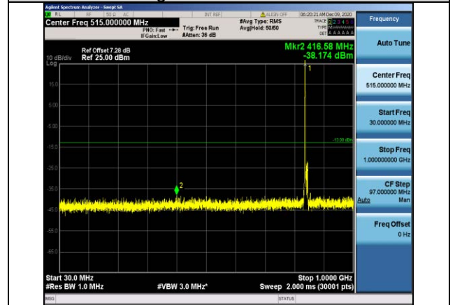
Band5-10MHz-16QAM-20600-1RB#0- Range1:30~1000MHz
