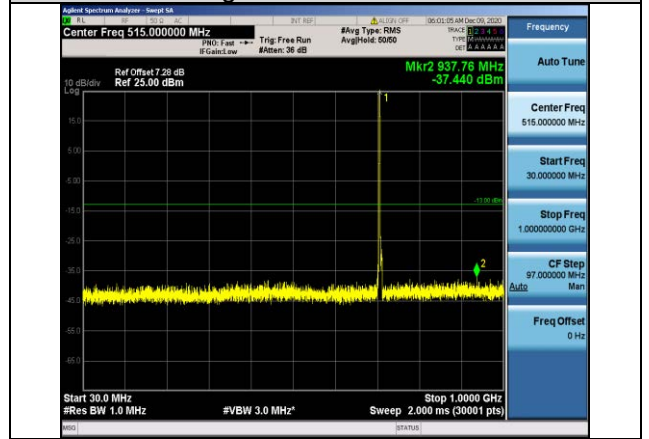
Band12-3MHz-QPSK-23165-1RB#0- Range1:30~1000MHz
