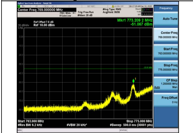
Band13-10MHz-QPSK-23230-1RB#0- Range3:763~775MHz
