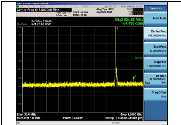
Band13-10MHz-QPSK-23230-1RB#0- Range1:30~1000MHz
