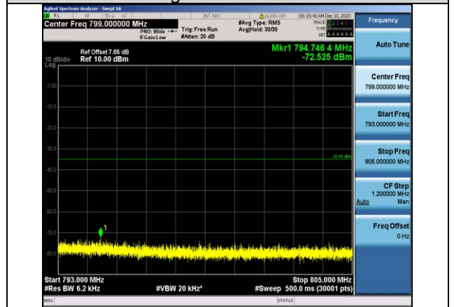
Band13-5MHz-16QAM-23255-1RB#0- Range4:793~805MHz
