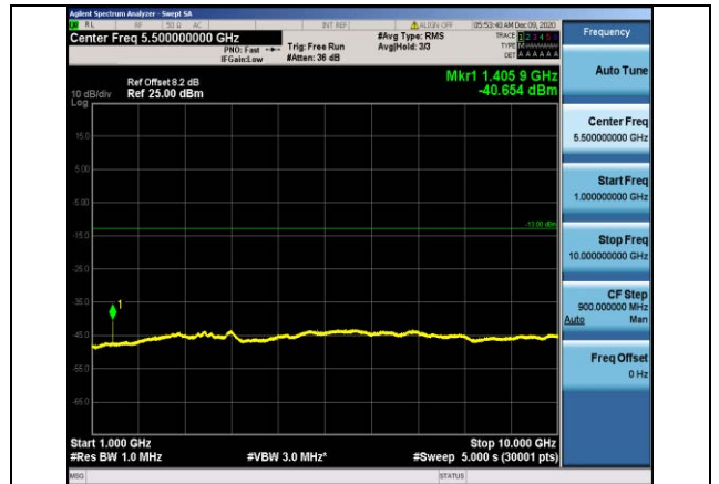
Band12-10MHz-16QAM-23095-1RB#0- Range2:1000~10000MHz
