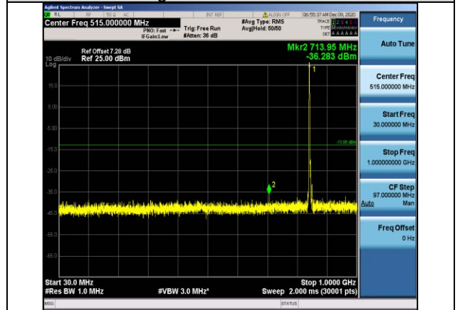
Band5-5MHz-QPSK-20625-1RB#0- Range1:30~1000MHz
