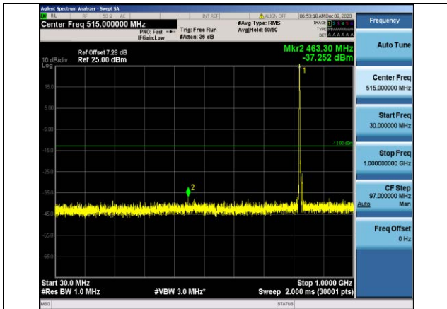
Band5-5MHz-QPSK-20425-1RB#0- Range1:30~1000MHz
