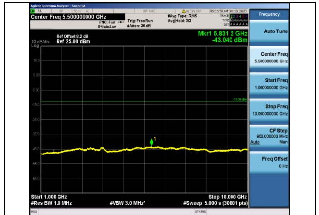
Band13-10MHz-QPSK-23230-1RB#0- Range2:1000~10000MHz
