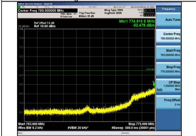
Band13-5MHz-16QAM-23205-1RB#0- Range3:763~775MHz
