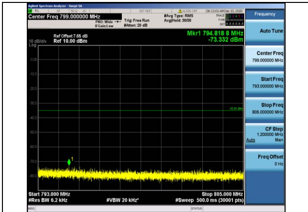
Band13-5MHz-16QAM-23230-1RB#0- Range4:793~805MHz
