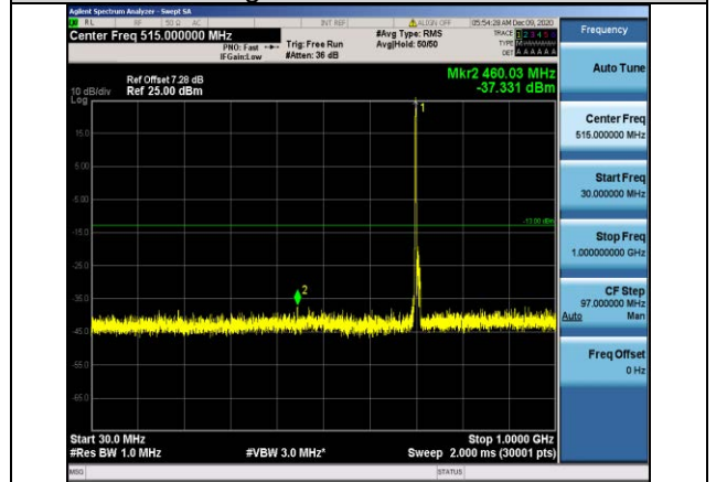
Band12-10MHz-16QAM-23130-1RB#0- Range1:30~1000MHz
