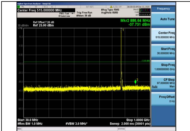
Band13-5MHz-QPSK-23205-1RB#0-Range1:30~1000MHz
