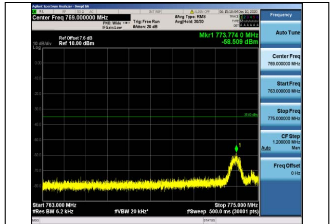
Band13-5MHz-16QAM-23255-1RB#0- Range3:763~775MHz
