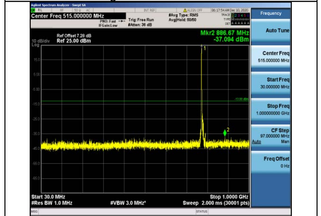
Band13-10MHz-16QAM-23230-1RB#0- Range1:30~1000MHz
