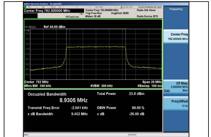
Band13-10MHz-QPSK-23230-50RB#0-8.9305
