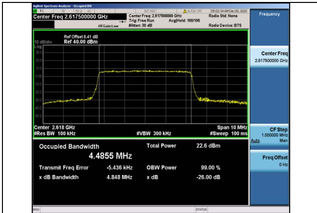
Band38-5MHz-16QAM-38225-25RB#0-4.4855
