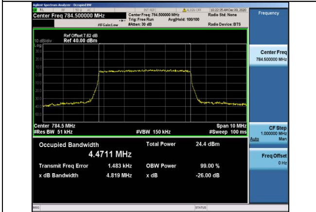
Band13-5MHz-16QAM-23255-25RB#0-4.4711
