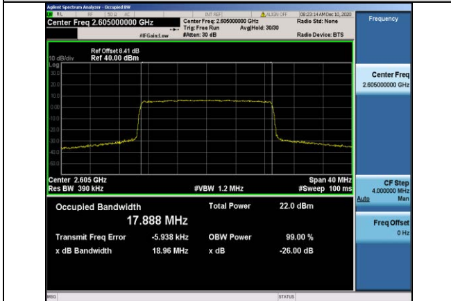
Band41-20MHz-QPSK-40740-100RB#0-17.888
