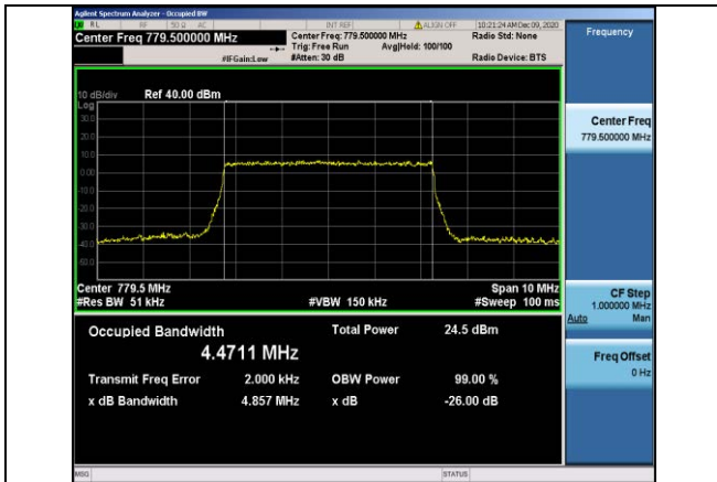
Band13-5MHz-16QAM-23205-25RB#0-4.4711
