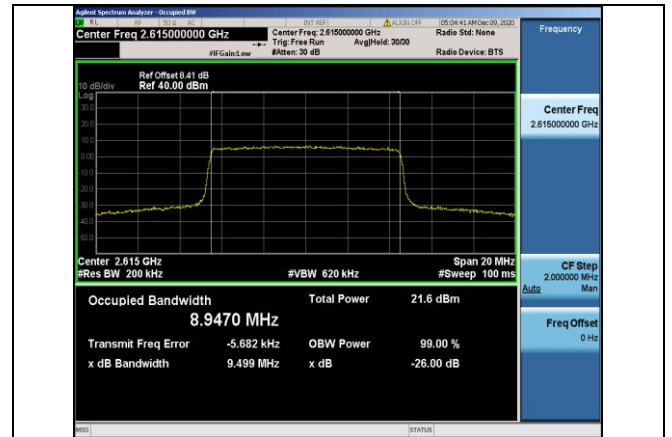
Band38-10MHz-QPSK-38200-50RB#0-8.9470
