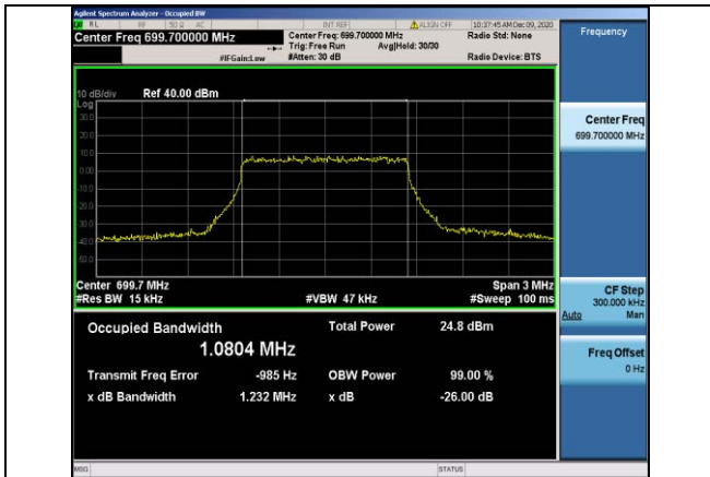
Band12-1.4MHz-16QAM-23017-6RB#0-1.0804
