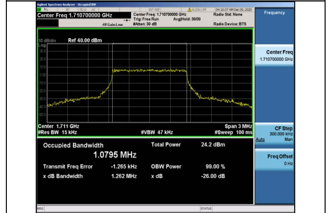
Band66-1.4MHz-16QAM-131979-6RB#0-1.0795
