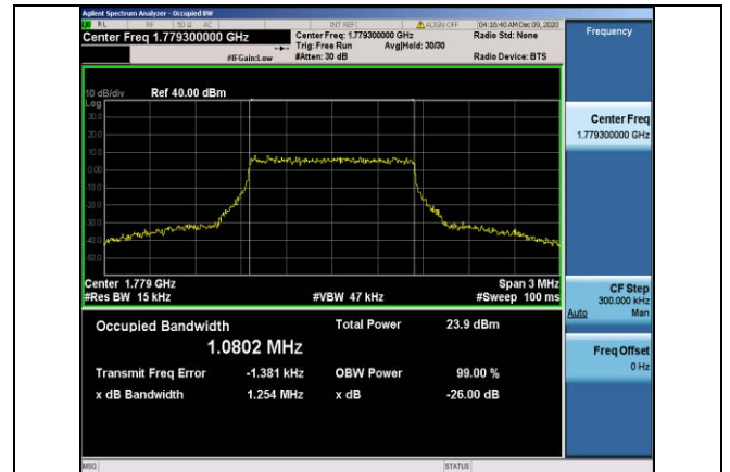
Band66-1.4MHz-QPSK-132665-6RB#0-1.0802
