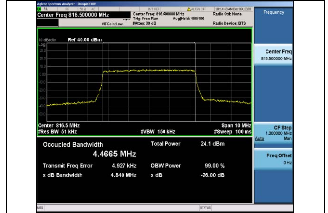
Band26-5MHz-QPSK-26715-25RB#0-4.4665
