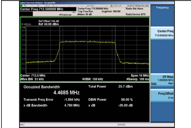
Band17-5MHz-QPSK-23825-25RB#0-4.4685
