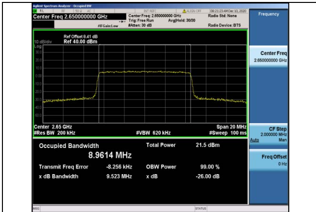
Band41-10MHz-16QAM-41190-50RB#0-8.9614
