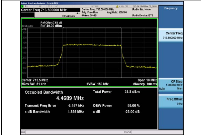
Band12-5MHz-16QAM-23155-25RB#0-4.4689
