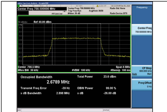
Band12-3MHz-16QAM-23025-15RB#0-2.6789
