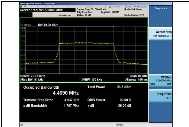
Band12-5MHz-16QAM-23035-25RB#0-4.4690
