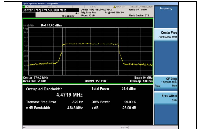
Band13-5MHz-QPSK-23205-25RB#0-4.4719
