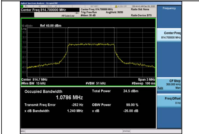
Band26-1.4MHz-16QAM-26697-6RB#0-1.0786
