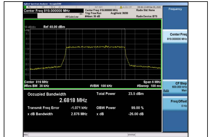
Band26-3MHz-16QAM-26740-15RB#0-2.6818
