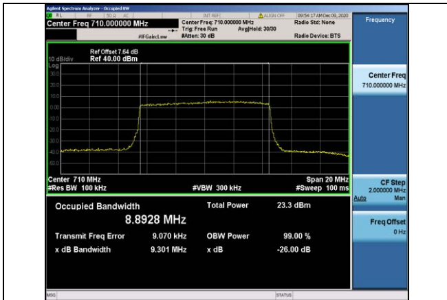
Band17-10MHz-QPSK-23790-50RB#0-8.8928
