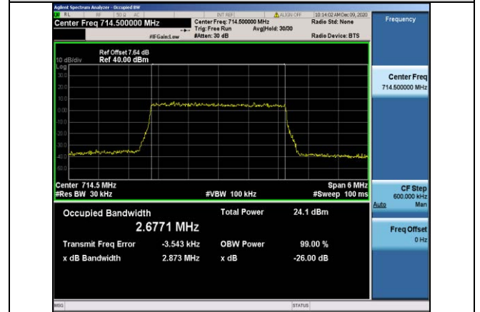
Band12-3MHz-QPSK-23165-15RB#0-2.6771
