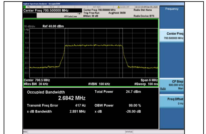
Band12-3MHz-QPSK-23025-15RB#0-2.6842
