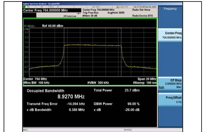
Band12-10MHz-QPSK-23060-50RB#0-8.9270
