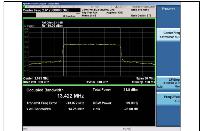
Band38-15MHz-QPSK-38175-75RB#0-13.422
