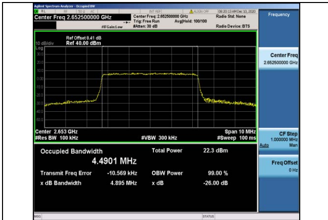
Band41-5MHz-16QAM-41215-25RB#0-4.4901
