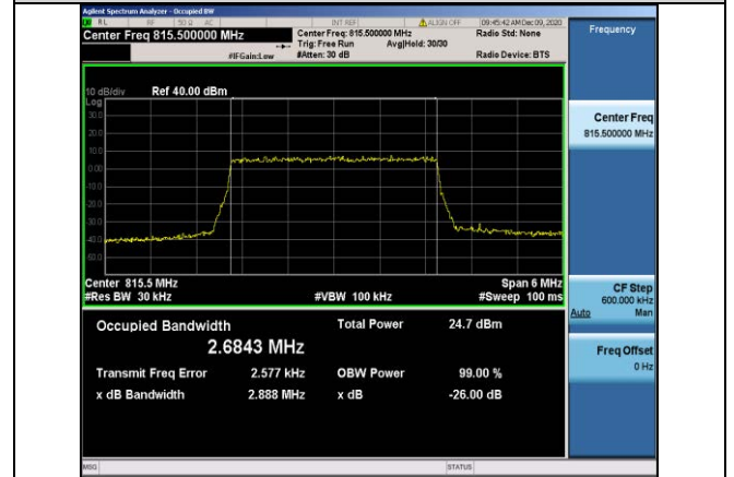
Band26-3MHz-QPSK-26705-15RB#0-2.6843
