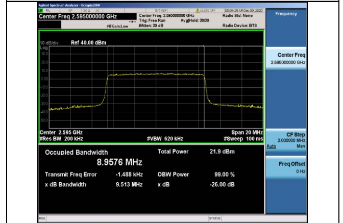
Band38-10MHz-16QAM-38000-50RB#0-8.9576
