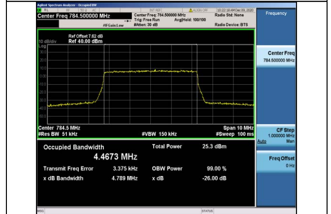
Band13-5MHz-QPSK-23255-25RB#0-4.4673
