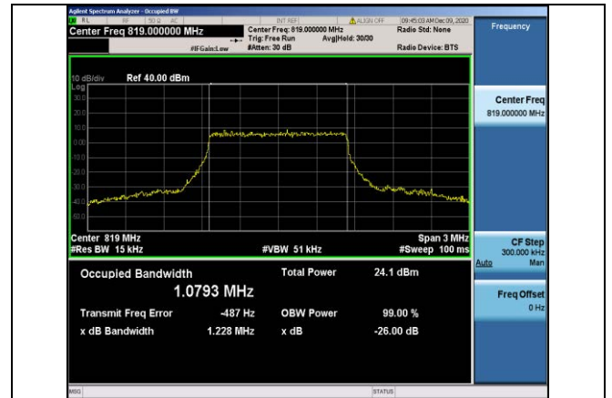
Band26-1.4MHz-16QAM-26740-6RB#0-1.0793
