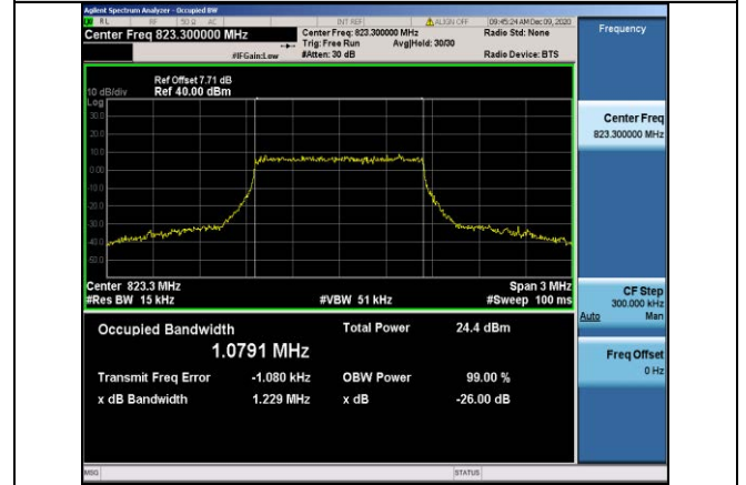
Band26-1.4MHz-16QAM-26783-6RB#0-1.0791
