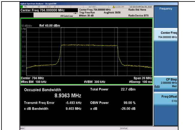
Band12-10MHz-16QAM-23060-50RB#0-8.9363
