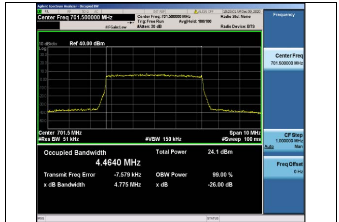
Band12-5MHz-QPSK-23035-25RB#0-4.4640
