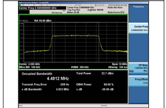
Band38-5MHz-16QAM-38000-25RB#0-4.4912
