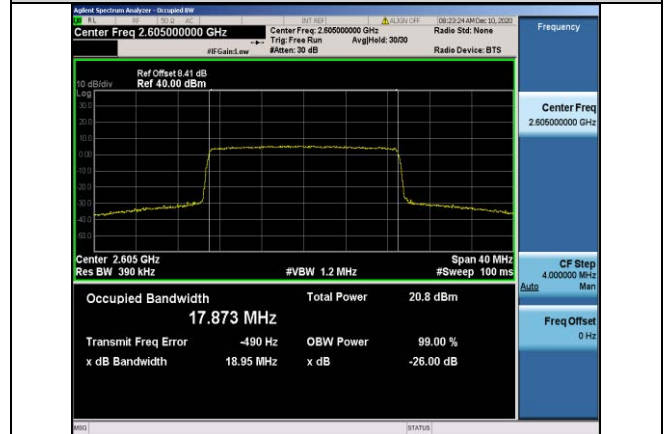
Band41-20MHz-16QAM-40740-100RB#0-17.873
