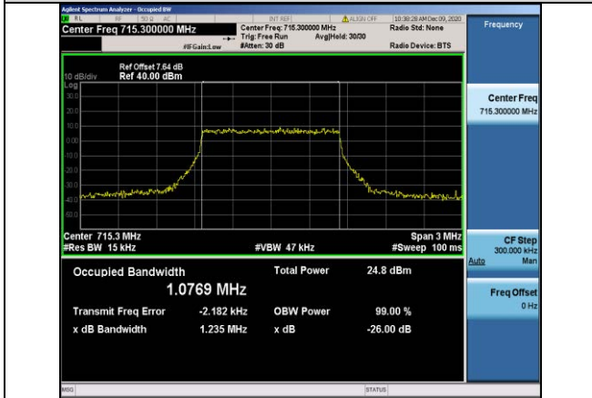
Band12-1.4MHz-16QAM-23173-6RB#0-1.0769
