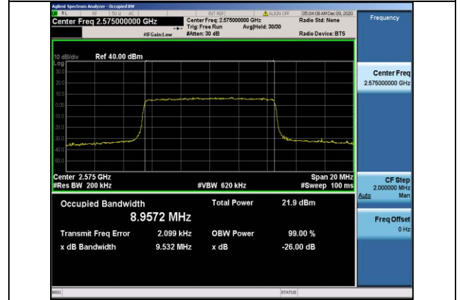
Band38-10MHz-16QAM-37800-50RB#0-8.9572
