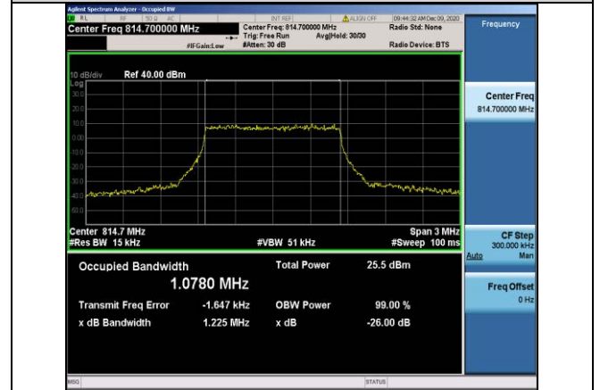
Band26-1.4MHz-QPSK-26697-6RB#0-1.0780
