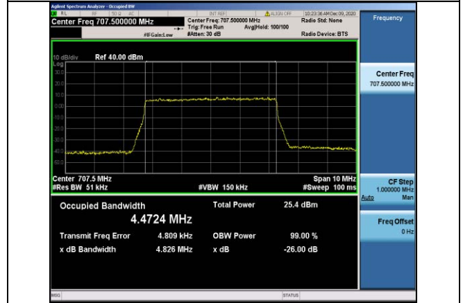
Band12-5MHz-QPSK-23095-25RB#0-4.4724
