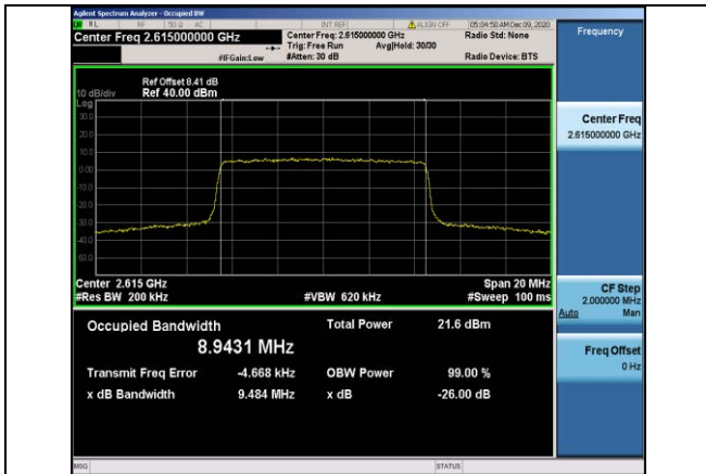
Band38-10MHz-16QAM-38200-50RB#0-8.9431
