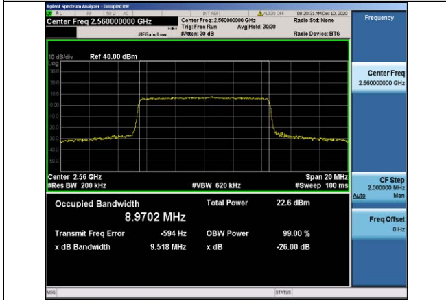
Band41-10MHz-QPSK-40290-50RB#0-8.9702
