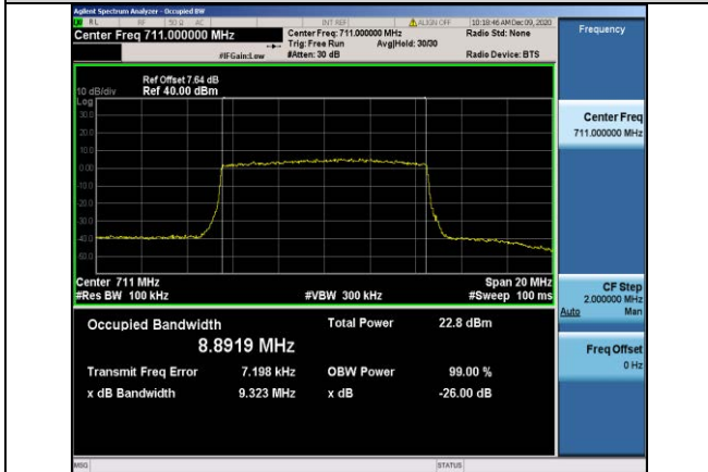
Band12-10MHz-16QAM-23130-50RB#0-8.8919
