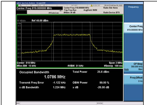
Band26-1.4MHz-QPSK-26740-6RB#0-1.0786
