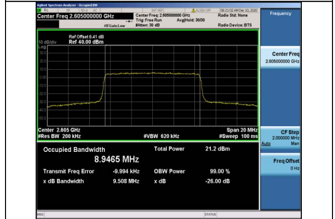
Band41-10MHz-16QAM-40740-50RB#0-8.9465
