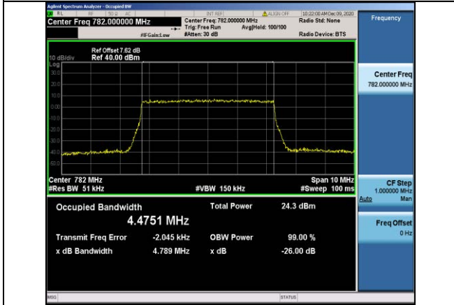
Band13-5MHz-16QAM-23230-25RB#0-4.4751
