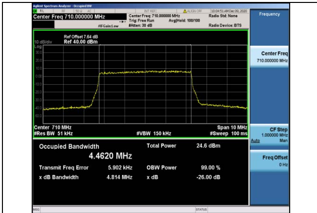
Band17-5MHz-QPSK-23790-25RB#0-4.4620
