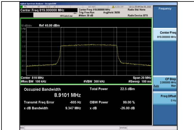
Band26-10MHz-16QAM-26740-50RB#0-8.9101
