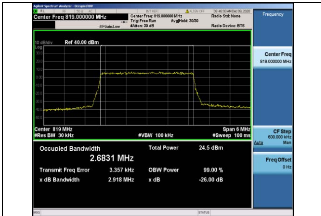
Band26-3MHz-QPSK-26740-15RB#0-2.6831
