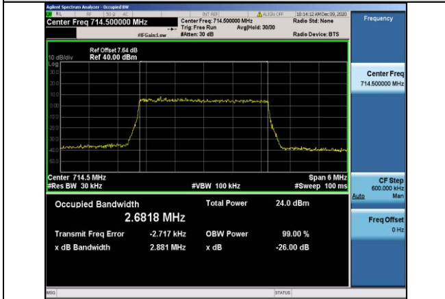
Band12-3MHz-16QAM-23165-15RB#0-2.6818
