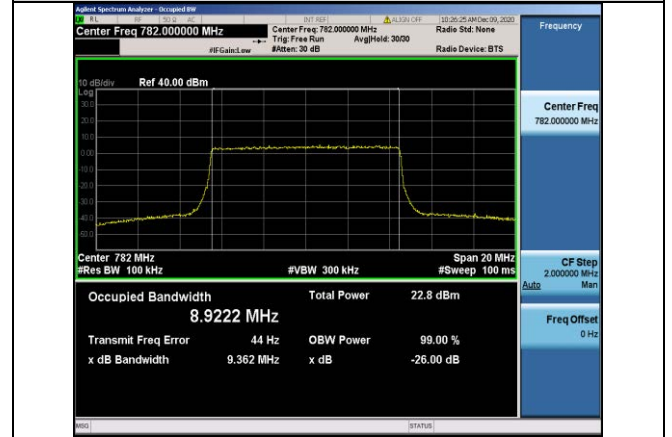
Band13-10MHz-16QAM-23230-50RB#0-8.9222
