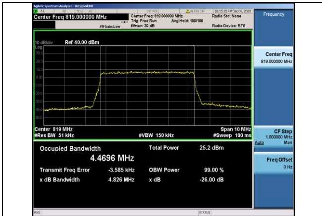
Band26-5MHz-QPSK-26740-25RB#0-4.4696
