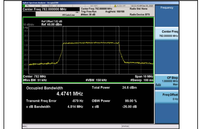
Band13-5MHz-QPSK-23230-25RB#0-4.4741
