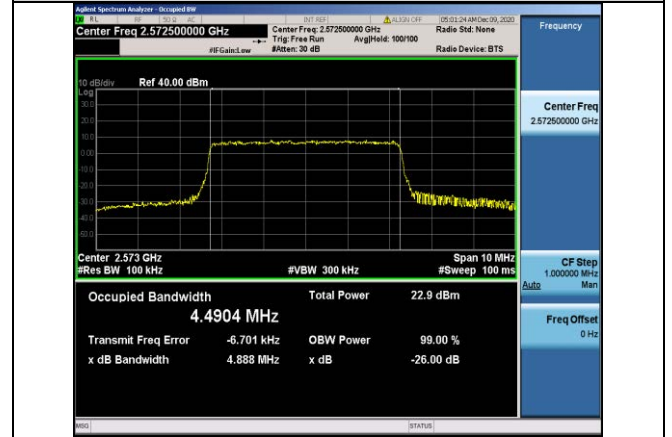
Band38-5MHz-16QAM-37775-25RB#0-4.4904
