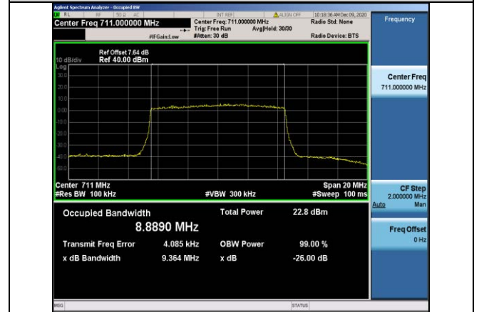
Band12-10MHz-QPSK-23130-50RB#0-8.8890
