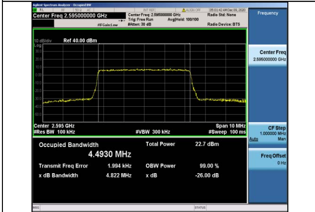
Band38-5MHz-QPSK-38000-25RB#0-4.4930
