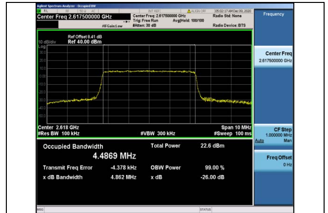
Band38-5MHz-QPSK-38225-25RB#0-4.4869
