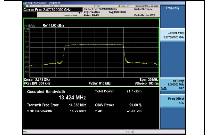
Band38-15MHz-16QAM-37825-75RB#0-13.424
