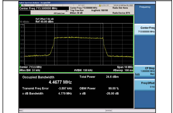
Band12-5MHz-QPSK-23155-25RB#0-4.4677
