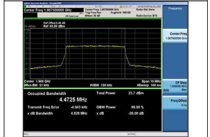
Band2-5MHz-QPSK-19175-25RB#0-4.4725
