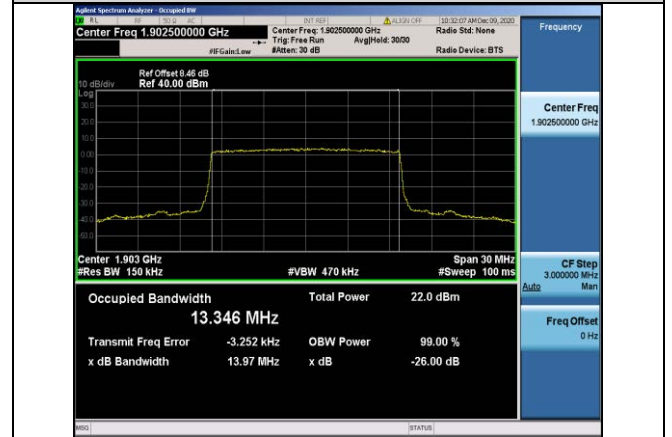
Band2-15MHz-QPSK-19125-75RB#0-13.346
