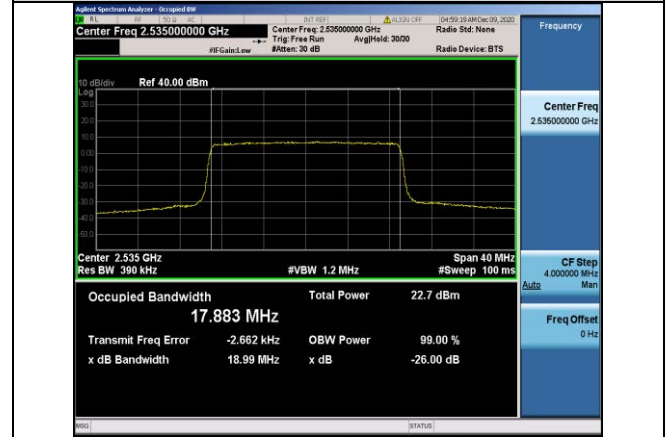
Band7-20MHz-QPSK-21100-100RB#0-17.883
