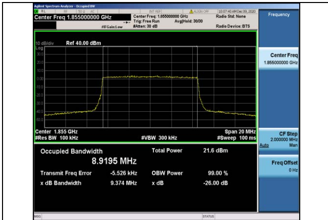
Band2-10MHz-16QAM-18650-50RB#0-8.9195
