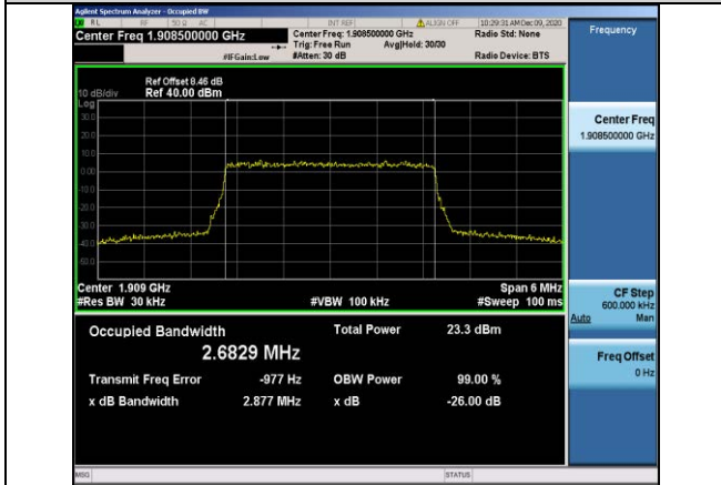
Band2-3MHz-16QAM-19185-15RB#0-2.6829
