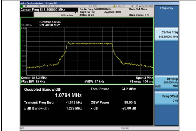
Band5-1.4MHz-16QAM-20643-6RB#0-1.0784
