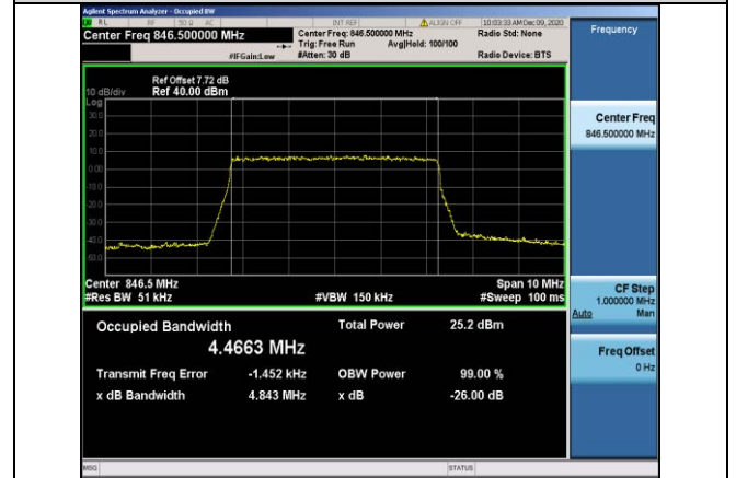
Band5-5MHz-QPSK-20625-25RB#0-4.4663
