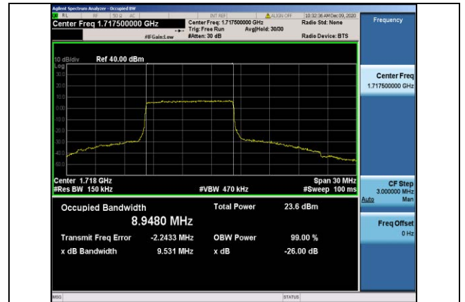
Band4-15MHz-QPSK-20025-75RB#0-8.9480
