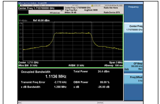
Band4-1.4MHz-QPSK-19957-6RB#0-1.1136
