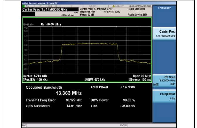
Band4-15MHz-QPSK-20325-75RB#0-13.363
