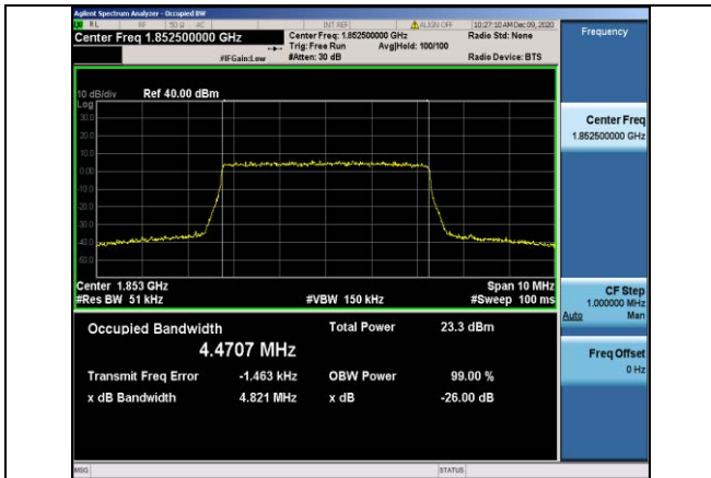
Band2-5MHz-16QAM-18625-25RB#0-4.4707
