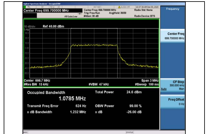
Band12-1.4MHz-QPSK-23017-6RB#0-1.0785
