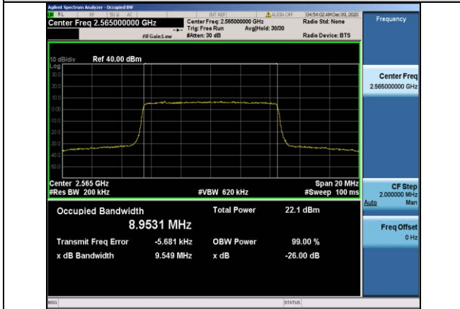
Band7-10MHz-16QAM-21400-50RB#0-8.9531
