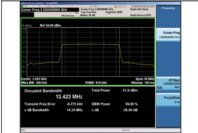
Band7-15MHz-16QAM-21375-75RB#0-13.423
