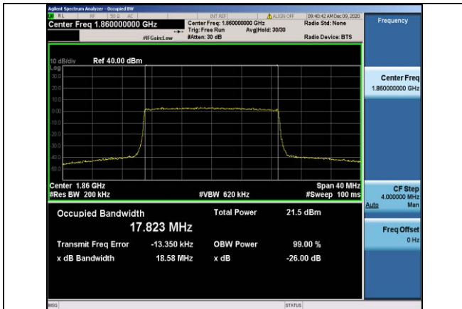
Band2-20MHz-16QAM-18700-100RB#0-17.823
