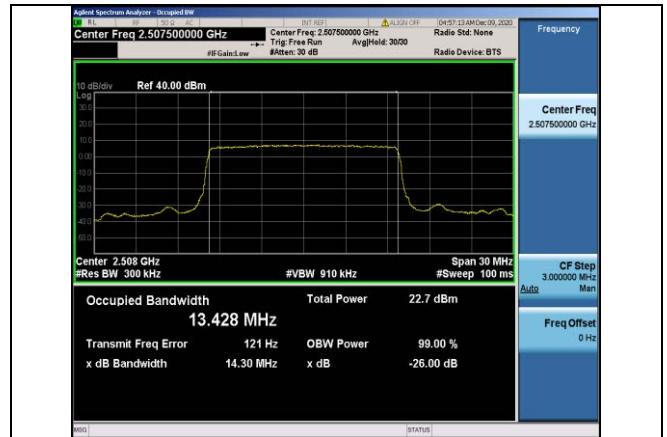
Band7-15MHz-QPSK-20825-75RB#0-13.428
