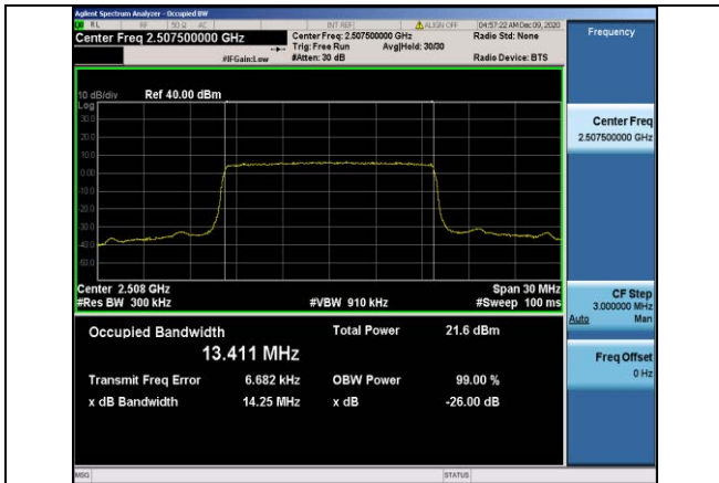
Band7-15MHz-16QAM-20825-75RB#0-13.411
