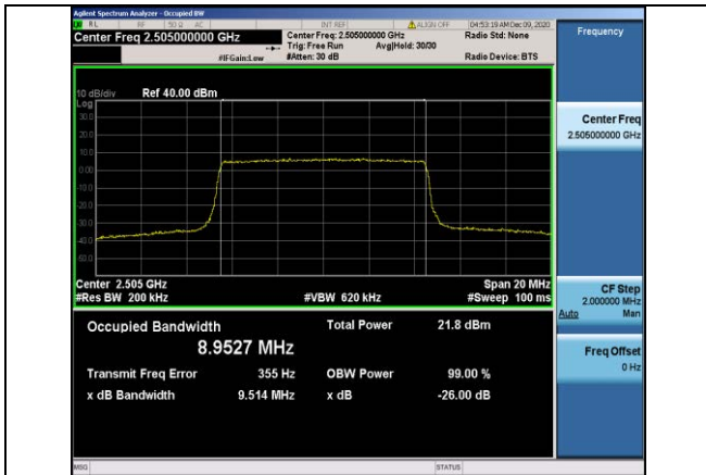
Band7-10MHz-16QAM-20800-50RB#0-8.9527
