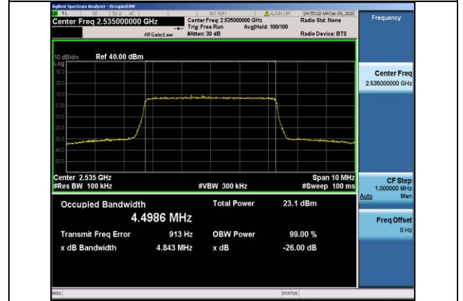
Band7-5MHz-QPSK-21100-25RB#0-4.4986
