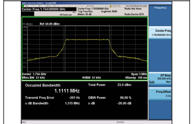
Band4-1.4MHz-QPSK-20393-6RB#0-1.1111
