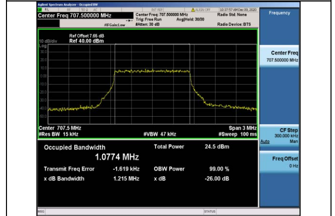
Band12-1.4MHz-QPSK-23095-6RB#0-1.0774
