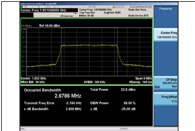
Band2-3MHz-16QAM-18615-15RB#0-2.6786
