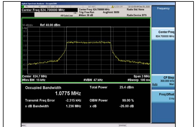
Band5-1.4MHz-QPSK-20407-6RB#0-1.0775
