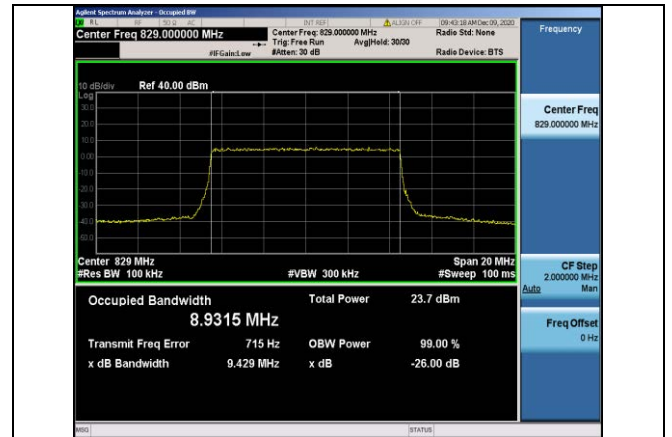
Band5-10MHz-QPSK-20450-50RB#0-8.9315
