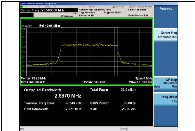
Band5-3MHz-16QAM-20415-15RB#0-2.6870
