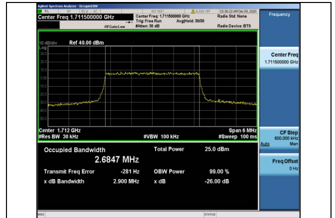
Band4-3MHz-QPSK-19965-15RB#0-2.6847
