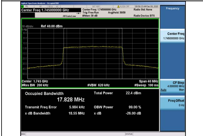
Band4-20MHz-16QAM-20300-100RB#0-17.828
