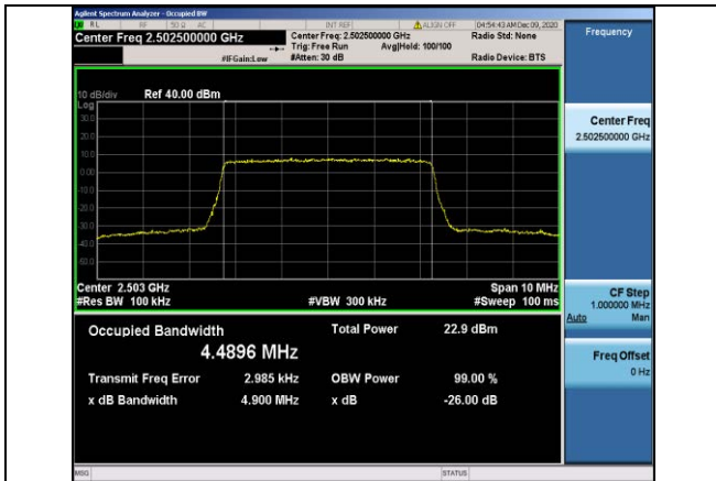
Band7-5MHz-16QAM-20775-25RB#0-4.4896
