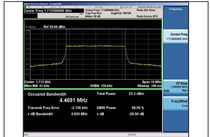
Band4-5MHz-QPSK-19975-25RB#0-4.4691
