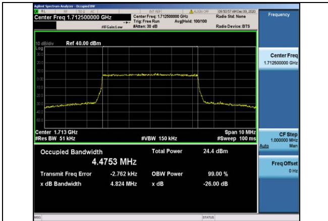
Band4-5MHz-16QAM-19975-25RB#0-4.4753
