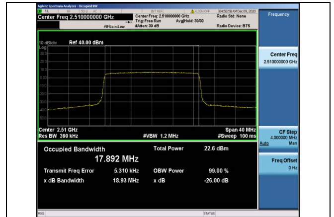
Band7-20MHz-QPSK-20850-100RB#0-17.892
