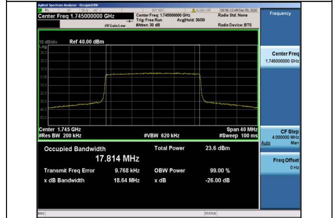
Band4-20MHz-QPSK-20300-100RB#0-17.814
