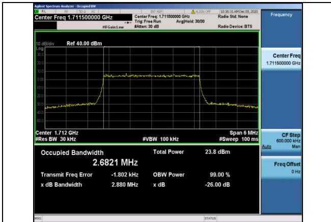
Band4-3MHz-16QAM-19965-15RB#0-2.6821
