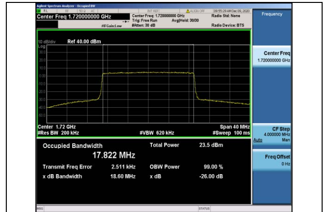
Band4-20MHz-QPSK-20050-100RB#0-17.822
