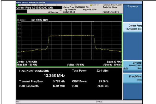
Band4-15MHz-16QAM-20325-75RB#0-13.356
