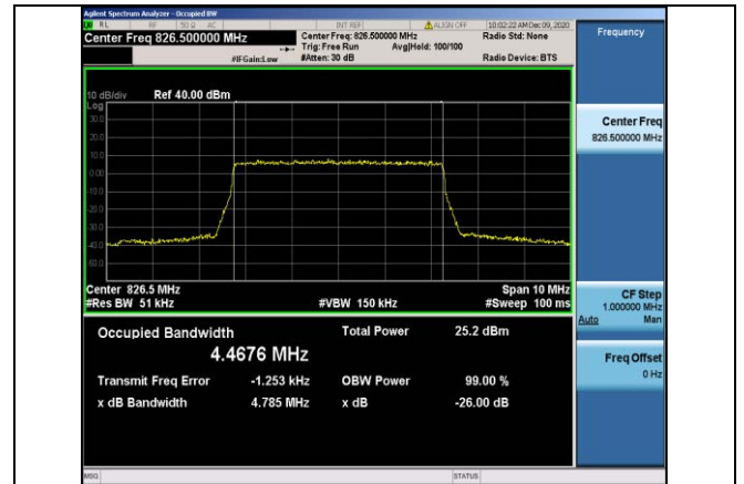
Band5-5MHz-QPSK-20425-25RB#0-4.4676
