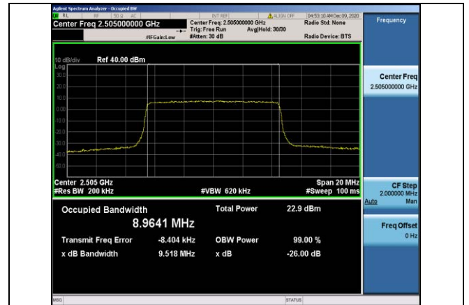
Band7-10MHz-QPSK-20800-50RB#0-8.9641
