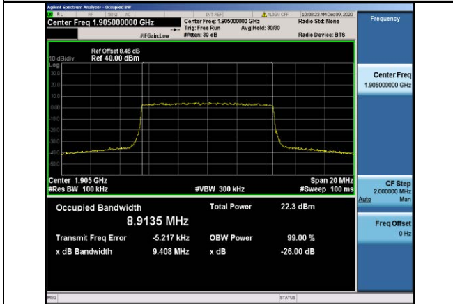
Band2-10MHz-16QAM-19150-50RB#0-8.9135
