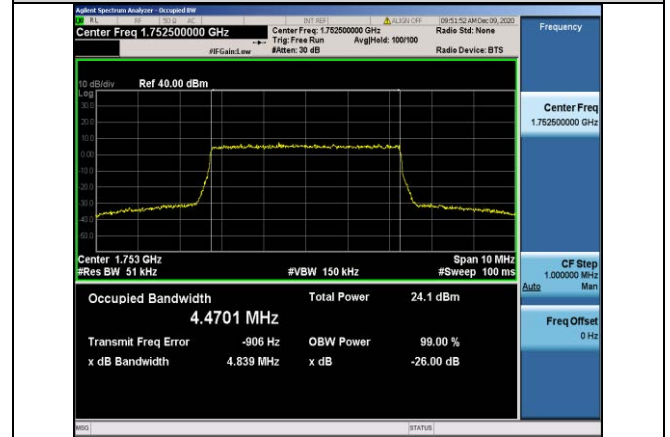
Band4-5MHz-QPSK-20375-25RB#0-4.4701
