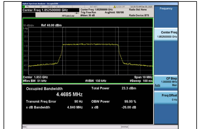
Band2-5MHz-QPSK-18625-25RB#0-4.4685
