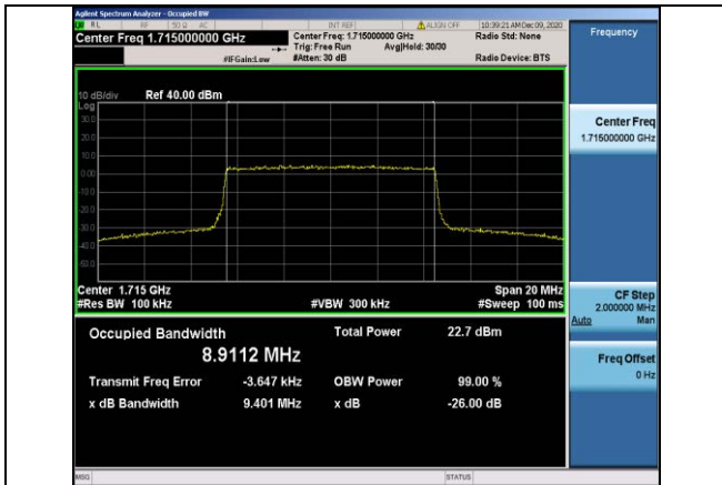
Band4-10MHz-16QAM-20000-50RB#0-8.9112
