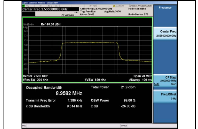
Band7-10MHz-QPSK-21100-50RB#0-8.9582
