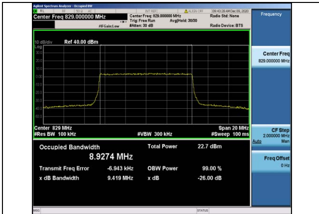
Band5-10MHz-16QAM-20450-50RB#0-8.9274
