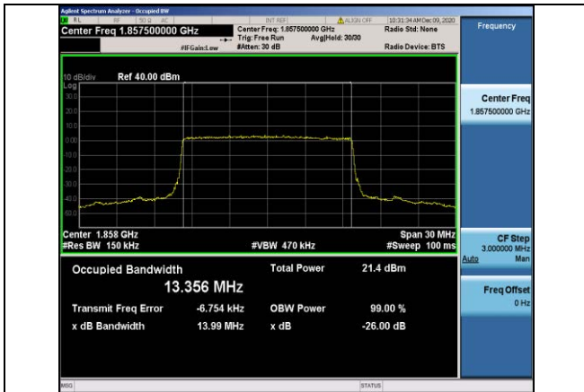
Band2-15MHz-16QAM-18675-75RB#0-13.356
