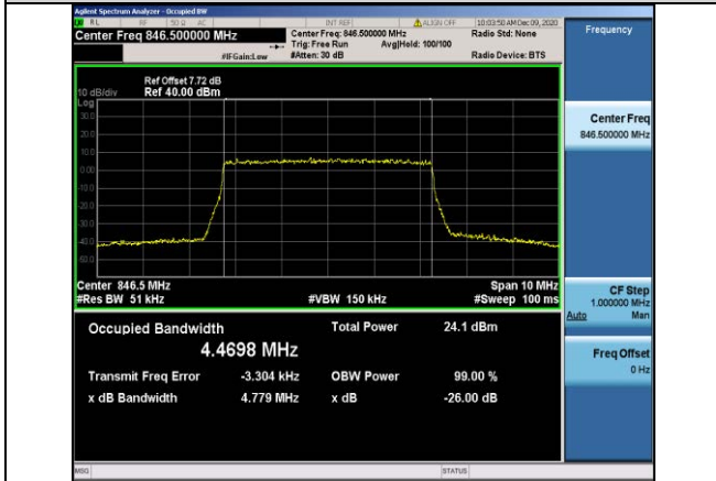
Band5-5MHz-16QAM-20625-25RB#0-4.4698
