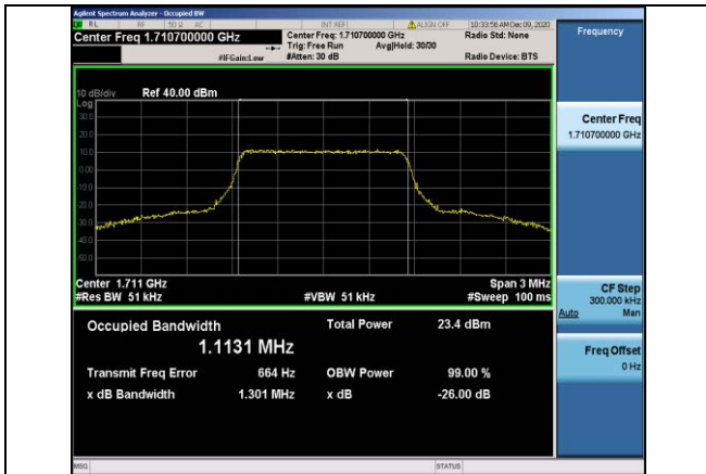
Band4-1.4MHz-16QAM-19957-6RB#0-1.1131
