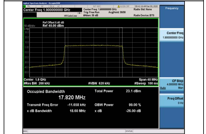
Band2-20MHz-QPSK-19100-100RB#0-17.820
