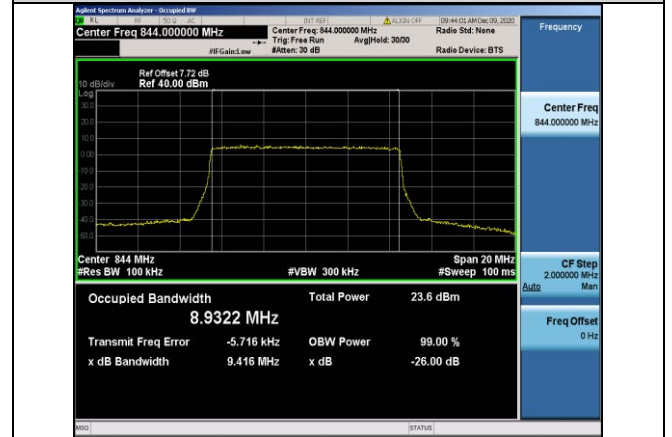
Band5-10MHz-QPSK-20600-50RB#0-8.9322
