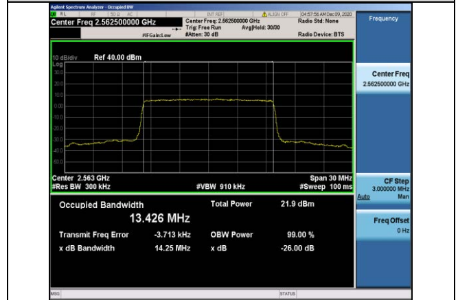
Band7-15MHz-QPSK-21375-75RB#0-13.426
