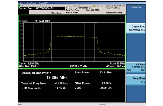
Band2-15MHz-QPSK-18675-75RB#0-13.365
