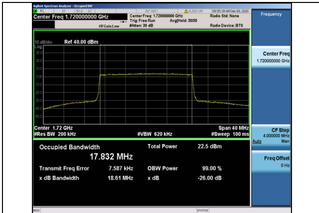
Band4-20MHz-16QAM-20050-100RB#0-17.832
