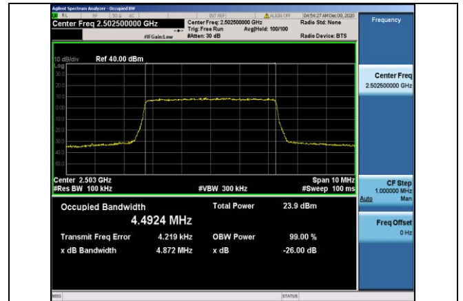
Band7-5MHz-QPSK-20775-25RB#0-4.4924
