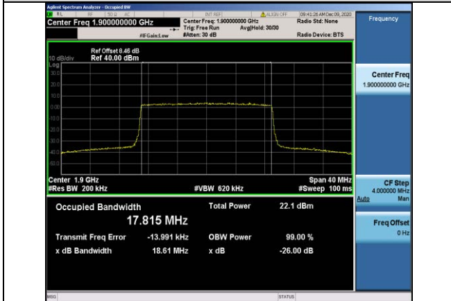
Band2-20MHz-16QAM-19100-100RB#0-17.815
