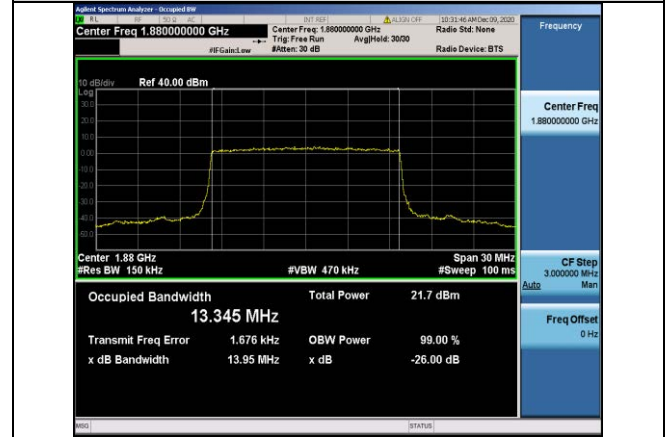
Band2-15MHz-QPSK-18900-75RB#0-13.345
