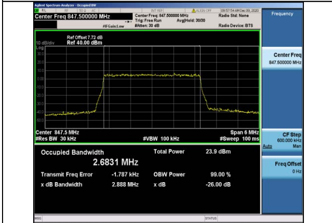
Band5-3MHz-16QAM-20635-15RB#0-2.6831
