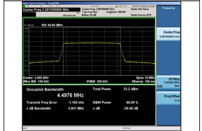
Band7-5MHz-QPSK-21425-25RB#0-4.4976
