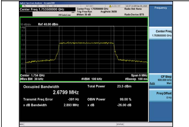
Band4-3MHz-16QAM-20385-15RB#0-2.6799
