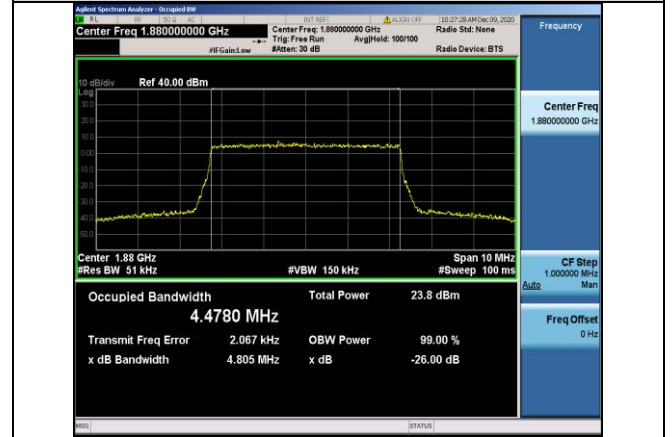
Band2-5MHz-QPSK-18900-25RB#0-4.4780
