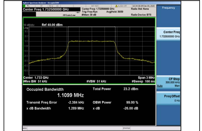
Band4-1.4MHz-QPSK-20175-6RB#0-1.1099
