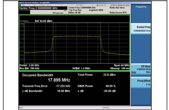
Band7-20MHz-QPSK-21350-100RB#0-17.895
