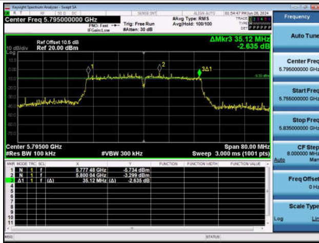
11AC40SISO-Ant1-5795-PASS
