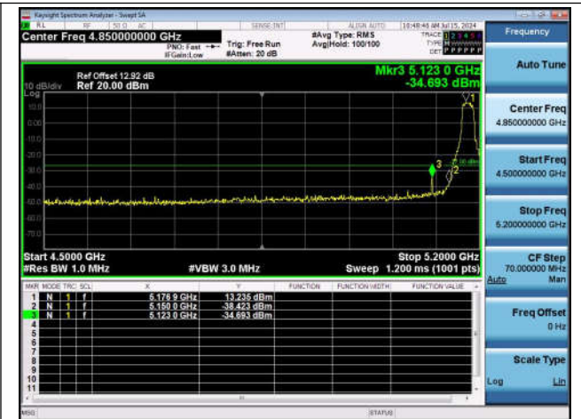
11N20SISO-Ant1-5180-PASS
