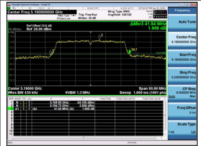
11N40SISO-Ant1-5190-26dB EBW
