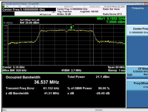
11N40SISO-Ant1-5190-99% OBW
