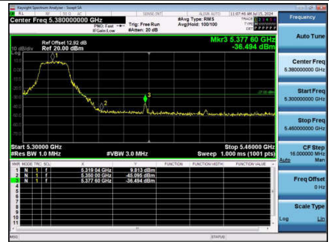
11AC20SISO-Ant1-5320-PASS
