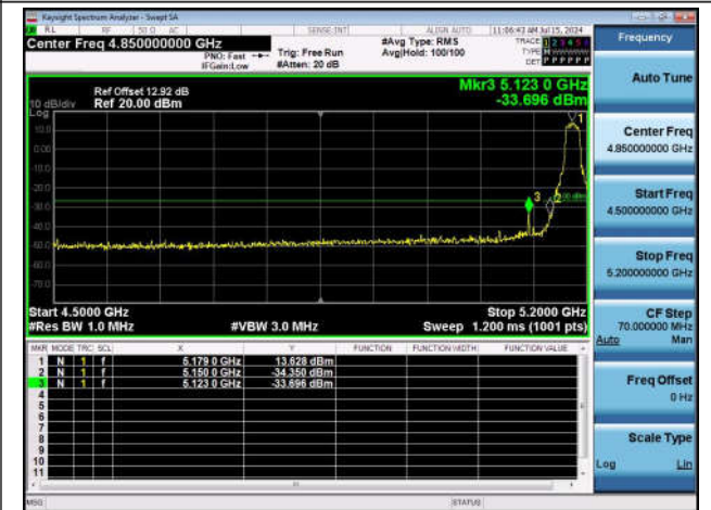
11AC20SISO-Ant1-5180-PASS
