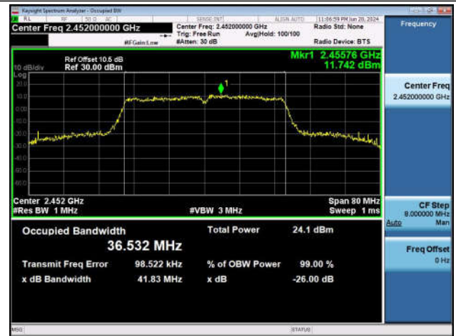
11N40SISO-Ant1-2452
