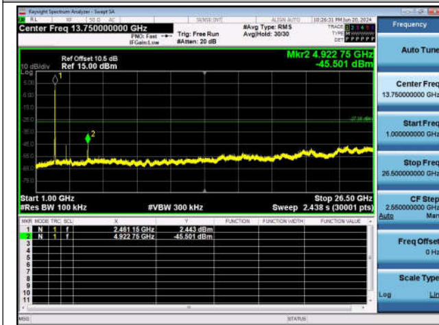
11N20SISO-Ant1-2462-1000~26500-PASS
