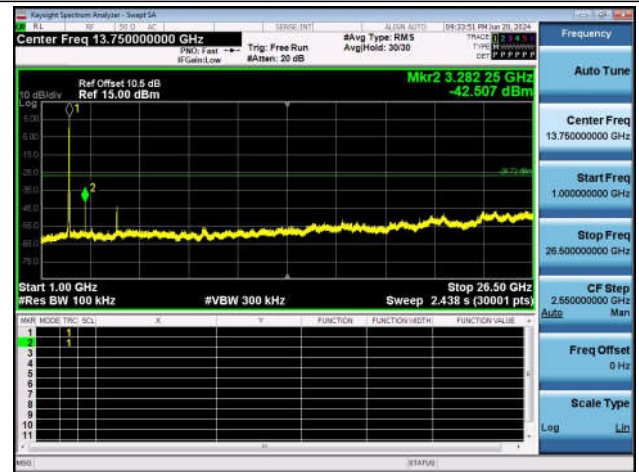
11G-Ant1-2462-1000~26500-PASS
