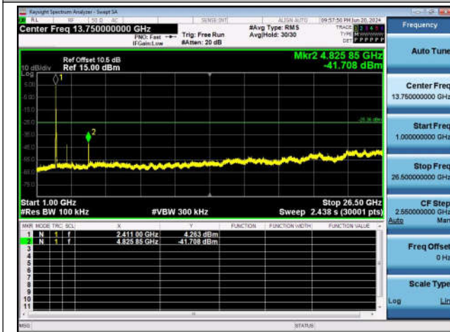
11N20SISO-Ant1-2412-1000~26500-PASS
