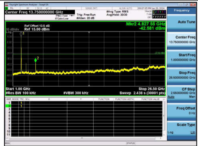
11G-Ant1-2412-1000~26500-PASS
