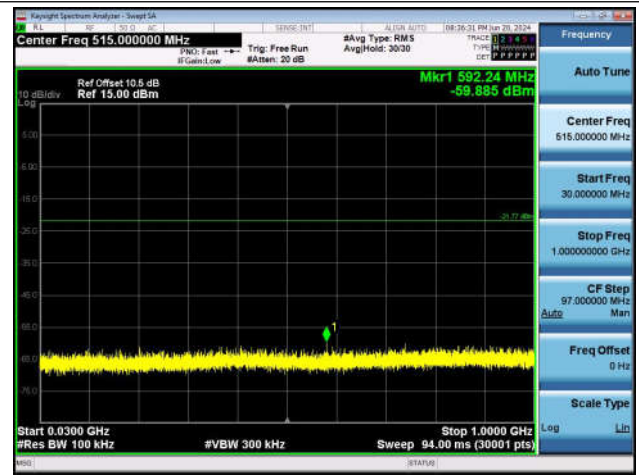
11B-Ant1-2462-30~1000-PASS
