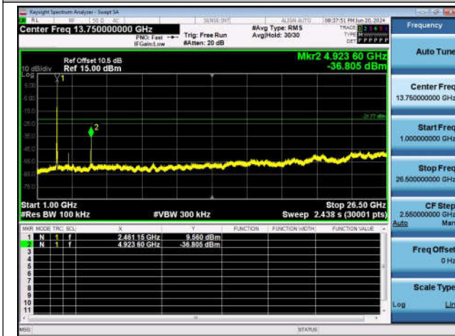
11B-Ant1-2462-1000~26500-PASS
