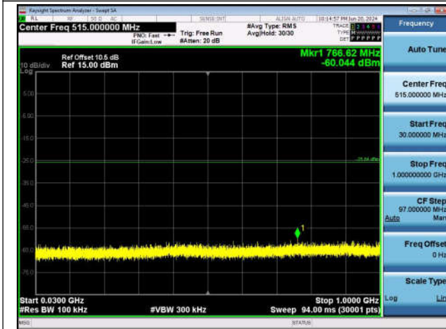
11N20SISO-Ant1-2437-30~1000-PASS
