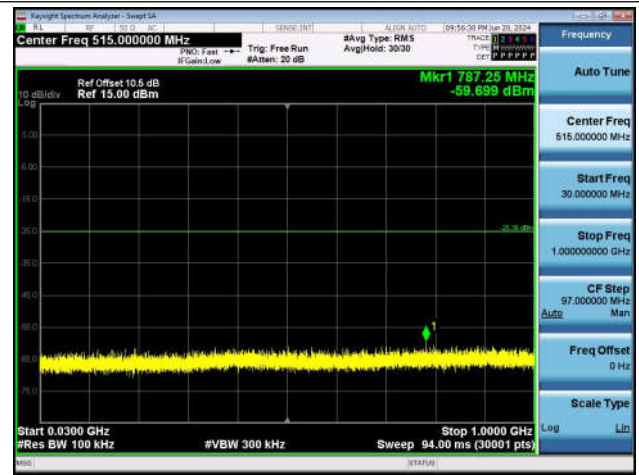
11N20SISO-Ant1-2412-30~1000-PASS
