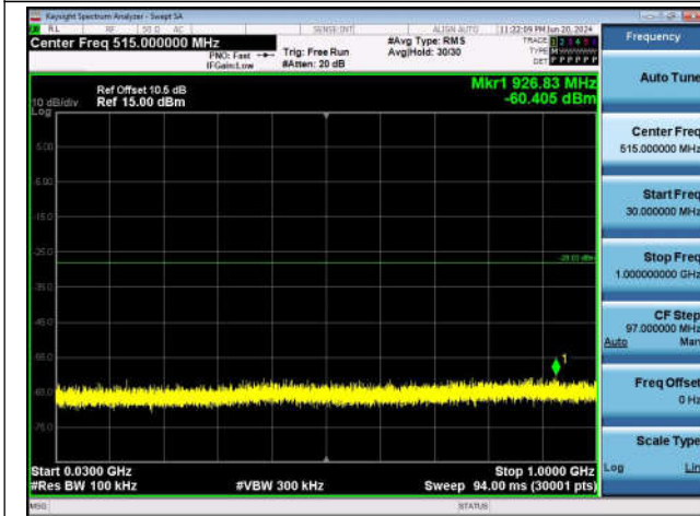
11N40SISO-Ant1-2452-30~1000-PASS
