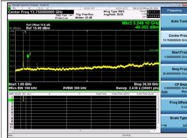
11G-Ant1-2437-1000~26500-PASS
