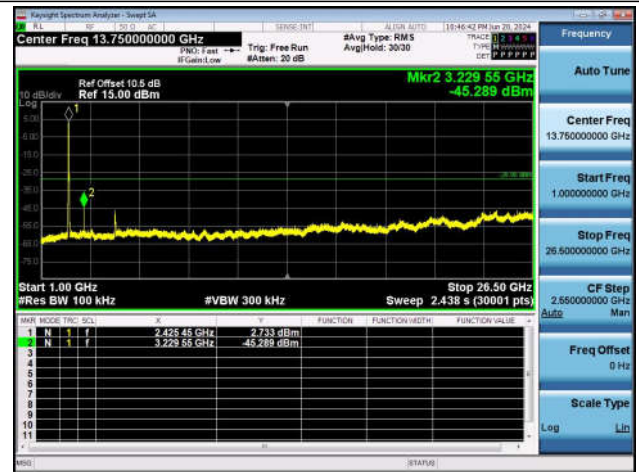
11N40SISO-Ant1-2422-1000~26500-PASS
