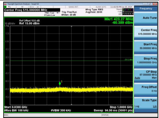
11N40SISO-Ant1-2437-30~1000-PASS
