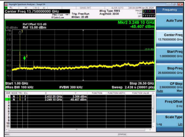
11N20SISO-Ant1-2437-1000~26500-PASS
