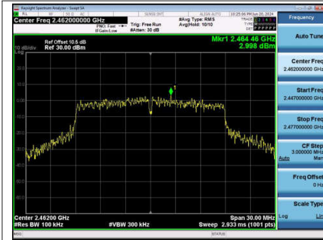
11N20SISO-Ant1-2462-0~Reference-PASS
