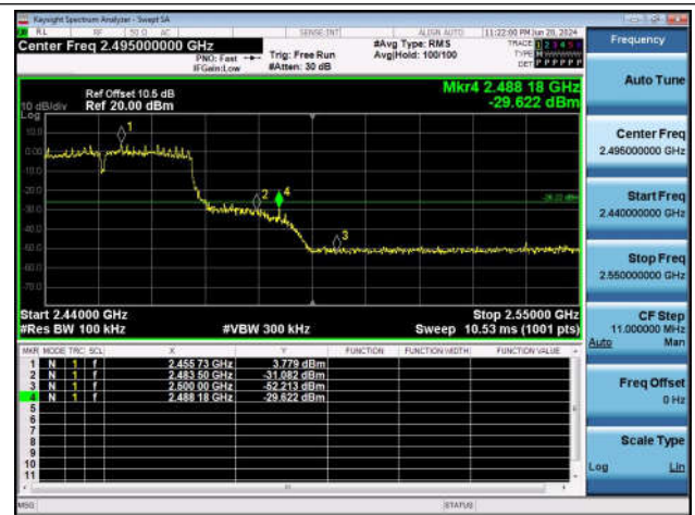
11N40SISO-Ant1-2452-PASS
