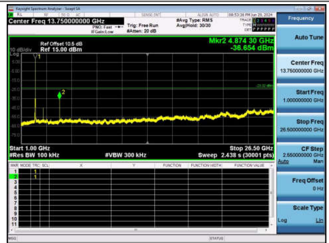
11B-Ant1-2437-1000~26500-PASS
