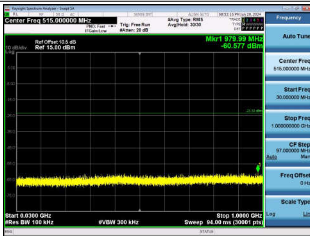
11B-Ant1-2437-30~1000-PASS
