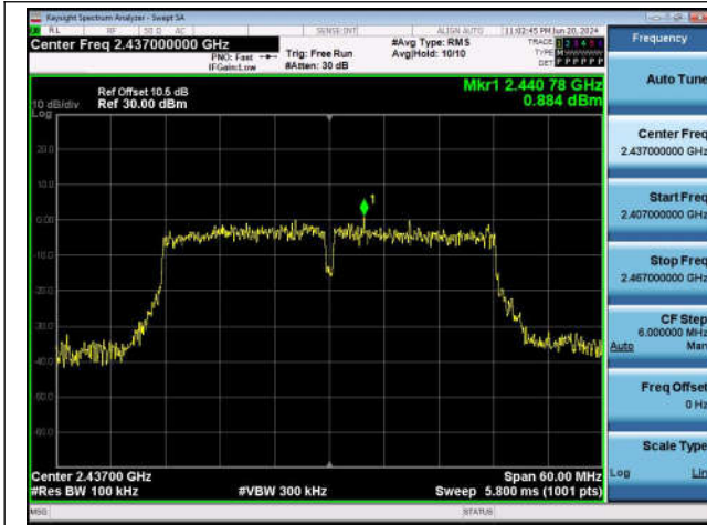
11N40SISO-Ant1-2437-0~Reference-PASS
