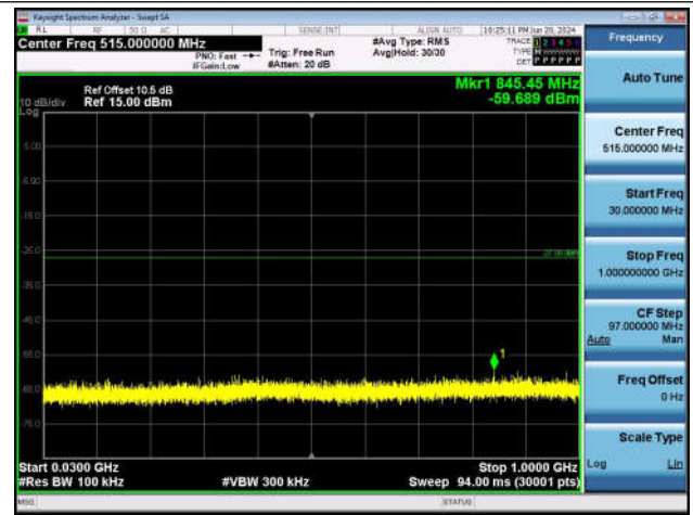
11N20SISO-Ant1-2462-30~1000-PASS
