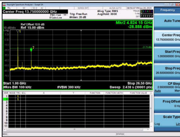
11B-Ant1-2412-1000~26500-PASS
