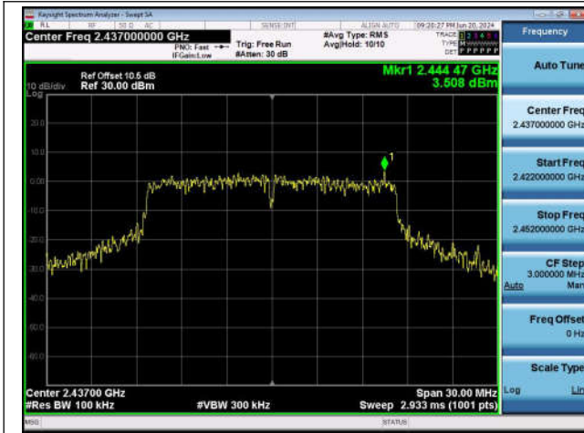
11G-Ant1-2437-0~Reference-PASS
