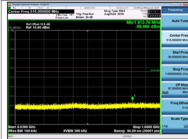
11N40SISO-Ant1-2422-30~1000-PASS
