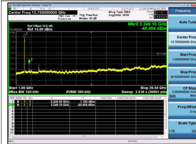
11N40SISO-Ant1-2437-1000~26500-PASS
