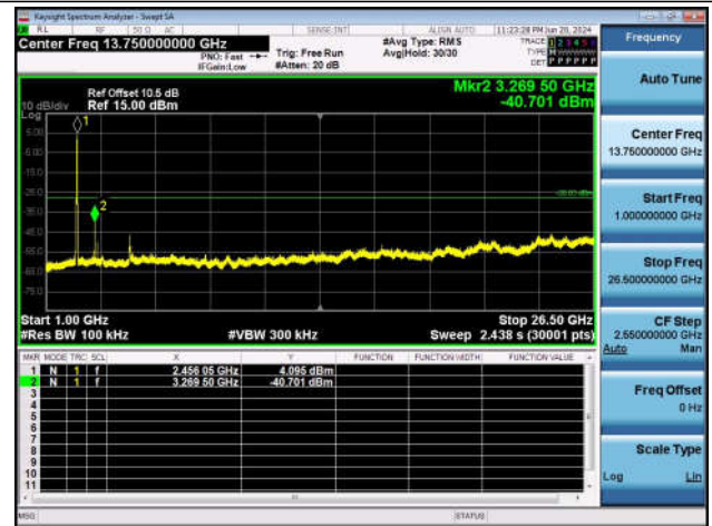
11N40SISO-Ant1-2452-1000~26500-PASS
