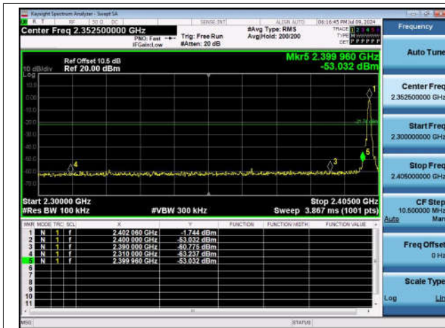
BLE_1M-Ant1-2402-PASS
