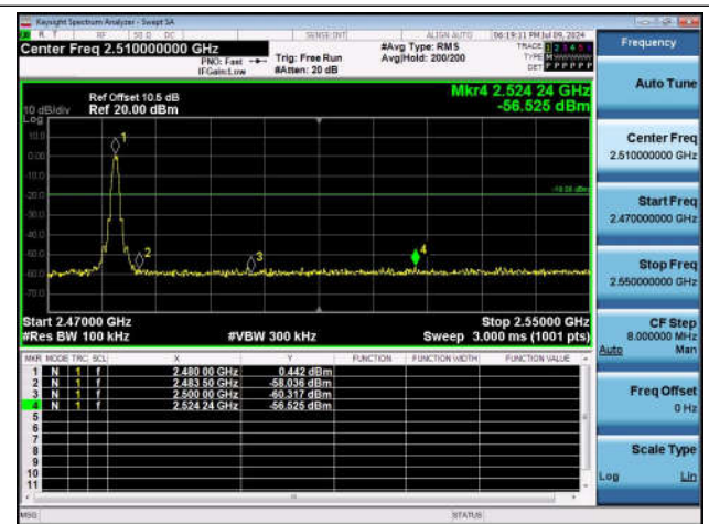
BLE_1M-Ant1-2480-PASS
