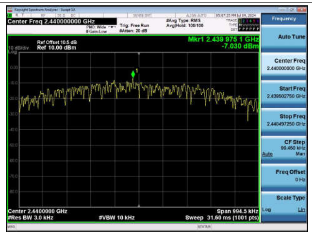
BLE_1M-Ant1-2440-PASS
