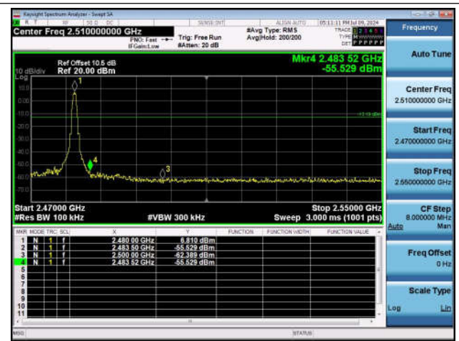
BLE_1M-Ant1-2480-PASS
