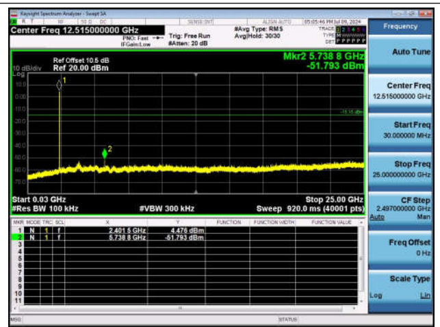
BLE_1M-Ant1-2402-30~25000-PASS
