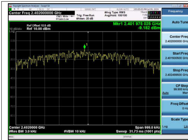
BLE_1M-Ant1-2402-PASS
