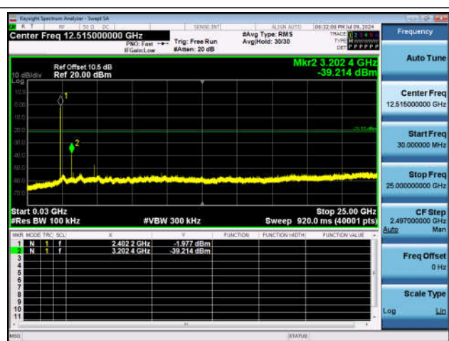
DH5-Ant1-2402-30~25000-PASS
