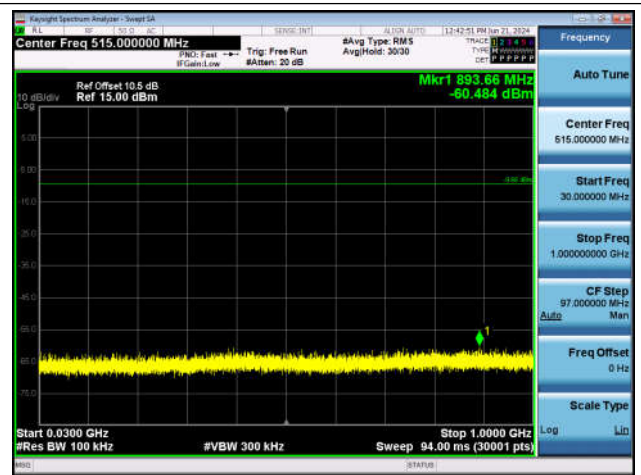
2DH5-Ant1-2441-30~1000-PASS
