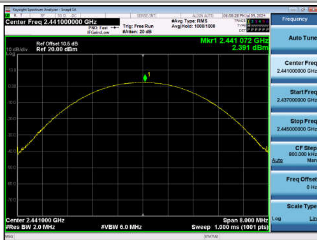
2DH5-Ant1-2441-PASS
