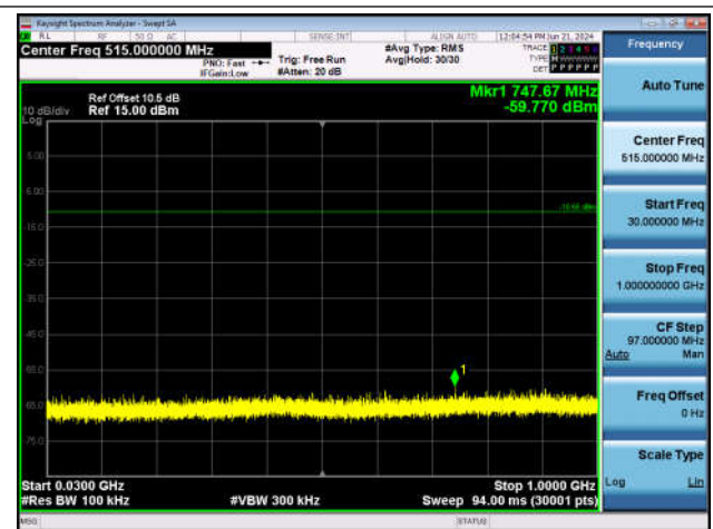
DH5-Ant1-2402-30~1000-PASS
