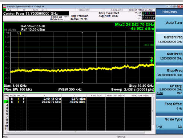
3DH5-Ant1-2402-1000~26500-PASS
