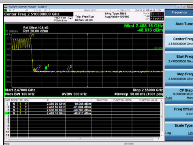
DH5-Ant1-Hop_2480-PASS
