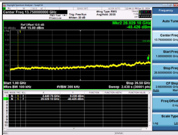
2DH5-Ant1-2441-1000~26500-PASS
