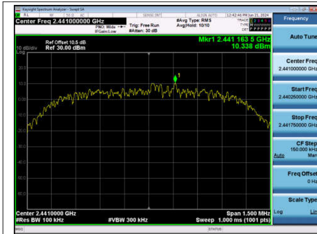
2DH5-Ant1-2441-0~Reference-PASS
