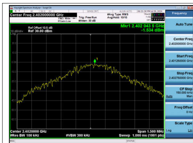
DH5-Ant1-2402-0~Reference-PASS
