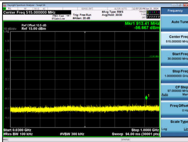
2DH5-Ant1-2480-30~1000-PASS
