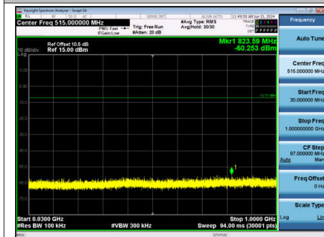
DH5-Ant1-2441-30~1000-PASS
