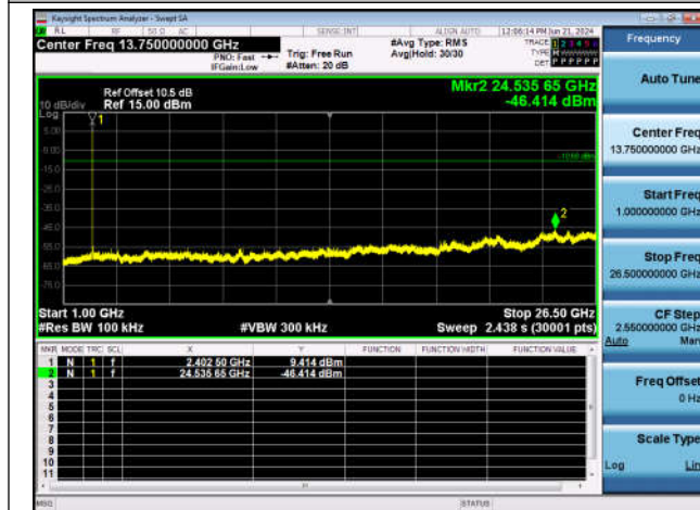
DH5-Ant1-2402-1000~26500-PASS
