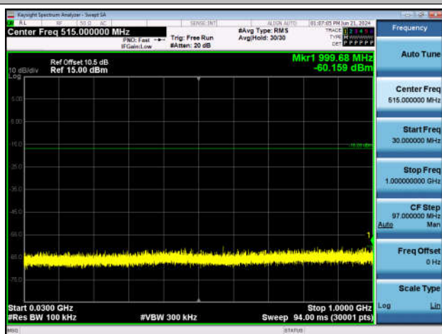
3DH5-Ant1-2441-30~1000-PASS
