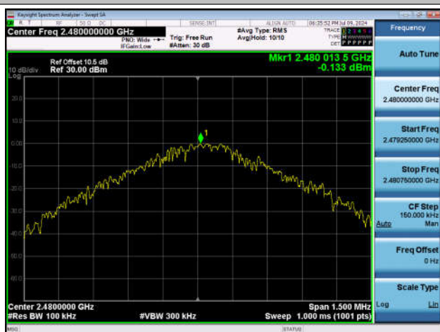
DH5-Ant1-2480-0~Reference-PASS
