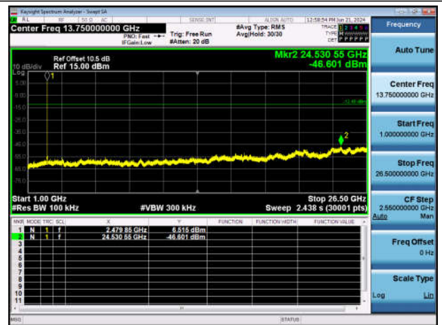
2DH5-Ant1-2480-1000~26500-PASS
