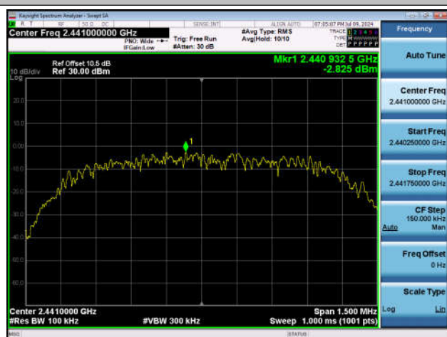
3DH5-Ant1-2441-0~Reference-PASS
