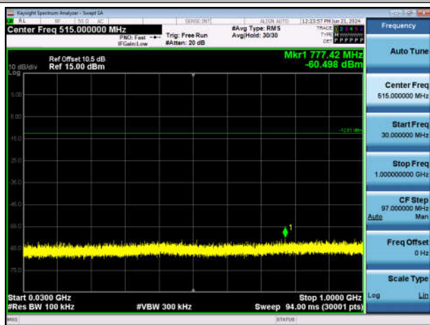
2DH5-Ant1-2402-30~1000-PASS
