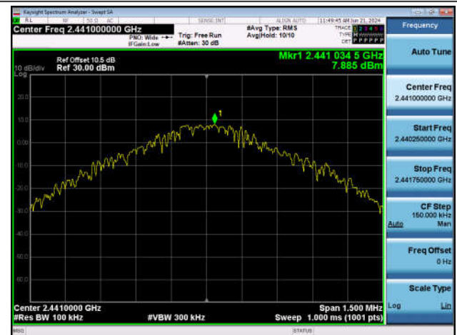
DH5-Ant1-2441-0~Reference-PASS
