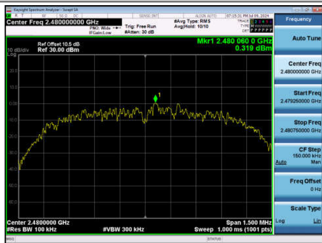
3DH5-Ant1-2480-0~Reference-PASS
