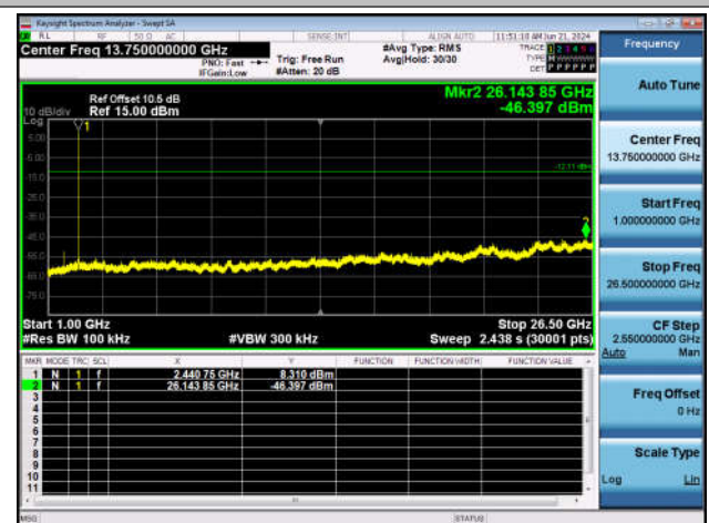
DH5-Ant1-2441-1000~26500-PASS
