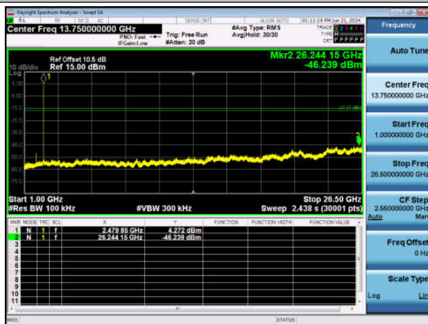
3DH5-Ant1-2480-1000~26500-PASS
