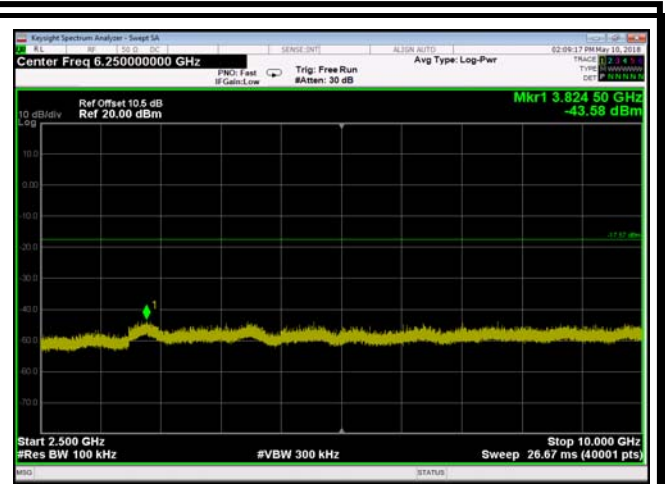
Transmitter Spurious Emission: 2440,Reference Level
