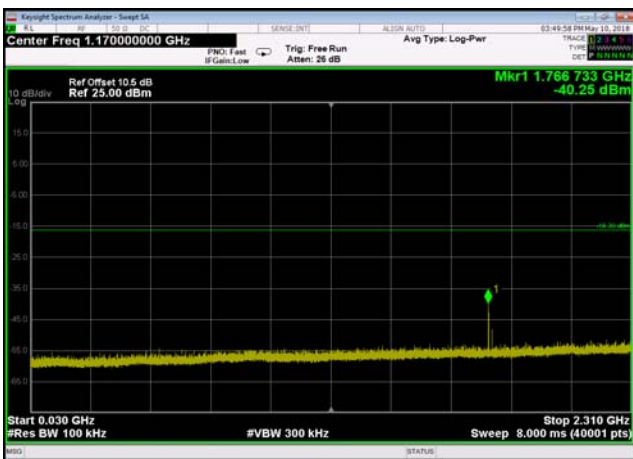
Conducted Emission: PI/4QPSK,2441,2DH5, Reference Level
