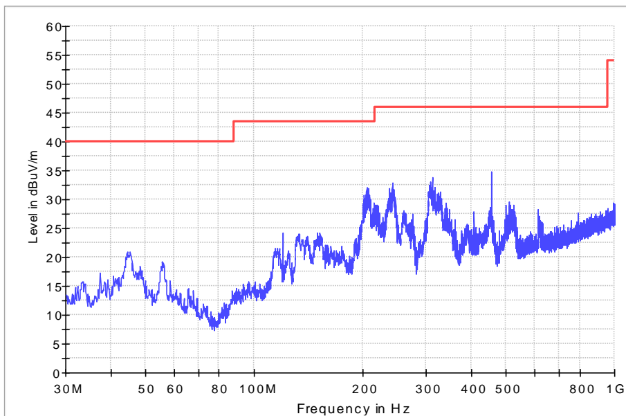
Copy of Field strength 30M-1GHz
