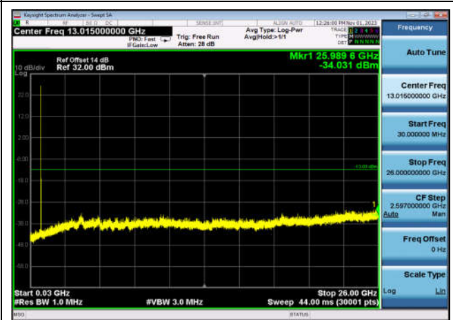
FDD07_LowRange_20MHz_30MHz~26GHz
