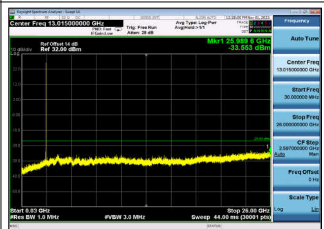
FDD07_HighRange_10MHz_30MHz~26GHz
