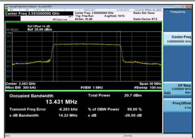
TDD41_MidRange_20_2593_Q16
