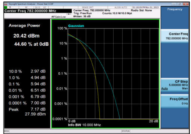
FDD13_MidRange_10MHz_782_fullIRB_Q16
