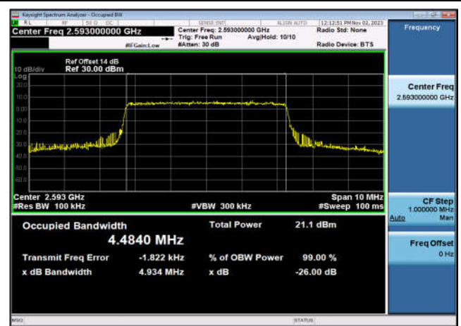
TDD41_MidRange_5_2593_Q16
