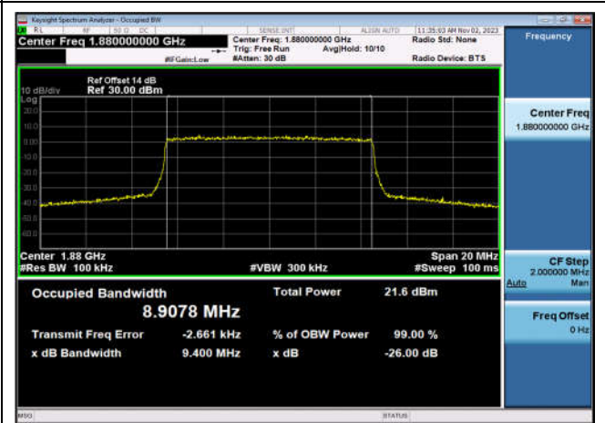
FDD02_MidRange_15_1880_Q16
