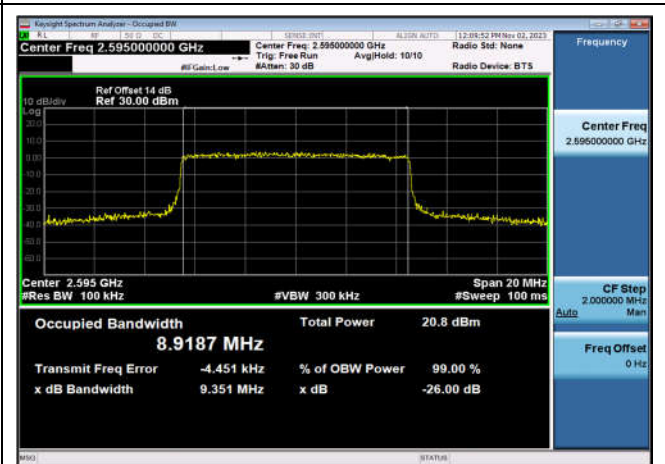
TDD38_MidRange_10_2595_Q16
