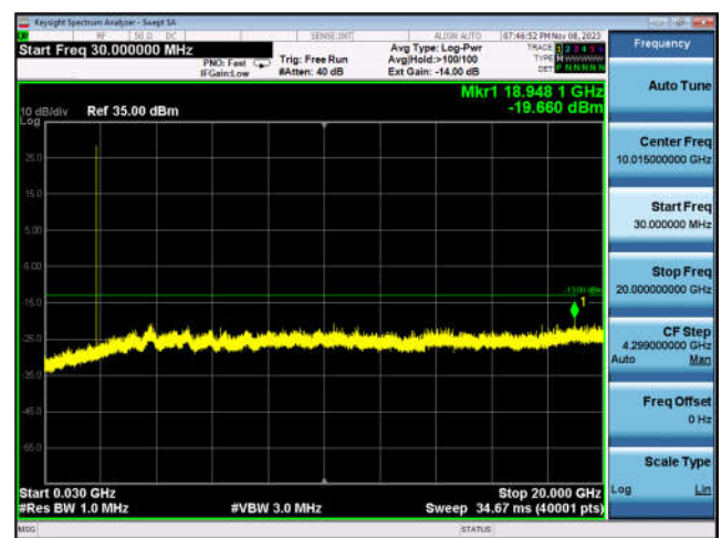
EDGE 1900-810, 30MHz to 20GHz
