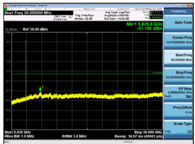
WCDMA 1900-9538, 30MHz to 20GHz
