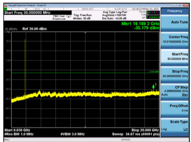
WCDMA 1900-9538, 30MHz to 20GHz
