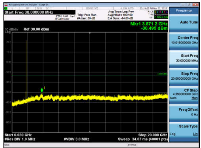
WCDMA 1900-9400, 30MHz to 20GHz
