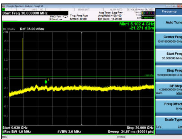
PCS 1900-810, 30MHz to 20GHz
