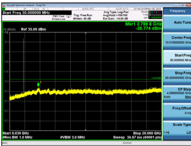
PCS 1900-661, 30MHz to 20GHz
