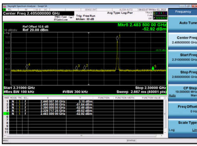
,Plot ,2Conducted Emission: 2440 ,Band Edge
