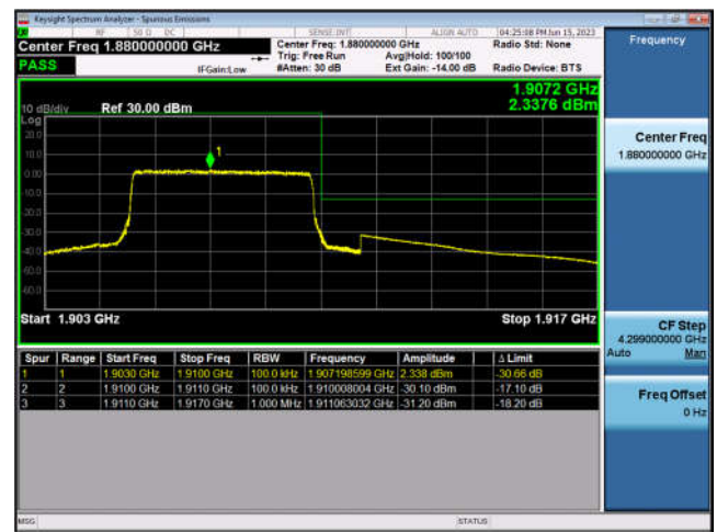
FDD2-5MHz-16QAM-HCH-25RB#0
