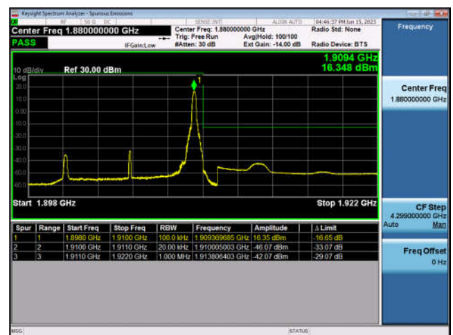
FDD2-10MHz-16QAM-HCH-1RB#49
