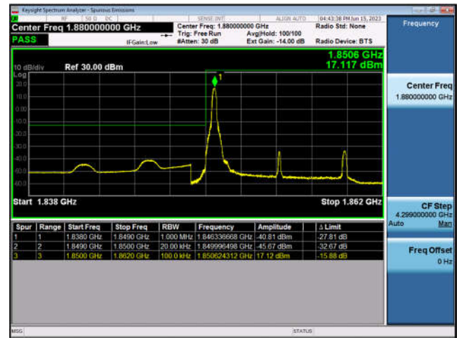
FDD2-10MHz-16QAM-LCH-50RB#0
