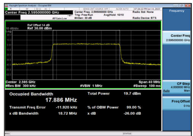
TDD38_MidRange_20_2595_Q16
