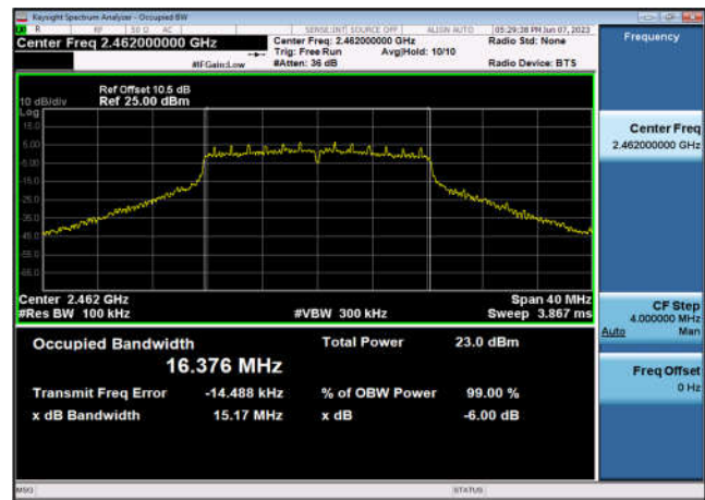
6dB Bandwidth-802.11g,2462MHz,Ant0
