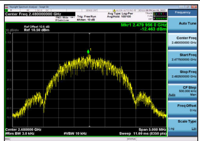
PSD: 2480MHz – 2MHz bandwidth
