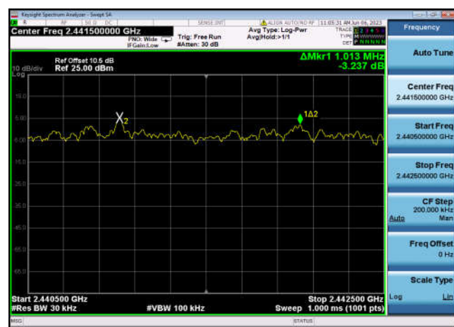
DQPSK,Hopping2DH5,2440.5~2442.5
