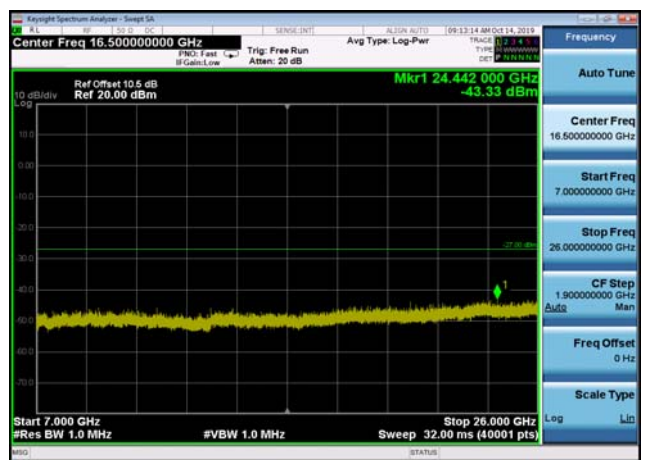
U-NII-3 ,Plot 4,7000MHz~26000MHz-802. 11a(20MHz),5785MHz,Ant2
