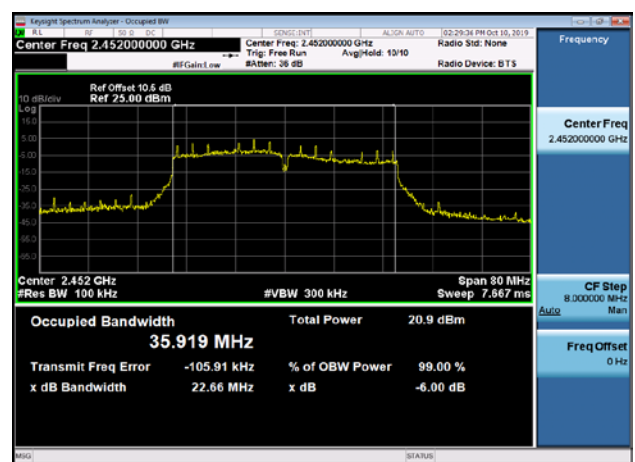
6dB Bandwidth-802.11n(HT40),2452MHz
