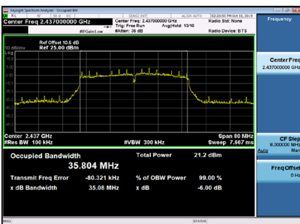
6dB Bandwidth-802.11n(HT40),2437MHz
