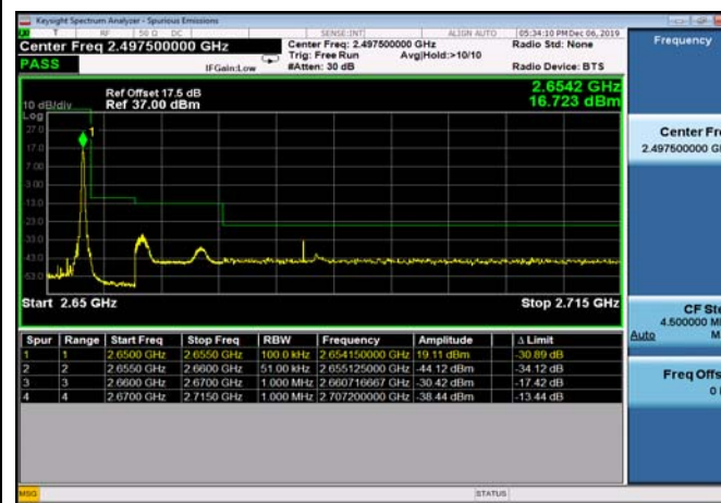
HighRange_TDD41_15MHz_2647.5_fullRB_high_QPSK
