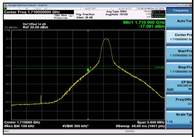
LowRange_FDD66_10MHz_1715_fullRB_Low_Q16
