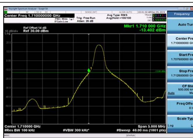
LowRange_FDD66_10MHz_1715_OneRB_low_QPSK
