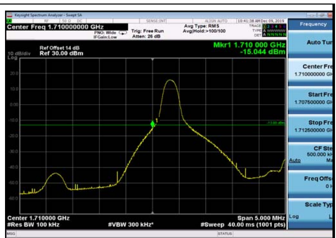
LowRange_FDD66_10MHz_1715_OneRB_low_Q16
