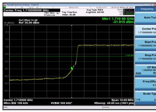
LowRange_FDD66_15MHz_1717.5_OneRB_low_QPSK
