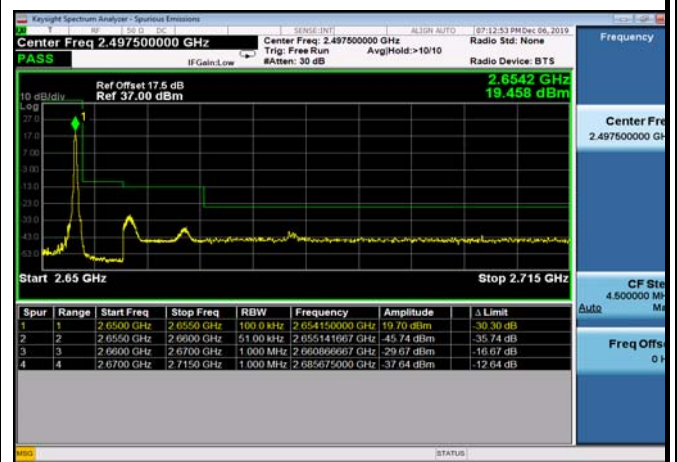
HighRange_TDD41_15MHz_2647.5_fullRB_high_Q16
