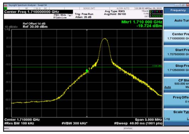
LowRange_FDD66_10MHz_1715_fullRB_Low_QPSK
