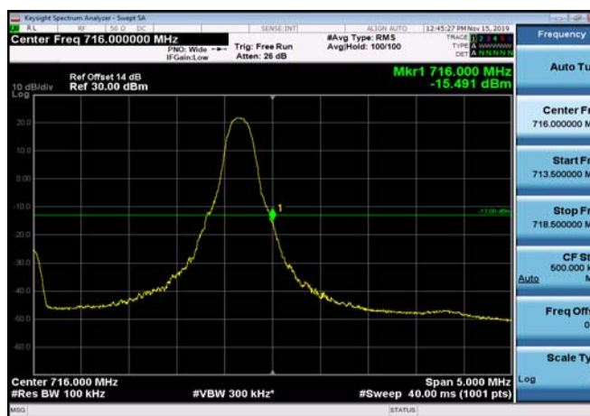
HighRange_FDD12_5MHz_713.5_fullRB_High_QPSK
