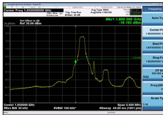
LowRange_FDD25_1.4MHz_1850.7_fullRB_Low_QPSK
