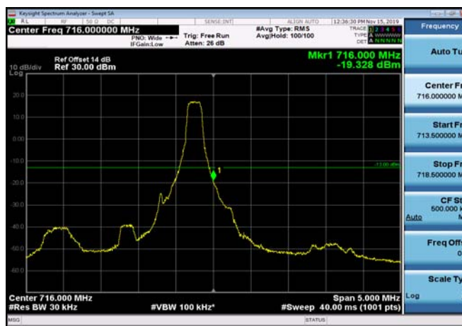
HighRange_FDD12_1.4MHz_715.3_fullRB _High_QPSK
