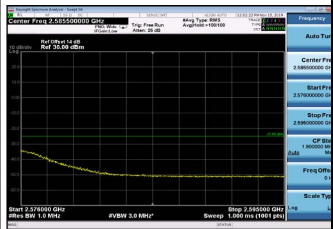
HighRange_FDD07_10MHz_2565_OneRB_high_Q16
