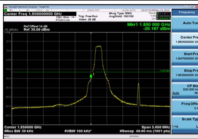
LowRange_FDD25_5MHz_1852.5_OneRB _low_Q16
