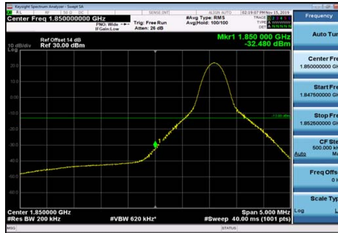
LowRange_FDD25_20MHz_1860_fullRB_Low_Q16
