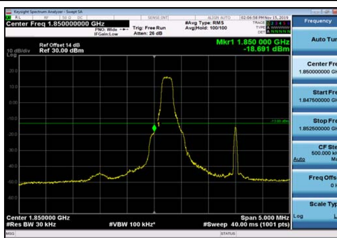
LowRange_FDD25_5MHz_1852.5_OneRB _low_QPSK
