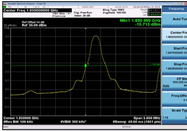
LowRange_FDD25_5MHz_1852.5_fullRB _Low_QPSK
