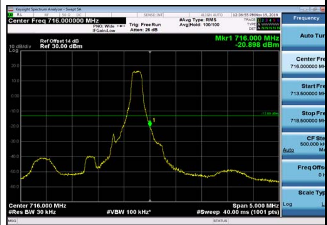
HighRange_FDD12_1.4MHz_715.3_fullRB _High_Q16
