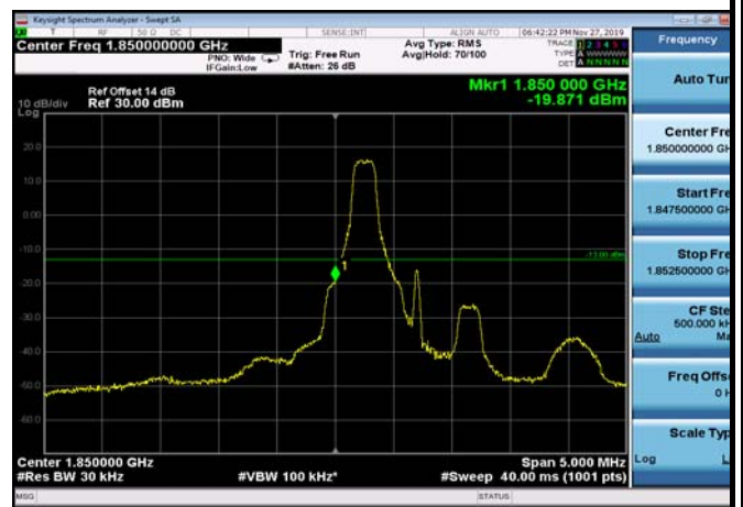
LowRange_FDD25_1.4MHz_1850.7_fullRB_Low_Q16
