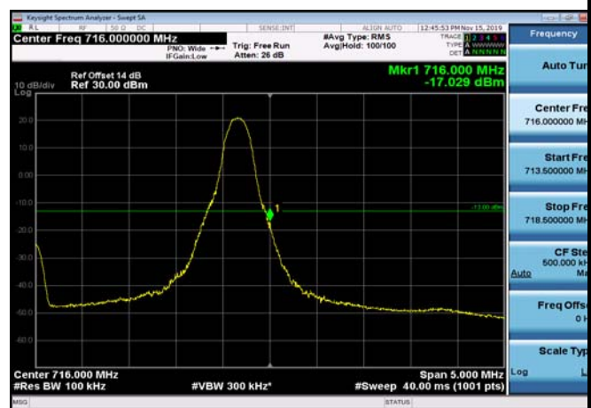
HighRange_FDD12_5MHz_713.5_fullRB_High_Q16
