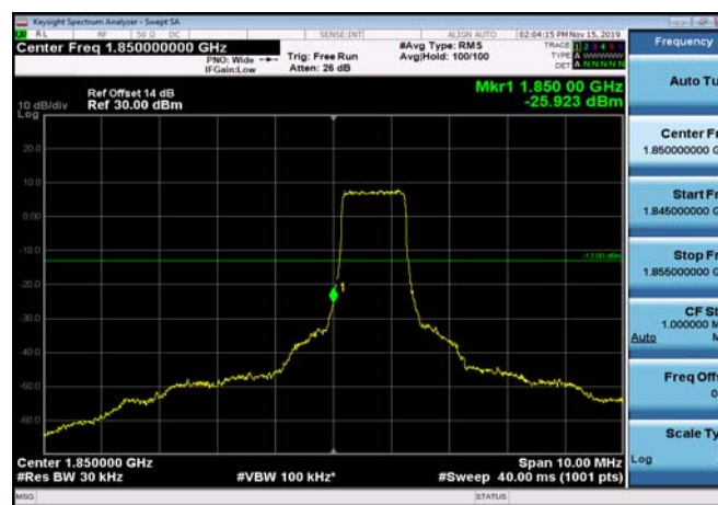
LowRange_FDD25_3MHz_1851.5_OneRB_low_QPSK
