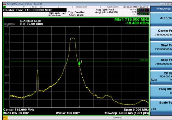
HighRange_FDD12_3MHz_714.5_fullRB _High_QPSK
