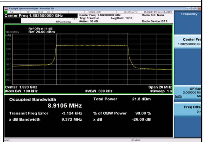
FDD25_MidRange_10_1882.5_Q16
