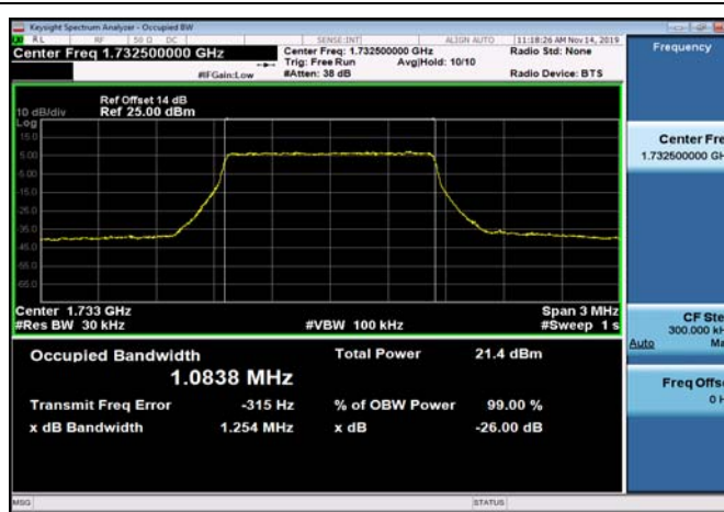
FDD04_MidRange_3_1732.5_Q16
