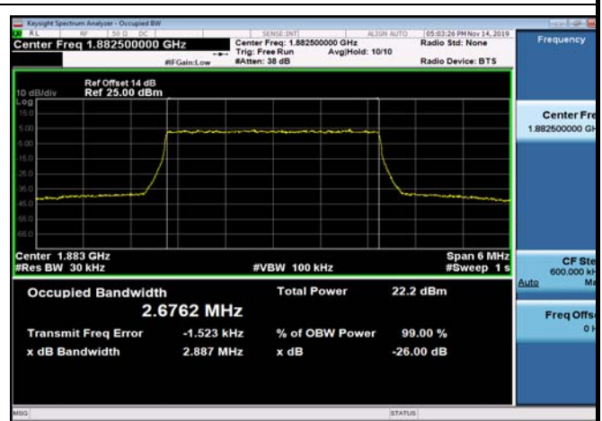
FDD25_MidRange_5_1882.5_Q16
