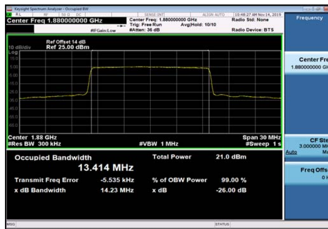
FDD02_MidRange_15MHz_1880MHz_Q16
