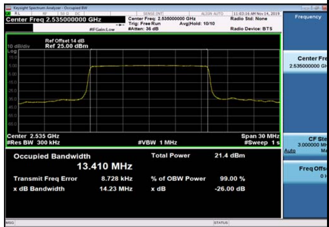
FDD07_MidRange_20MHz_2535MHz_Q16
