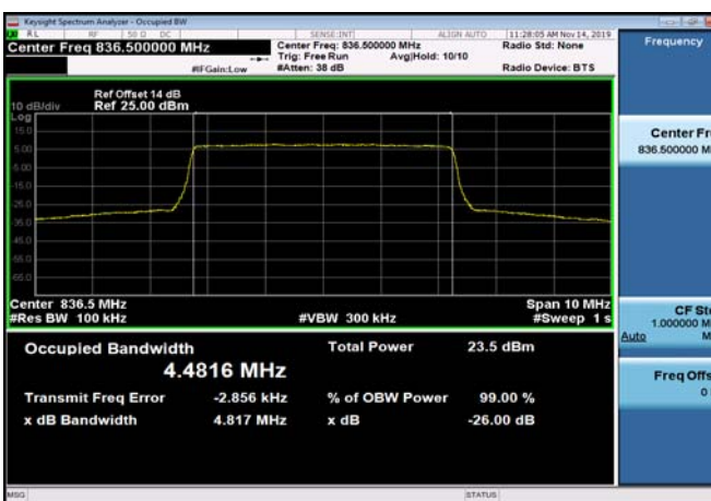
FDD05_MidRange_5_836.5_QPSK
