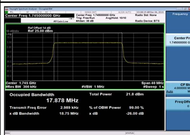
FDD66_MidRange_20_1745_QPSK
