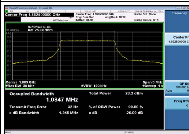
FDD25_MidRange_1.4_1882.5_QPSK
