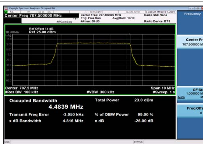
FDD12_MidRange_10_707.5_QPSK
