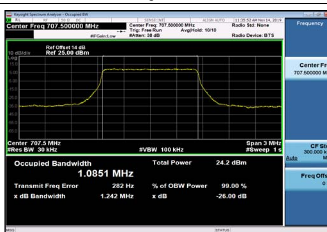
FDD12_MidRange_1.4_707.5_QPSK
