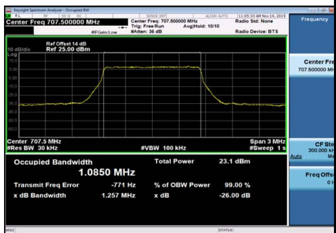
FDD12_MidRange_1.4MHz_707.5MHz_Q16
