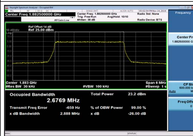
FDD25_MidRange_5_1882.5_QPSK
