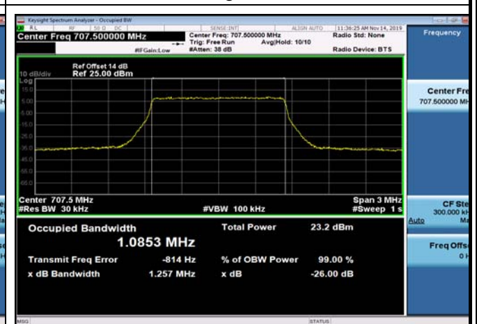
FDD12_MidRange_1.4_707.5_Q16
