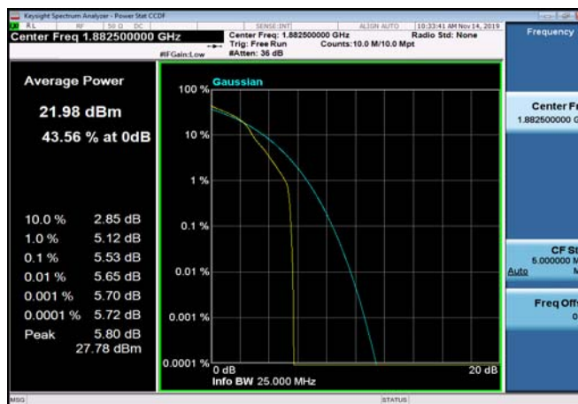
FDD25_HighRange_20MHz_1905_OneRB _high_Q16
