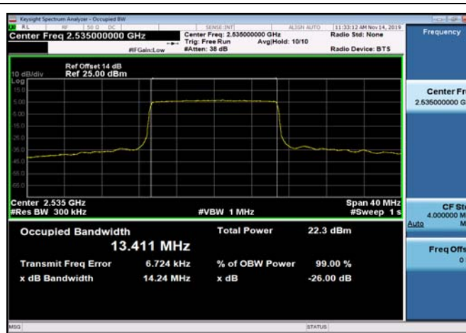
FDD07_MidRange_20_2535_QPSK
