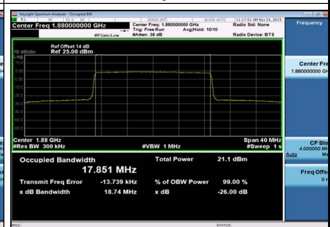
FDD02_MidRange_20_1880_Q16
