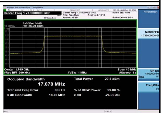
FDD66_MidRange_20_1745_Q16
