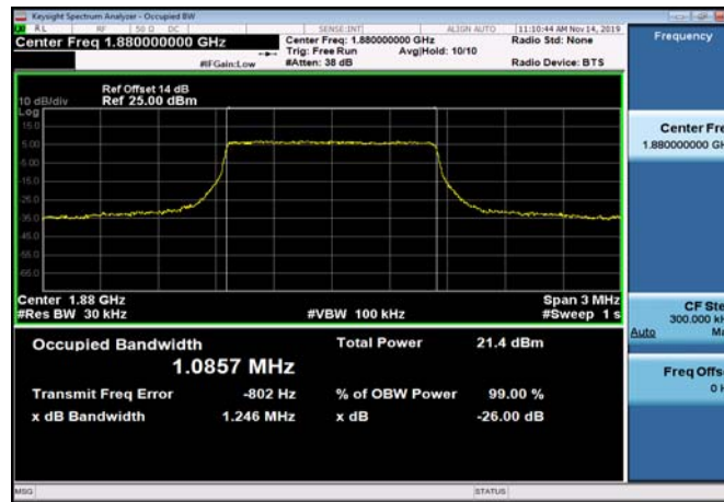
FDD02_MidRange_3_1880_Q16
