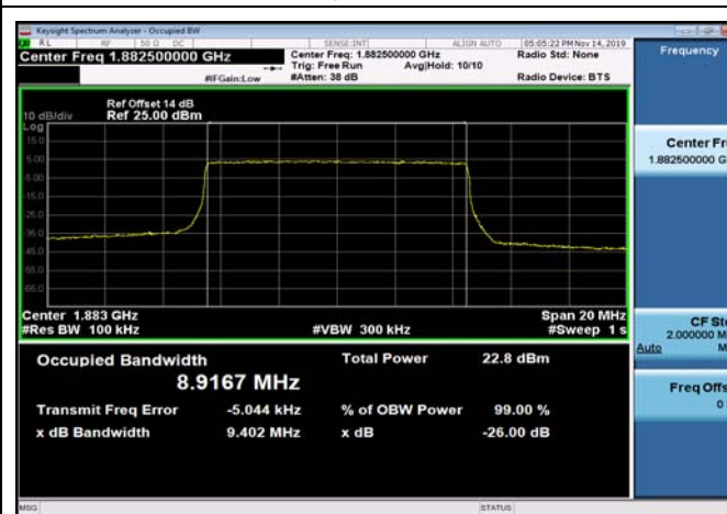
FDD25_MidRange_10_1882.5_QPSK
