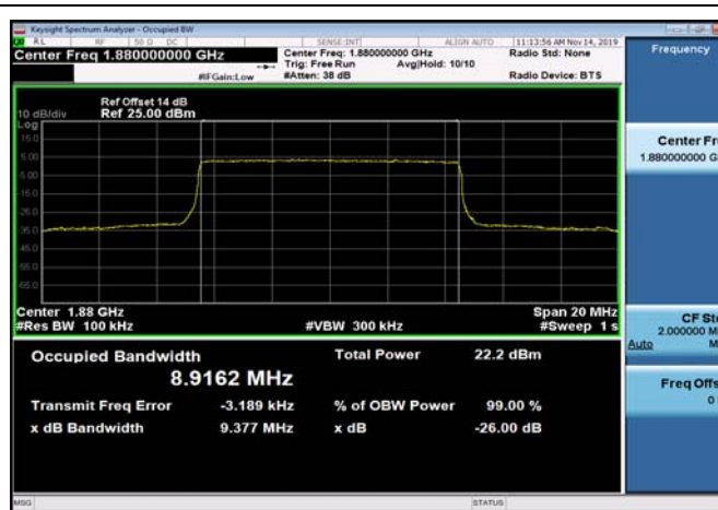
FDD02_MidRange_15_1880_QPSK
