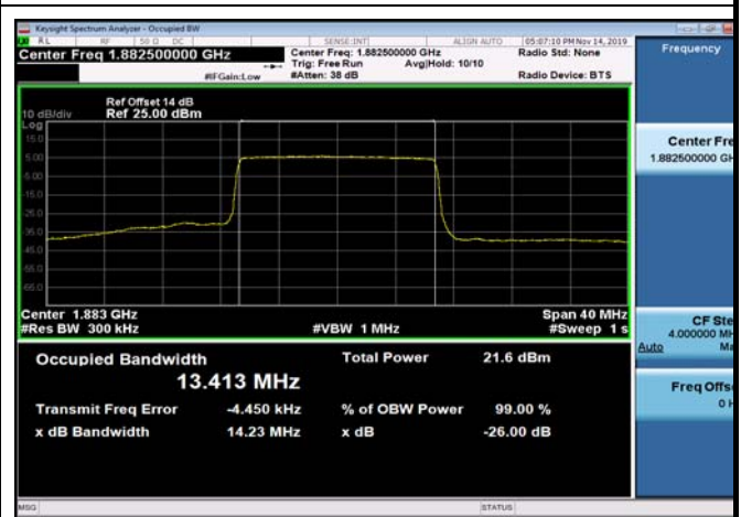
FDD25_MidRange_20_1882.5_Q16
