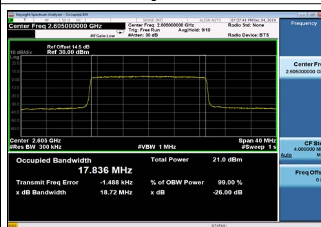
TDD41_MidRange_20_2605_QPSK
