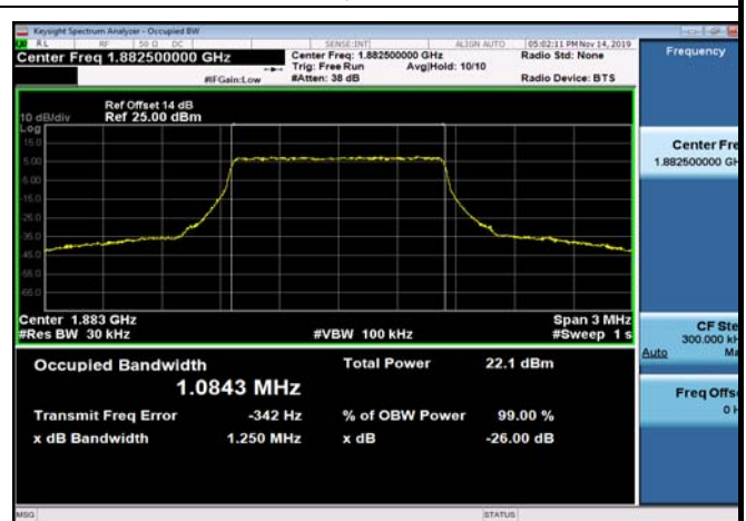
FDD25_MidRange_1.4_1882.5_Q16
