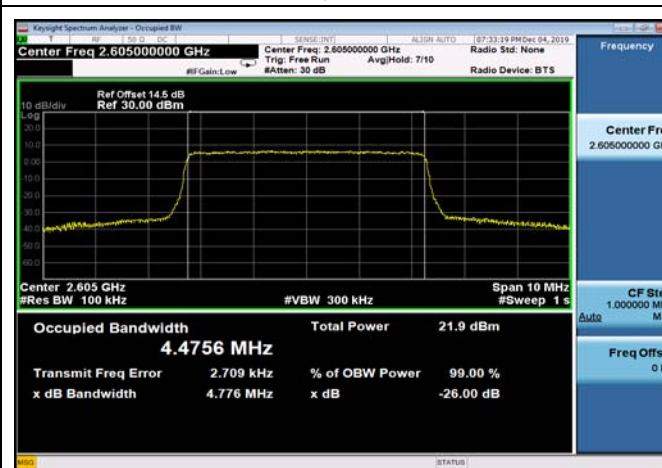
TDD41_MidRange_5_2605_QPSK
