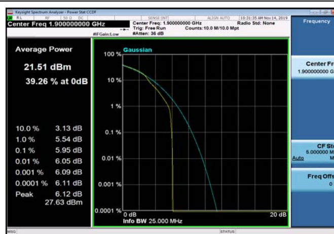
FDD02_HighRange_20MHz_1900_OneRB _high_Q16
