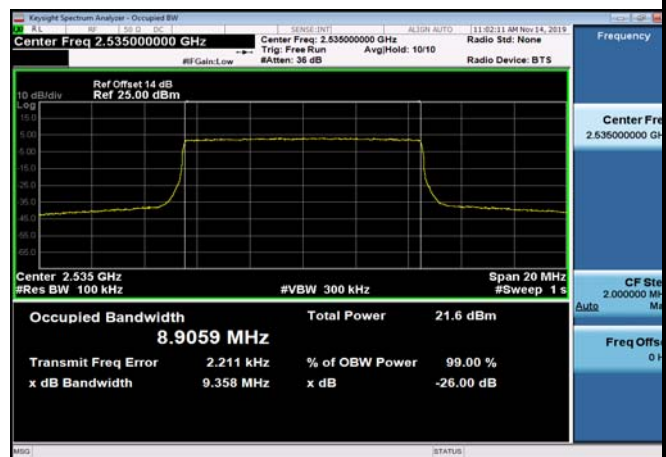
FDD07_MidRange_10MHz_2535MHz_Q16
