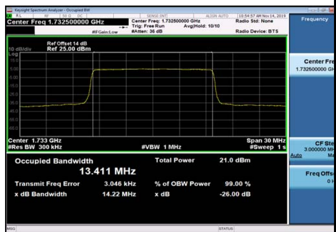
FDD04_MidRange_15MHz_1732.5MHz_Q16
