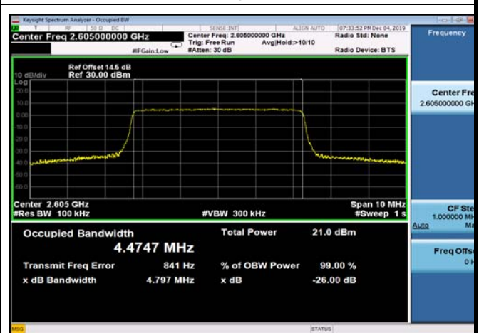
TDD41_MidRange_5_2605_Q16
