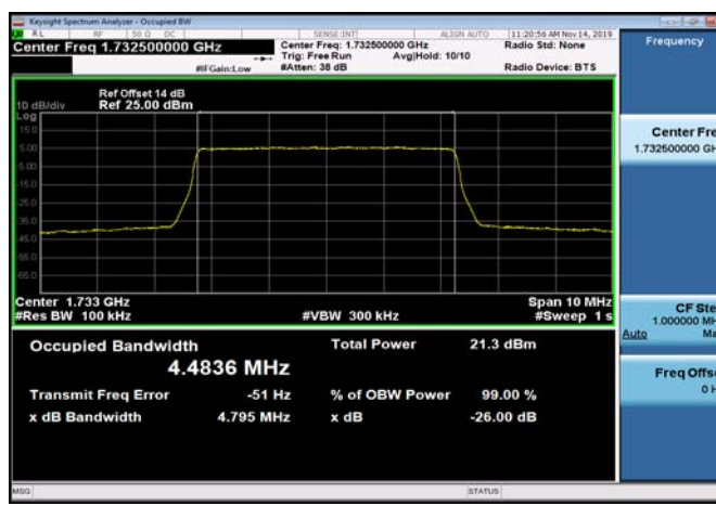
FDD04_MidRange_5_1732.5_Q16
