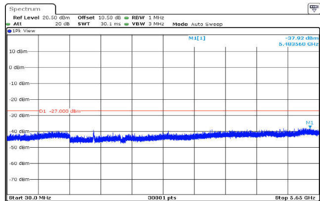
U-NII-3,802.11n(40MHz),5795MHz ,Ant1,Plot 2,30MHz~5650MHz
