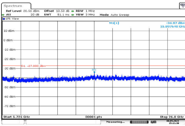
U-NII-2c,802.11a(20MHz),5500MHz ,Ant1,Plot 3,5725MHz~26000MHz
