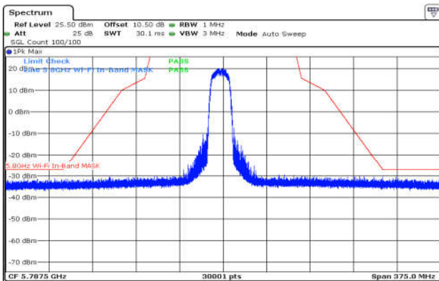
U-NII-3,802.11a(20MHz),5785MHz ,Ant1,Plot 1,Band Edge
