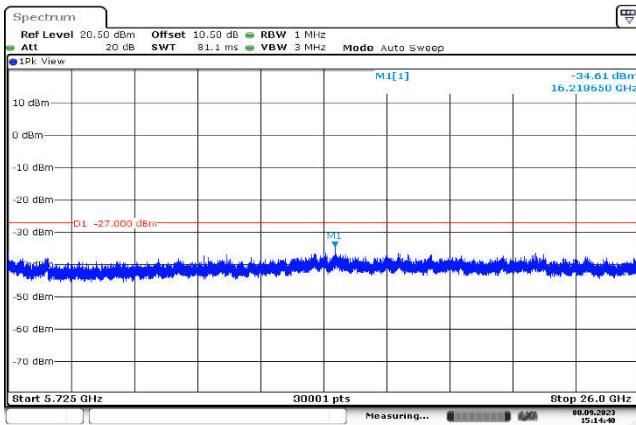
U-NII-2c,802.11a(20MHz),5700MHz ,Ant1,Plot 3,5725MHz~26000MHz
