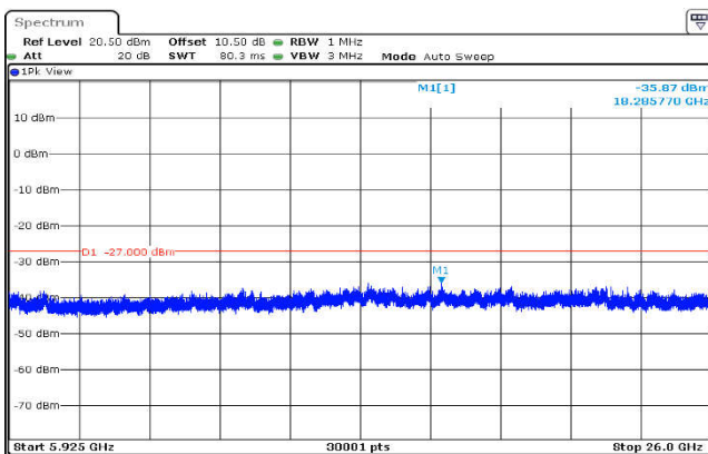
U-NII-3,802.11n(40MHz),5795MHz ,Ant1,Plot 3,5925MHz~26000MHz
