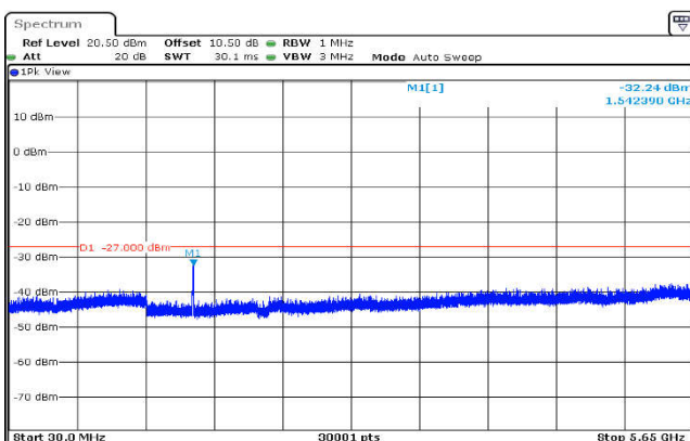
U-NII-3,802.11a(20MHz),5745MHz ,Ant1,Plot 2,30MHz~5650MHz
