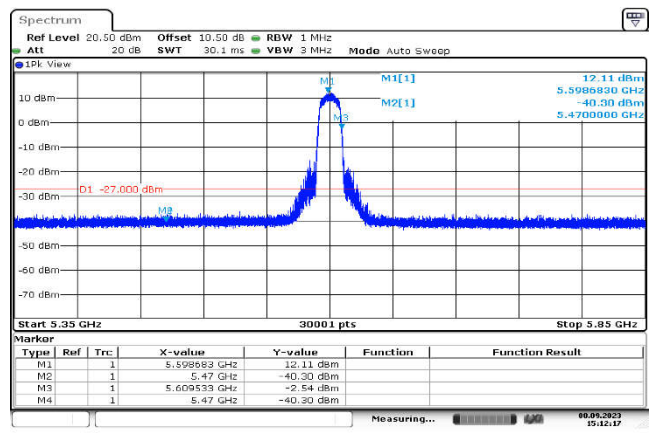
U-NII-2c,802.11a(20MHz),5600MHz ,Ant1,Plot 1,Band Edge
