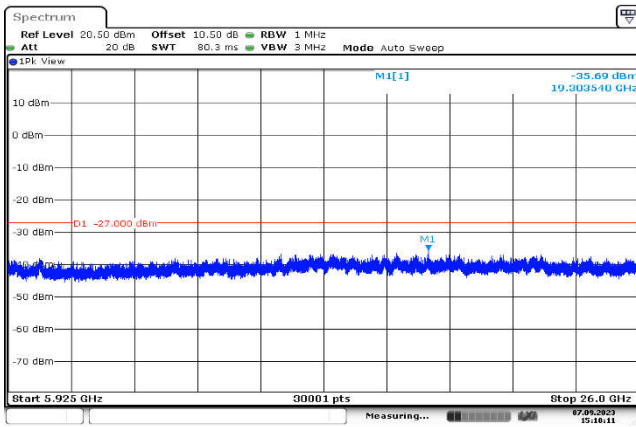
U-NII-3,802.11n(20MHz),5745MHz ,Ant1,Plot 3,5925MHz~26000MHz
