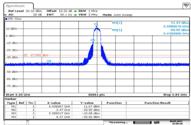
U-NII-2c,802.11n(20MHz),5600MHz ,Ant1,Plot 1,Band Edge
