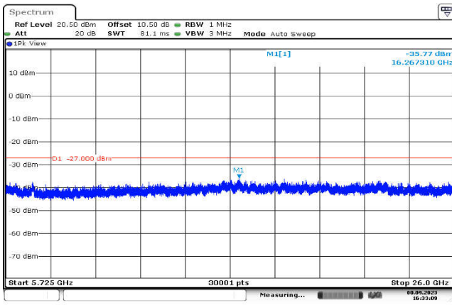
U-NII-2c,802.11n(40MHz),5590MHz ,Ant1,Plot 3,5725MHz~26000MHz
