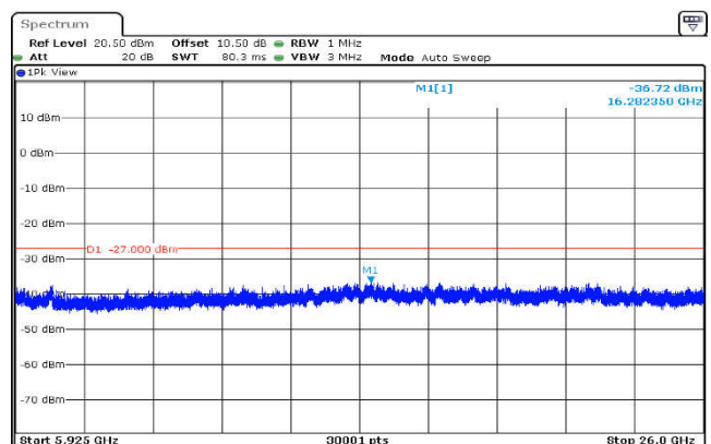
U-NII-3,802.11a(20MHz),5825MHz ,Ant1,Plot 3,5925MHz~26000MHz
