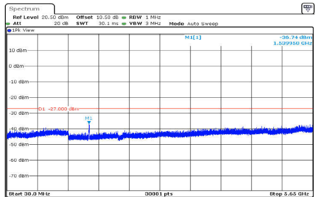
U-NII-3,802.11n(20MHz),5745MHz ,Ant1,Plot 2,30MHz~5650MHz
