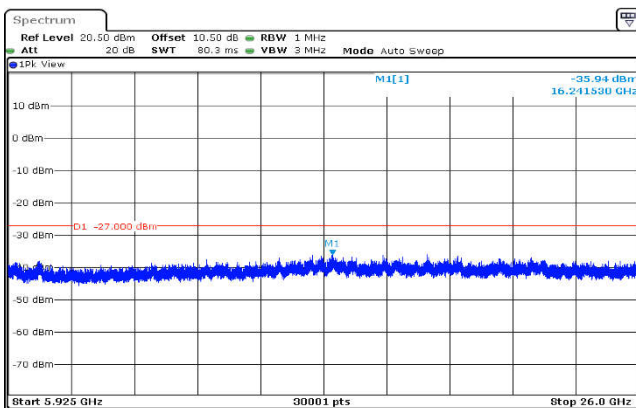
U-NII-3,802.11a(20MHz),5785MHz ,Ant1,Plot 3,5925MHz~26000MHz
