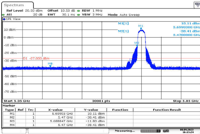
U-NII-2c,802.11n(20MHz),5700MHz ,Ant1,Plot 1,Band Edge
