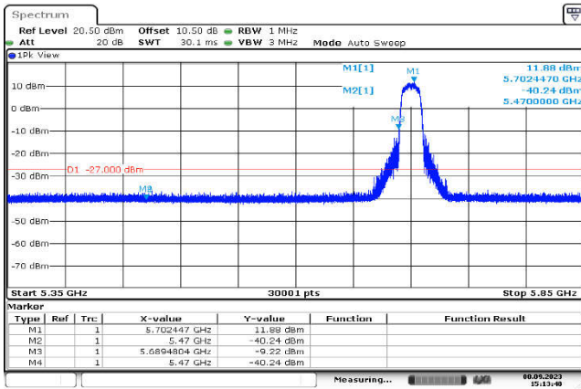
U-NII-2c,802.11a(20MHz),5700MHz ,Ant1,Plot 1,Band Edge
