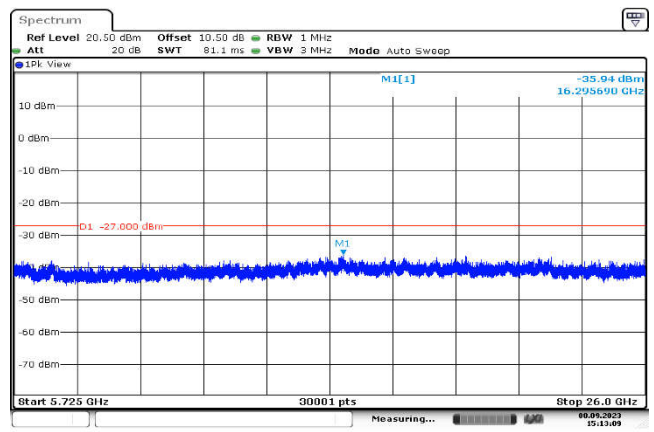
U-NII-2c,802.11a(20MHz),5600MHz ,Ant1,Plot 3,5725MHz~26000MHz
