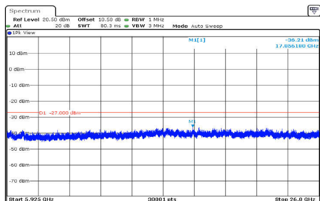
U-NII-3,802.11a(20MHz),5745MHz ,Ant1,Plot 3,5925MHz~26000MHz
