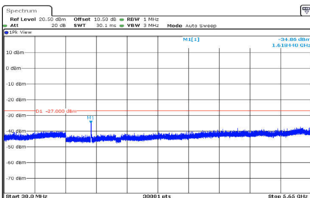
U-NII-3,802.11a(20MHz),5825MHz ,Ant1,Plot 2,30MHz~5650MHz
