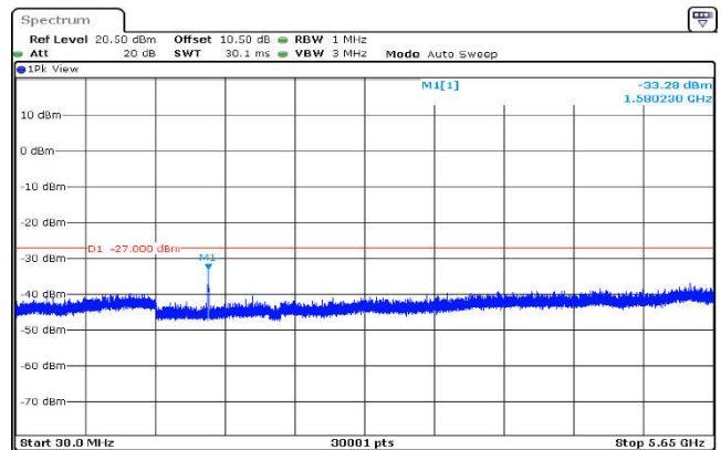
U-NII-3,802.11a(20MHz),5785MHz ,Ant1,Plot 2,30MHz~5650MHz
