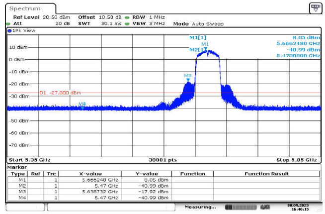
U-NII-2c,802.11n(40MHz),5670MHz ,Ant1,Plot 1,Band Edge
