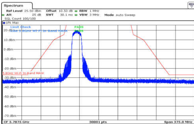
U-NII-3,802.11n(20MHz),5745MHz ,Ant1,Plot 1,Band Edge
