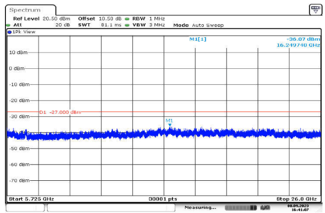
U-NII-2c,802.11n(40MHz),5670MHz ,Ant1,Plot 3,5725MHz~26000MHz
