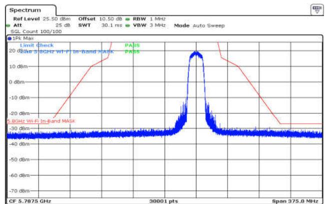
U-NII-3,802.11a(20MHz),5825MHz ,Ant1,Plot 1,Band Edge
