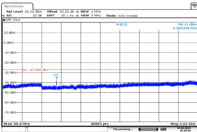
U-NII-3,802.11n(20MHz),5785MHz ,Ant1,Plot 2,30MHz~5650MHz
