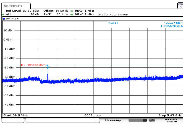
U-NII-2c,802.11a(20MHz),5600MHz ,Ant1,Plot 2,30MHz~5470MHz
