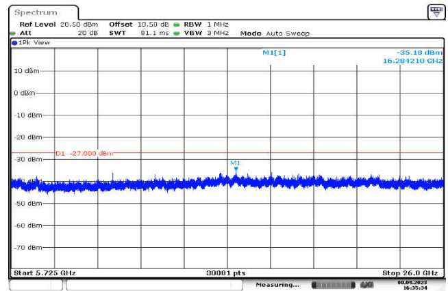
U-NII-2c,802.11n(40MHz),5510MHz ,Ant1,Plot 3,5725MHz~26000MHz
