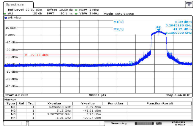
U-NII-2a,802.11ac(80MHz),5290MHz ,Ant1,Plot 1,Band Edge
