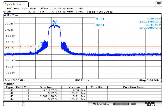
U-NII-2c,802.11n(40MHz),5510MHz ,Ant1,Plot 1,Band Edge
