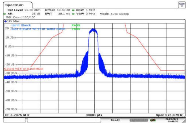
U-NII-3,802.11n(20MHz),5785MHz ,Ant1,Plot 1,Band Edge
