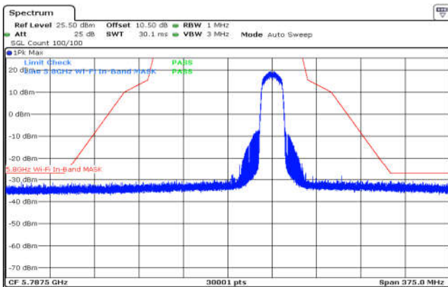
U-NII-3,802.11n(20MHz),5825MHz ,Ant1,Plot 1,Band Edge
