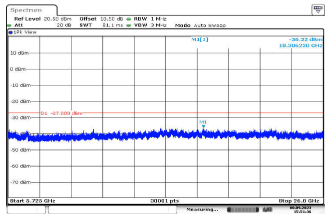
U-NII-2c,802.11n(20MHz),5600MHz ,Ant1,Plot 3,5725MHz~26000MHz
