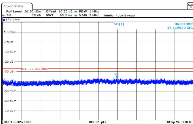
U-NII-3,802.11n(20MHz),5825MHz ,Ant1,Plot 3,5925MHz~26000MHz
