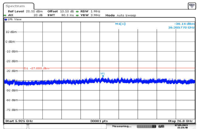
U-NII-3,802.11n(20MHz),5785MHz ,Ant1,Plot 3,5925MHz~26000MHz
