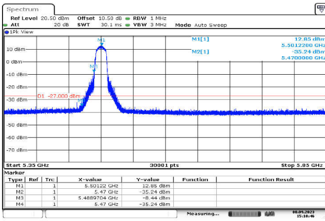
U-NII-2c,802.11a(20MHz),5500MHz ,Ant1,Plot 1,Band Edge
