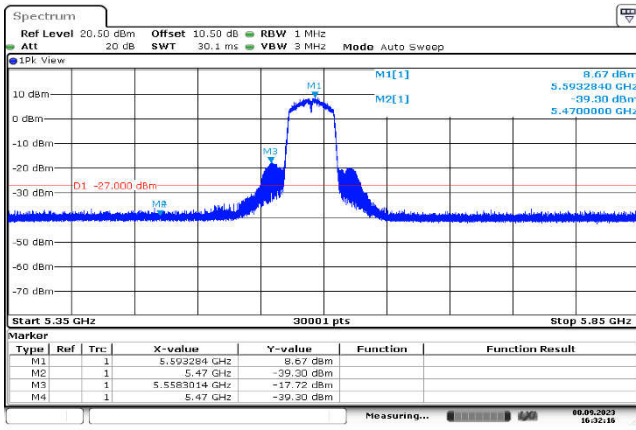
U-NII-2c,802.11n(40MHz),5590MHz ,Ant1,Plot 1,Band Edge
