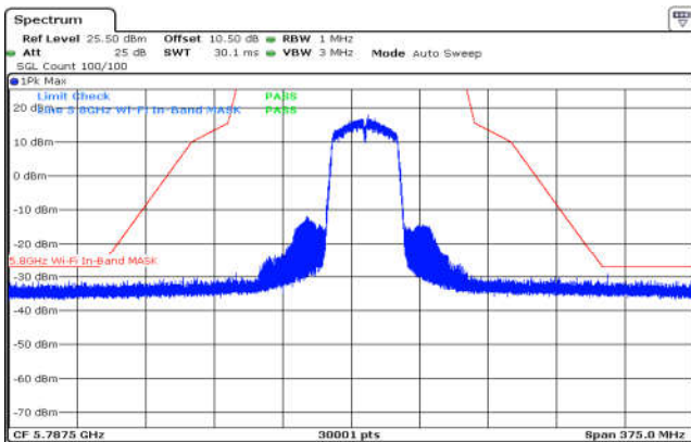
U-NII-3,802.11n(40MHz),5795MHz ,Ant1,Plot 1,Band Edge
