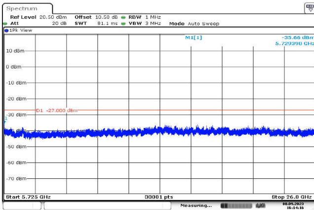
U-NII-2c,802.11n(20MHz),5700MHz ,Ant1,Plot 3,5725MHz~26000MHz
