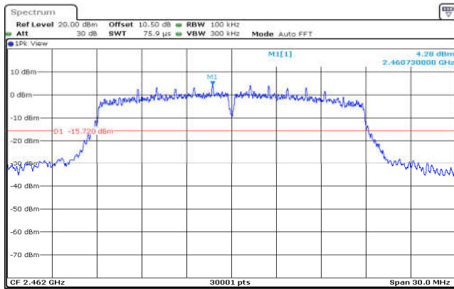
802.11n(HT20),2462MHz,Ant0,Plot 1,Reference Level
