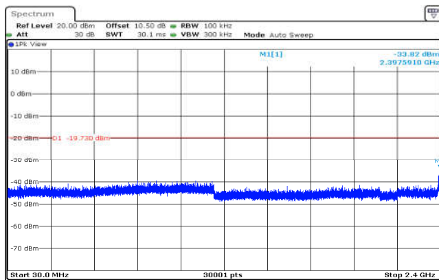
802.11n(HT40),2422MHz,Ant0,Plot 3,30MHz~2400MHz
