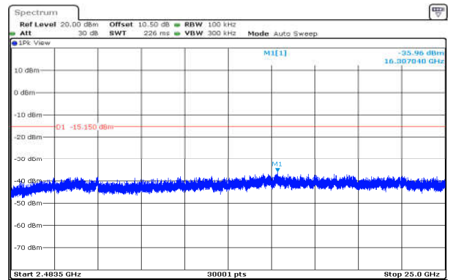
802.11g,2437MHz,Ant0,Plot 4,2483.5MHz ~25000MHz
