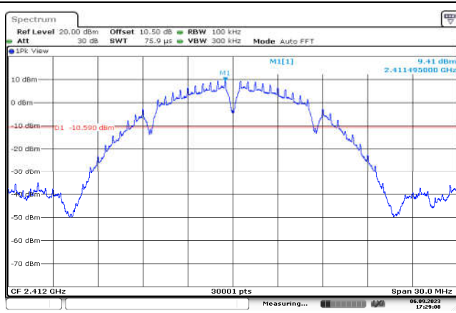
802.11b,2412MHz,Ant0,Plot 1,Reference Level
