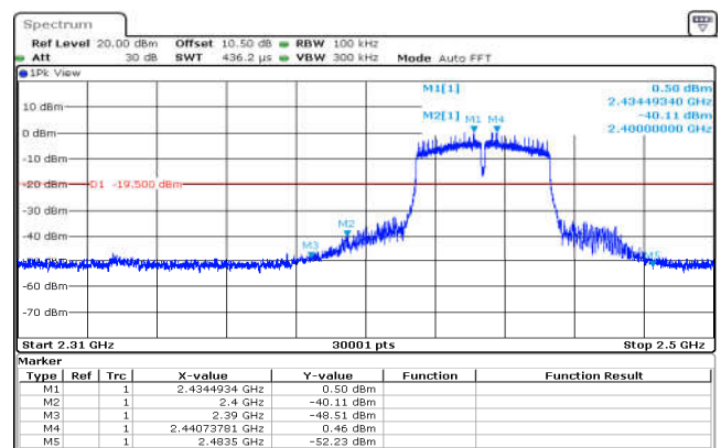
802.11n(HT40),2437MHz,Ant0,Plot 2,Band Edge
