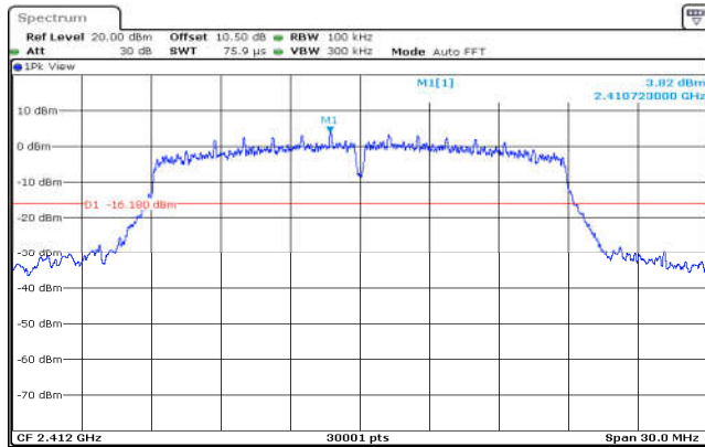
802.11n(HT20),2412MHz,Ant0,Plot 1,Reference Level
