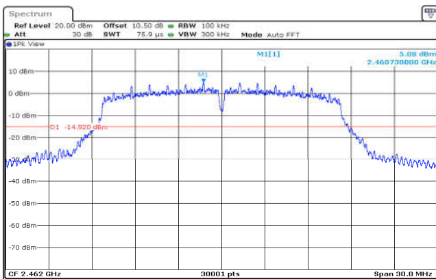
802.11g,2462MHz,Ant0,Plot 1,Reference Level
