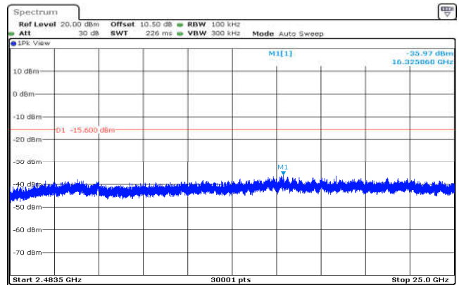
802.11g,2412MHz,Ant0,Plot 4,2483.5MHz ~25000MHz
