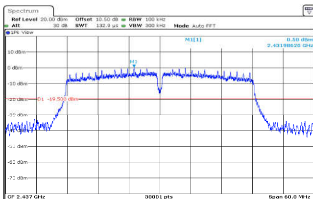
802.11n(HT40),2437MHz,Ant0,Plot 1,Reference Level
