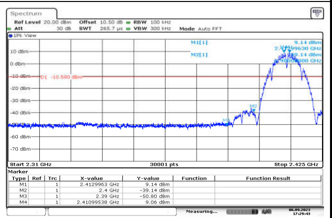
802.11b,2412MHz,Ant0,Plot 2,Band Edge
