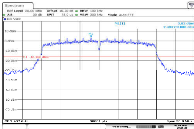
802.11n(HT20),2437MHz,Ant0,Plot 1,Reference Level
