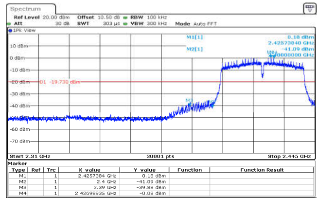
802.11n(HT40),2422MHz,Ant0,Plot 2,Band Edge
