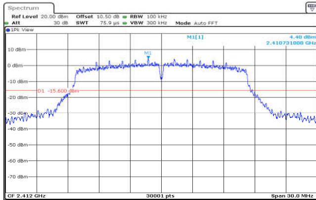
802.11g,2412MHz,Ant0,Plot 1,Reference Level
