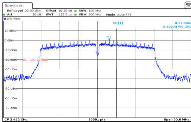
802.11n(HT40),2422MHz,Ant0,Plot 1,Reference Level
