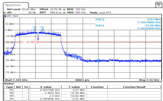
802.11n(HT40),2452MHz,Ant0,Plot 2,Band Edge
