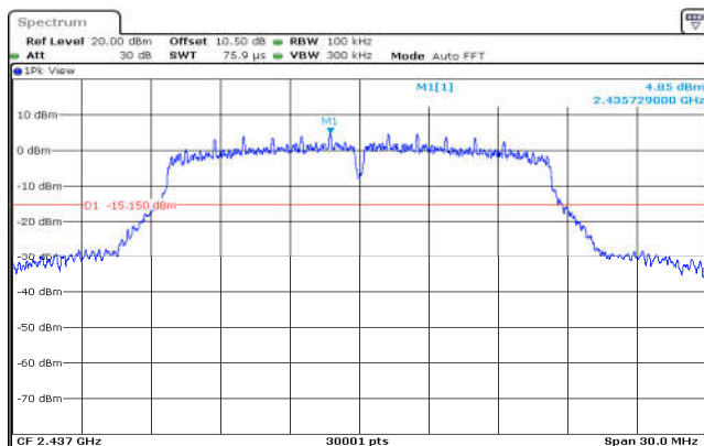
802.11g,2437MHz,Ant0,Plot 1,Reference Level
