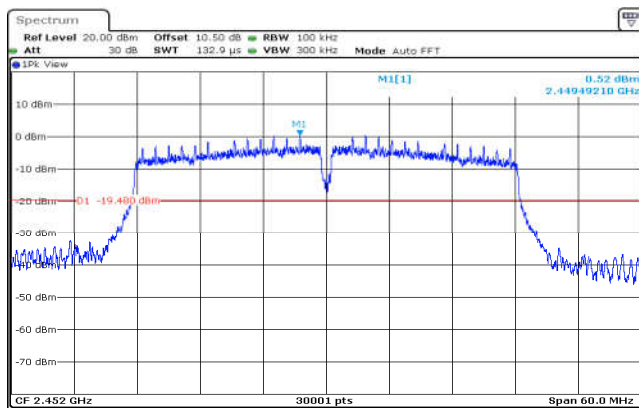
802.11n(HT40),2452MHz,Ant0,Plot 1,Reference Level
