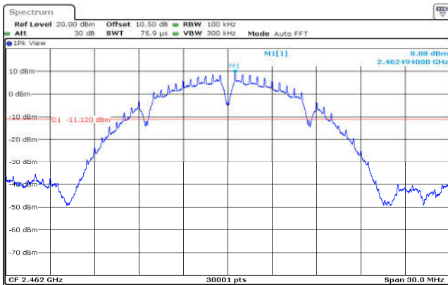
802.11b,2462MHz,Ant0,Plot 1,Reference Level
