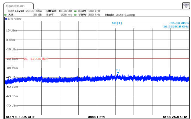
802.11n(HT40),2422MHz,Ant0,Plot 4,2483.5MHz~25000MHz
