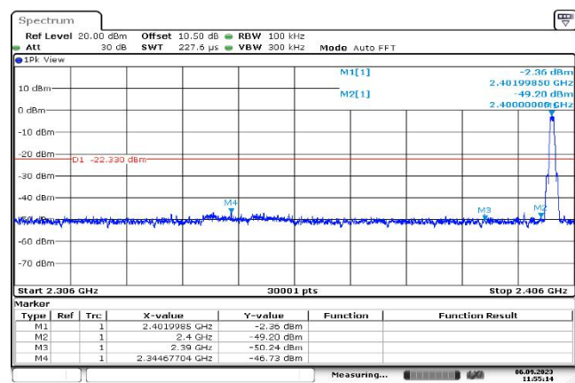
,Plot ,2Conducted Emission: 2402 ,Band Edge
