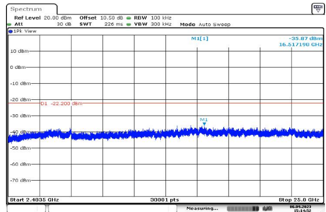
,Plot ,4Transmitter Spurious Emission : 2402,2483.5MHz~25000MHz
