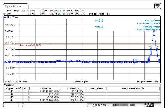
,Plot ,2Conducted Emission: 2402 ,Band Edge
