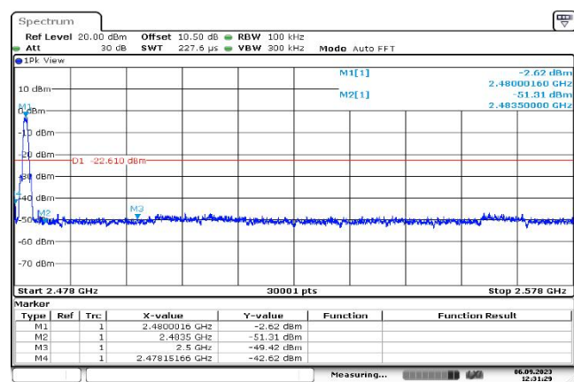
,Plot ,2Conducted Emission: 2480 ,Band Edge
