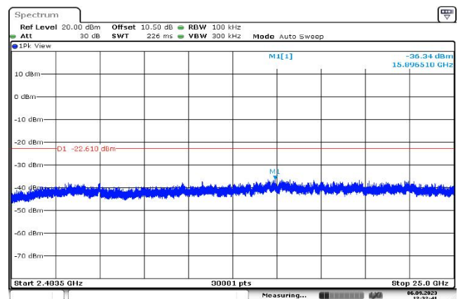
,Plot ,4Transmitter Spurious Emission : 2480,2483.5MHz~25000MHz
