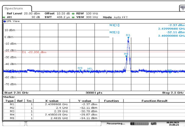
,Plot ,2Conducted Emission: 2440 ,Band Edge
