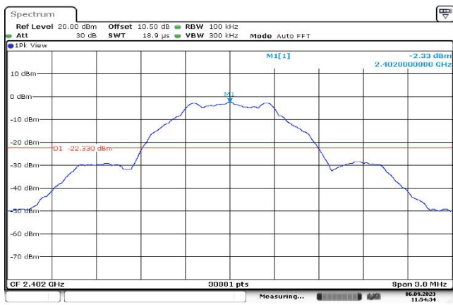
,Plot ,1Transmitter Spurious Emission : 2402,Referecy Level
