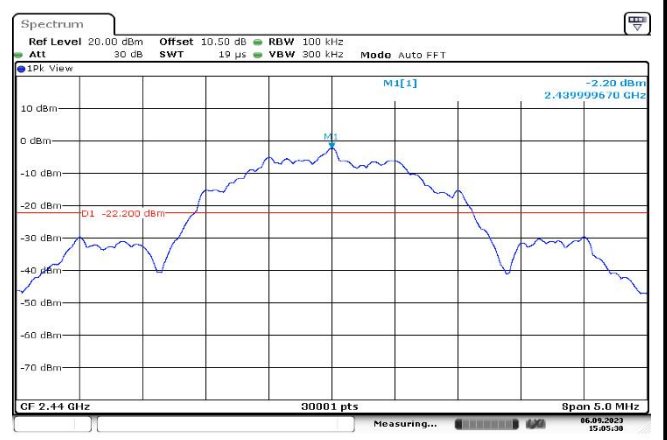
,Plot ,1Transmitter Spurious Emission : 2440,Referecy Level
