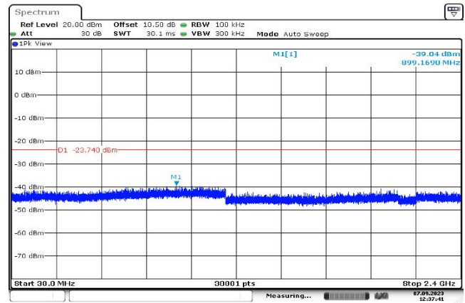
,Plot ,3Transmitter Spurious Emission : 2440,30MHz~2400MHz
