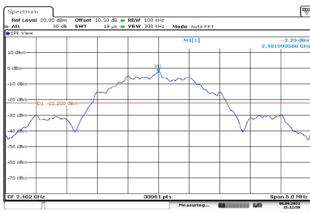
,Plot ,1Transmitter Spurious Emission : 2402,Referecy Level
