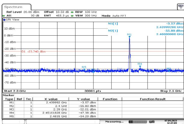
,Plot ,2Conducted Emission: 2440 ,Band Edge
