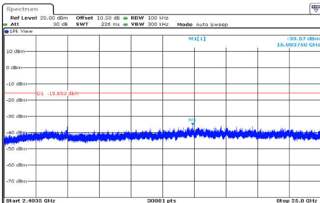
,Plot ,3Conducted Emission: 8DPSK ,2480,3DH5,2483.5MHz~25000MHz
