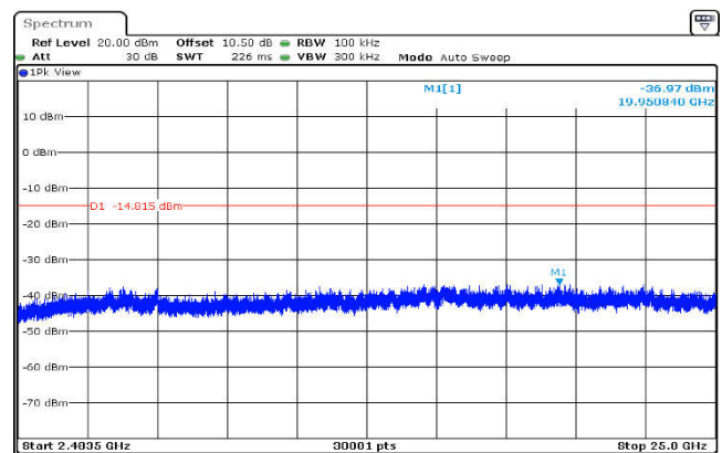
,Plot ,3Conducted Emission: DQPSK ,2480,2DH5,2483.5MHz~25000MHz
