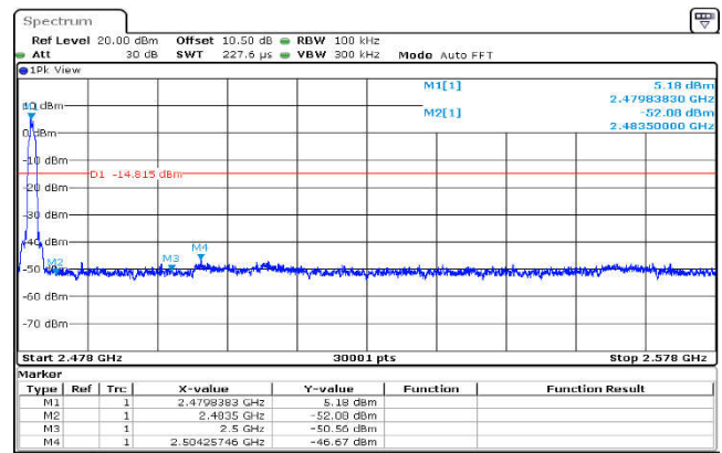
,Plot ,1Conducted Emission: DQPSK ,2480,2DH5,Band Edge HoppingOFF
