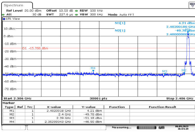
,Plot ,1Conducted Emission: 8DPSK ,2402,3DH5,Band Edge HoppingOFF
