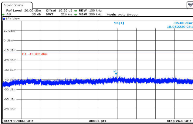
,Plot ,3Conducted Emission: GFSK ,2402,DH5,2483.5MHz~25000MHz
