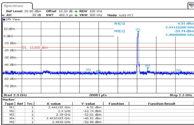
,Plot ,1Conducted Emission: DQPSK ,2441,2DH5,Band Edge HoppingOFF
