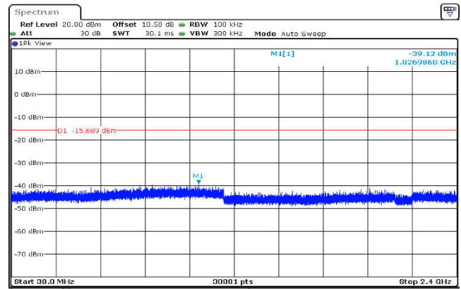
,Plot ,2Conducted Emission: DQPSK ,2441,2DH5,30MHz~2400MHz
