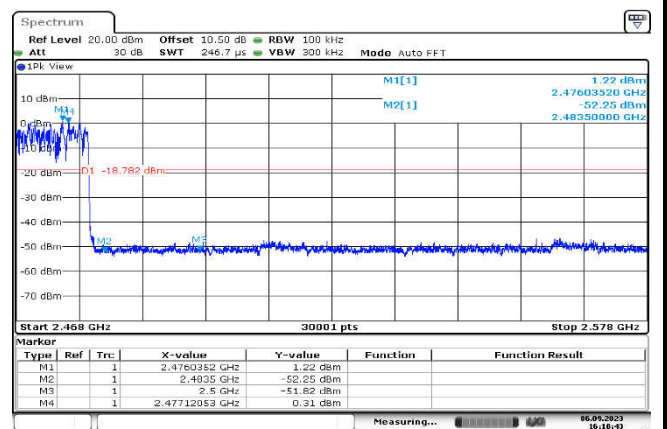
Conducted Emission: DQPSK,2480,2DH5 ,Band Edge
