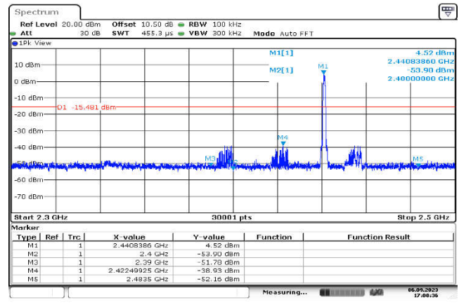
,Plot ,1Conducted Emission: 8DPSK ,2441,3DH5,Band Edge HoppingOFF
