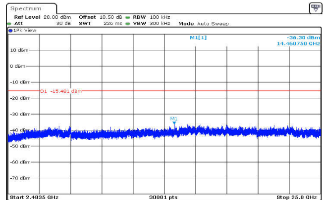
,Plot ,3Conducted Emission: 8DPSK ,2441,3DH5,2483.5MHz~25000MHz
