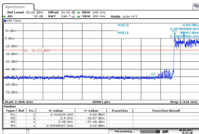
Conducted Emission: 8DPSK,2402,3DH5 ,Band Edge
