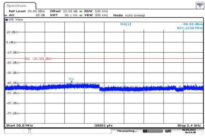
,Plot ,2Conducted Emission: 8DPSK ,2402,3DH5,30MHz~2400MHz
