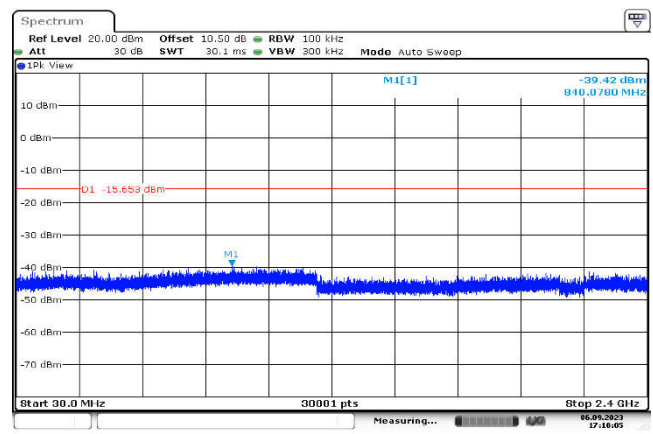
,Plot ,2Conducted Emission: 8DPSK ,2480,3DH5,30MHz~2400MHz
