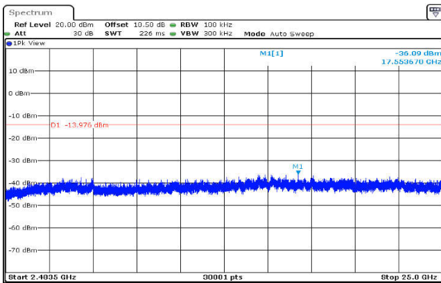
,Plot ,3Conducted Emission: GFSK ,2480,DH5,2483.5MHz~25000MHz
