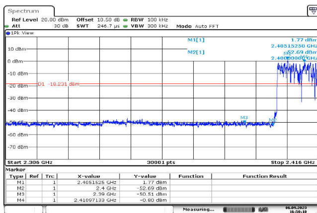
Conducted Emission: DQPSK,2402,2DH5 ,Band Edge
