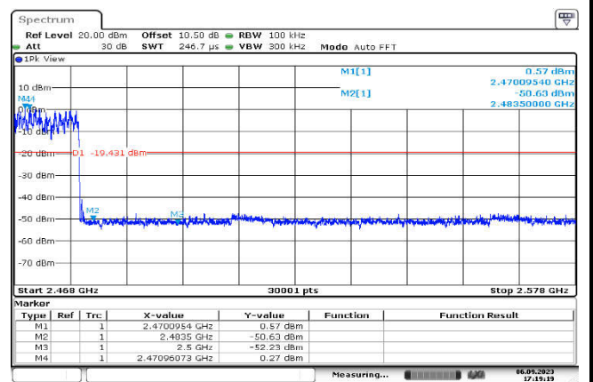
Conducted Emission: 8DPSK,2480,3DH5 ,Band Edge
