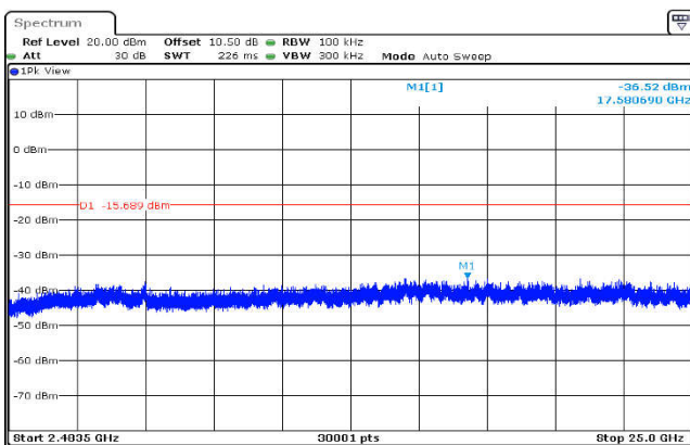
,Plot ,3Conducted Emission: DQPSK ,2441,2DH5,2483.5MHz~25000MHz
