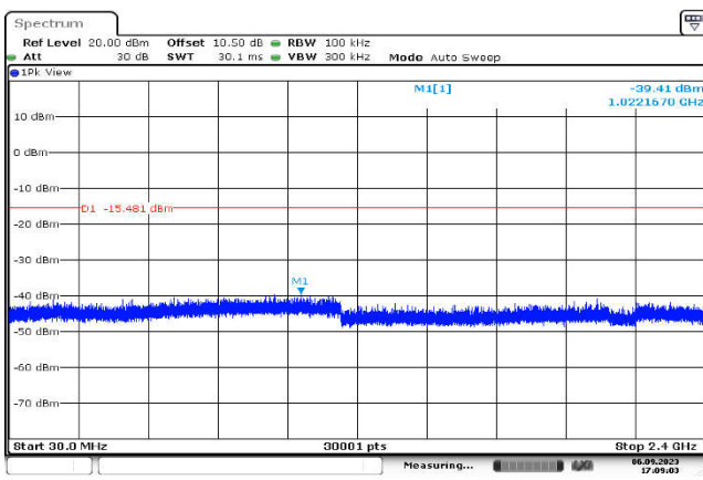
,Plot ,2Conducted Emission: 8DPSK ,2441,3DH5,30MHz~2400MHz
