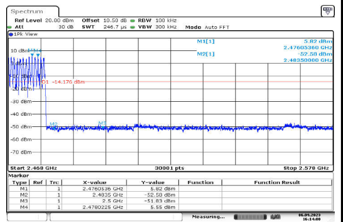
Conducted Emission: GFSK,2480,DH5 ,Band Edge
