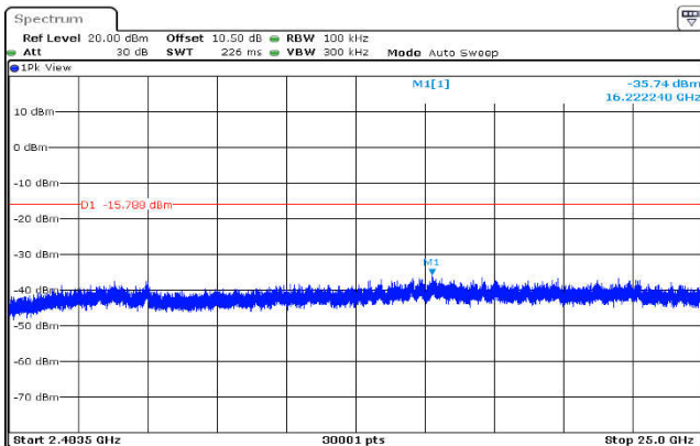
,Plot ,3Conducted Emission: 8DPSK ,2402,3DH5,2483.5MHz~25000MHz
