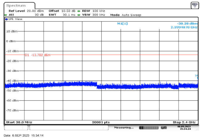
,Plot ,2Conducted Emission: GFSK ,2480,DH5,30MHz~2400MHz
