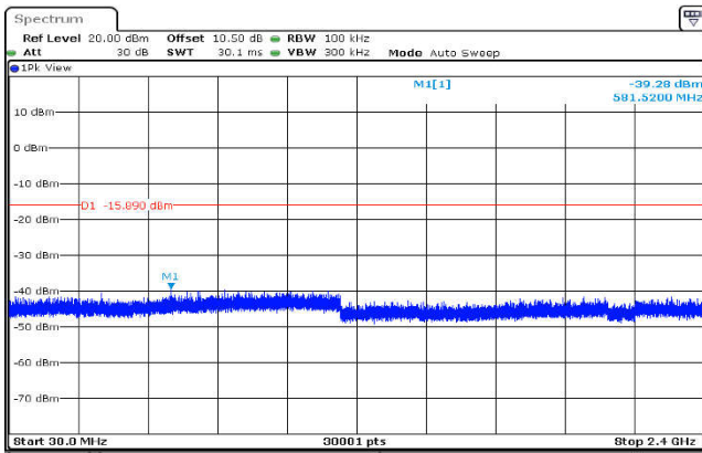
,Plot ,2Conducted Emission: DQPSK ,2402,2DH5,30MHz~2400MHz
