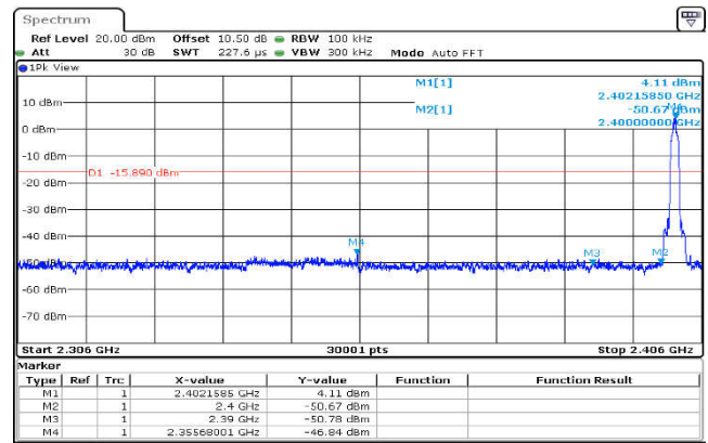
,Plot ,1Conducted Emission: DQPSK ,2402,2DH5,Band Edge HoppingOFF
