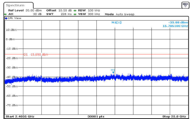
,Plot ,3Conducted Emission: DQPSK ,2402,2DH5,2483.5MHz~25000MHz
