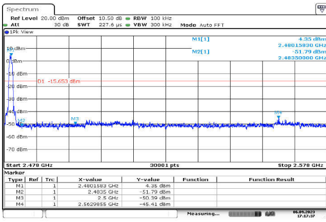
,Plot ,1Conducted Emission: 8DPSK ,2480,3DH5,Band Edge HoppingOFF
