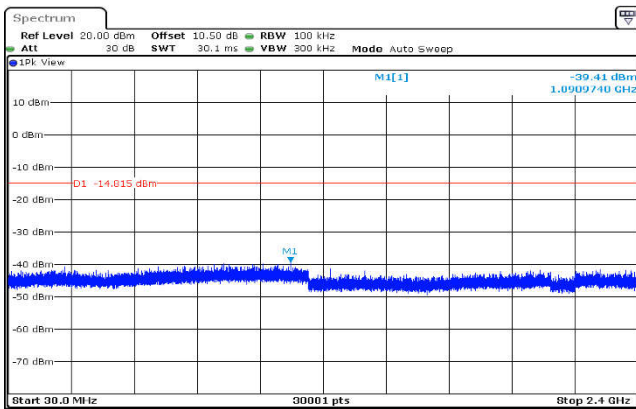
,Plot ,2Conducted Emission: DQPSK ,2480,2DH5,30MHz~2400MHz
