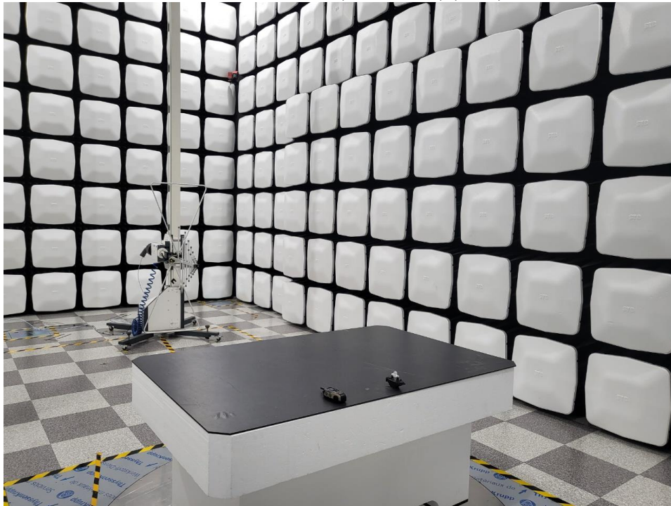
Radiated Emission (Below 1 GHz) (Rear)
