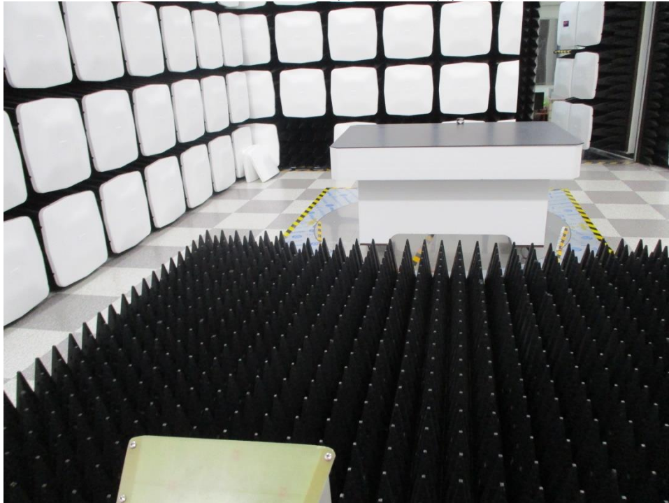
Radiated Emission (Above 1 GHz) (Rear)
