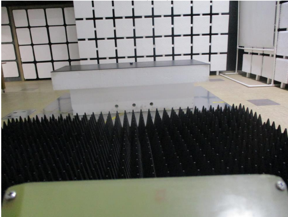
Radiated Emission (Front)_Above 1 GHz
